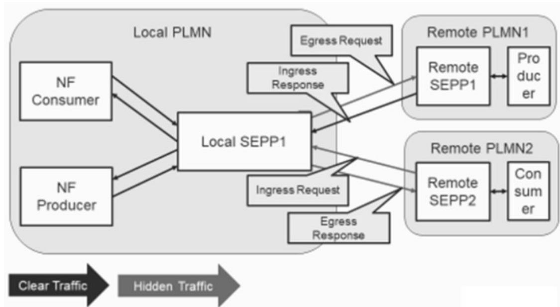
Figure 3-14 Topology Hiding Architecture
