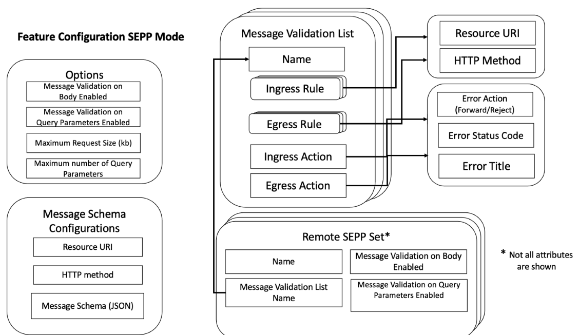
Figure 3-57 CNC Console options available for Cat-0 SBI Message Schema Validation feature in SEPP Mode
