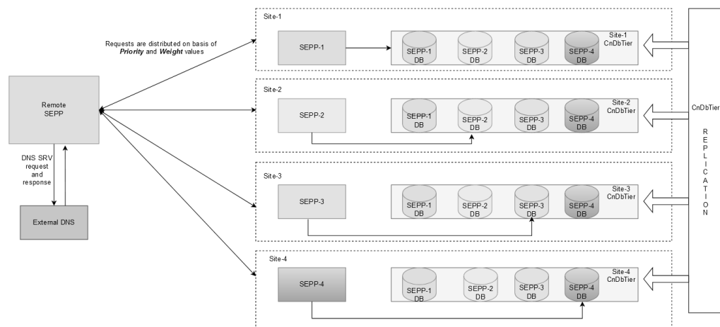
Figure 3-46 Georedundancy Overview
