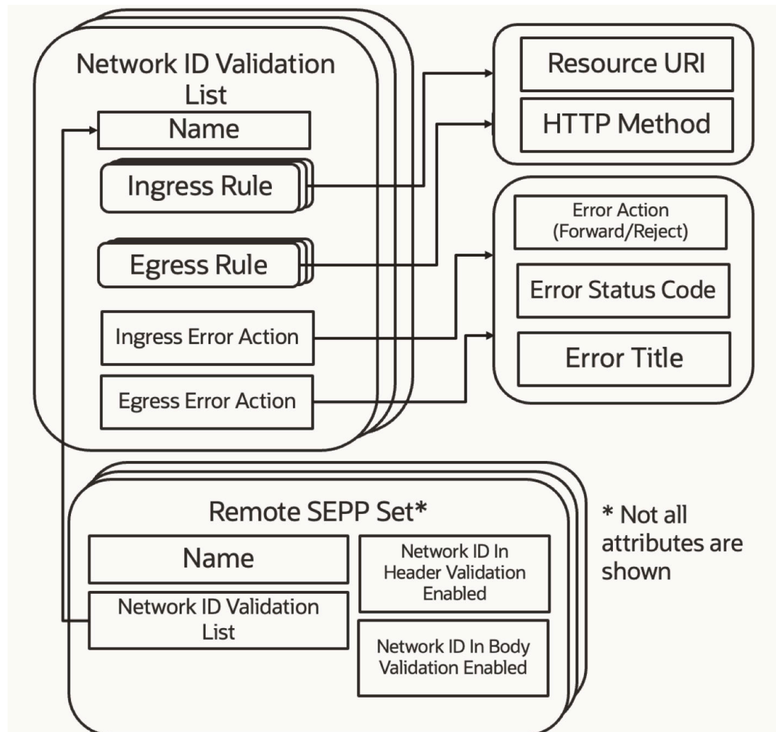
Figure 3-63 Feature Configuration – Network ID Validation List
