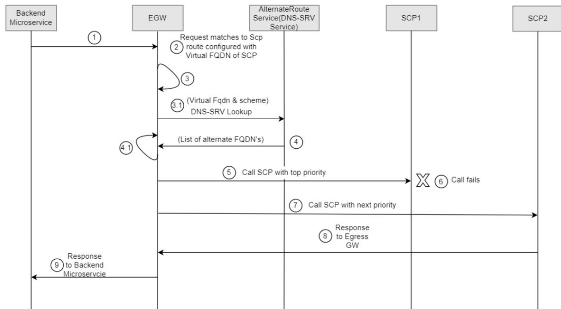
Figure 3-52 Priority Based Routing
