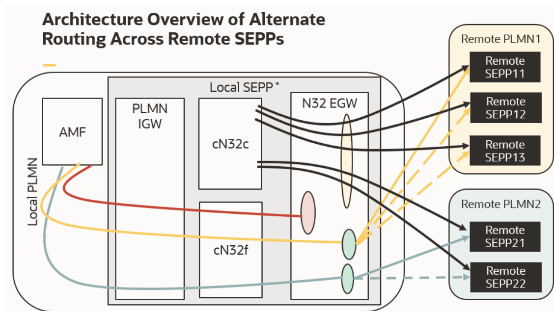
Figure 3-28 Architecture
