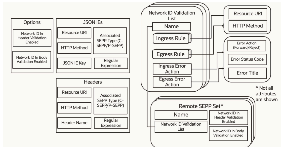
Figure 3-62 CNC Console options available for Cat 2 – Network ID Validation
