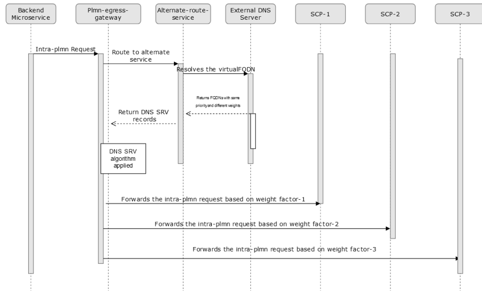
Figure 3-53 Weight Based Routing or Load Sharing
