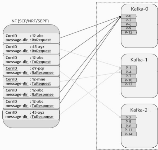
Figure 3-37 Same Kafka partition for the messages of the same transaction type
