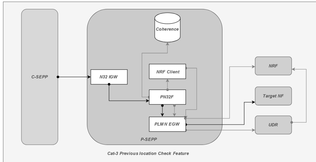
Figure 3-64 Design and Architecture
