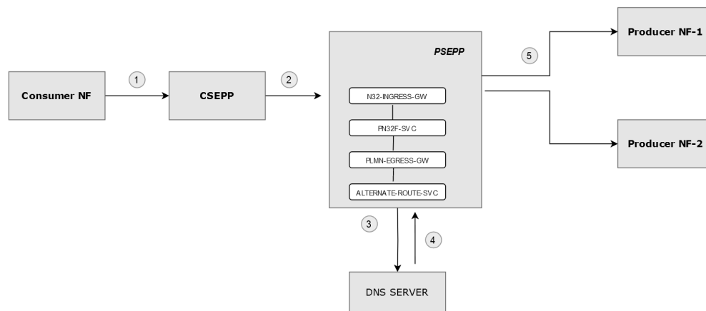
Figure 3-51 Routing to Producer NFs Through DNS SRV
