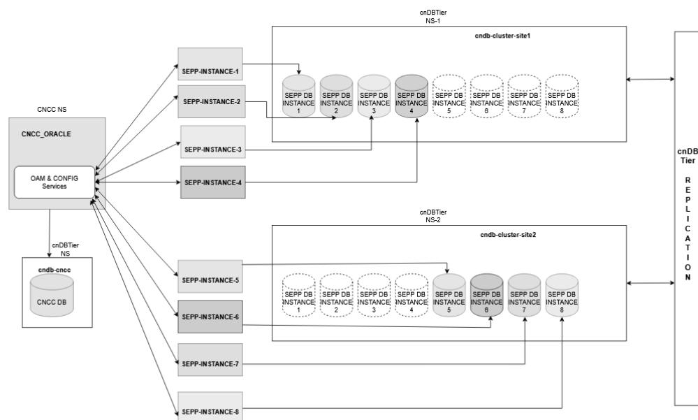
Figure 3-3 Multiple SEPP instances on shared cnDBTier cluster architecture
