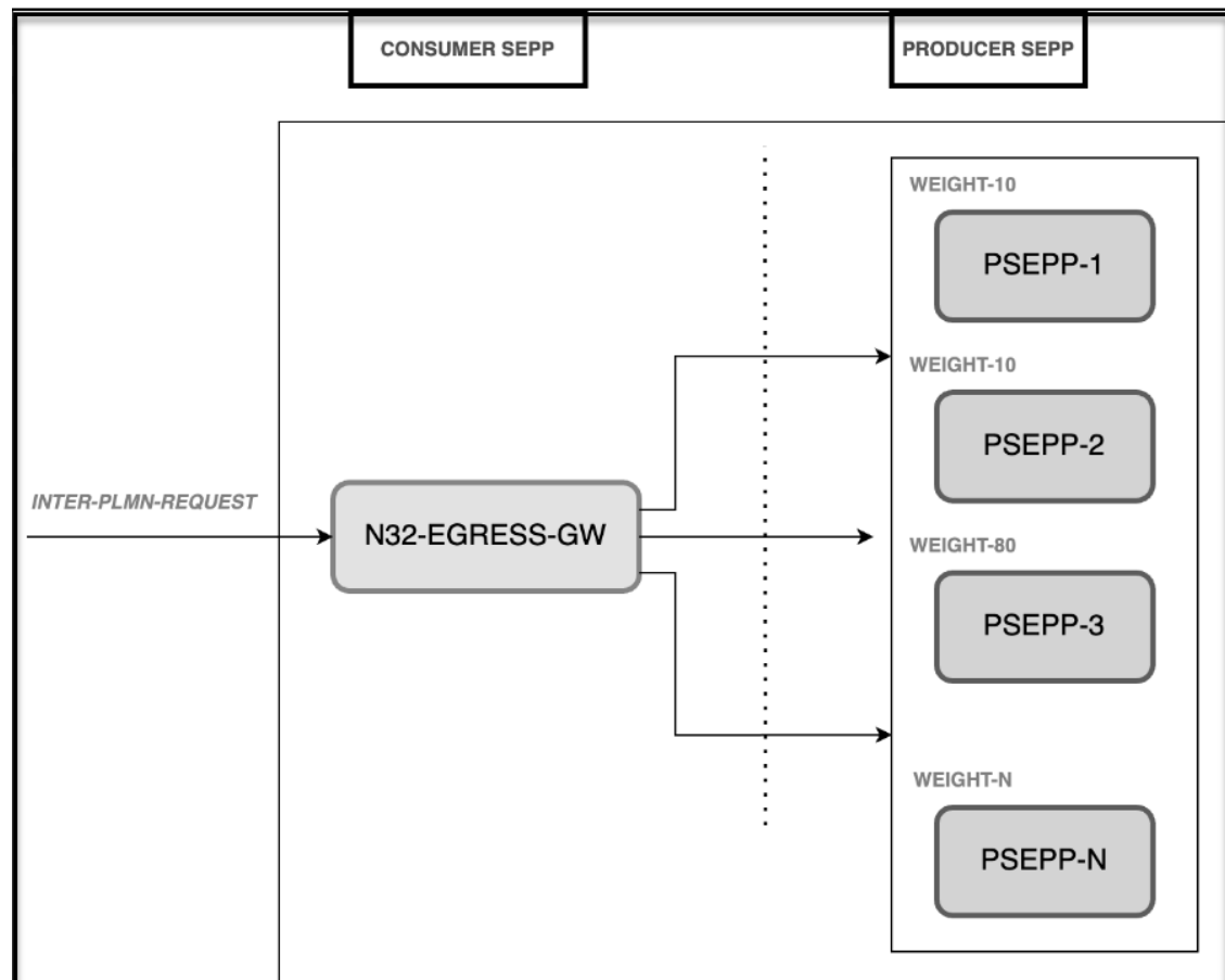
Figure 3-10 Architecture
