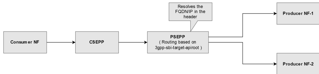
Figure 3-50 Direct Communication
