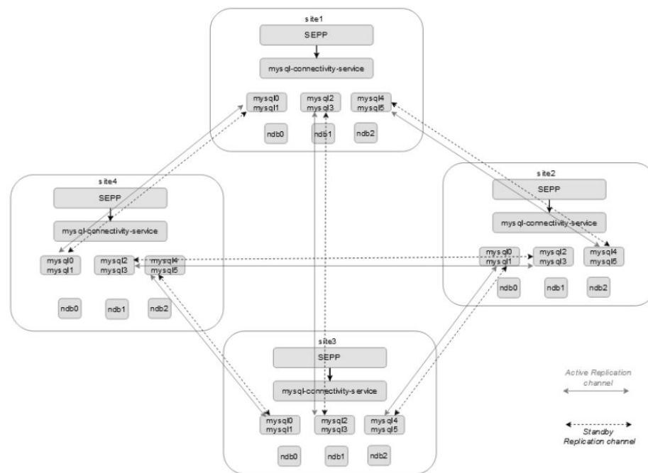
Figure 3-49 Four-site Georedundancy
