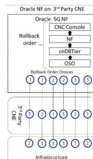
Figure 3-4 Rollback Sequence with Non-Oracle CNE
