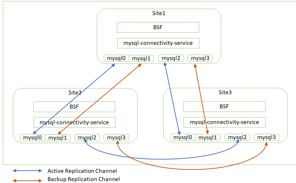
Figure 3-21 Three-Site Georedundancy
