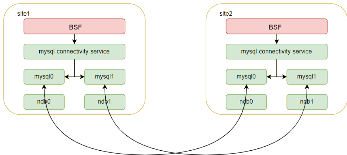
Figure 3-20 Two-Site Georedundancy
