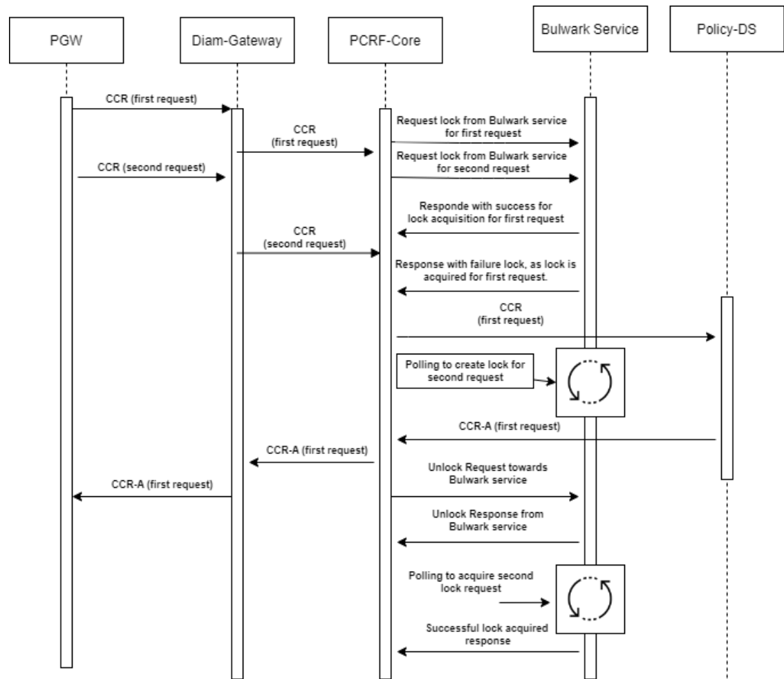
Figure 4-187 CCR-I, CCR-U and CCR-T messages Integration with Bulwark Service
