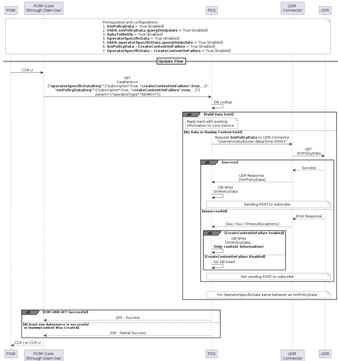
Figure 4-66 PDS Dummy Context Creation during SM or PCRF Core Update Call Flow
