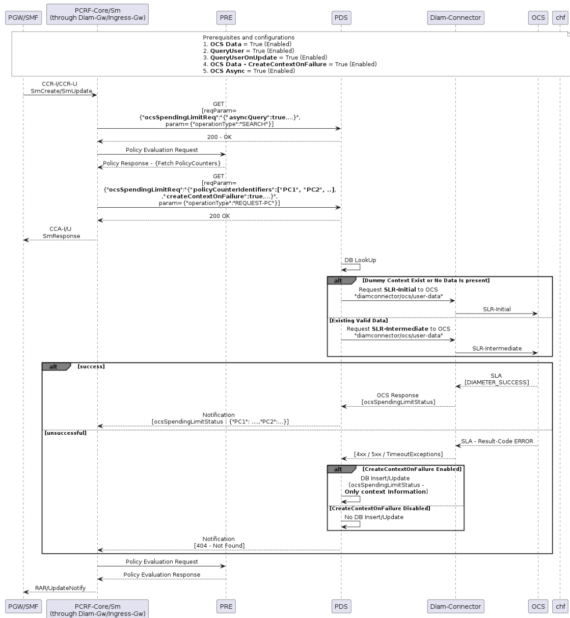
Figure 4-67 PDS Dummy Context Creation during SM and PCRF Core Create/Update Call Flow with OCS in Async Mode
