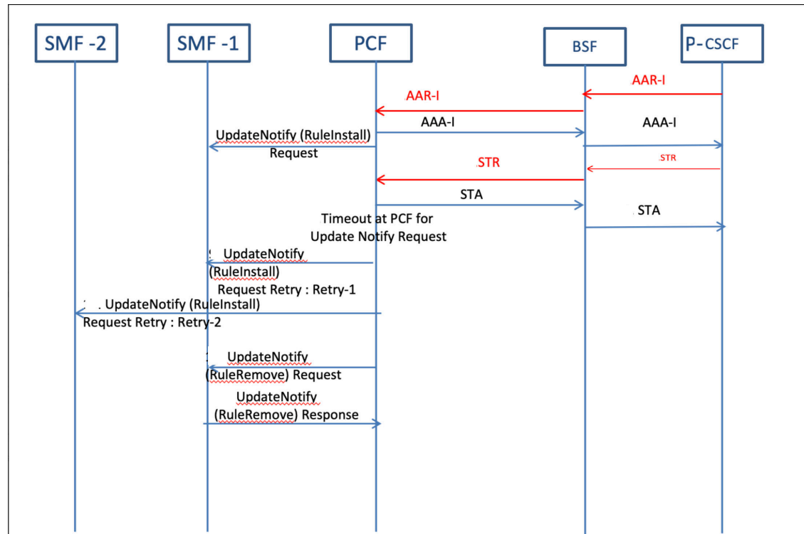
Figure 4-18 Handling Collision Between AAR and STR Messages During UpdateNotify Timeout
