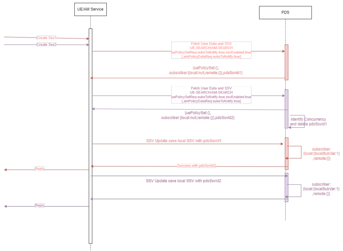
Figure 4-222 State variables in concurrent flows
