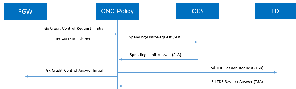
Figure 4-193 Call Flow for TDF Session
