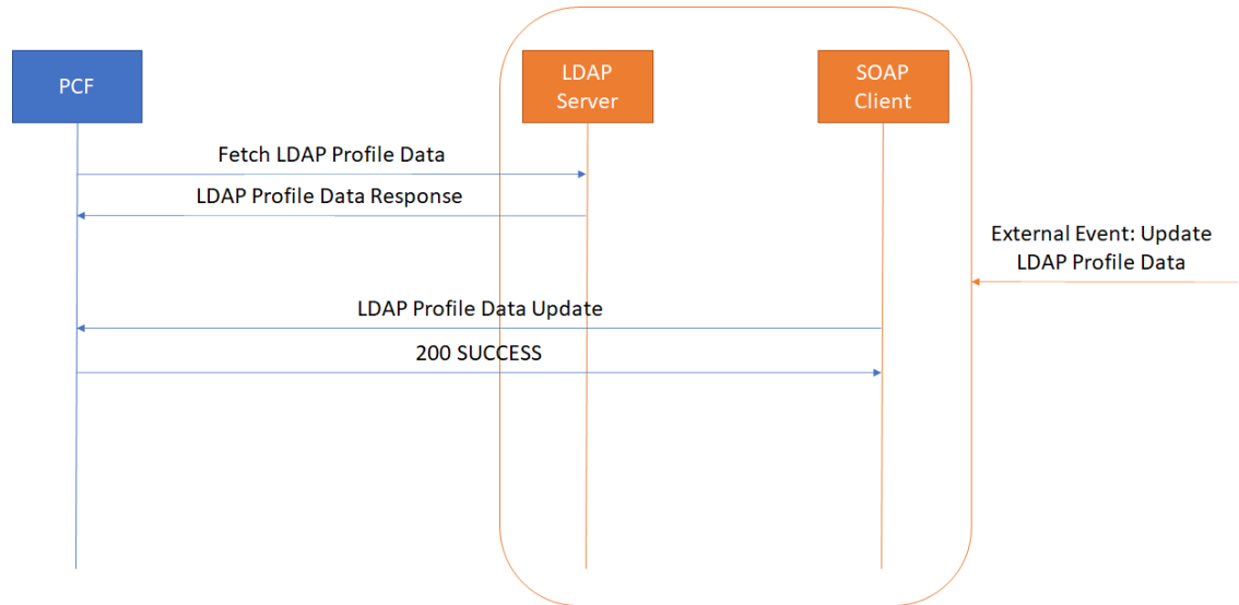
Figure 4-148 Fetching subscriber data
