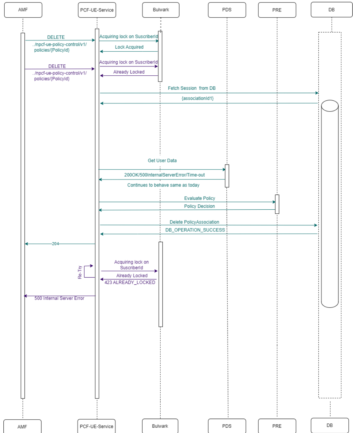
Figure 4-182 Two UE-Delete requests for same Subscriber and retry failure (retry=1)
