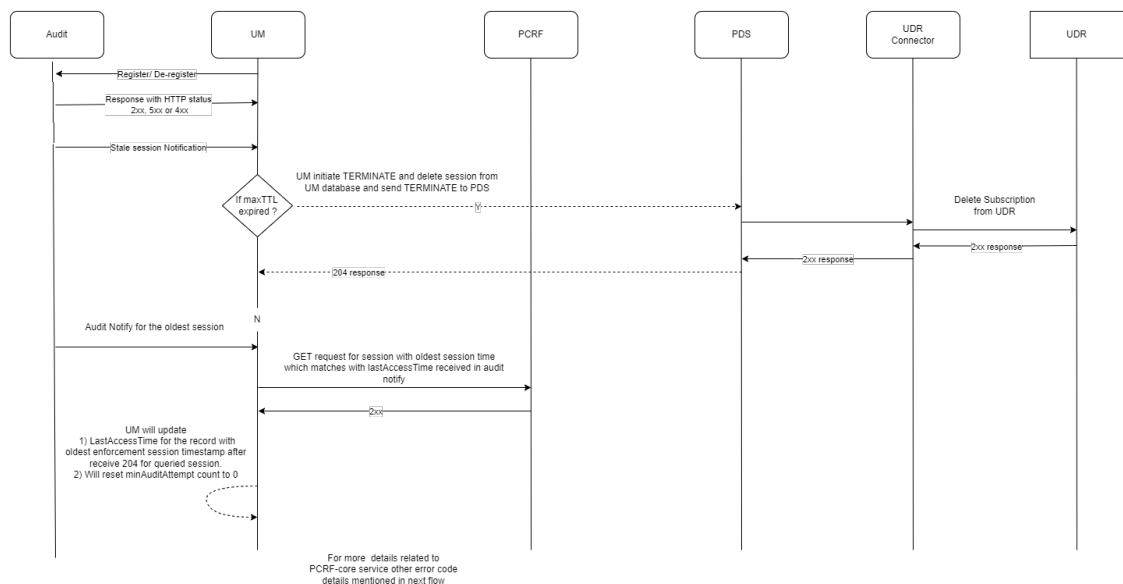
Figure 4-141 Example call flow for Stale Session Detection and Handling in Usage Monitoring Service
