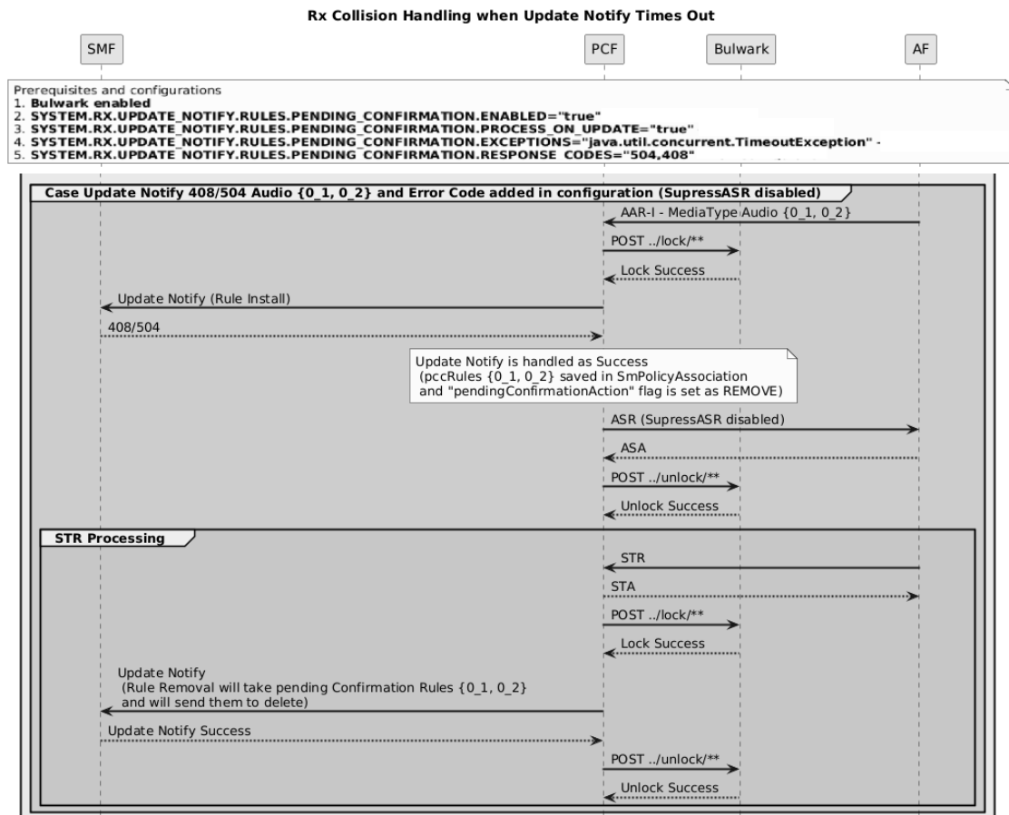
Figure 4-23 Handling Collision Between AAR and STR Messages During UpdateNotify-408 or 504 Errors from SMF When Error Codes are Configured
