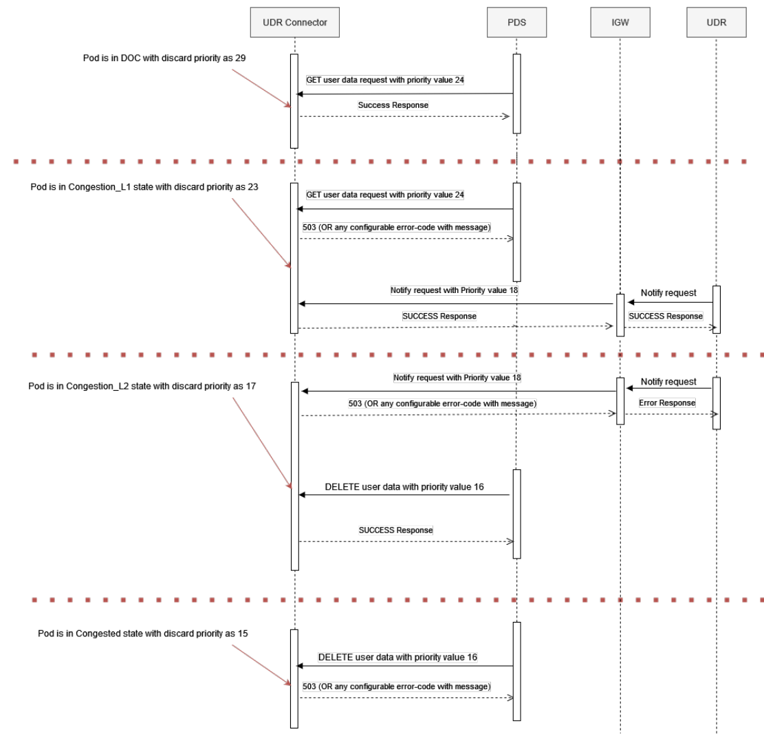
Figure 4-34 Call flow diagram for UDR Connector Congestion Control
