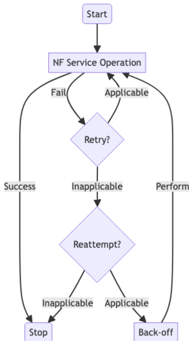
Figure 4-25 Reattempt Flow Chart
