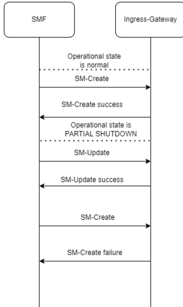
Figure 4-203 Call Flow for Ingress Gateway PARTIAL SHUTDOWN
