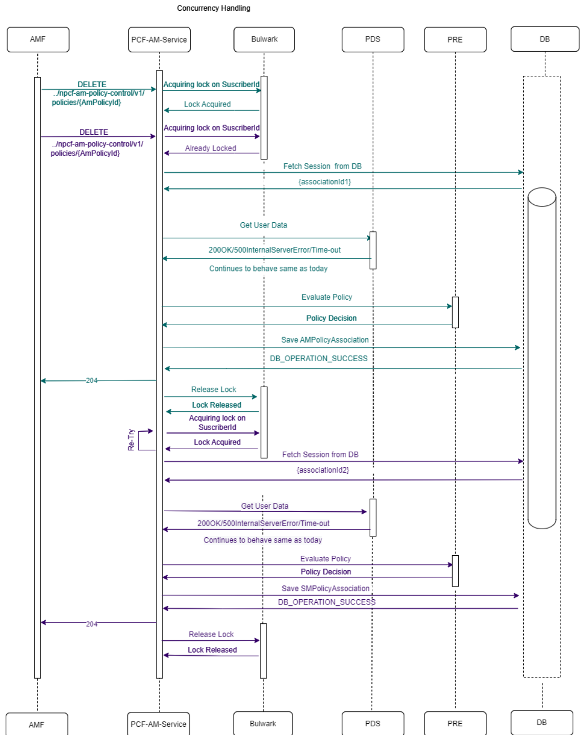
Figure 4-173 Two AM-Delete requests for same Subscriber and retry success
