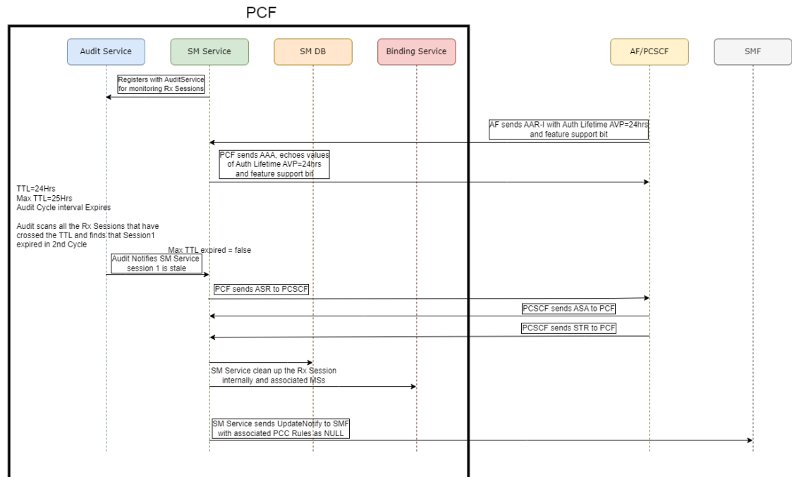
Figure 4-99 Rx Stale Session Detection and Deletion Based on TTL and Authorization-Lifetime
