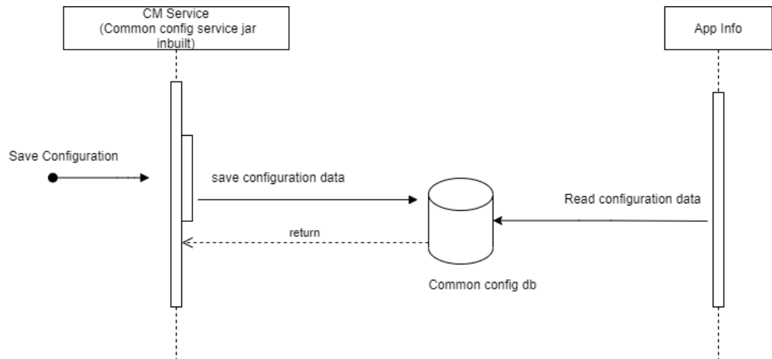
Figure 4-214 Call flow to Save Configuration Data
