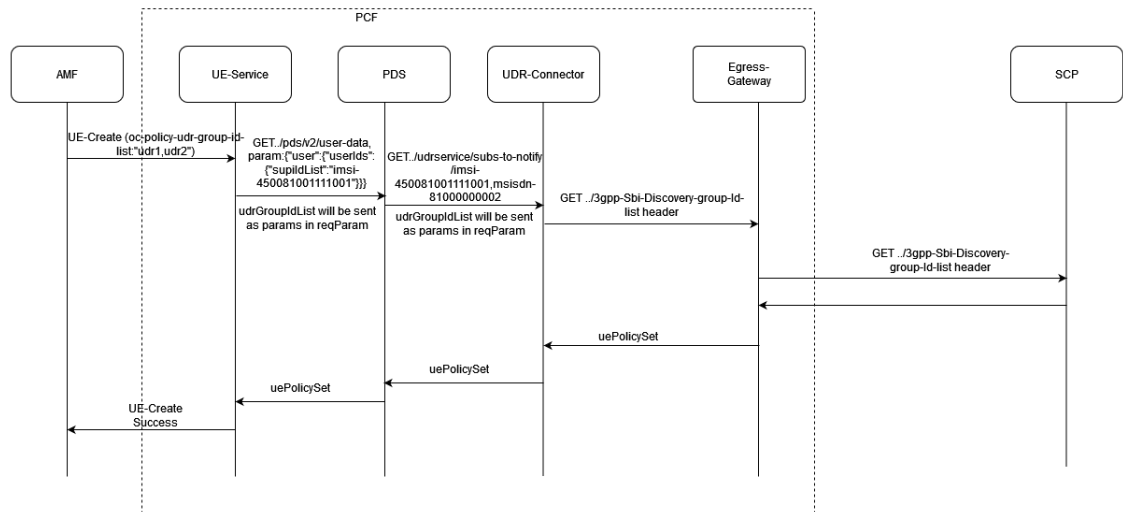
Figure 4-96 Model D, AMF sends UE Policy Association Request with oc-policy-udr-group-id-list
