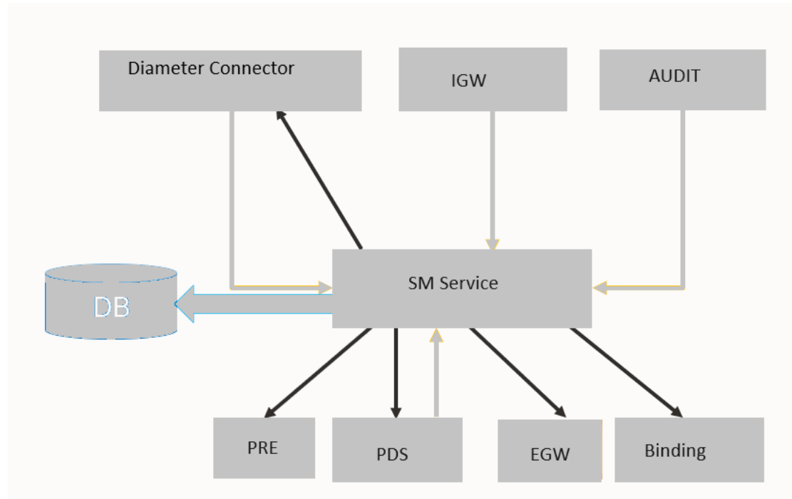
Figure 4-36 Policy Services and SM service interaction
