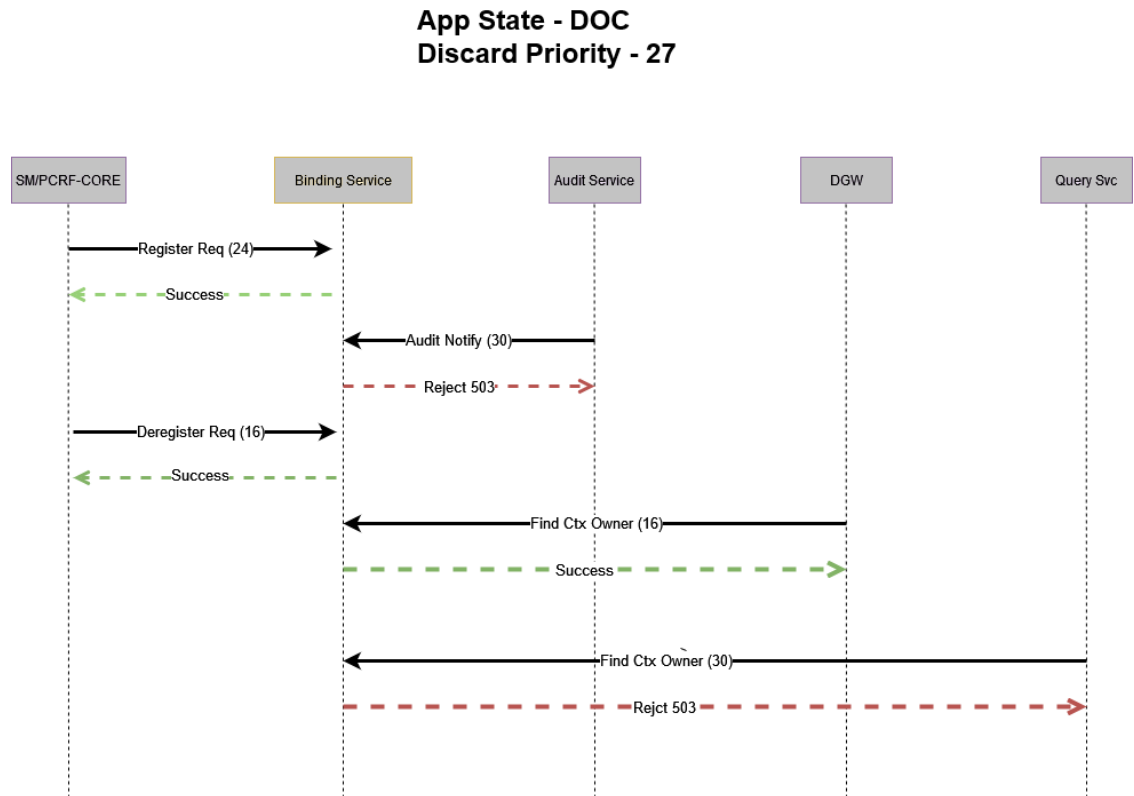
Figure 4-42 Binding Service Pod in DOC State
