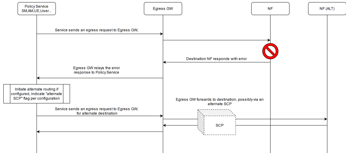
Figure 4-128 Egress Gateway get Error Response
