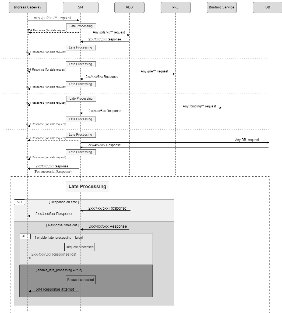
Figure 4-53 Sample call flow for stale requests cleanup by SM Service
