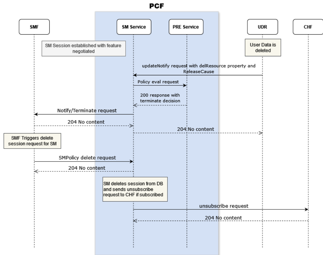
Figure 4-90 SM Terminate for UDR updateNotify with (or without) delResources:
