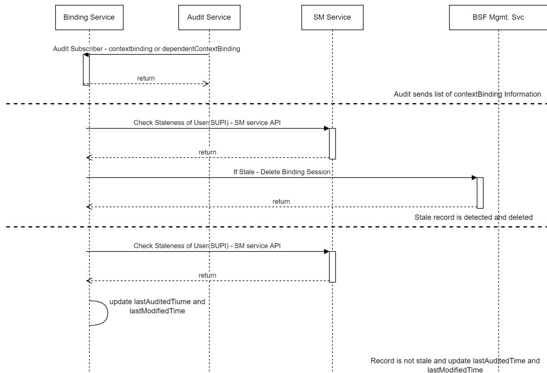
Figure 4-140 Example call flow for Stale Session Detection and Handling in Binding Service
