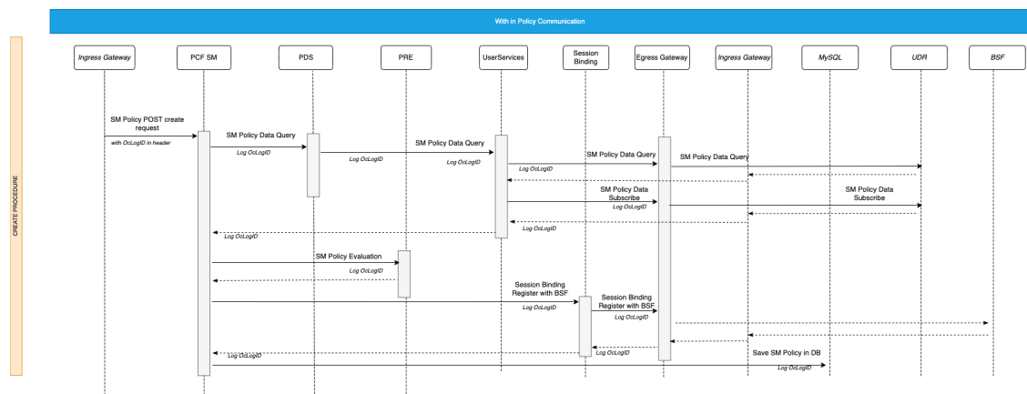
Figure 4-60 Example: Unique Identifier for SM Create Call Flow
