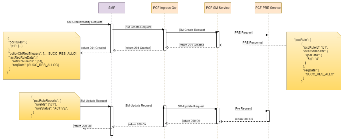
Figure 4-216 PCC Rule for SM Create and SM Update requests
