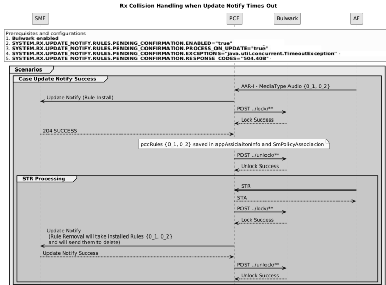
Figure 4-19 Handling Collision Between AAR and STR Messages During Update Notify-Success Scenario
