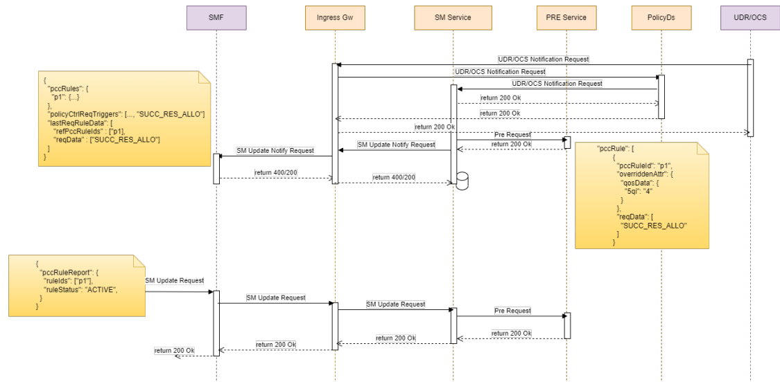
Figure 4-217 PCC Rule in SM-UPDATE-NOTIFY request (Re-authorization)
