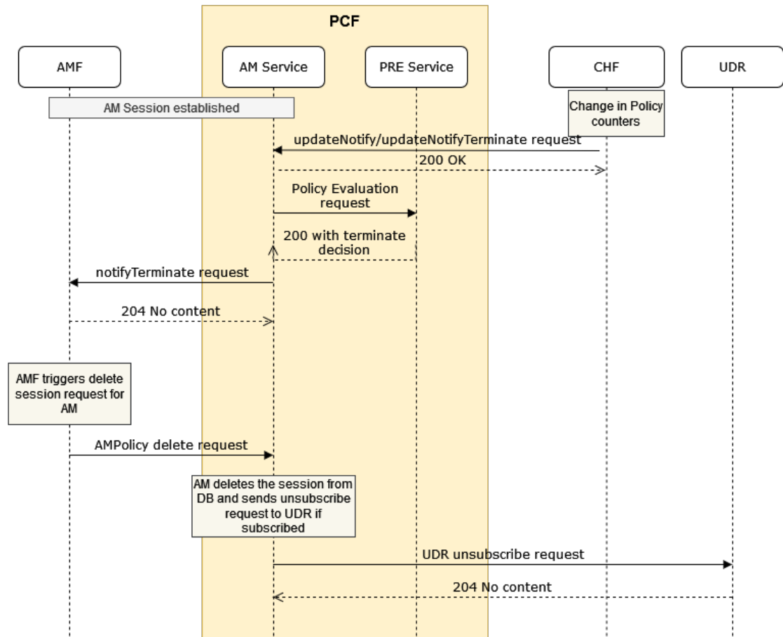
Figure 4-85 Call Flow for AM Terminate for CHF updateNotify or TerminateNotify
