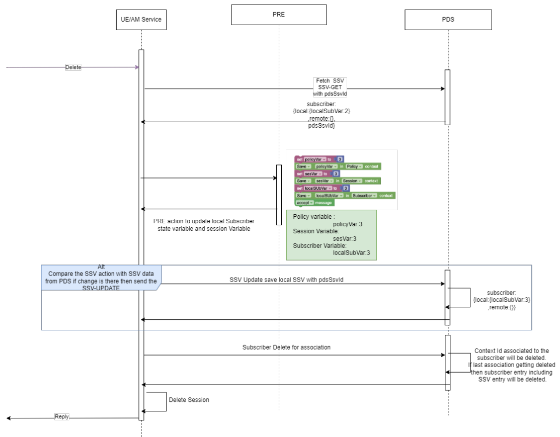
Figure 4-221 State variables in delete session call flow
