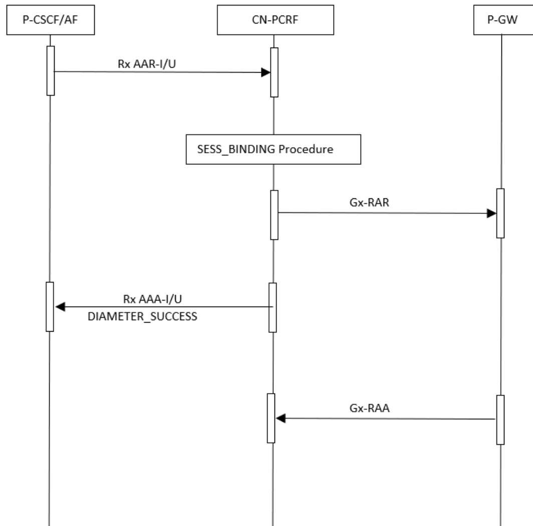
Figure 4-122 Subscription to notification of the AF Signaling Transmission in 4G
