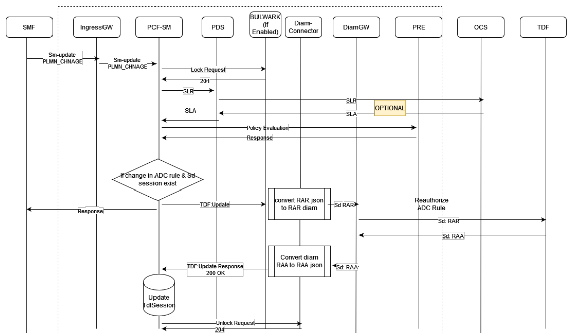
Figure 4-8 Sd Session Modification from PCF to TDF when PLMN Change
