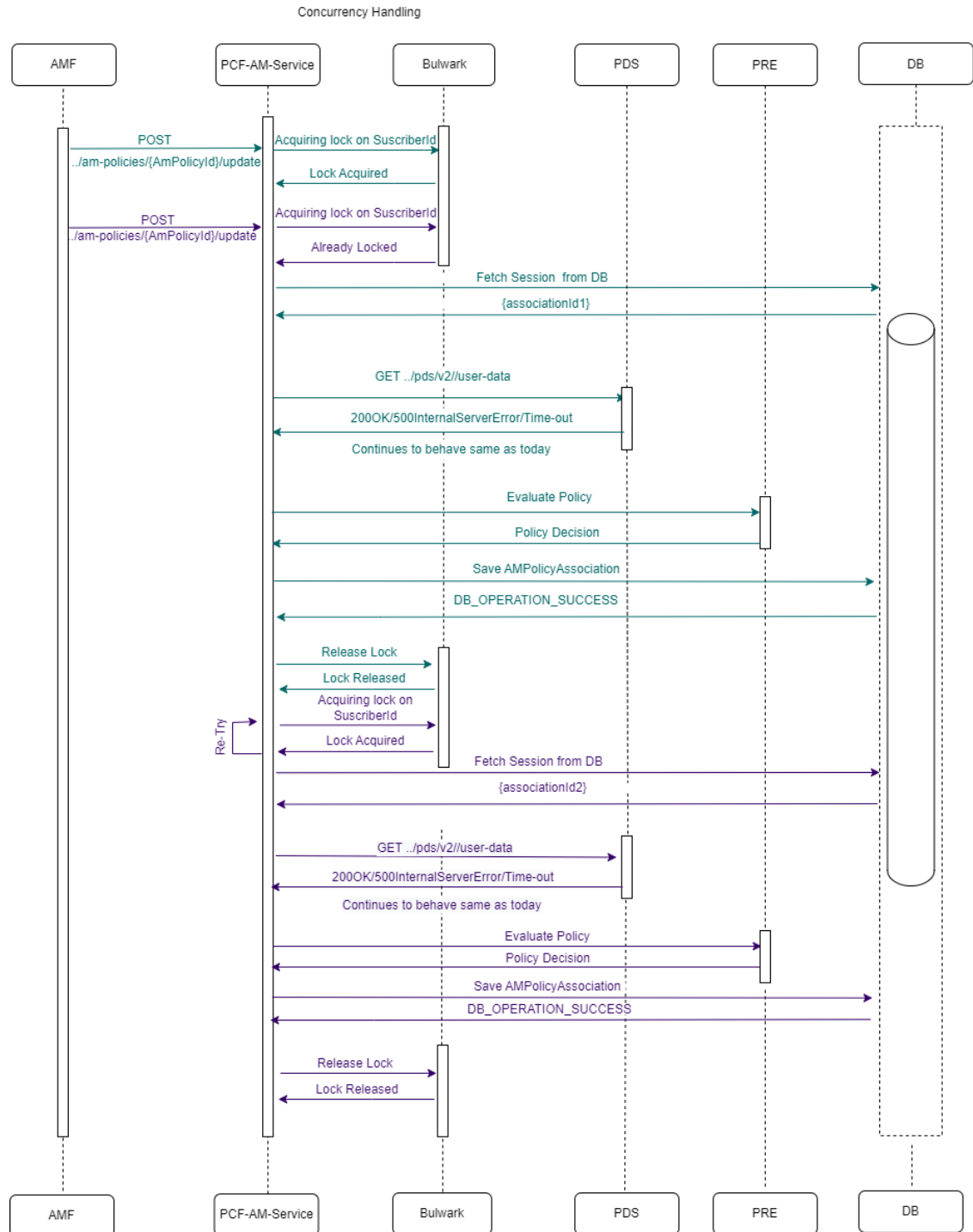
Figure 4-175 Two AM-Update requests for same Subscriber but different Sessions and retry success
