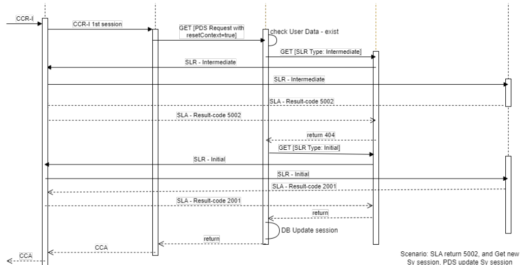
Figure 4-75 SLA Returns 5002, Get New Sy Session, PDS Update Sy Session
