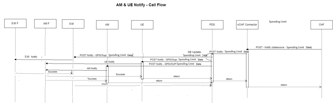
Figure 4-212 Update notification to SM service, AM service, and UE Policy service
