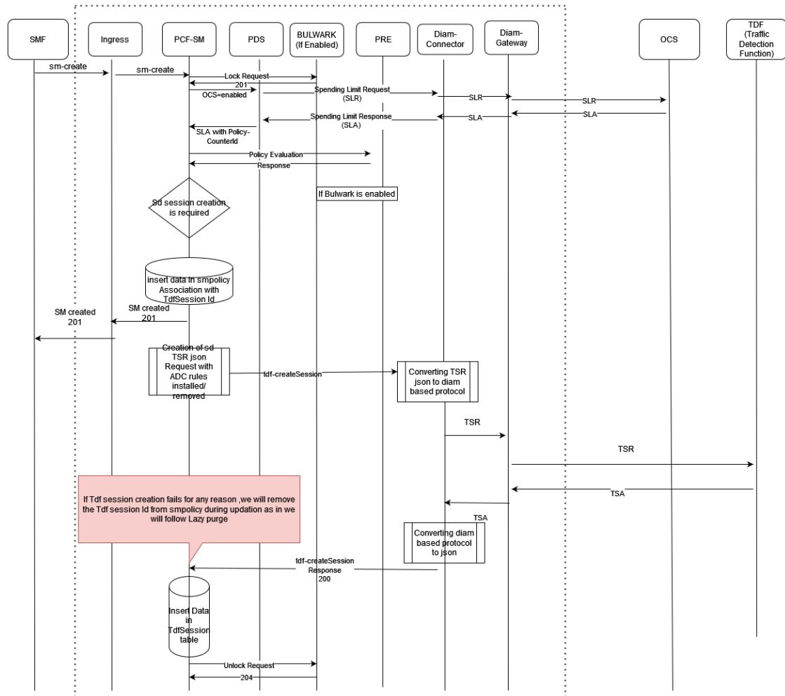
Figure 4-7 Sd Session Establishment (PCF → TDF)
