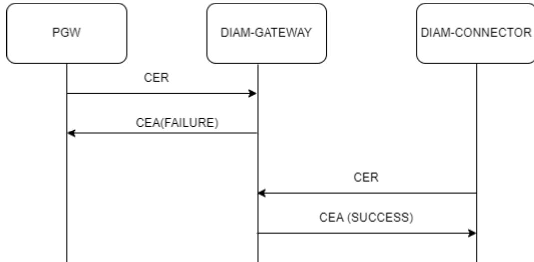
Figure 4-201 Call Flow for Diameter Gateway COMPLETE SHUTDOWN
