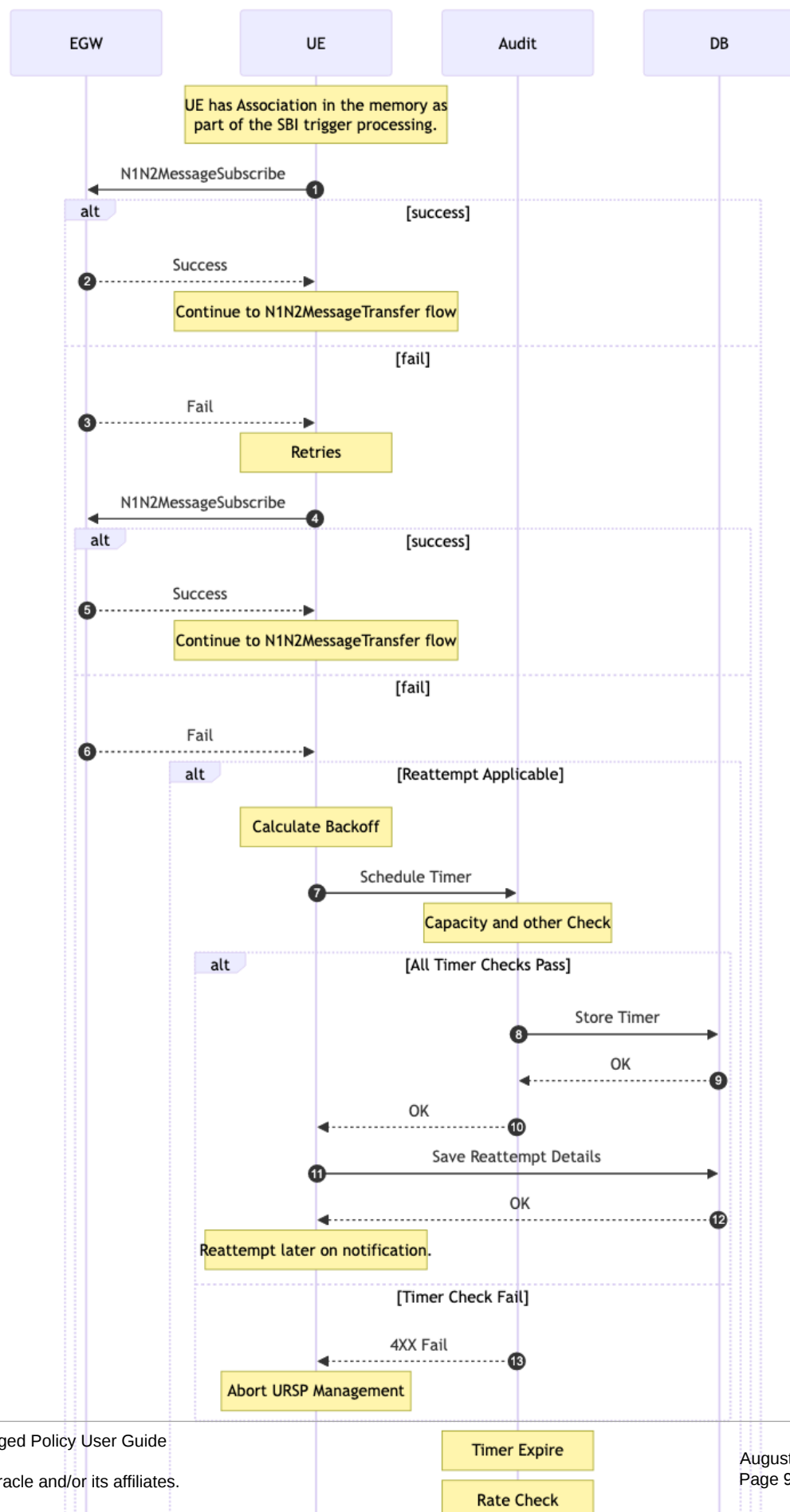
Figure 4-29 N1N2MessageSubscribe Call Flow
