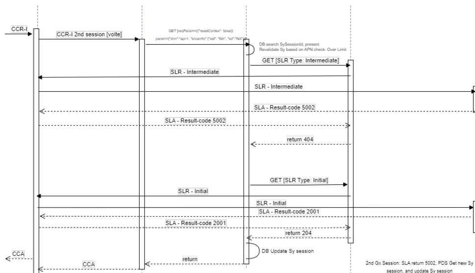
Figure 4-78 Second Gx Session: SLA Returns 5002, Get New Sy Session, PDS Update Sy Session
