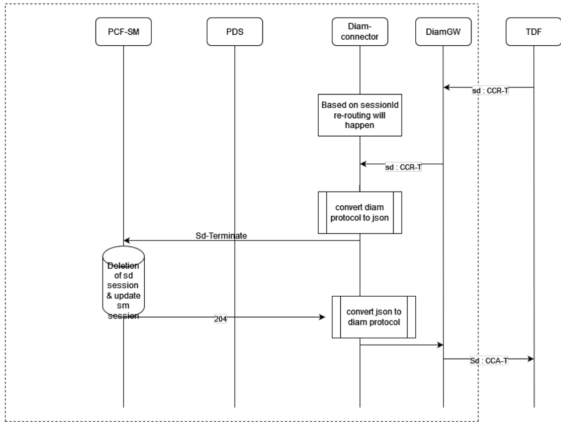
Figure 4-11 Sd Session Termination (TDF → PCF)
