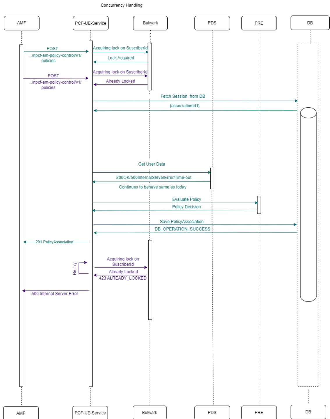
Figure 4-180 Two UE-Create requests for same Subscriber and retry failure (retry =1)
