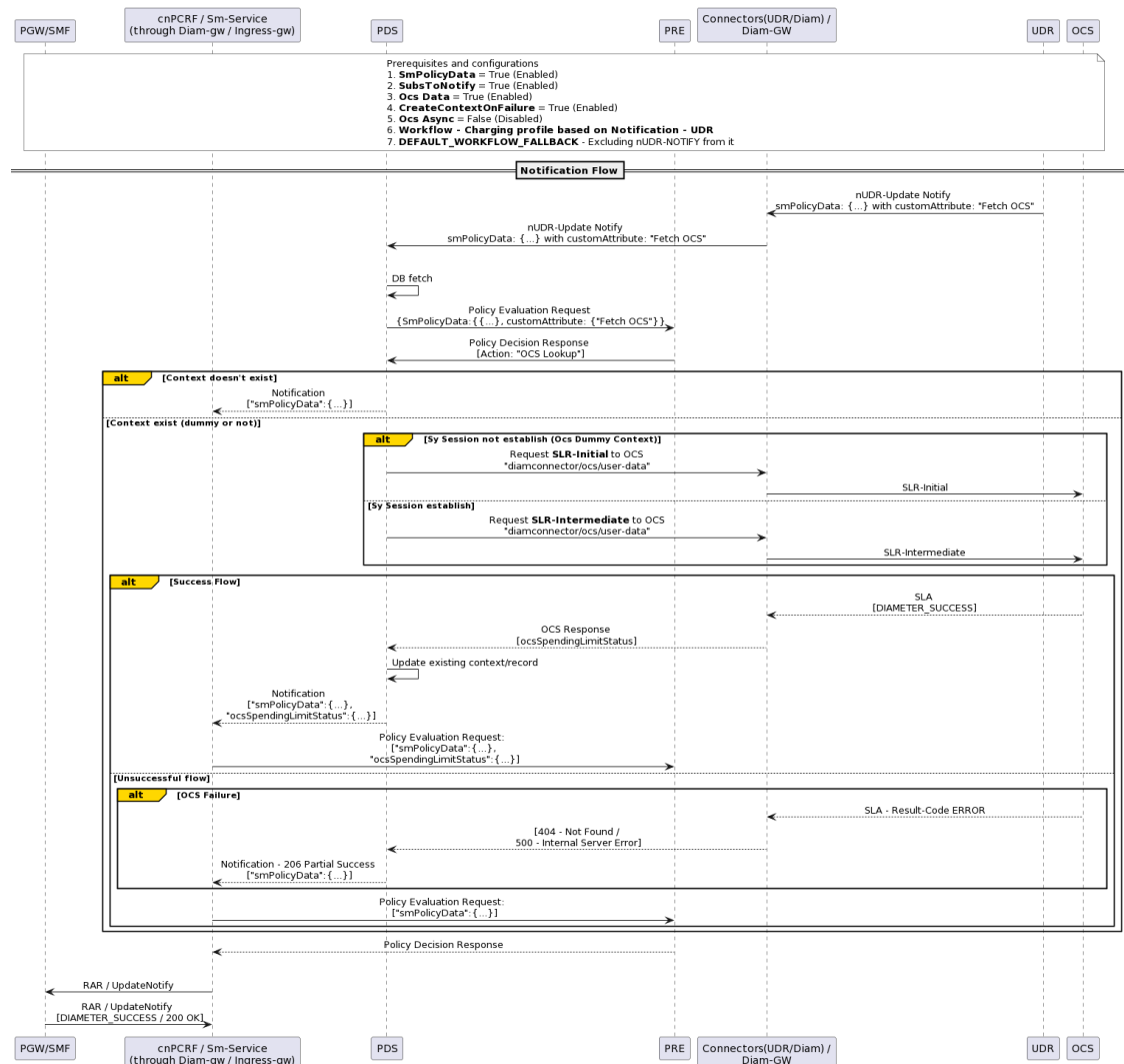
Figure 4-64 UDR PDS Notification Flow
