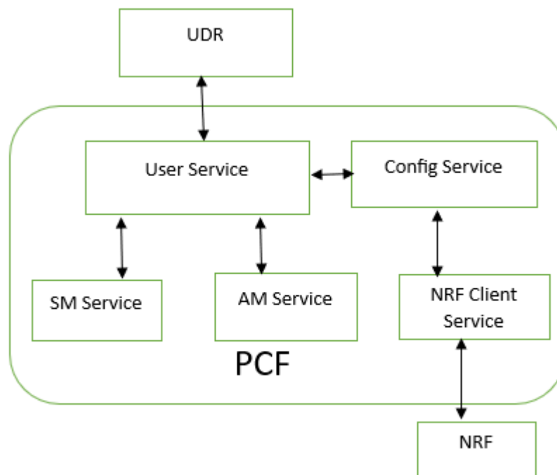
Figure 4-33 PCF User Service interactions with other services
