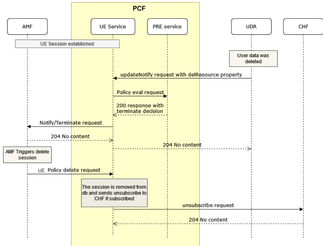
Figure 4-86 Call Flow for UE Terminate for UDR updateNotify with delResources
