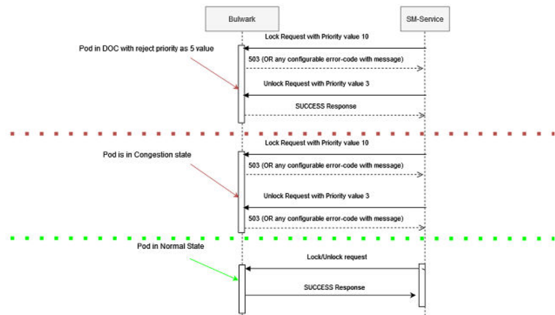
Figure 4-44 Call Flow Diagram for Bulwark Congestion Control
