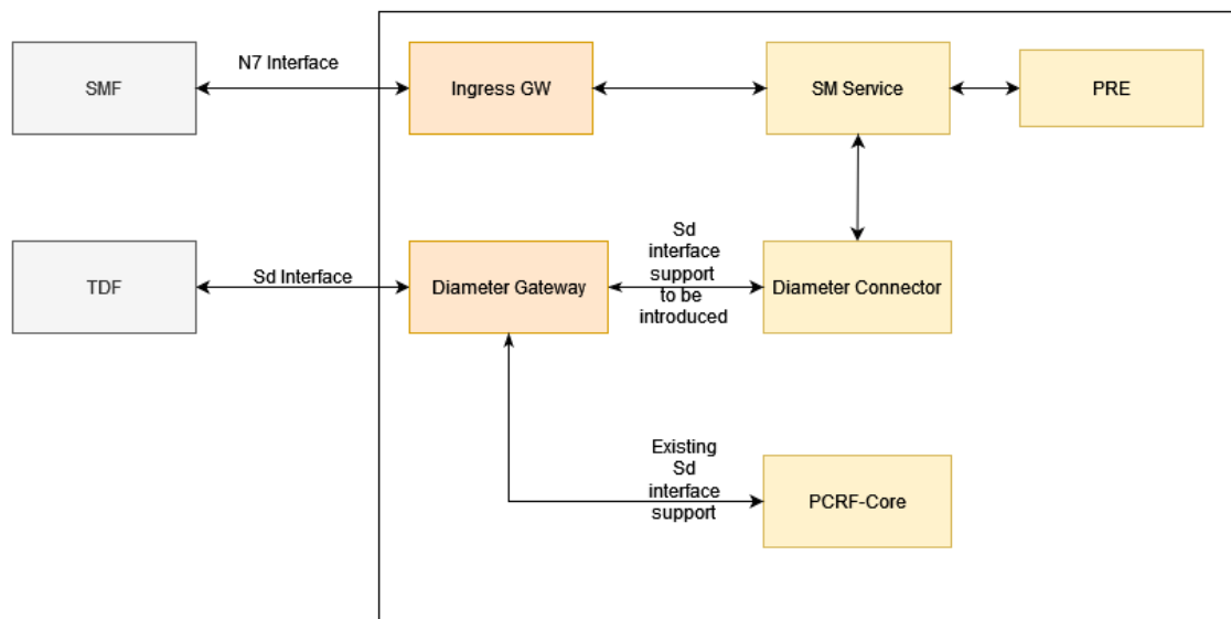
Figure 4-6 Sd interface in PCF
