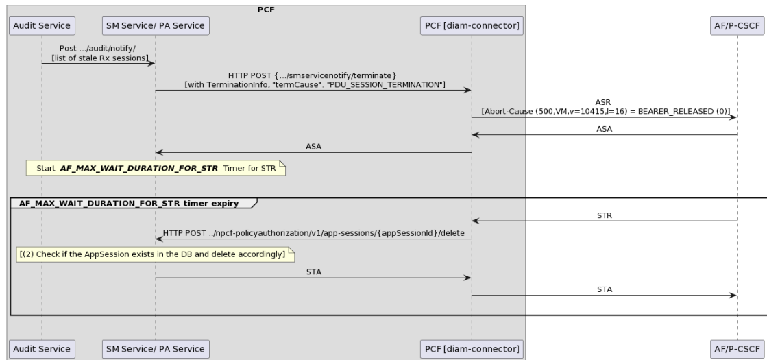
Figure 4-100 Rx session cleanup when Audit service detects a stale session
