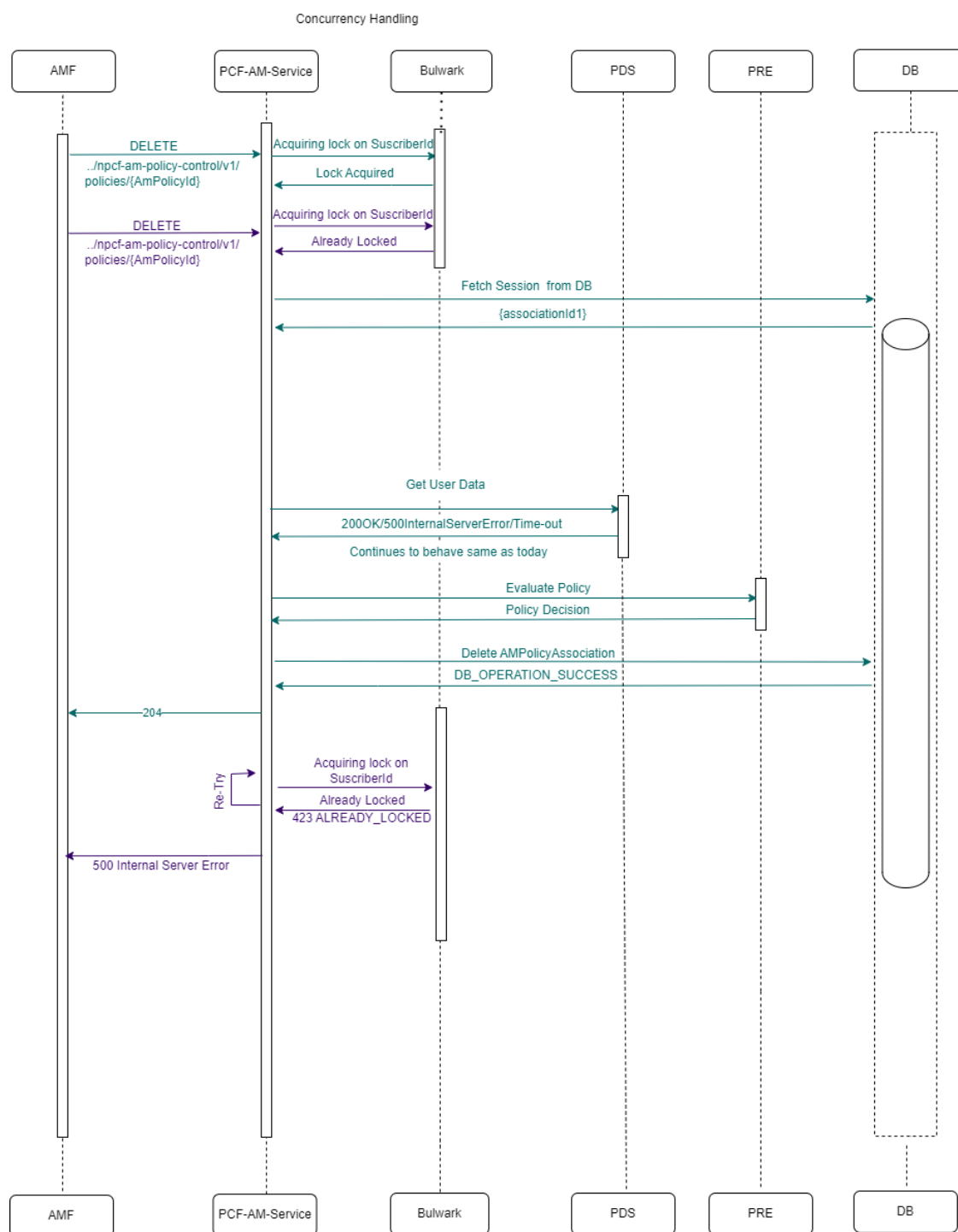
Figure 4-174 Two AM-Delete requests for same Subscriber and retry failure (retry =1)
