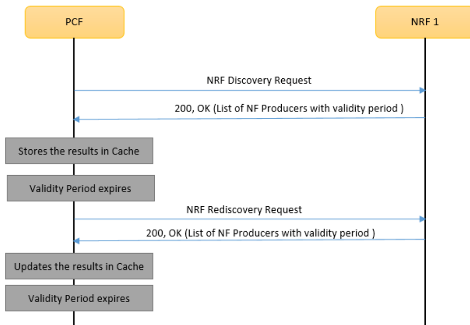
Figure 4-205 Call Flow - NRF Rediscovery
