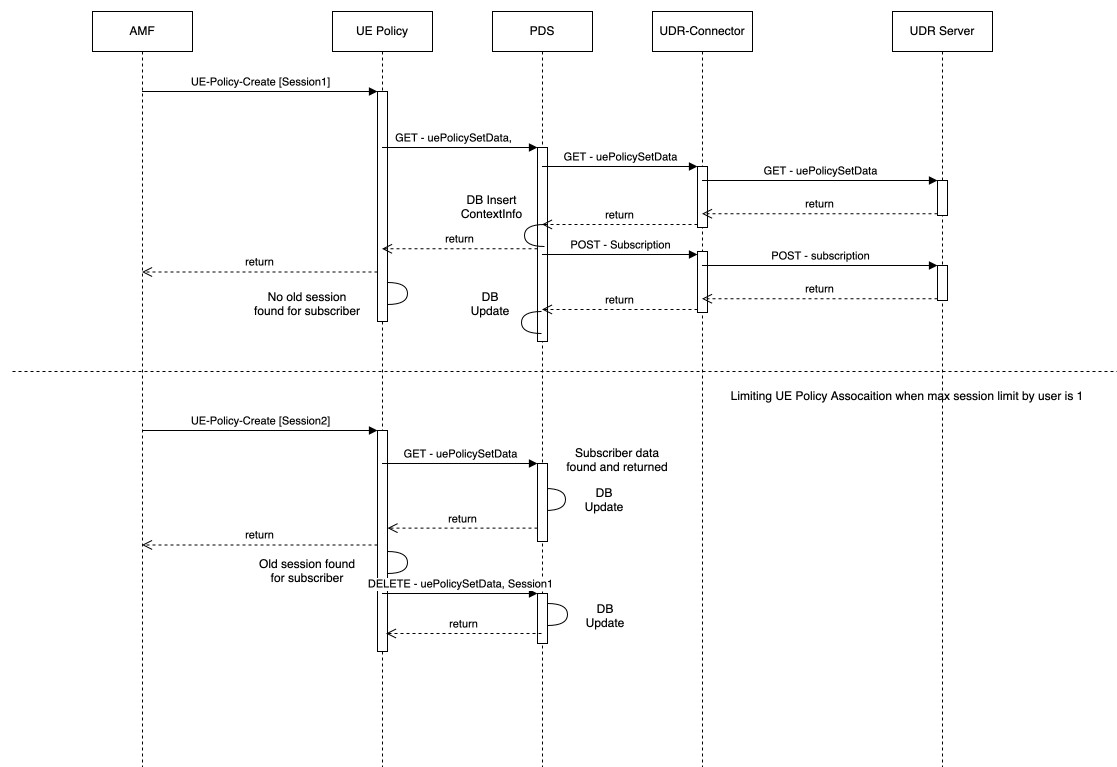
Figure 4-207 Limiting the number of sessions for UE Policy Service
