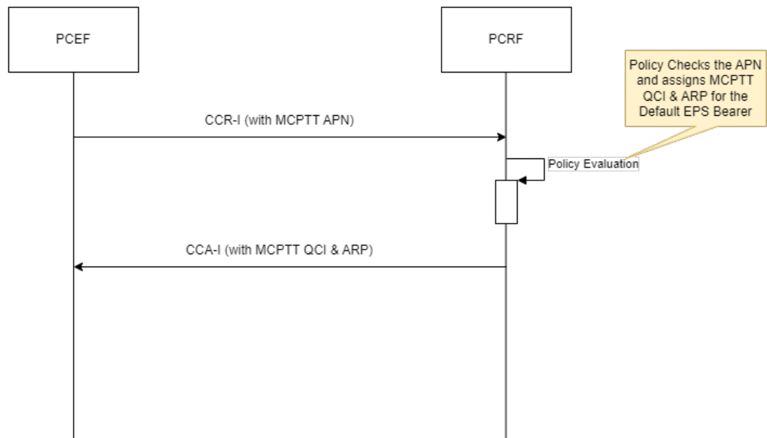
Figure 4-223 MCPTT APN Handling
