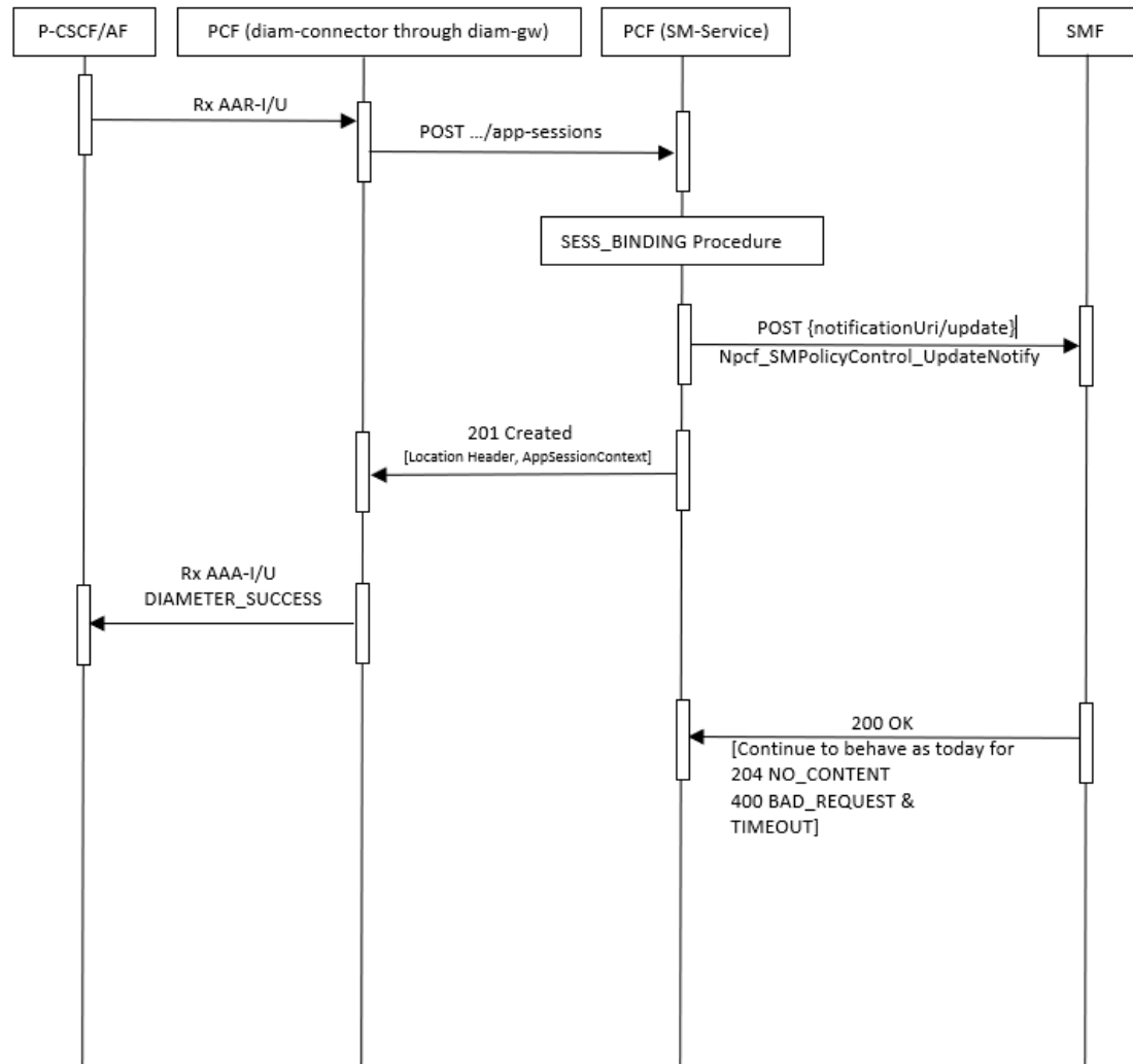
Figure 4-121 Subscription to notification of the AF Signaling Transmission in 5G
