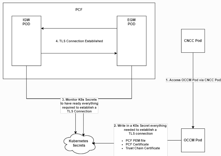
Figure 4-61 Policy Integration with OCCM
