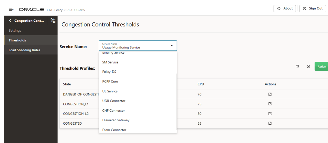
Figure 7-61 Congestion Control Thresholds
