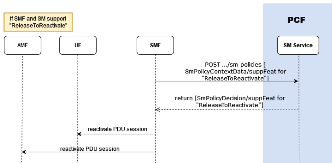
Figure 4-88 SM and SMF support for ReleaseToReactivate Feature
