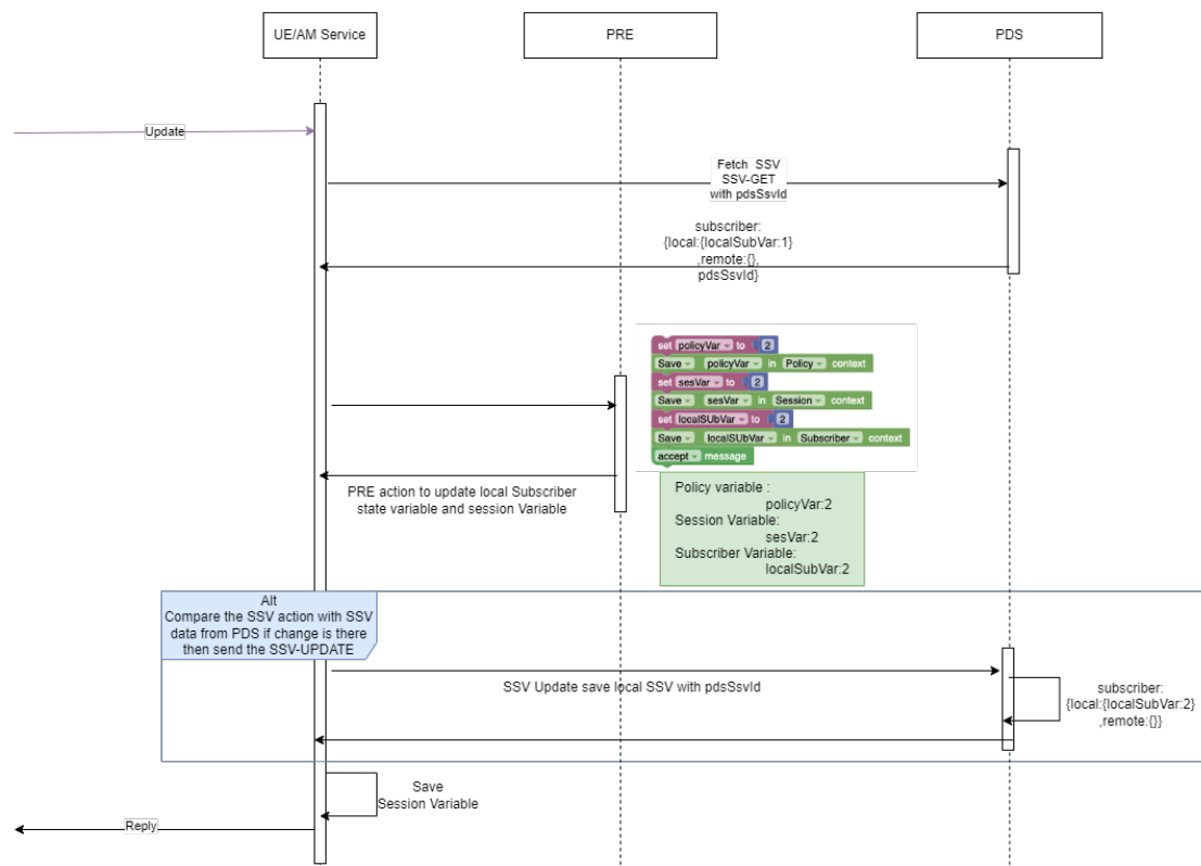
Figure 4-220 State variables in update session call flow
