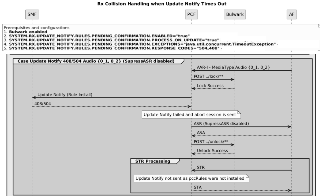
Figure 4-22 Handling Collision Between AAR and STR Messages During UpdateNotify-408 or 504 Errors from SMF
