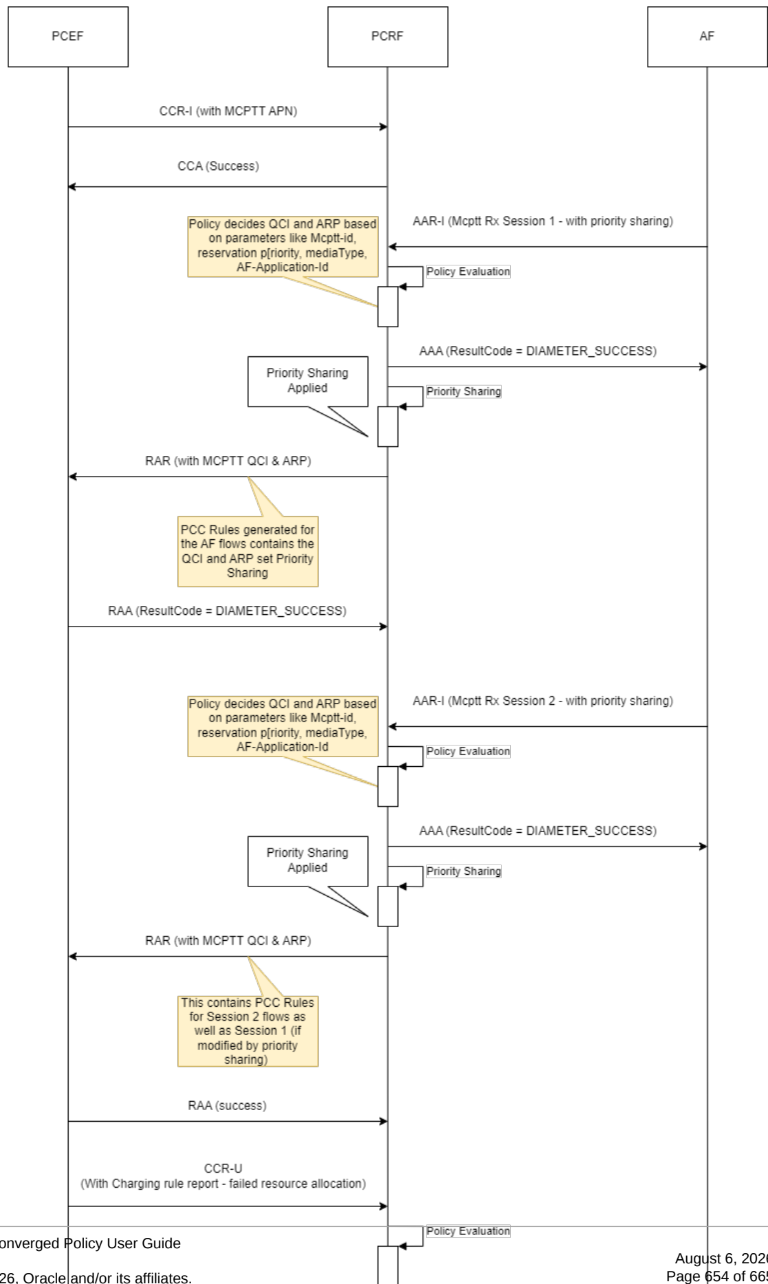
Figure 4-226 Preemption Control - CCRU- CharginRuleReport scenario
