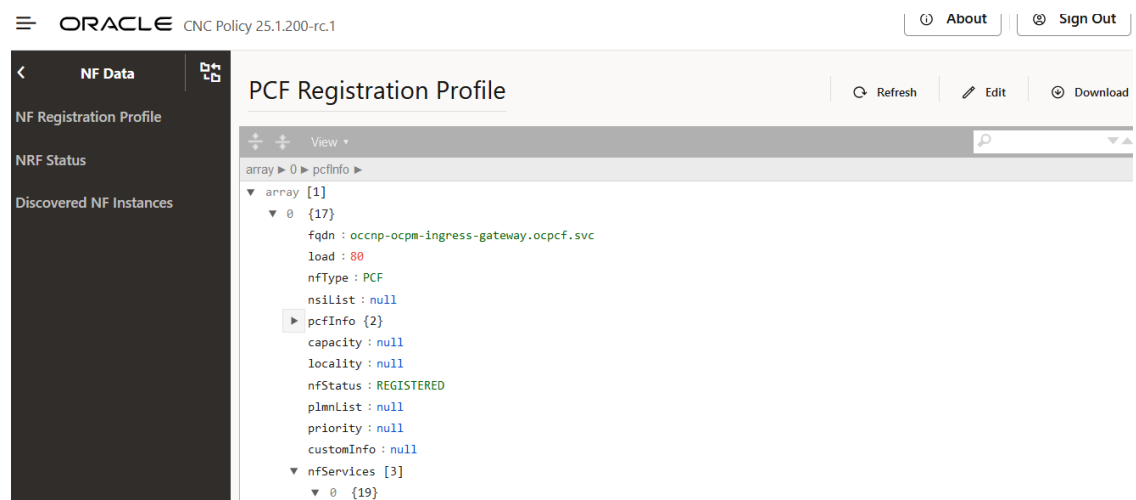
Figure 7-47 PCF Registration Profile
