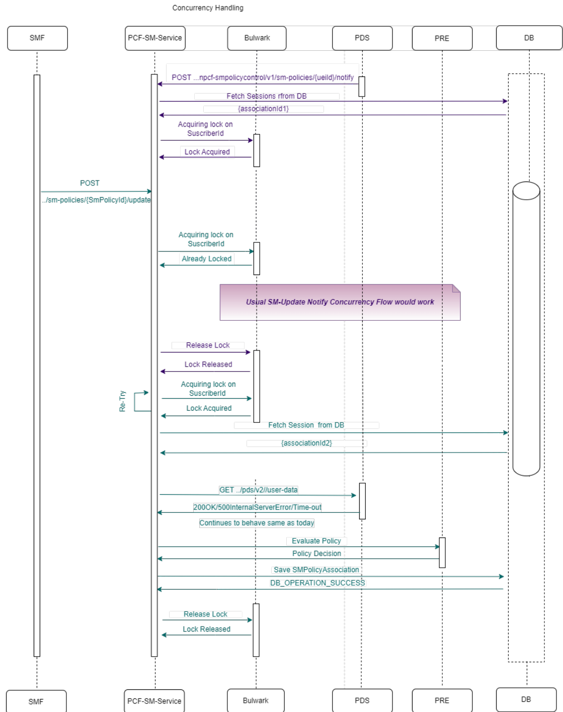
Figure 4-165 Concurrent SM-Update-Notify and Concurrent SM-Update - Success scenario
