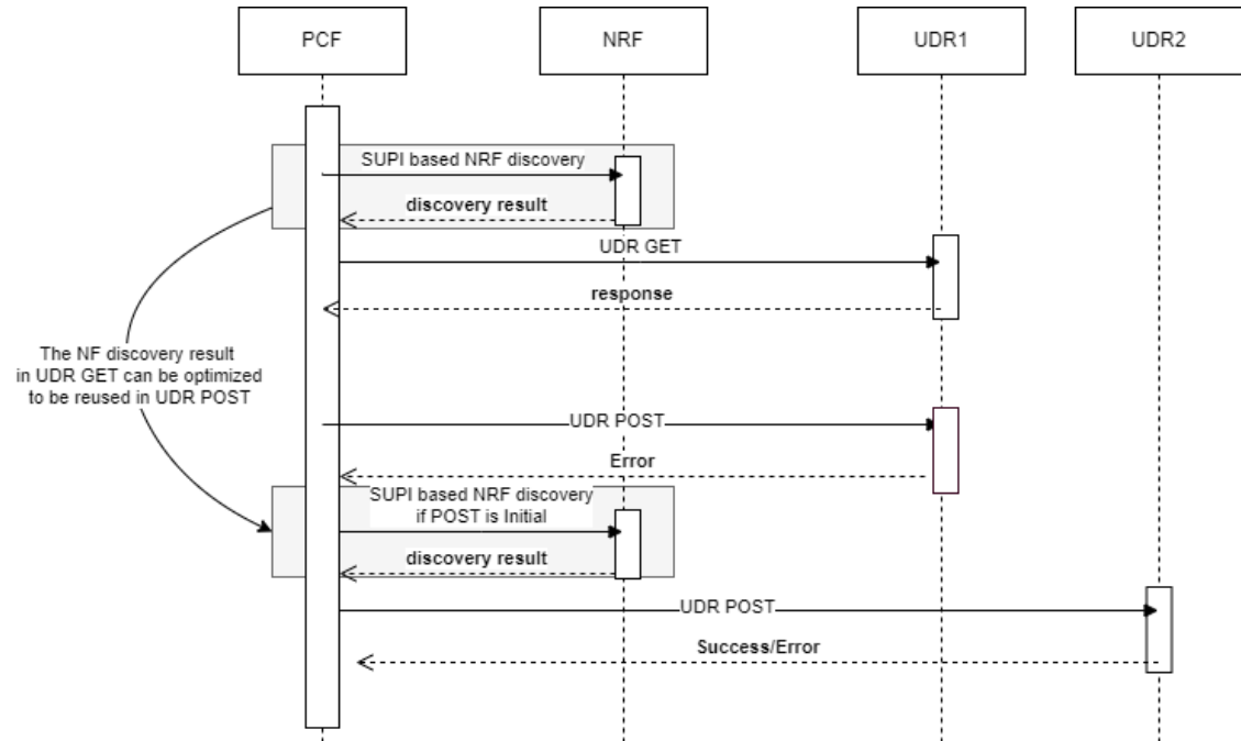
Figure 4-97 UDR GET Discovery Result Reused in UDR POST
