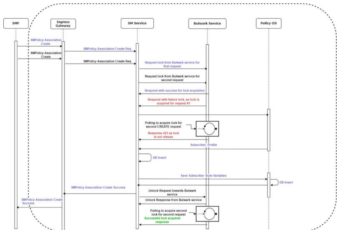
Figure 4-155 Call Flow - Bulwark Lock Request SM Create Procedure
