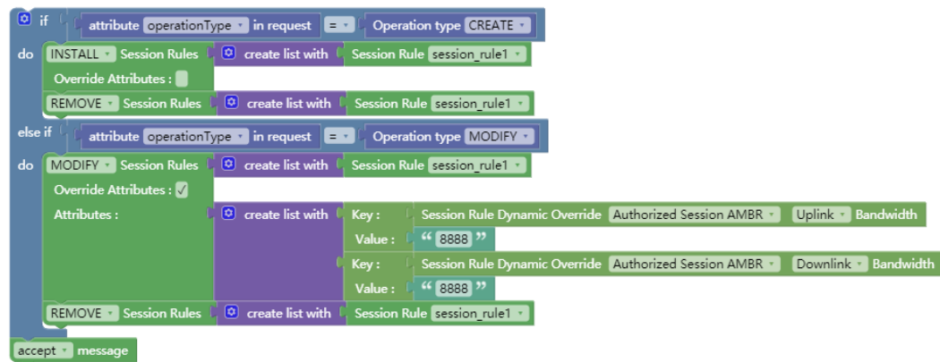
Figure 4-108 Example of Policy with Conflicts in a Session Rule
