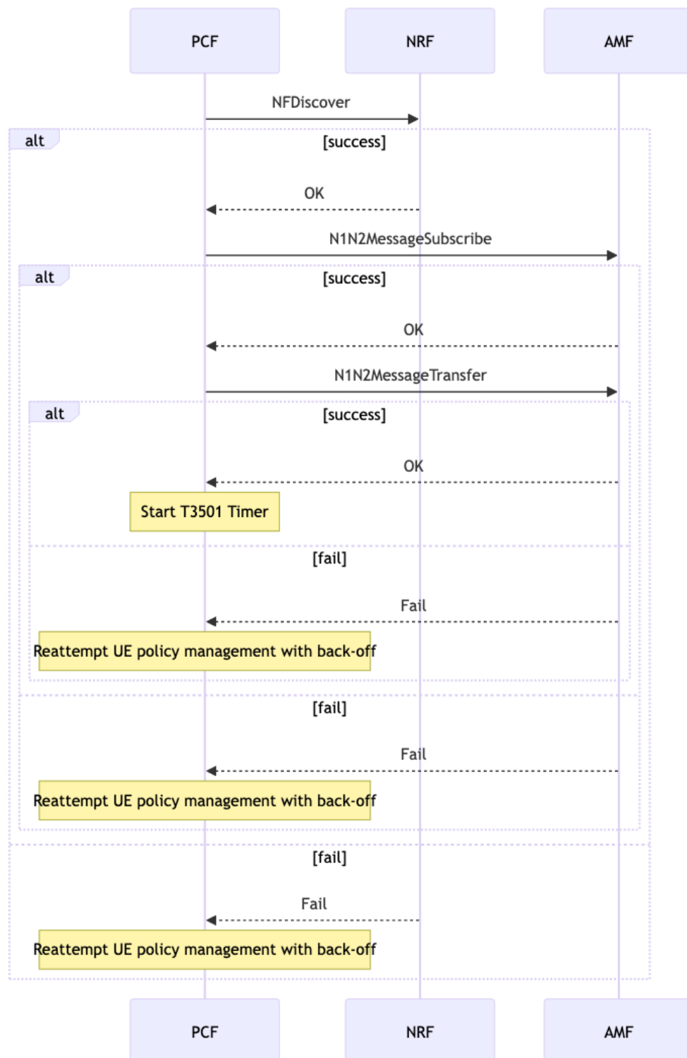
Figure 4-26 Reattempt and backoff Call flow
