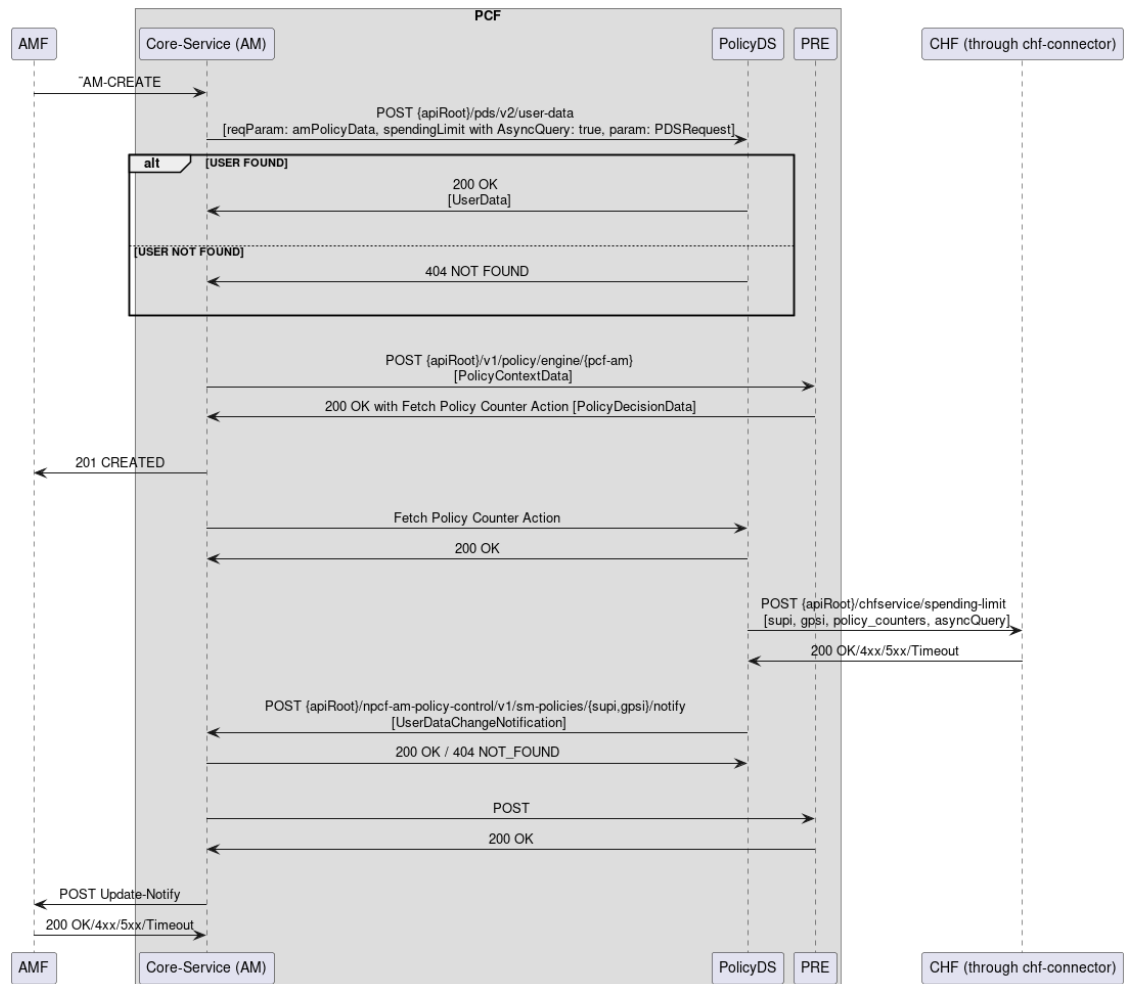
Figure 4-211 Spending limit status report for AM Service
