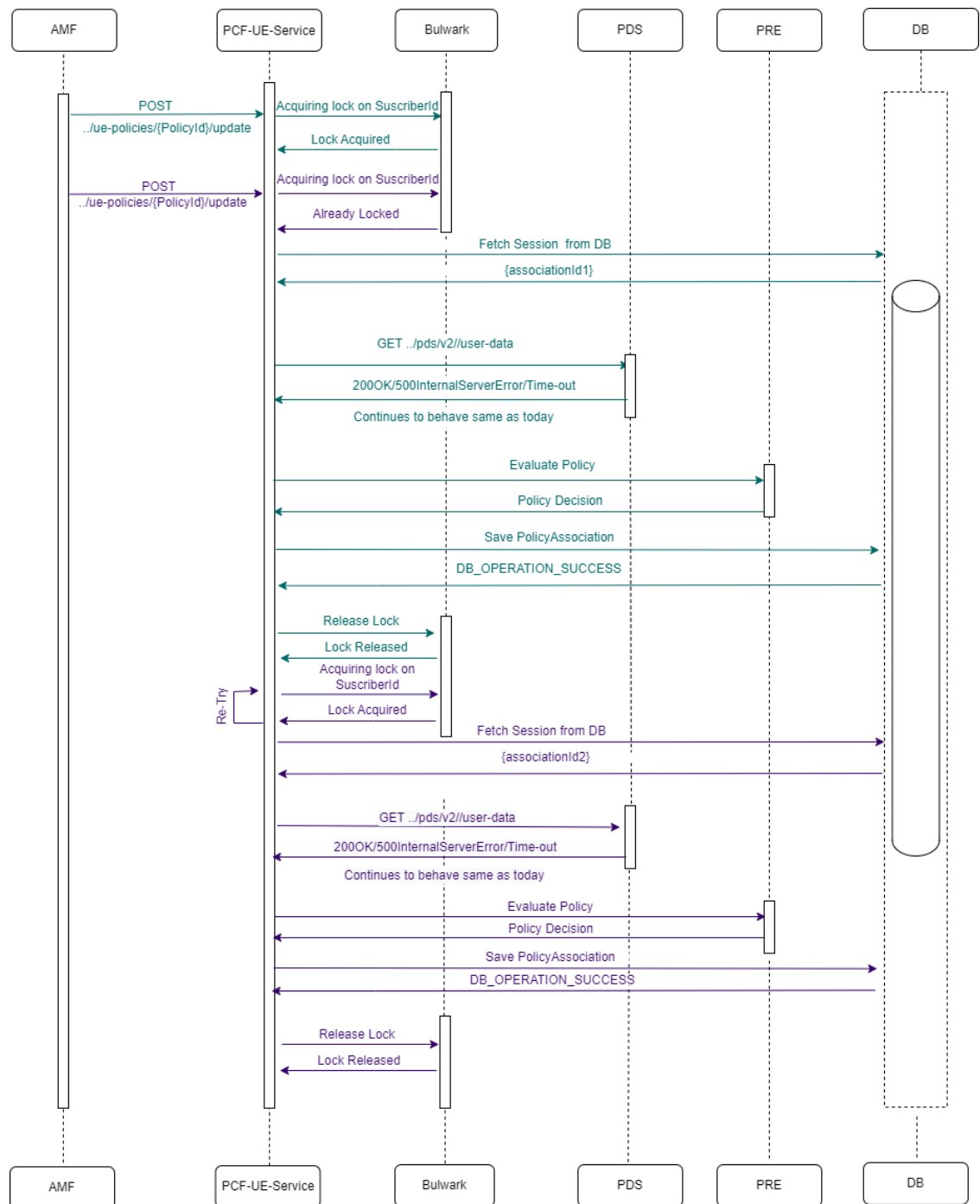
Figure 4-183 Two UE-Update requests for same Subscriber but different Sessions and retry success.
