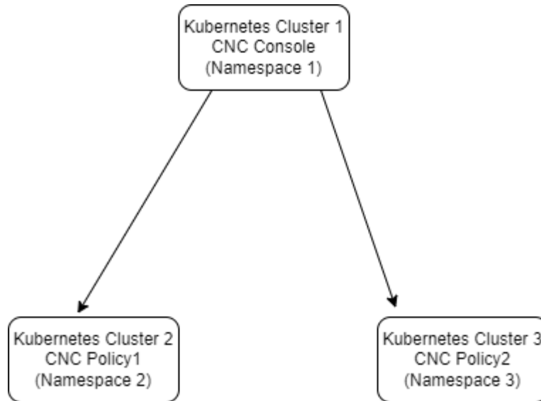
Figure 4-118 Support for Multicluster Deployment
