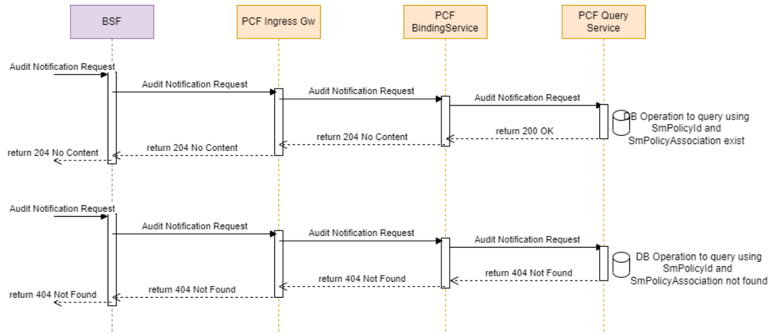
Figure 4-154 BSF and PCF Interaction for Stale Binding Detection
