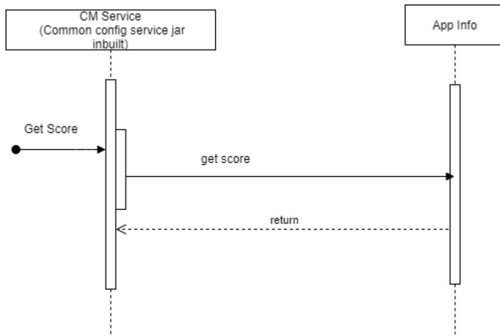
Figure 4-215 Call flow to Get the NF Score
