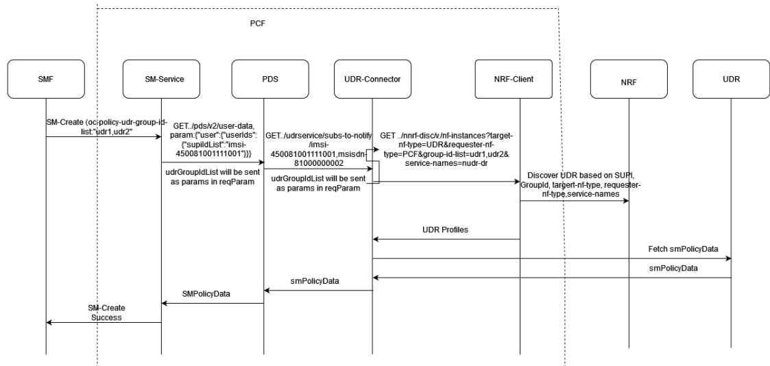
Figure 4-92 SMF sends SM Policy Association Request with oc-policy-udr-group-id
