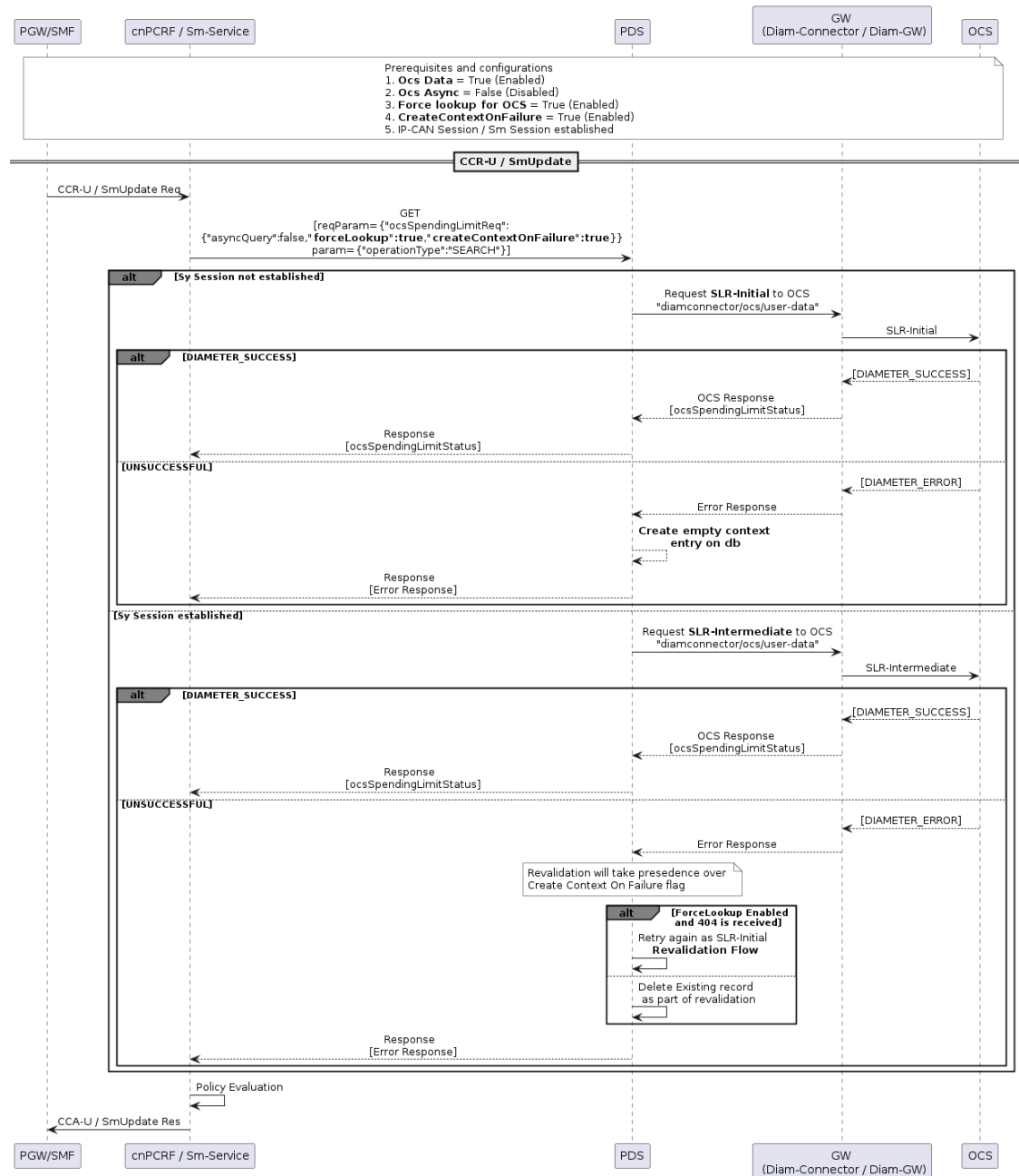
Figure 4-62 Update signalling flow for CnPCRF/SM service
