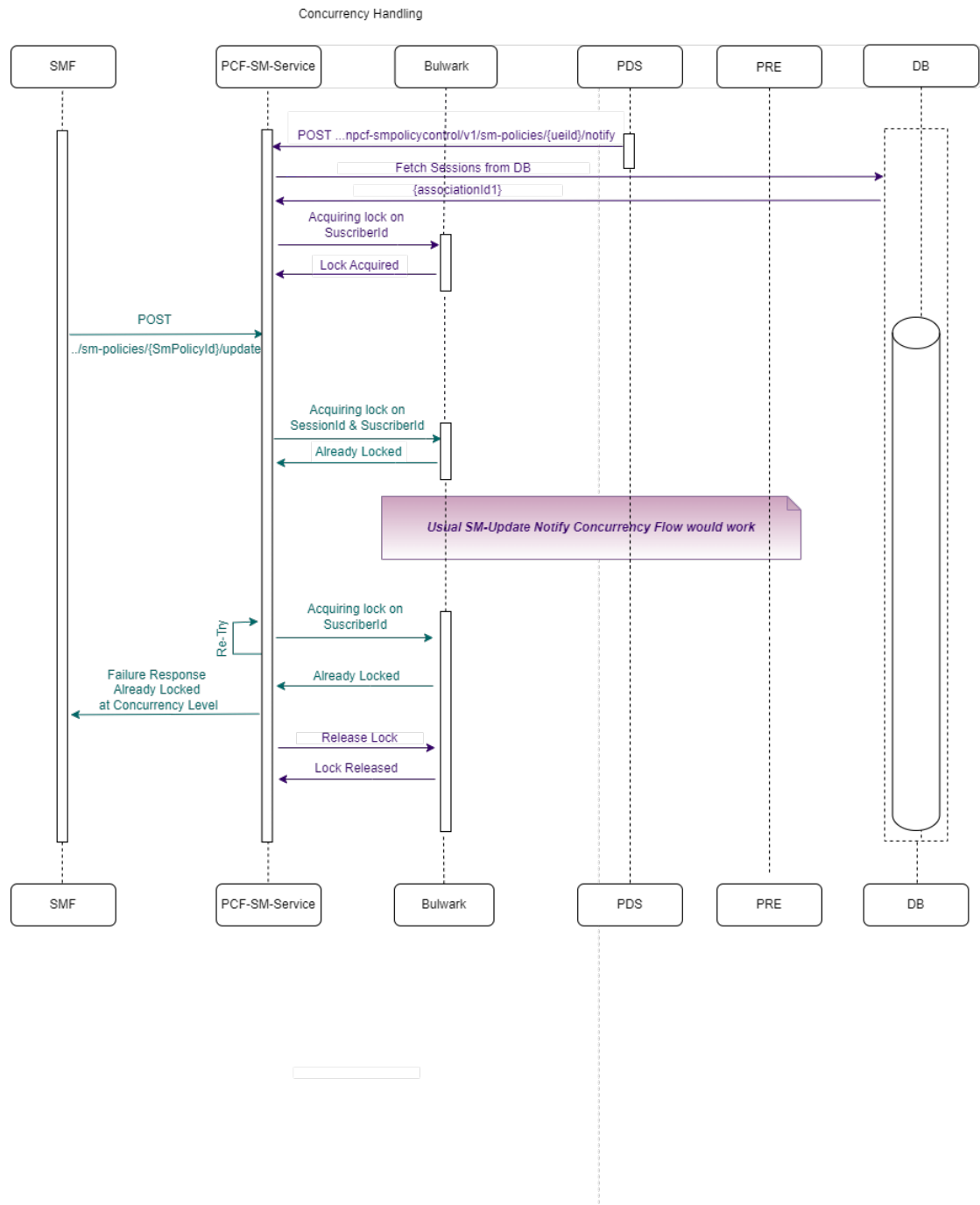
Figure 4-166 Concurrent SM-Update-Notify and Concurrent SM-Update - Failure scenario
