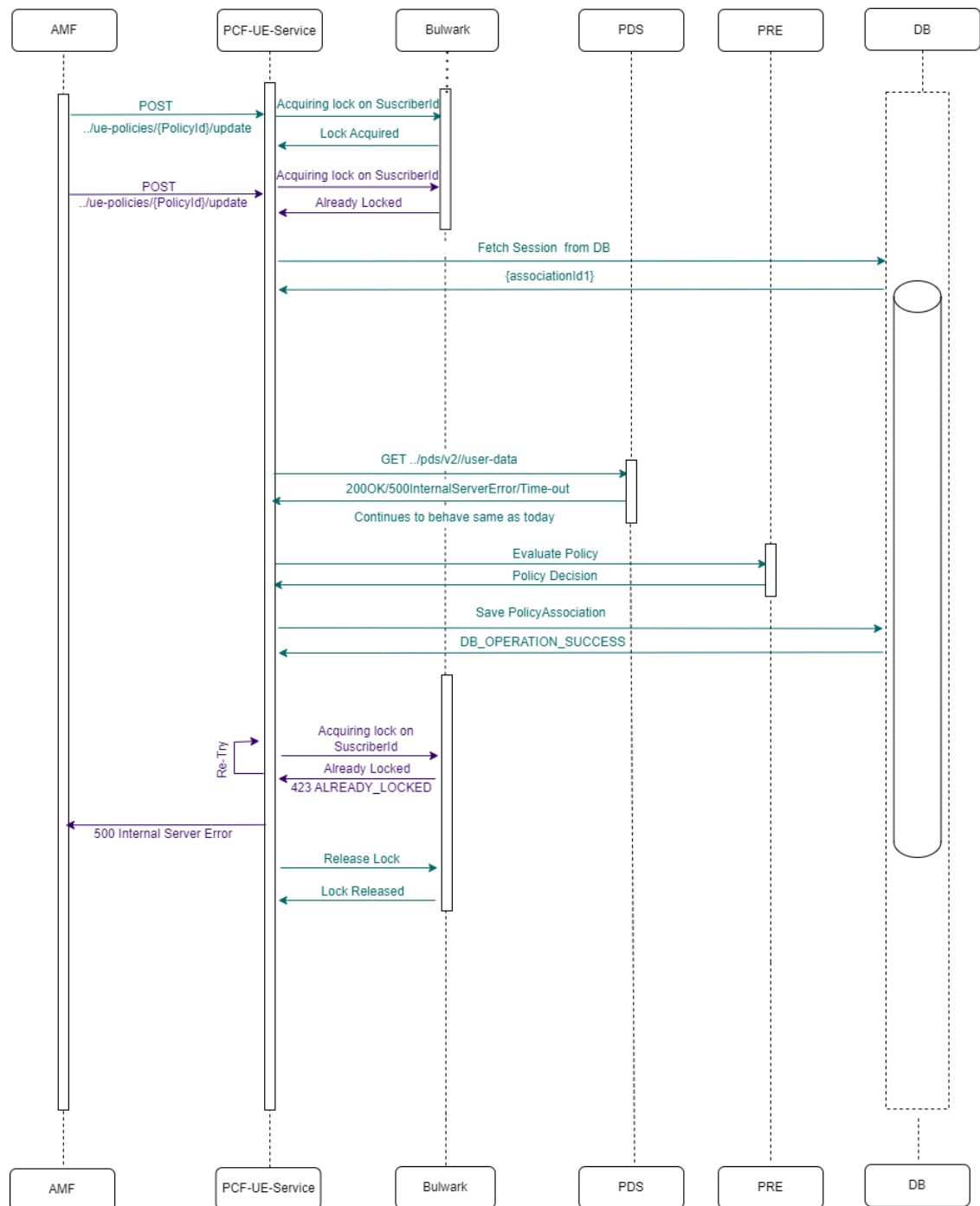
Figure 4-184 Two UE-Update requests for same Subscriber but different Sessions and retry failure (retry =1)
