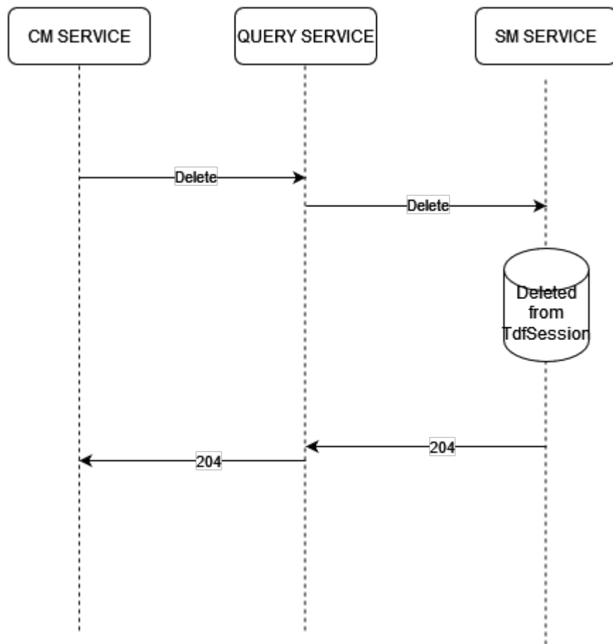
Figure 4-14 LOCAL DELETE TDF SESSION
