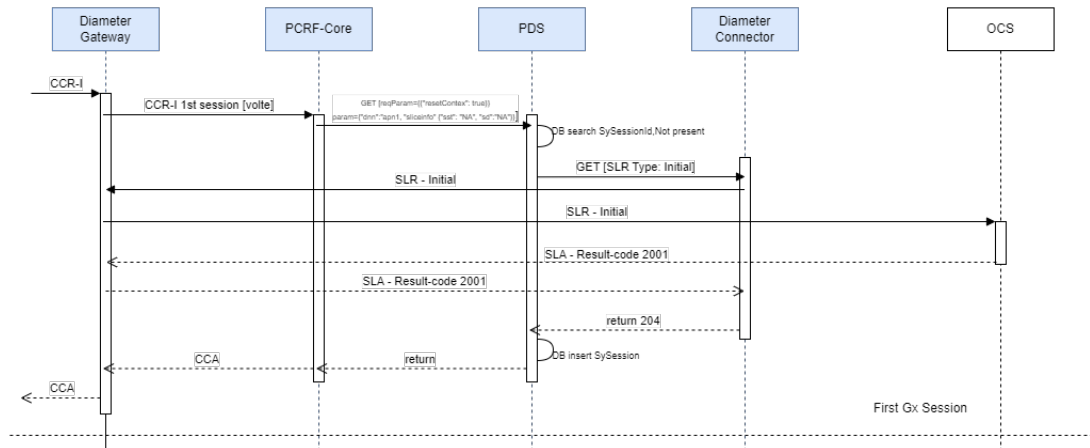
Figure 4-76 First Gx Session
