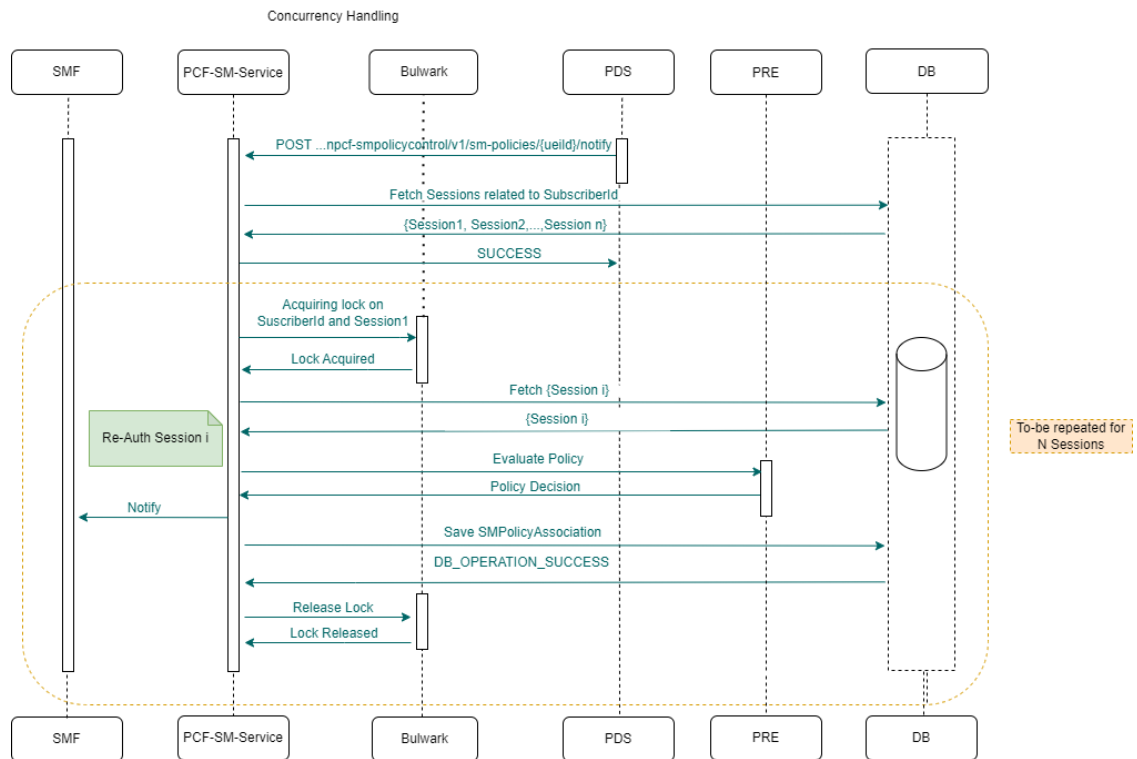
Figure 4-157 Call Flow for SM Update-Notify Request (One Notification and n Sessions)
