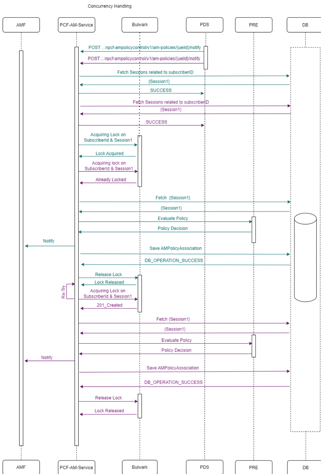
Figure 4-177 Two AM-Notify requests for same Subscriber each having 1 Session
