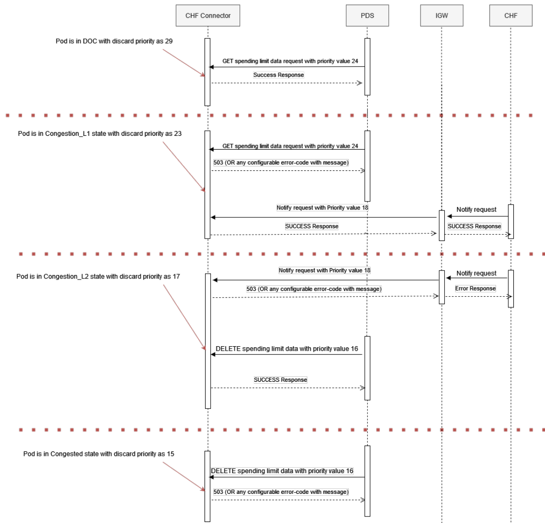
Figure 4-35 Call flow diagram for CHF Connector Congestion Control
