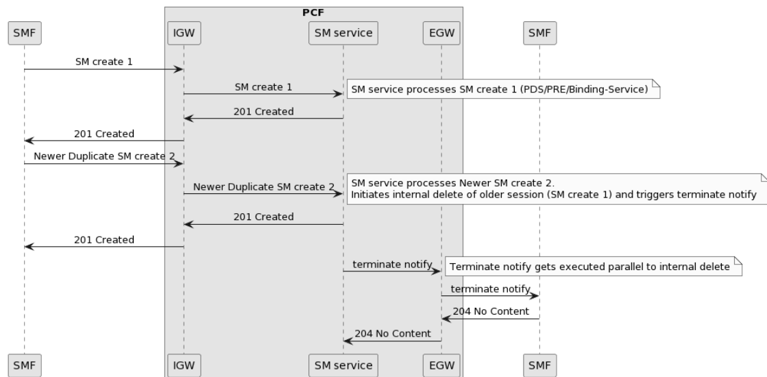
Figure 4-126 Sample call flow for sending Terminate Notify when duplicate session is found (collision detection) and SM service cleans up the older session from database
