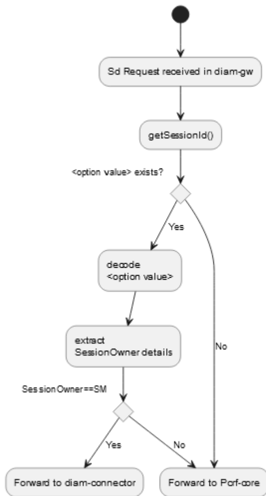
Figure 4-12 Flowchart for Diameter Gateway Routing Decision
