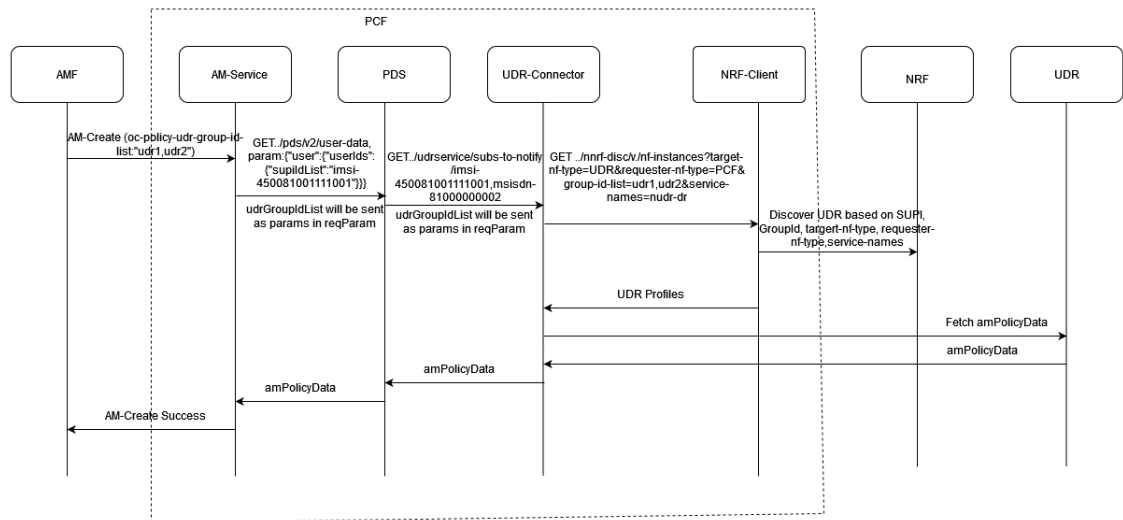
Figure 4-93 AMF sends AM Policy Association Request with oc-policy-udr-group-id
