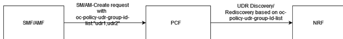
Figure 4-91 UDR Discovery with oc-policy-udr-group-id-list Header to NRF
