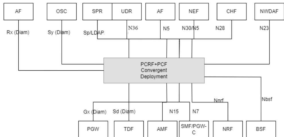
Figure 4-228 Converged Policy Architecture to Support EPC and 5GC
