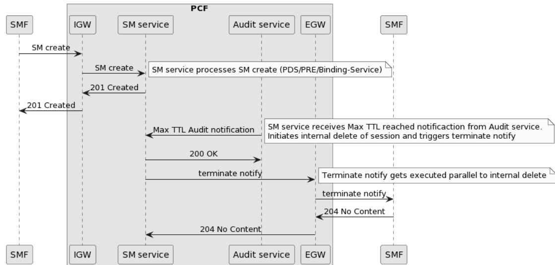
Figure 4-136 Sample call flow for sending Terminate Notify when Max TTL notification is received from Audit service.
