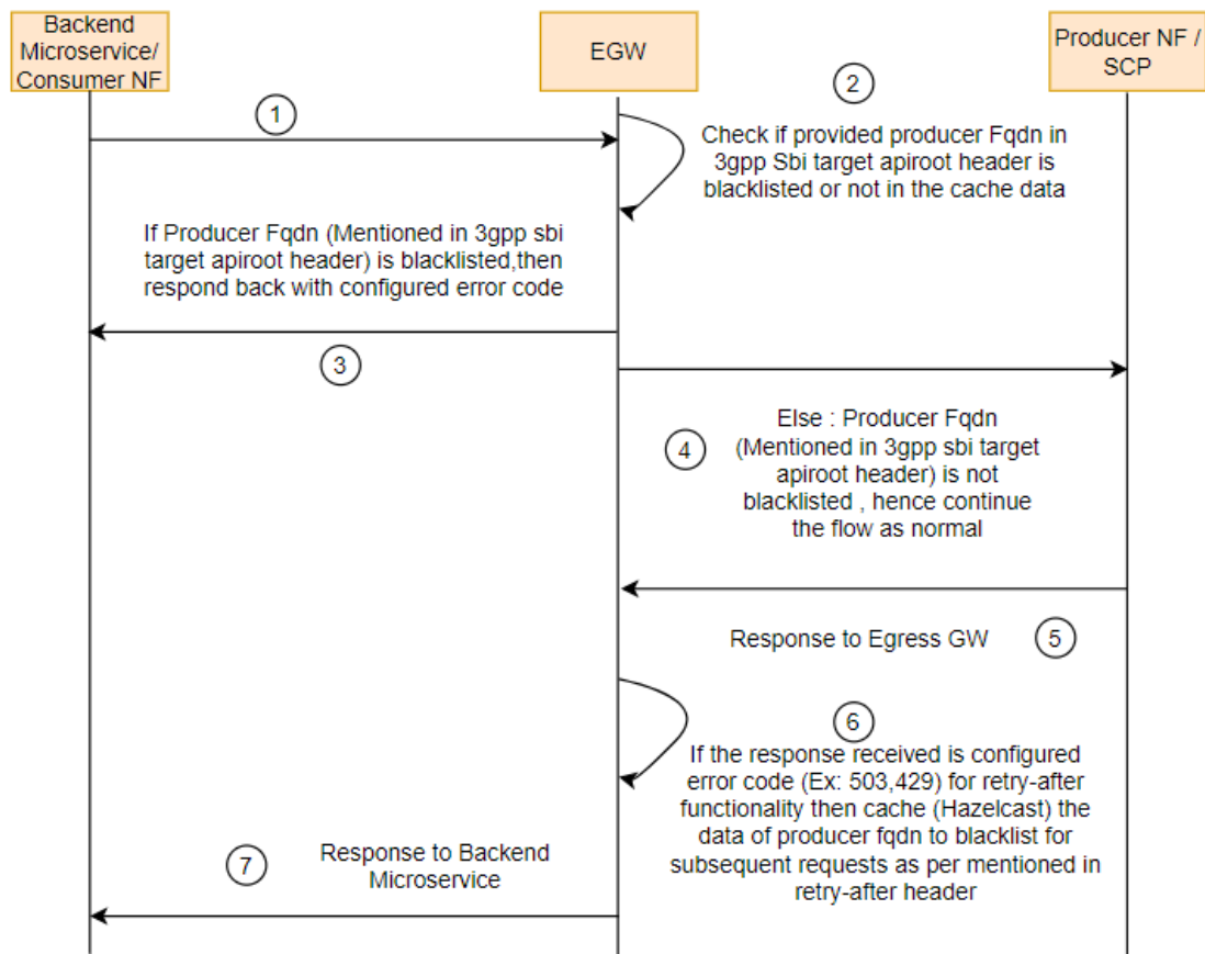
Figure 4-132 Subsequent Calls for Producer FQDN
