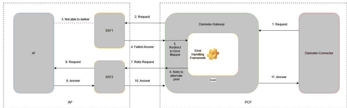
Figure 4-109 The block diagram represents the diameter Rx RAR and Rx ASR message flow with a retry:
