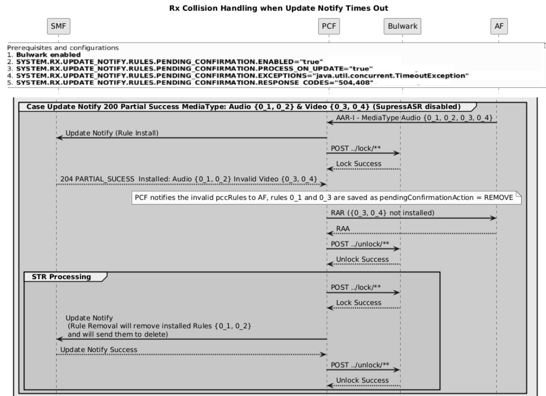
Figure 4-21 Handling Collision Between AAR and STR Messages During UpdateNotify-Partial Success Scenario
