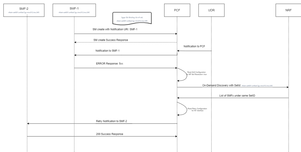
Figure 4-130 On demand NF Discovery is enabled (NF Set Resolution is set to NRF Discovery)
