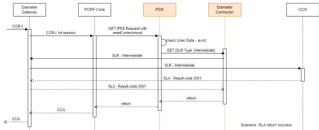
Figure 4-74 SLA Returns Success
