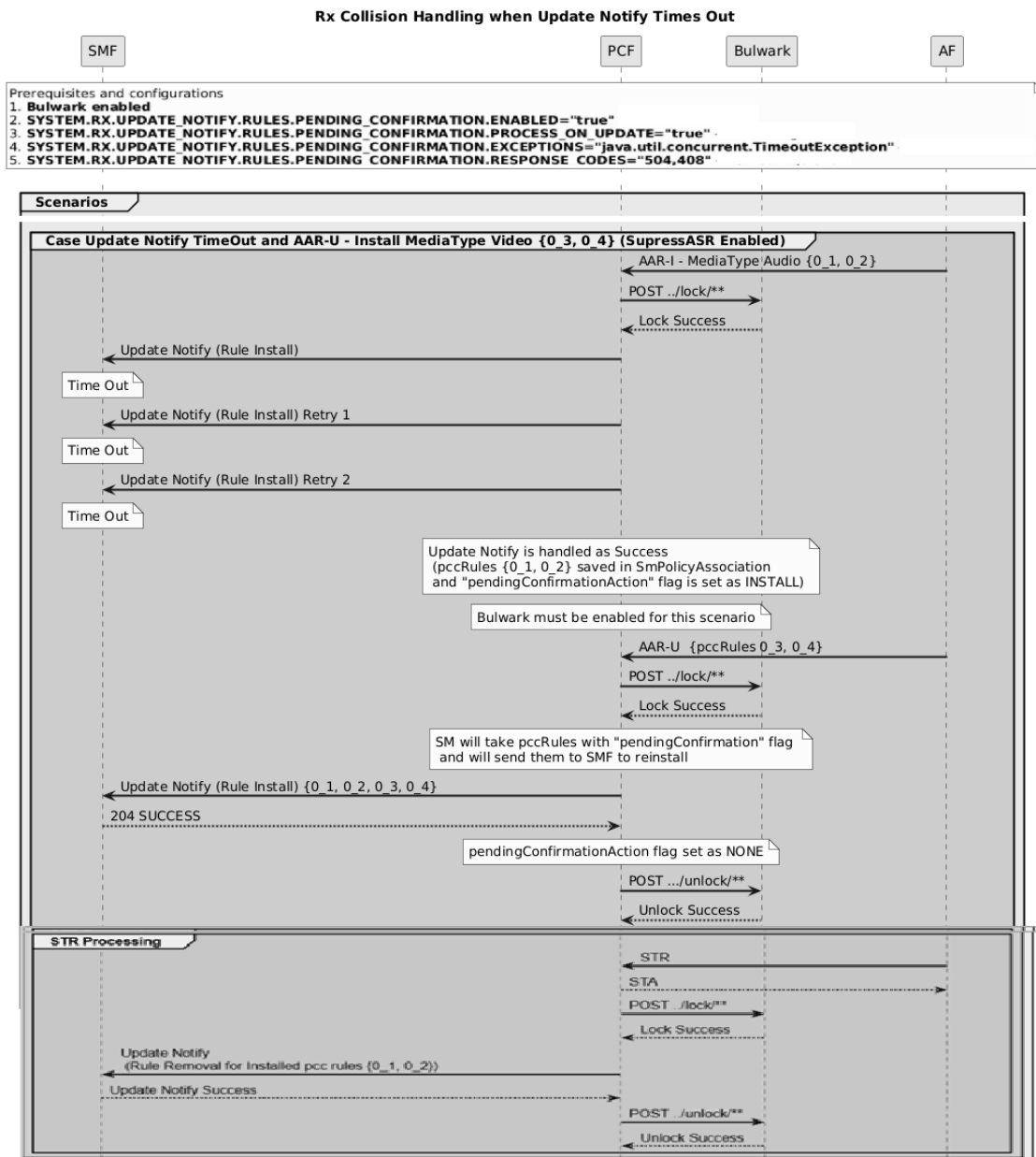
Figure 4-24 Handling Collision Between AAR-I, AAR-U, and STR Messages During UpdateNotify-Timeout Scenario with SupressASR Enabled
