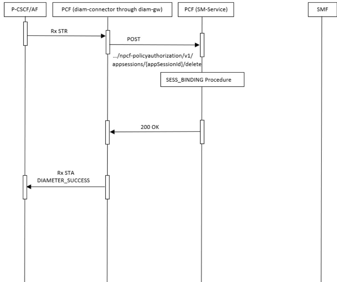
Figure 4-123 Cancellation of subscription to notification of the AF Signaling Transmission in 5G
