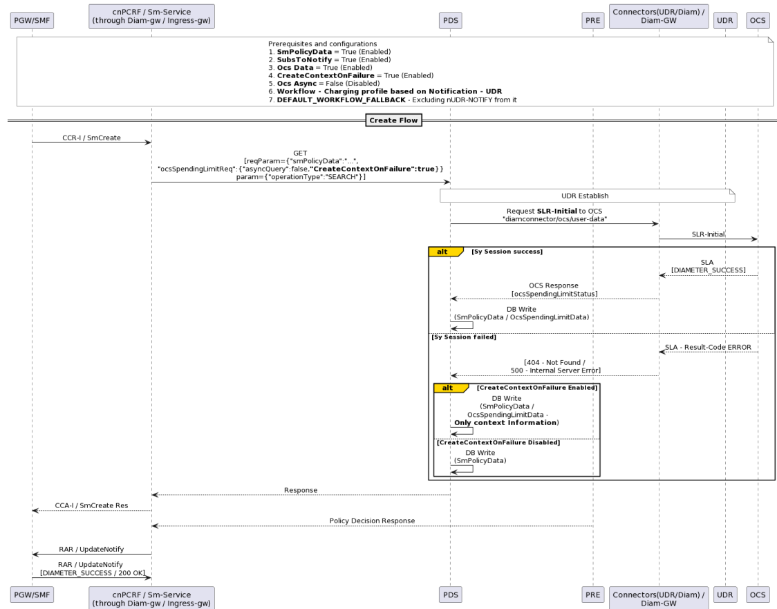
Figure 4-63 UDR PDS - Create Flow
