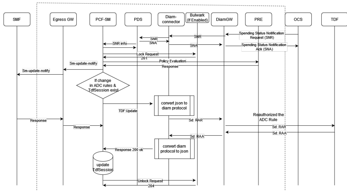
Figure 4-9 Sd Session Modification on Update Notification from OCS-Sy SNR
