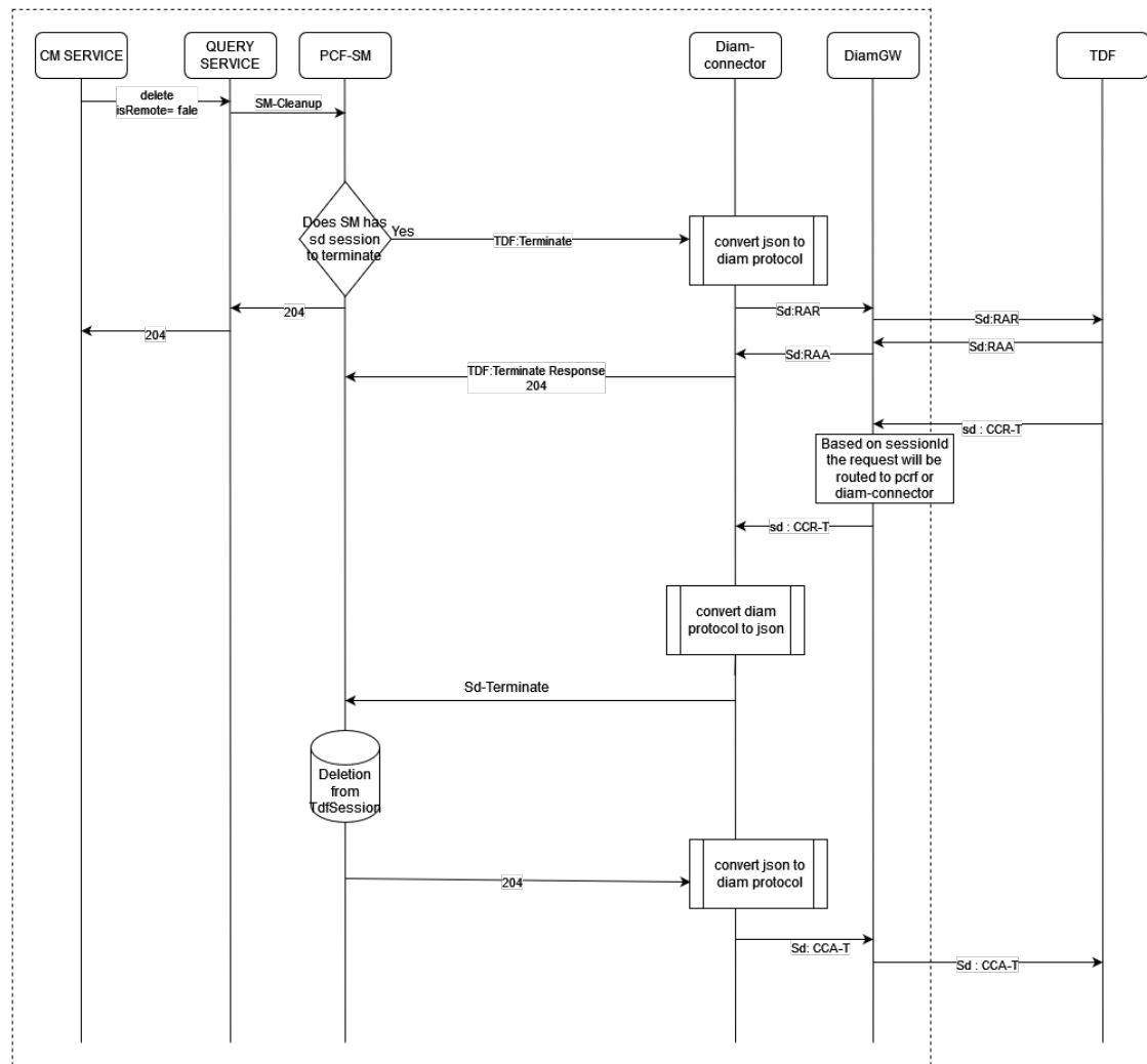
Figure 4-16 LOCAL DELETE SM SESSION
