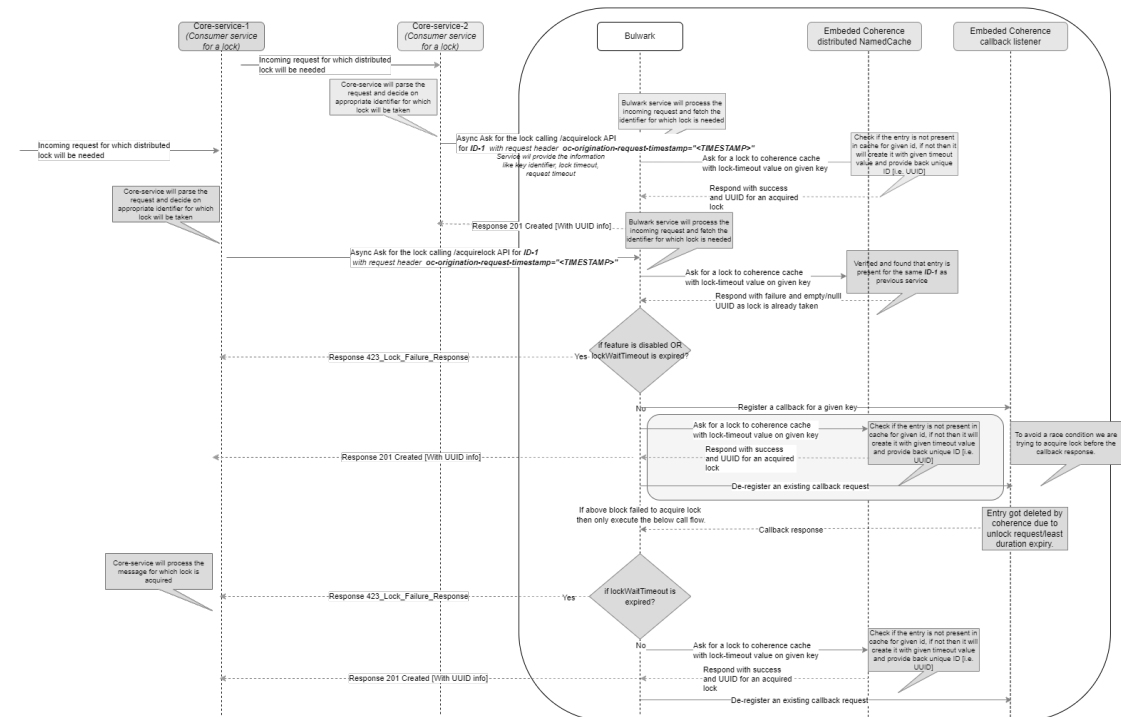
Figure 4-51 If lock is not available. Register for Long polling mechanism with the configured polling interval (20ms) and max lock re-attempts (5)
