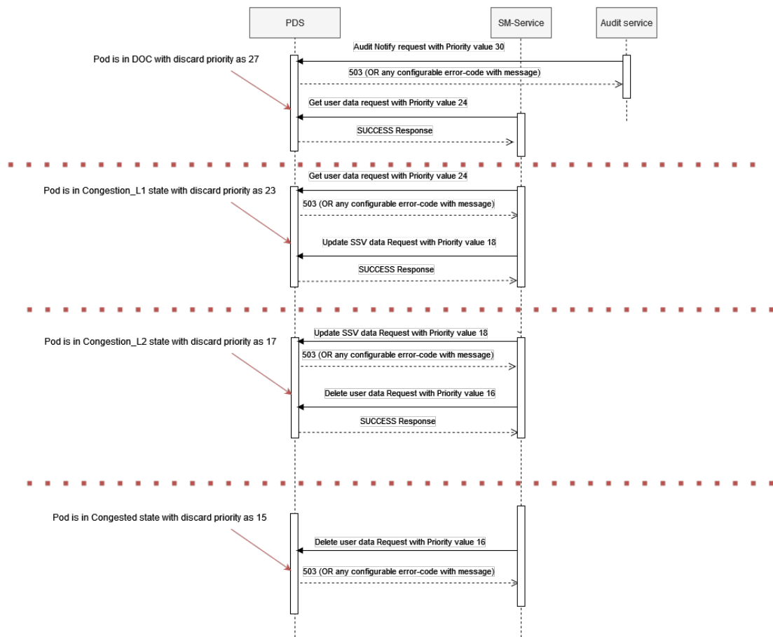
Figure 4-37 PDS Congestion Control Call Flow
