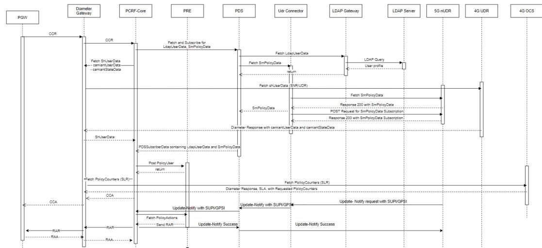
Figure 4-153 Call flow for notification handling from PDS for PCRF-Core
