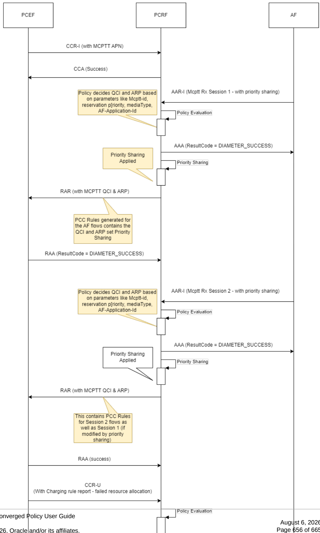
Figure 4-227 Preemption - No Preemptable Rule found
