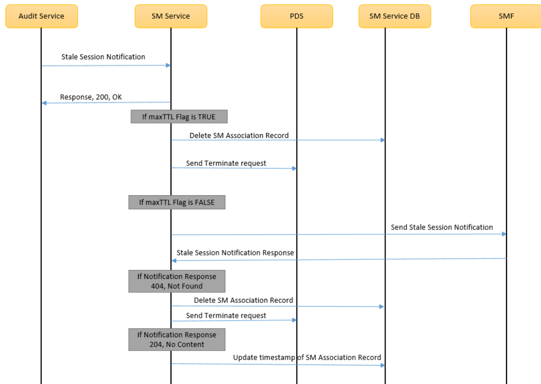
Figure 4-135 Example call flow for Stale Session Detection and Handling in SM Service
