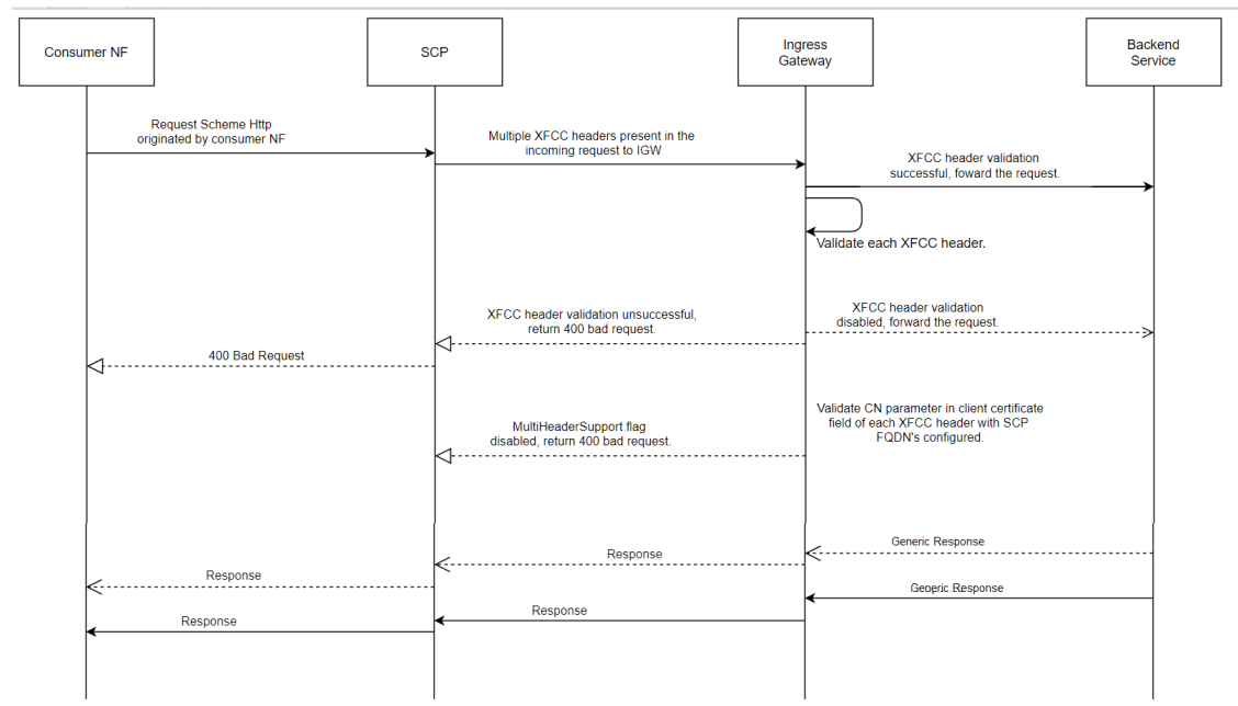
Figure 4-151 Call Flow Validating Multiple XFCC Headers
