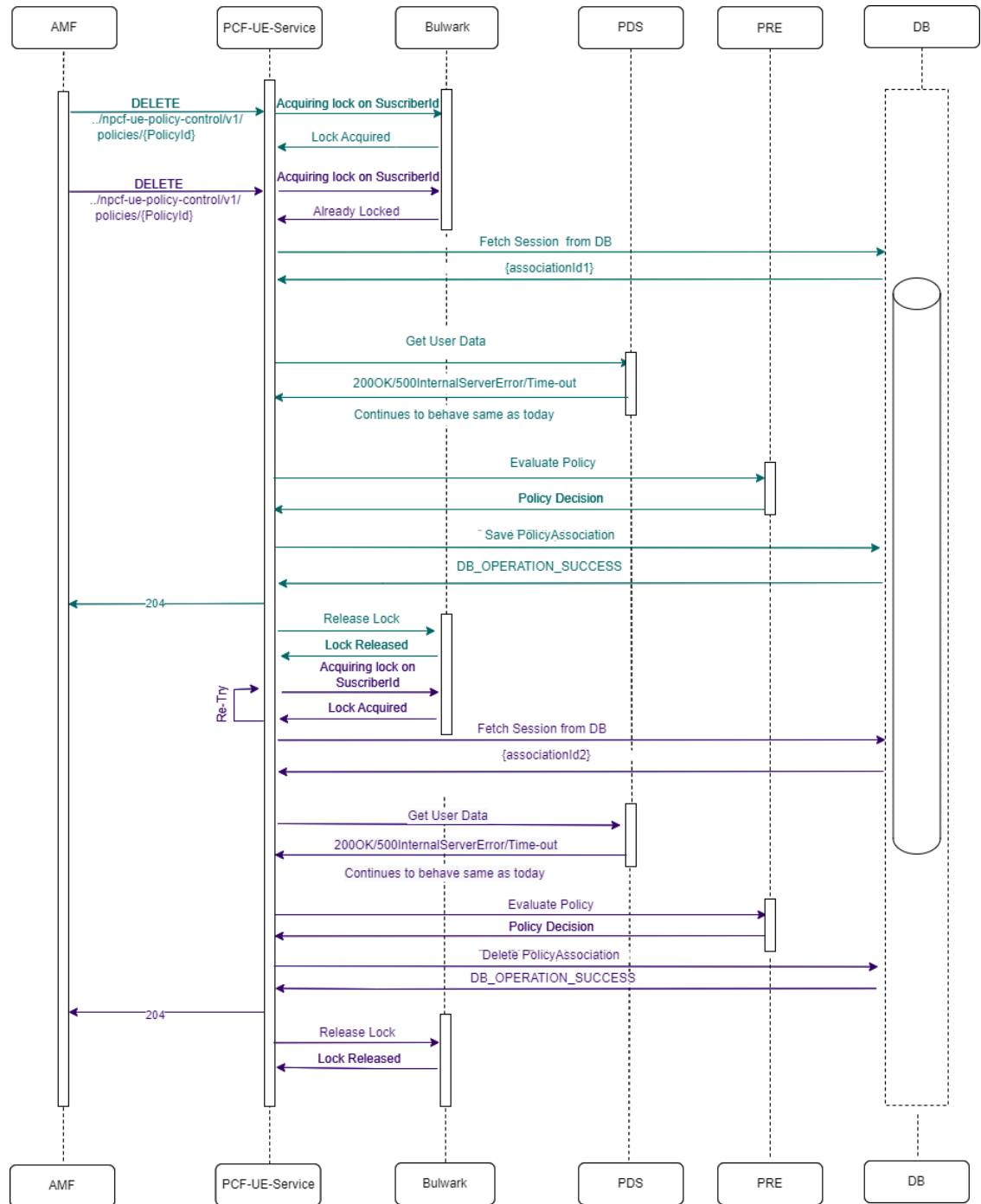
Figure 4-181 Two UE-Delete requests for same Subscriber and retry success.
