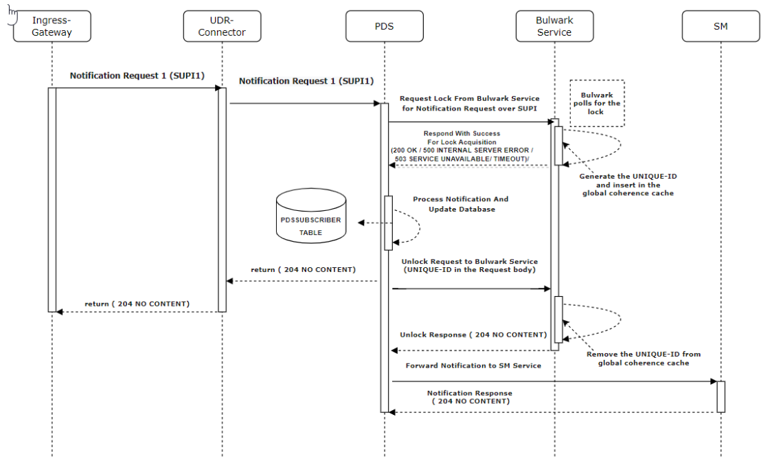
Figure 4-190 Call Flow - Bulwark Lock Request For UDR Notification
