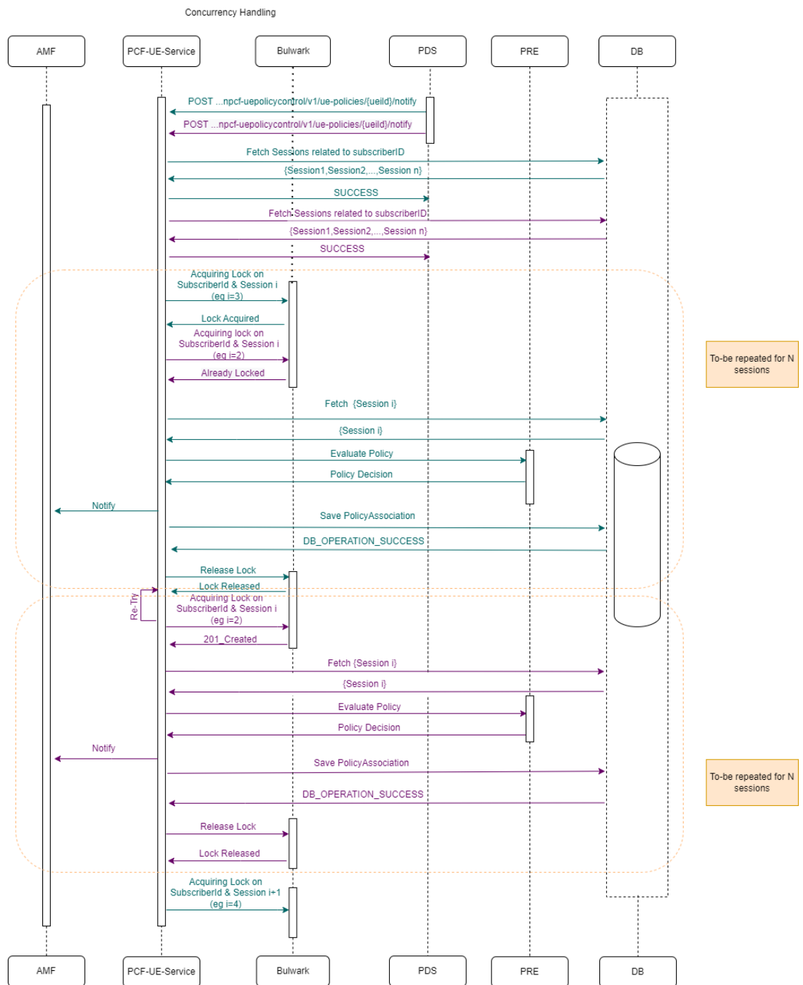
Figure 4-186 Two UENotify request for same Subscriber each having n sessions
