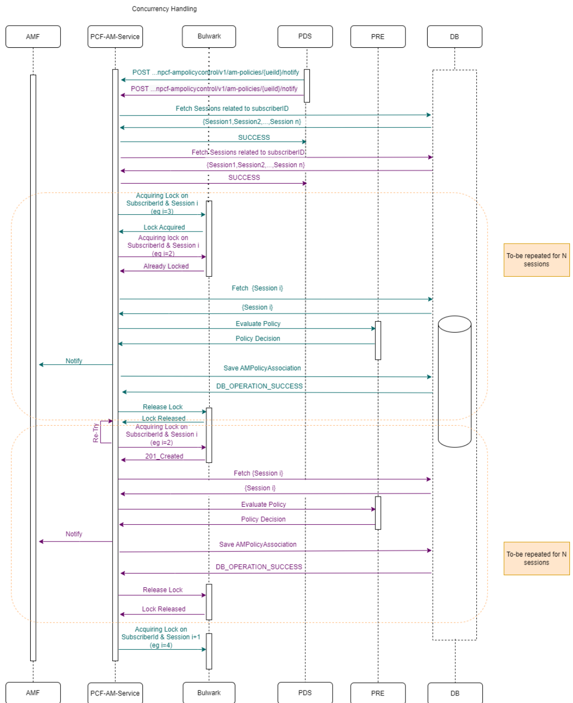
Figure 4-178 Two AM-Notify request for same Subscriber each having n Sessions
