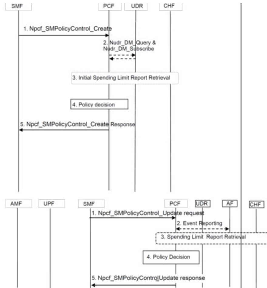
Figure 4-105 PRA Support for SM Service
