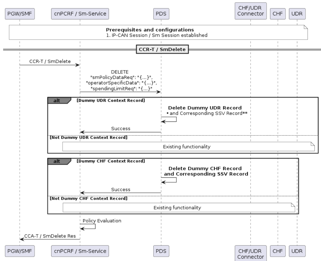
Figure 4-68 PDS Dummy Context during SM Delete or PCRF Core CCR-T Call Flow
