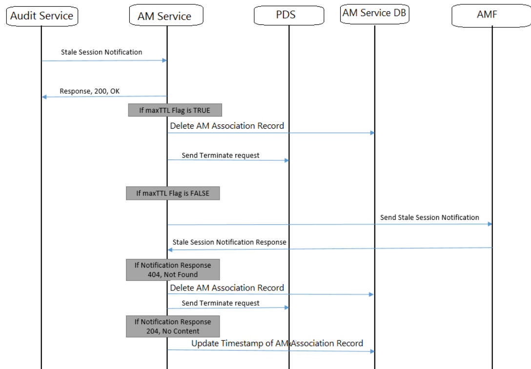
Figure 4-138 Example call flow for Stale Session Detection and Handling in AM Service:
