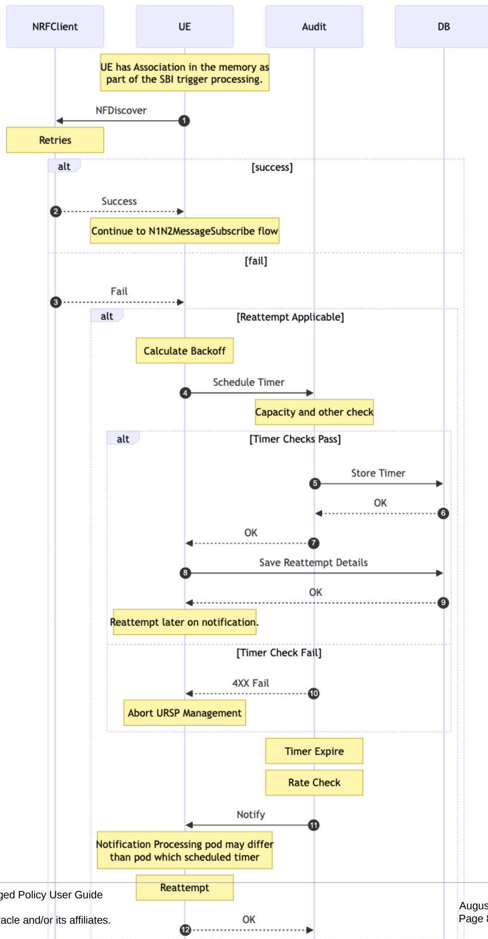
Figure 4-28 NFDDiscover Call Flow
