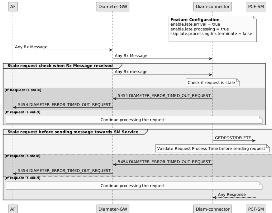
Figure 4-55 Sample call flow for stale Rx requests cleanup by Diameter Connector
