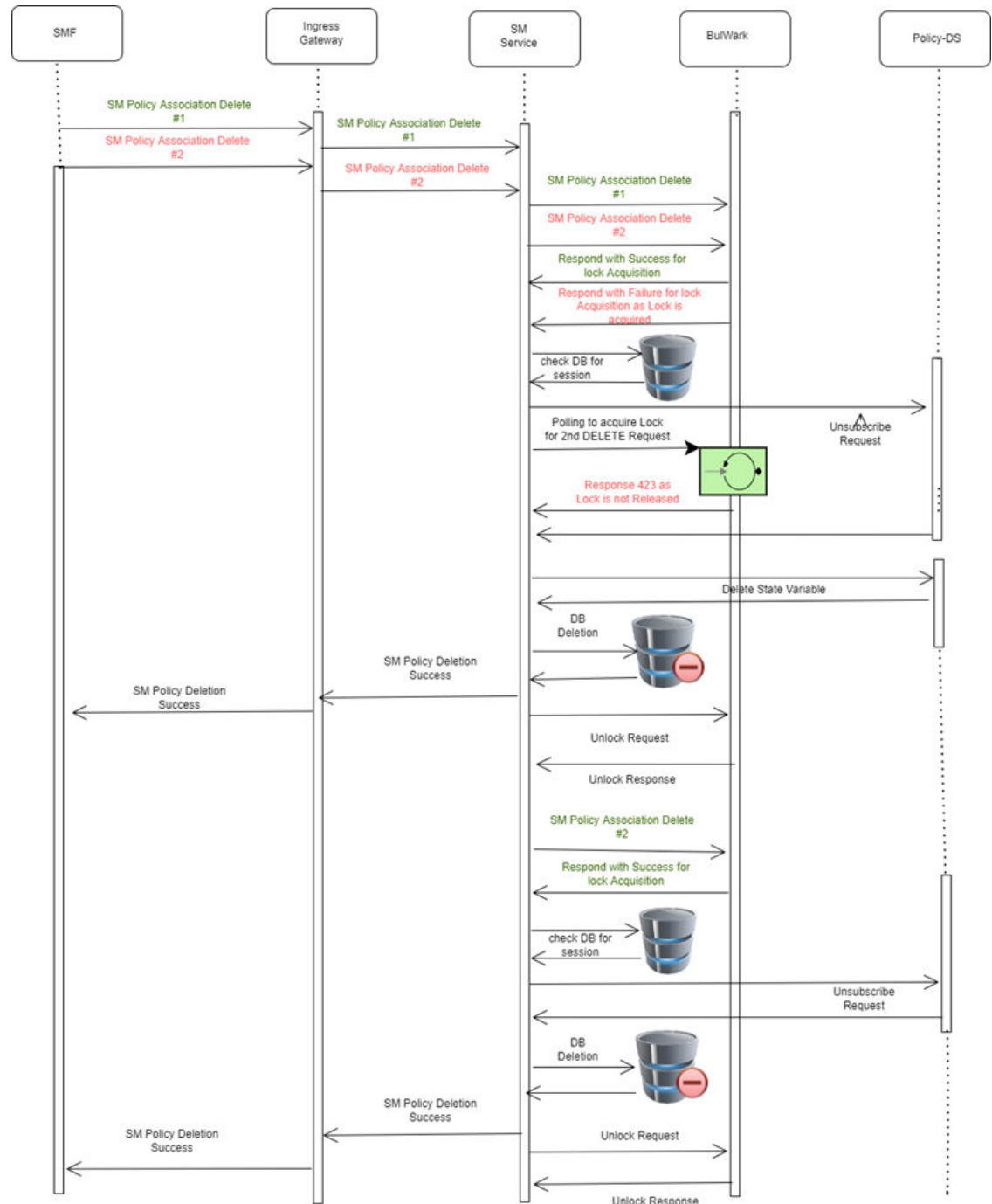
Figure 4-167 Call Flow - Bulwark Lock Request SM Delete Procedure
