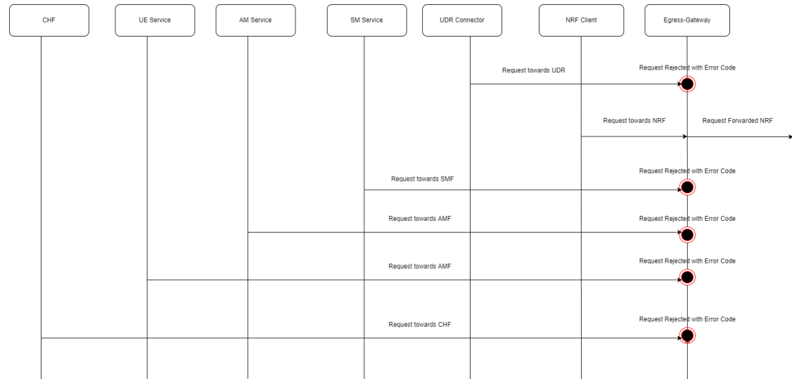
Figure 4-202 Call Flow for Egress Gateway COMPLETE SHUTDOWN
