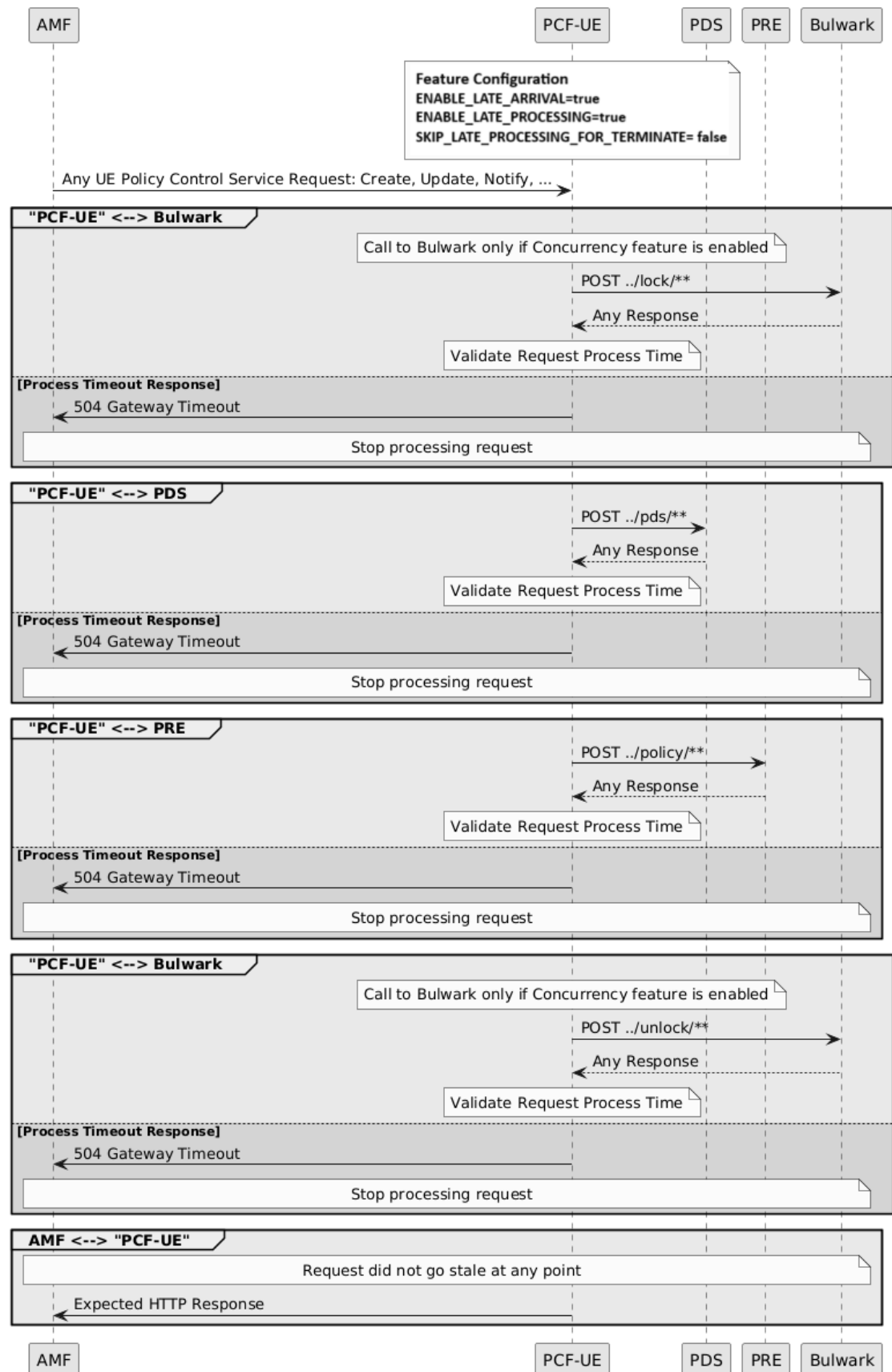
Figure 4-58 Sample call flow for stale requests cleanup by UE Policy service
