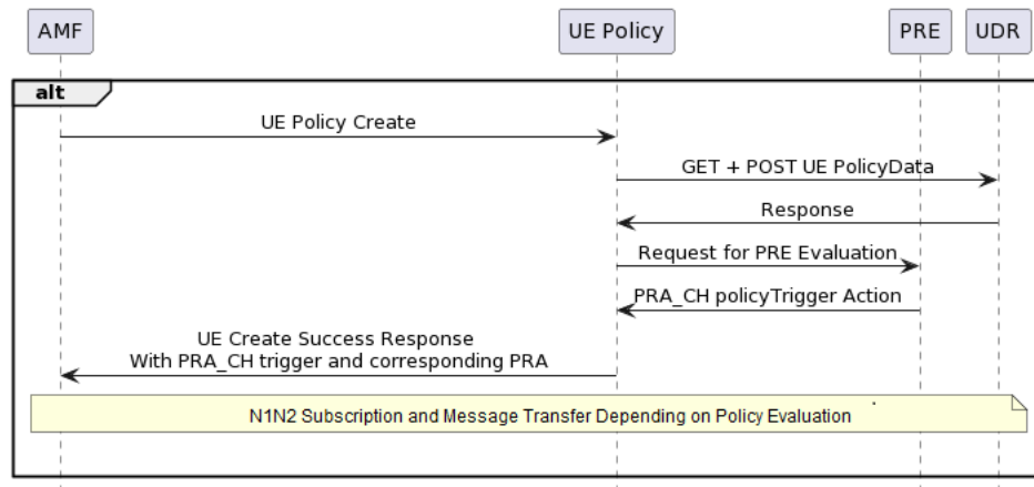
Figure 4-106 UE Policy Association create scenario:
