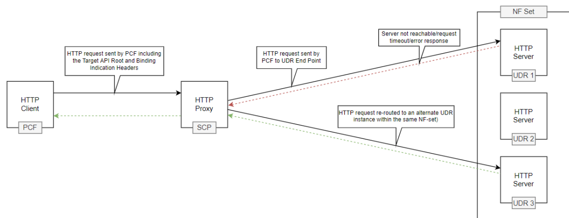
Figure 4-142 Example of NF Set and Binding Header based Indirect Communication
