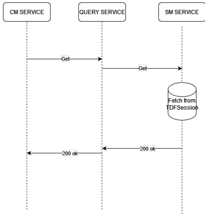
Figure 4-13 Fetch TDF Session
