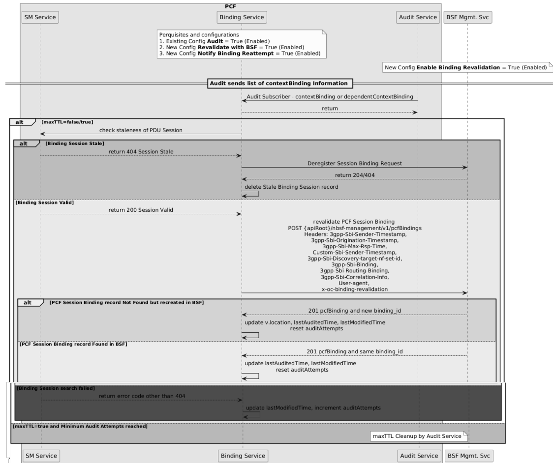
Figure 4-45 Stale binding detection and revalidation
