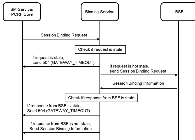
Figure 4-54 Sample call flow for stale requests cleanup by Binding service
