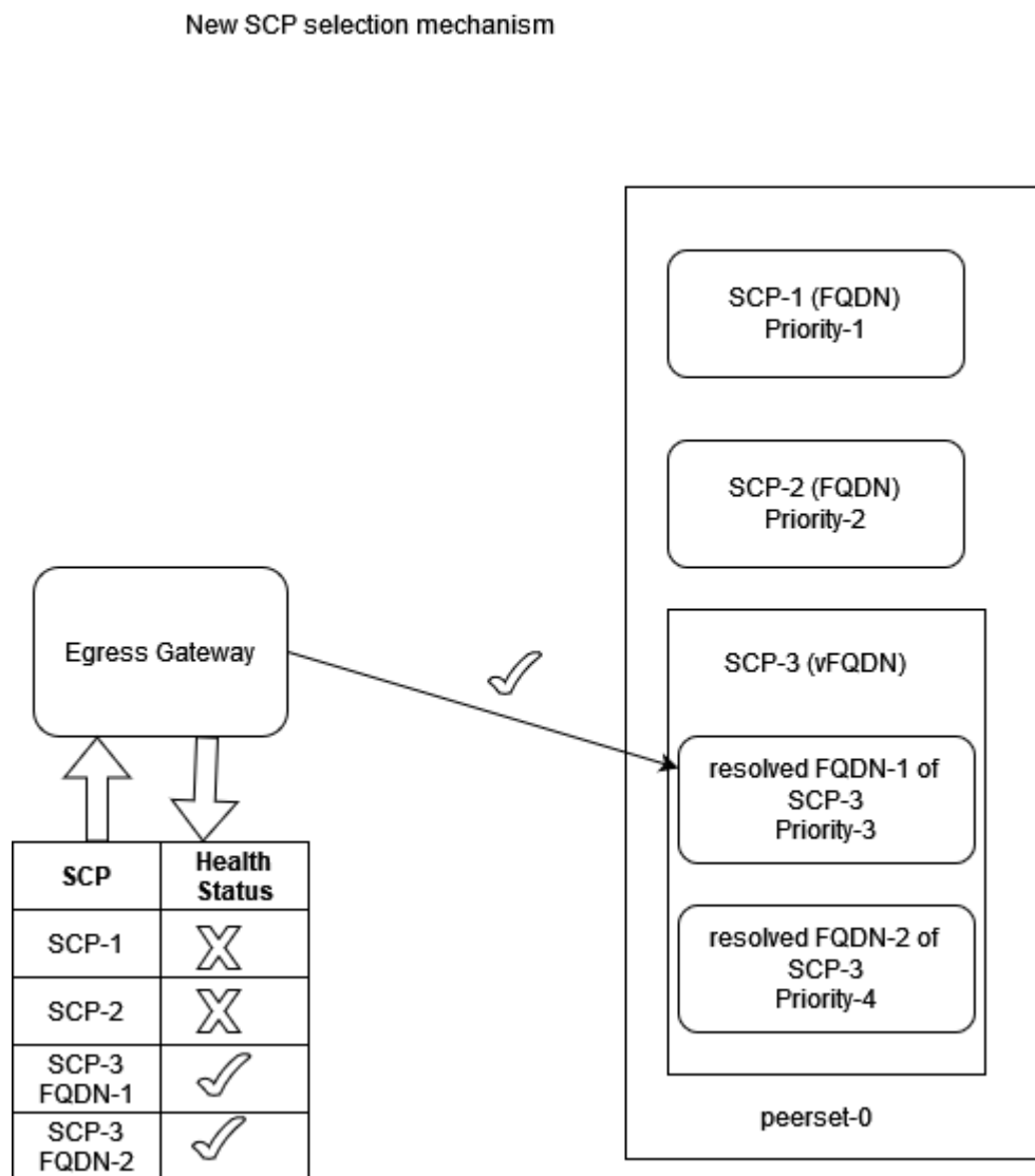
Figure 4-115 New SCP selection mechanism
