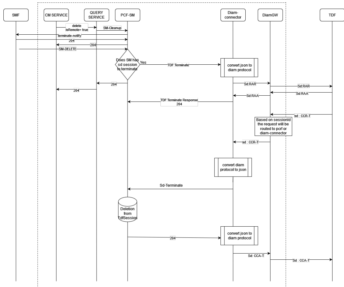
Figure 4-17 REMOTE DELETE SM SESSION
