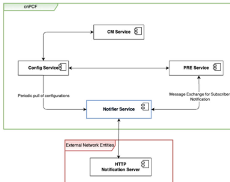
Figure 4-31 Notifier Service interactions with other Services
