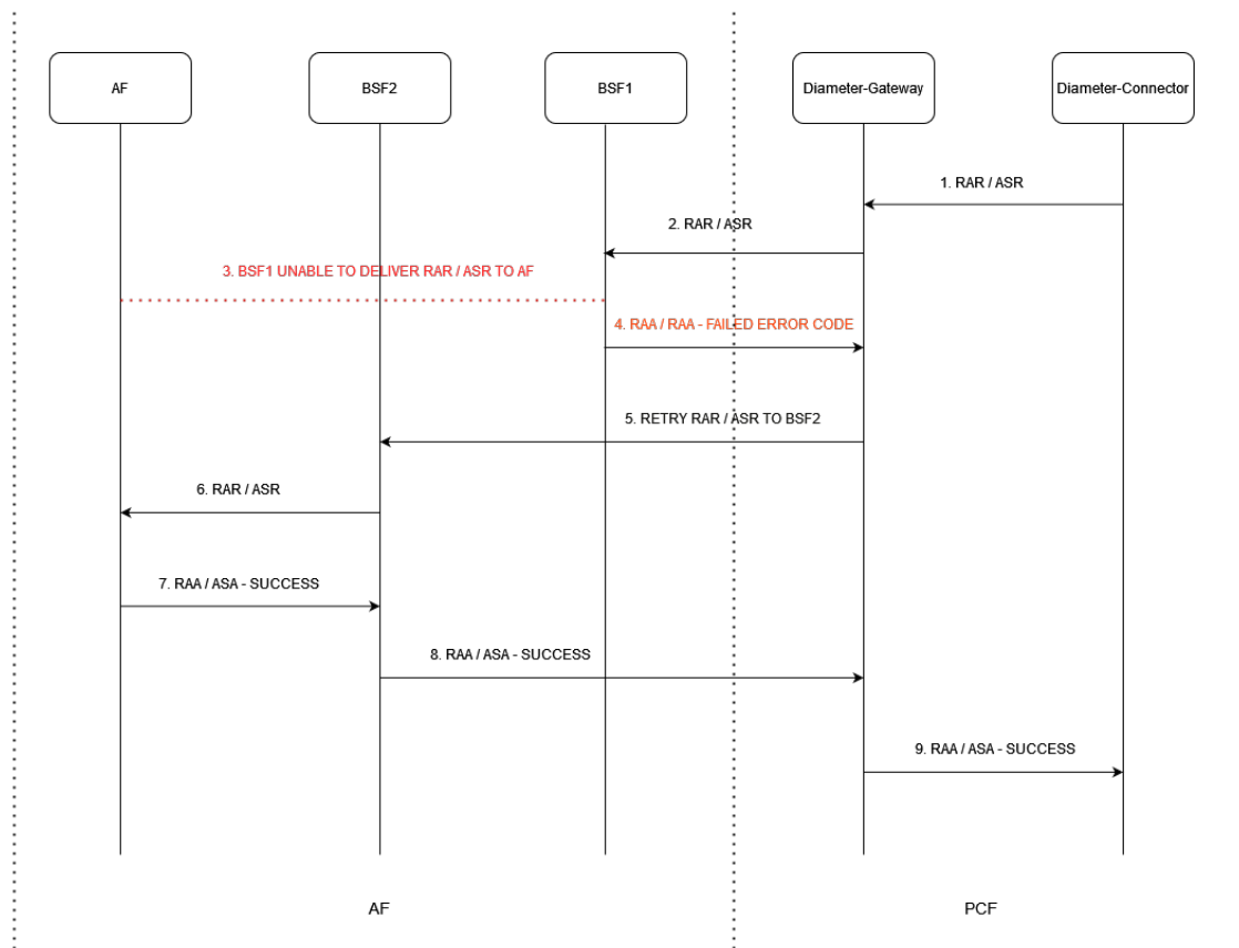
Figure 4-110 Call Flow Rx RAR or Rx ASR one time message retry - Success Case:
