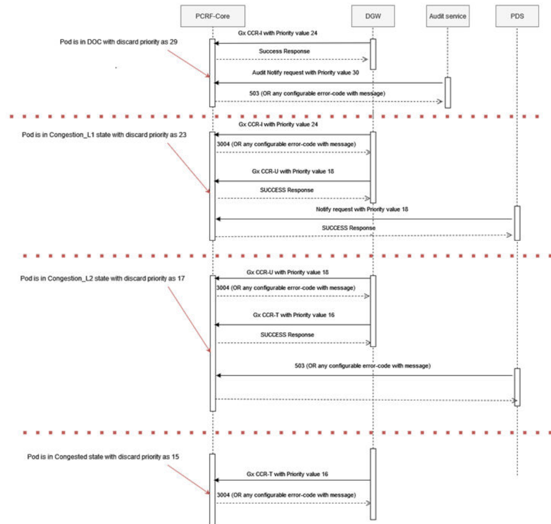
Figure 4-39 PCRF Core Service Congestion Control Call Flow
