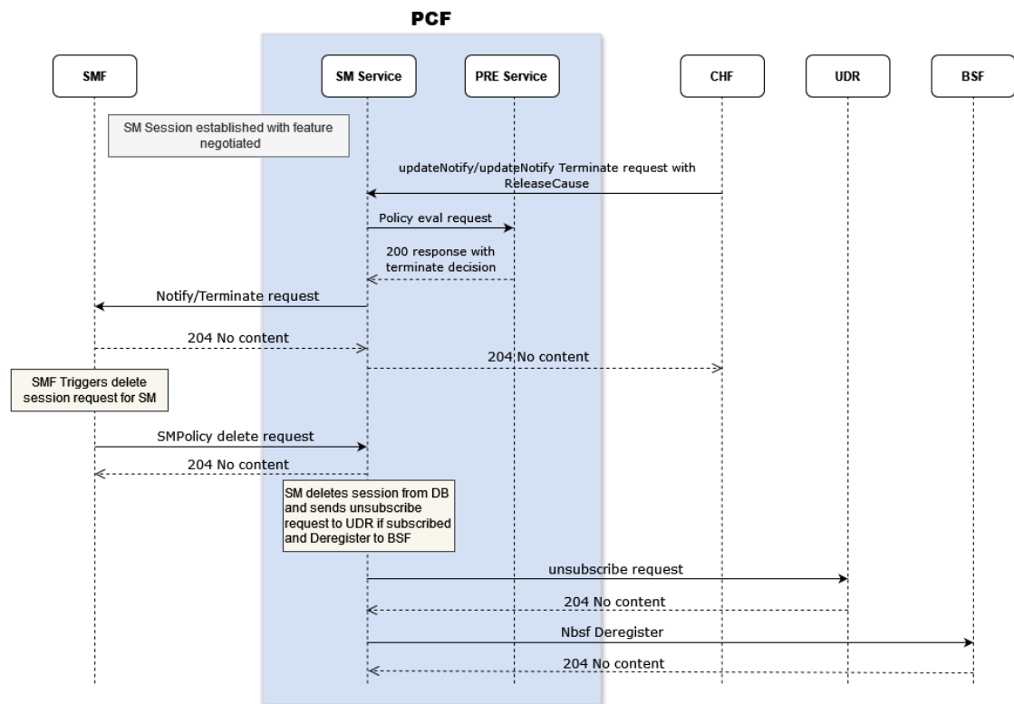
Figure 4-89 SM Terminate for CHF updateNotify or updateNotifyTerminate:
