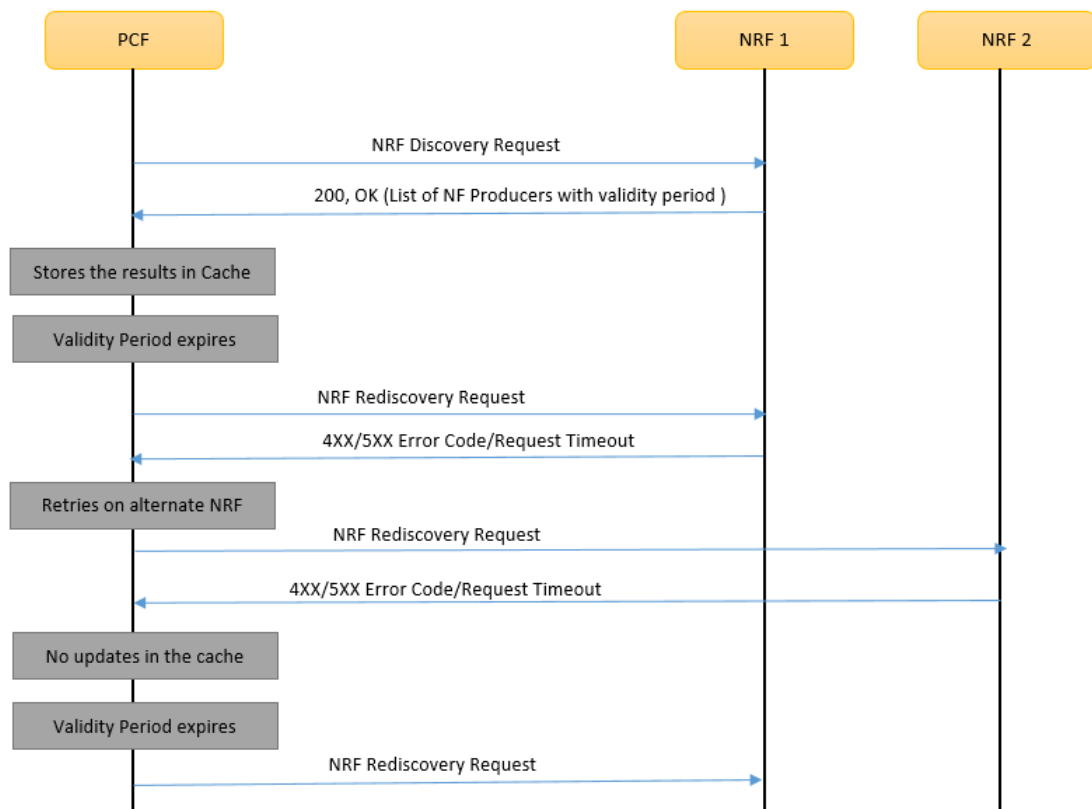
Figure 4-206 Call Flow - NF Discovery Error Scenario
