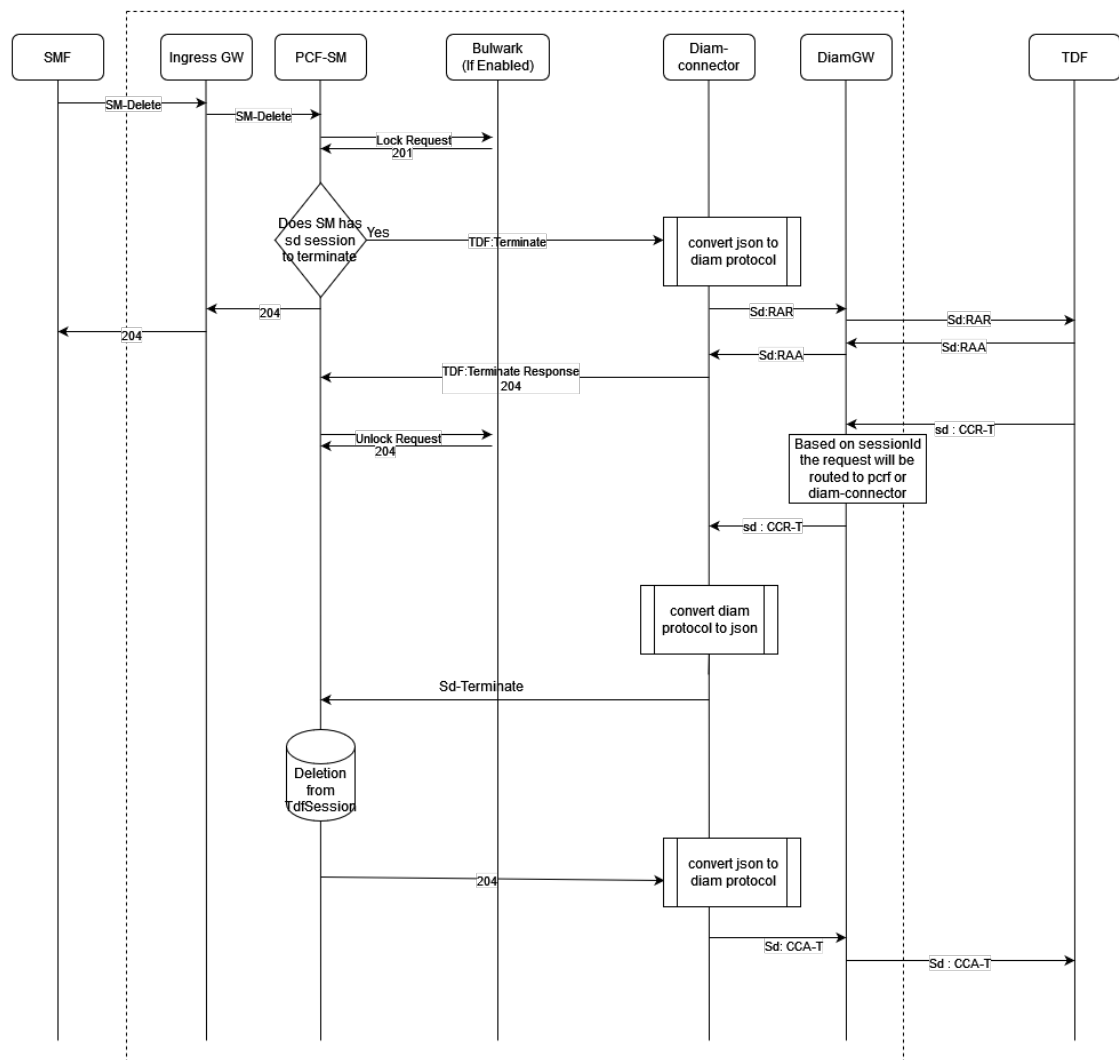
Figure 4-10 Sd Session Termination (PCF → TDF)
