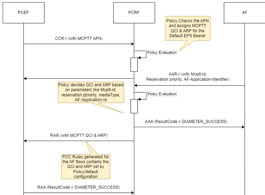
Figure 4-220 MCPTT QCI & ARP settings for MCPTT AF flows
