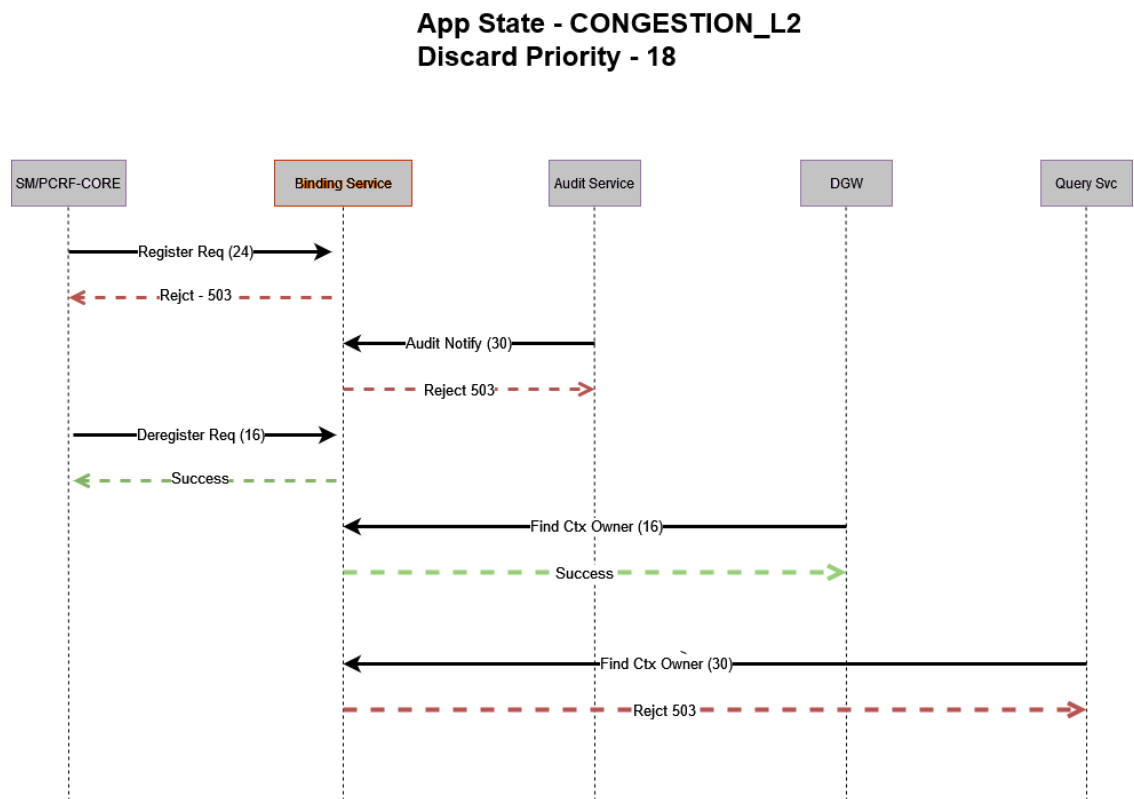
Figure 4-39 Binding Service in Congestion_L2 State
