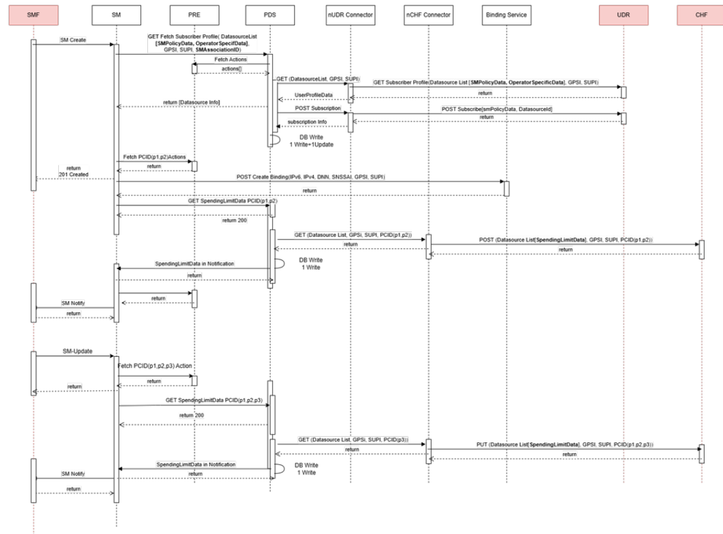
Figure 4-209 Intermediate Spending Limit with Specific Policy Counter ID for SM Service
