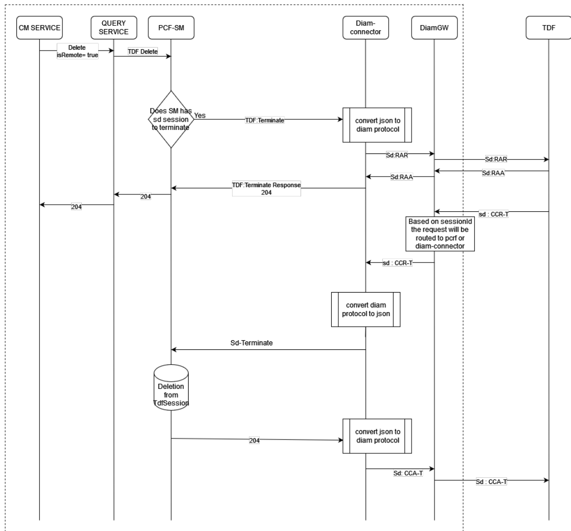
Figure 4-11 REMOTE DELETE TDF SESSION
