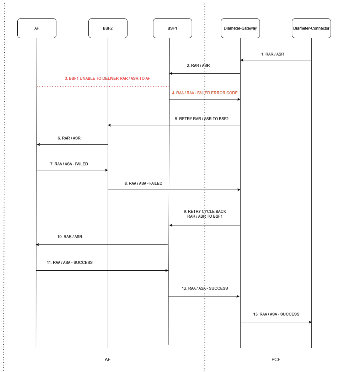
Figure 4-108 RX RAR/RX ASR Retry - Peer Cycle Back When Retry Count > Alternate Peers
