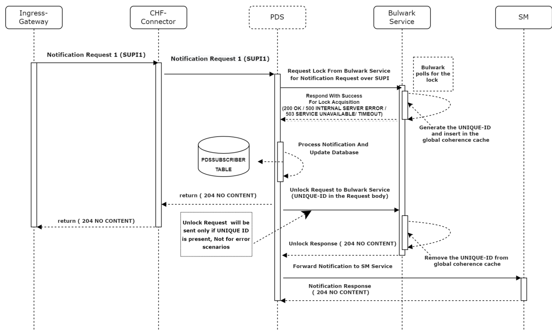
Figure 4-185 Call Flow - Bulwark Lock Request For CHF Notification
