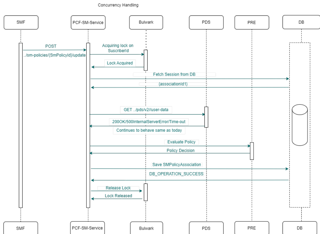
Figure 4-156 Concurrency enabled for SM Update for a single session
