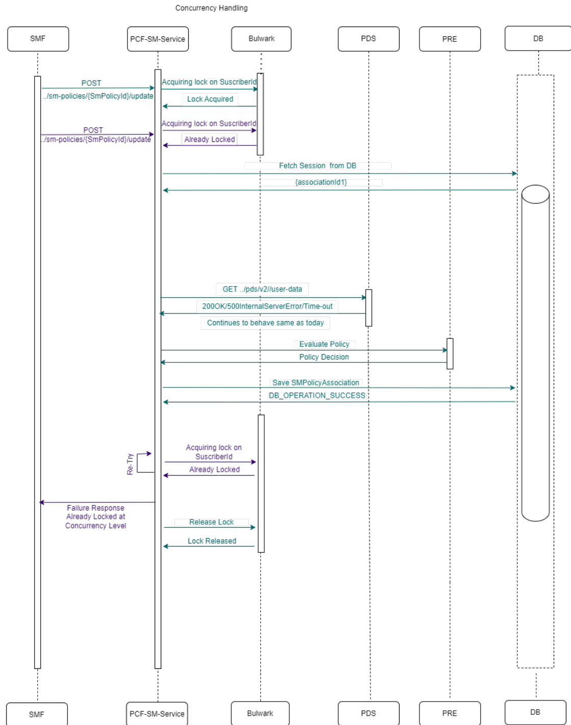
Figure 4-158 Retrial failure when there are multiple updates for same subscriber in different sessions
