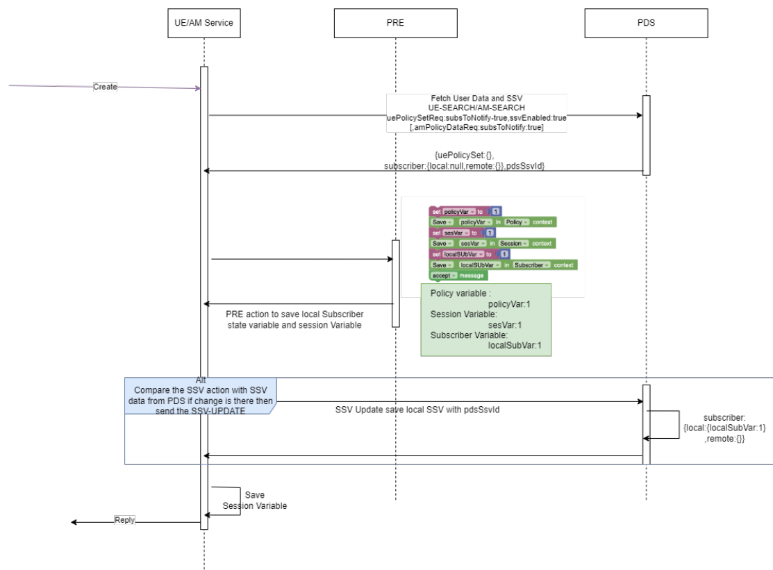
Figure 4-215 State variables in create session call flow
