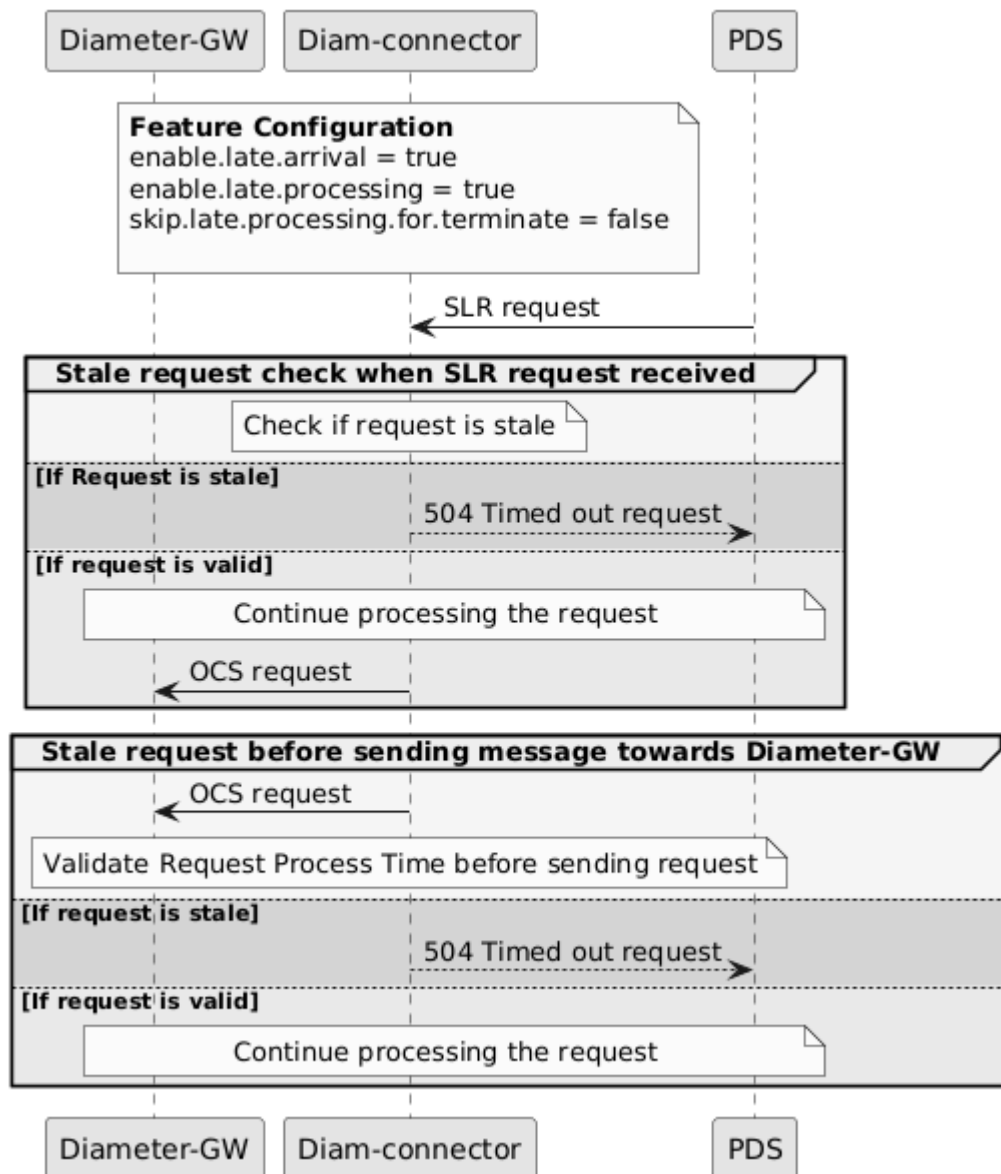
Figure 4-52 Sample call flow for stale SLR requests cleanup by Diameter Connector
