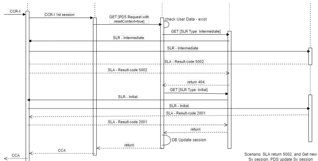
Figure 4-71 SLA Returns 5002, Get New Sy Session, PDS Update Sy Session
