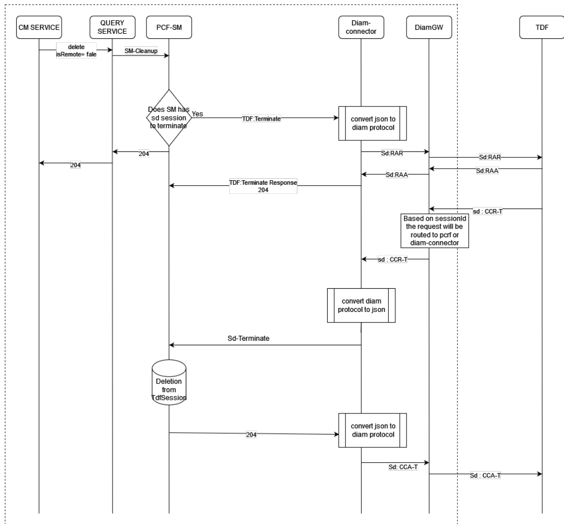
Figure 4-12 LOCAL DELETE SM SESSION
