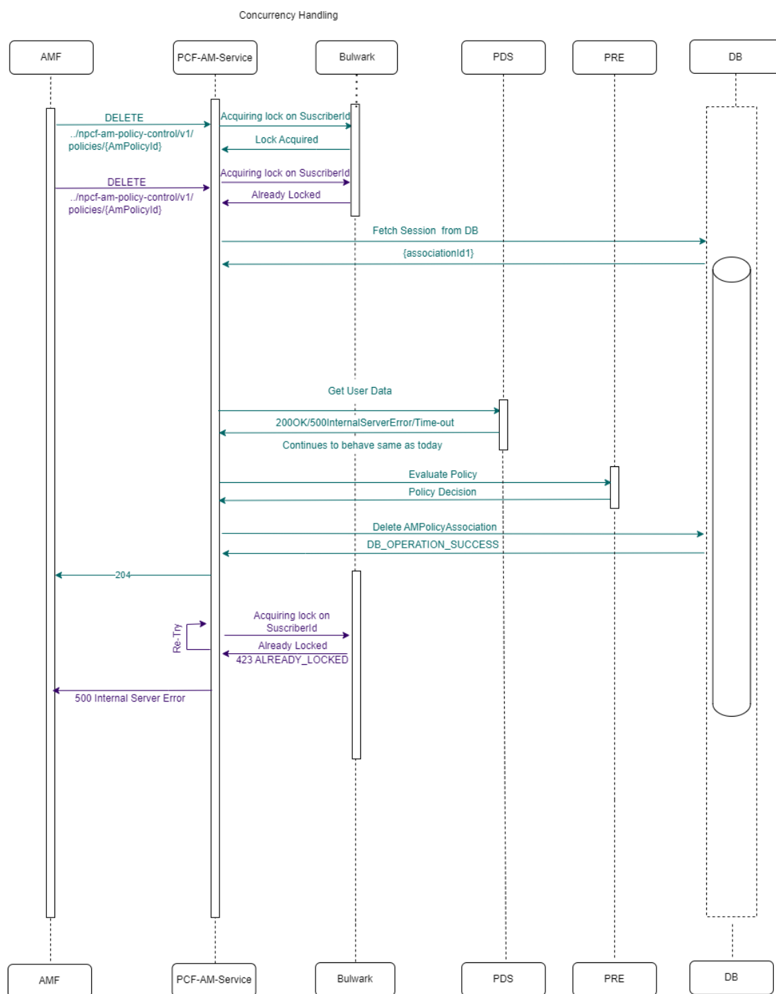
Figure 4-170 Two AM-Delete requests for same Subscriber and retry failure (retry =1)
