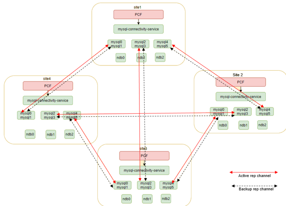
Figure 4-141 Four-Site Georedundancy Deployment
