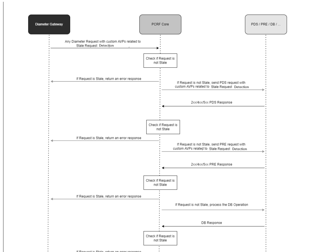
Figure 4-48 Sample call flow for stale requests cleanup by PCRF Core
