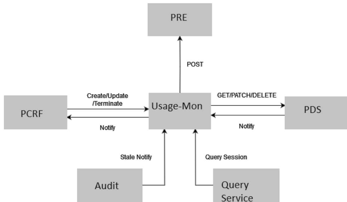
Figure 4-34 Usage Monitoring Service and other Policy services
