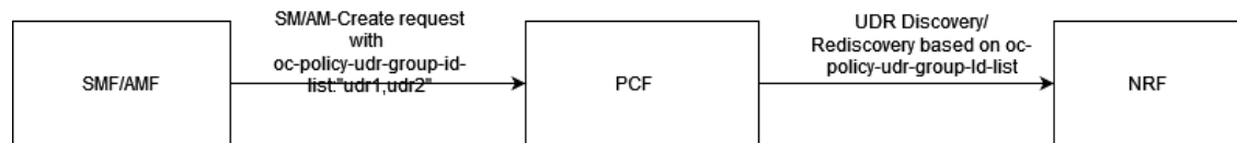
Figure 4-87 UDR Discovery with oc-policy-udr-group-id-list Header to NRF
