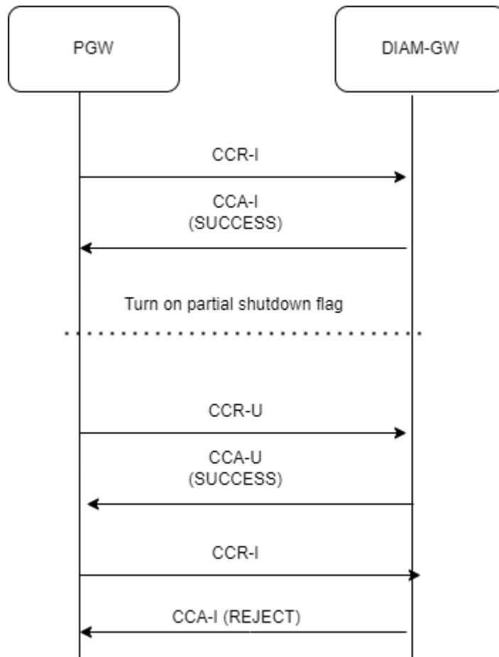
Figure 4-196 Call Flow for Diameter Gateway PARTIAL SHUTDOWN
