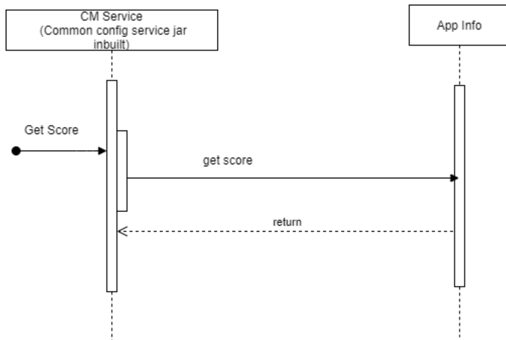
Figure 4-211 Call flow to Get the NF Score
