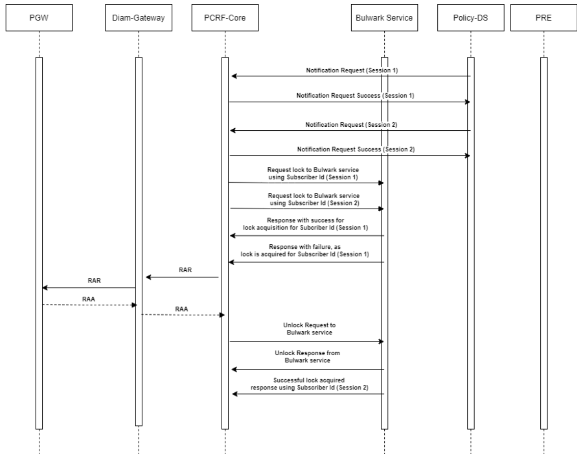
Figure 4-184 Call Flow- PDS notification (RAR) Integration with Bulwark Service
