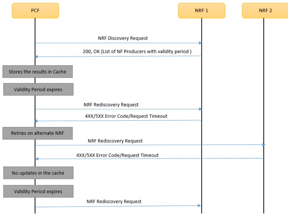
Figure 4-202 Call Flow - NF Discovery Error Scenario
