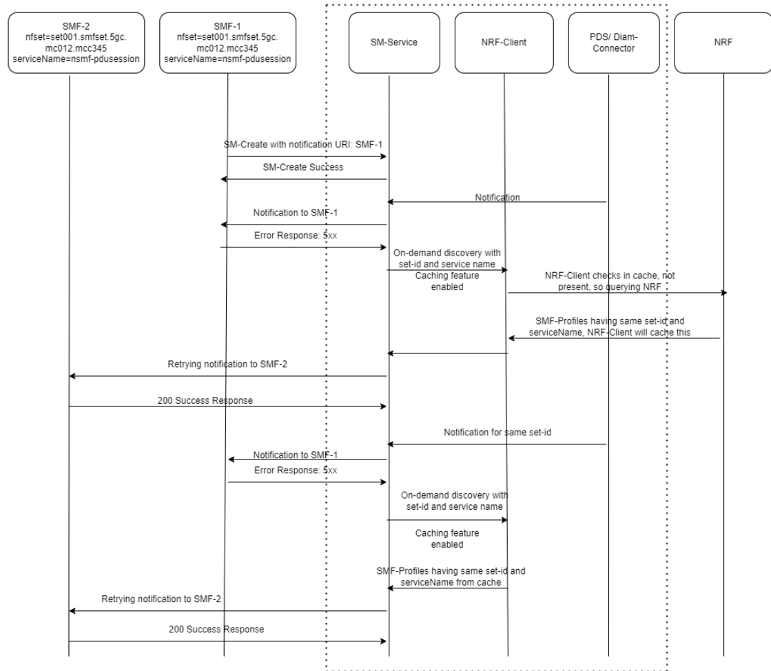
Figure 4-65 SMF Notification for SM Policy (NFSetid based discovery for retry on Notification Request failure)
