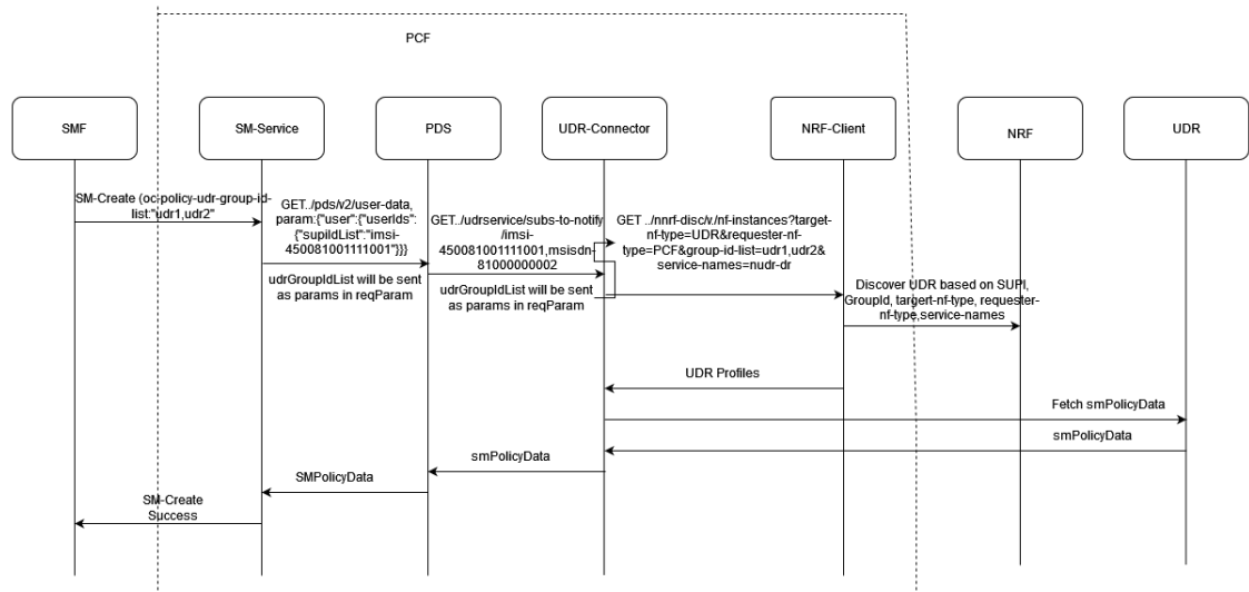
Figure 4-88 SMF sends SM Policy Association Request with oc-policy-udr-group-id
