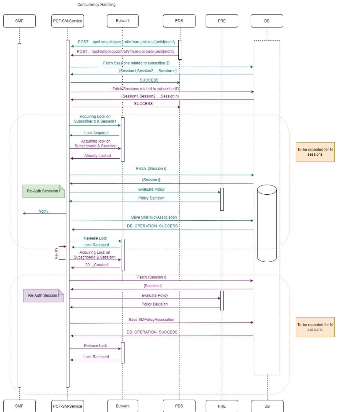
Figure 4-155 Call Flow for SM Update-Notify Request (Two Notifications from Same Subscriber and n Sessions Each)
