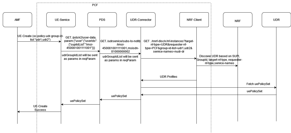
Figure 4-90 AMF sends UE Policy Association Request with oc-policy-udr-group-id
