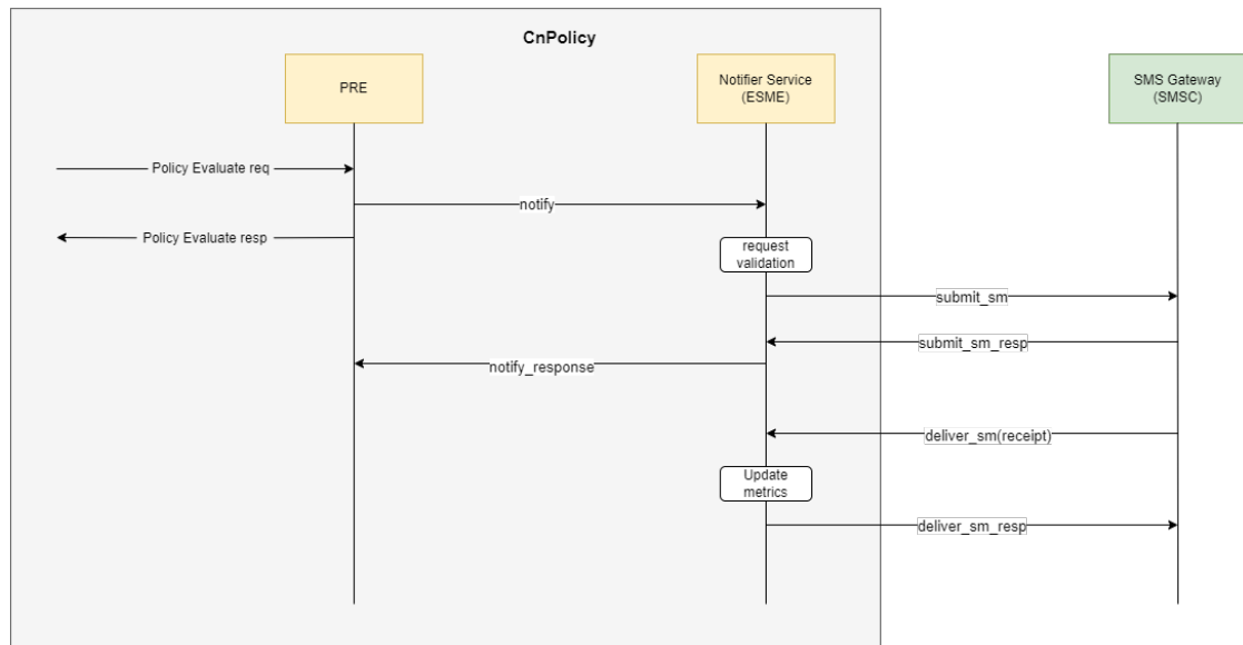
Figure 4-99 Call flow for sending messages using SMPP protocol
