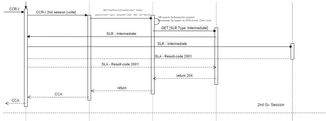
Figure 4-73 Second Gx Session
