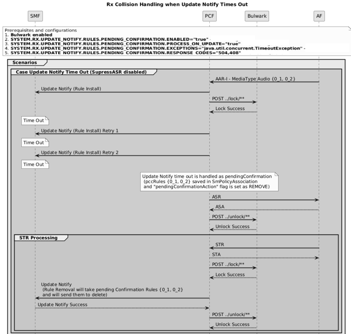
Figure 4-16 Handling Collision Between AAR and STR Messages During UpdateNotify-Timeout Scenario
