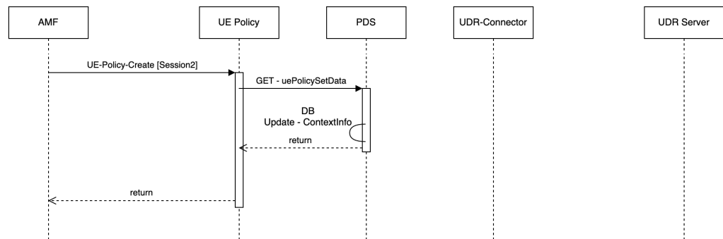
Figure 4-205 resetContextUePolicySetData set to false when there are existing sessions for UE Policy service
