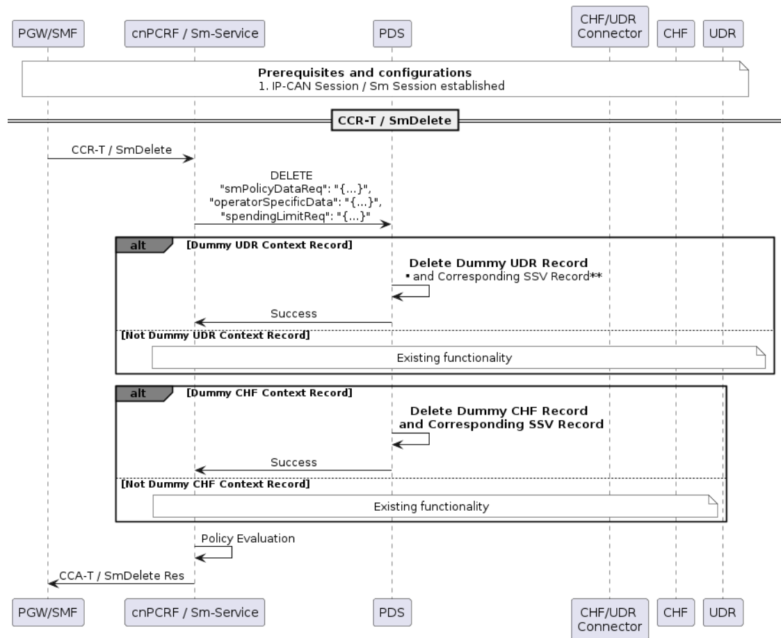
Figure 4-64 PDS Dummy Context during SM Delete or PCRF Core CCR-T Call Flow
