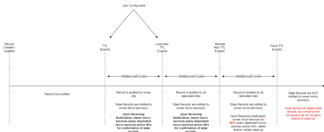
Figure 4-130 Timeline view of Audit Service
