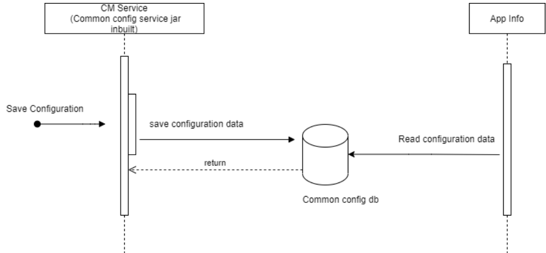
Figure 4-210 Call flow to Save Configuration Data
