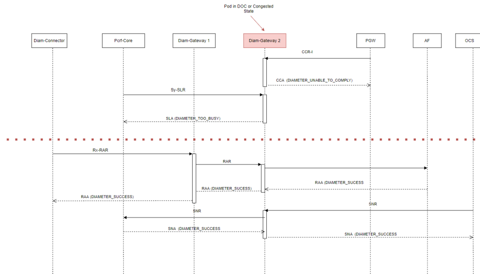
Figure 4-143 Call flow diagram for Diameter Congestion Control
