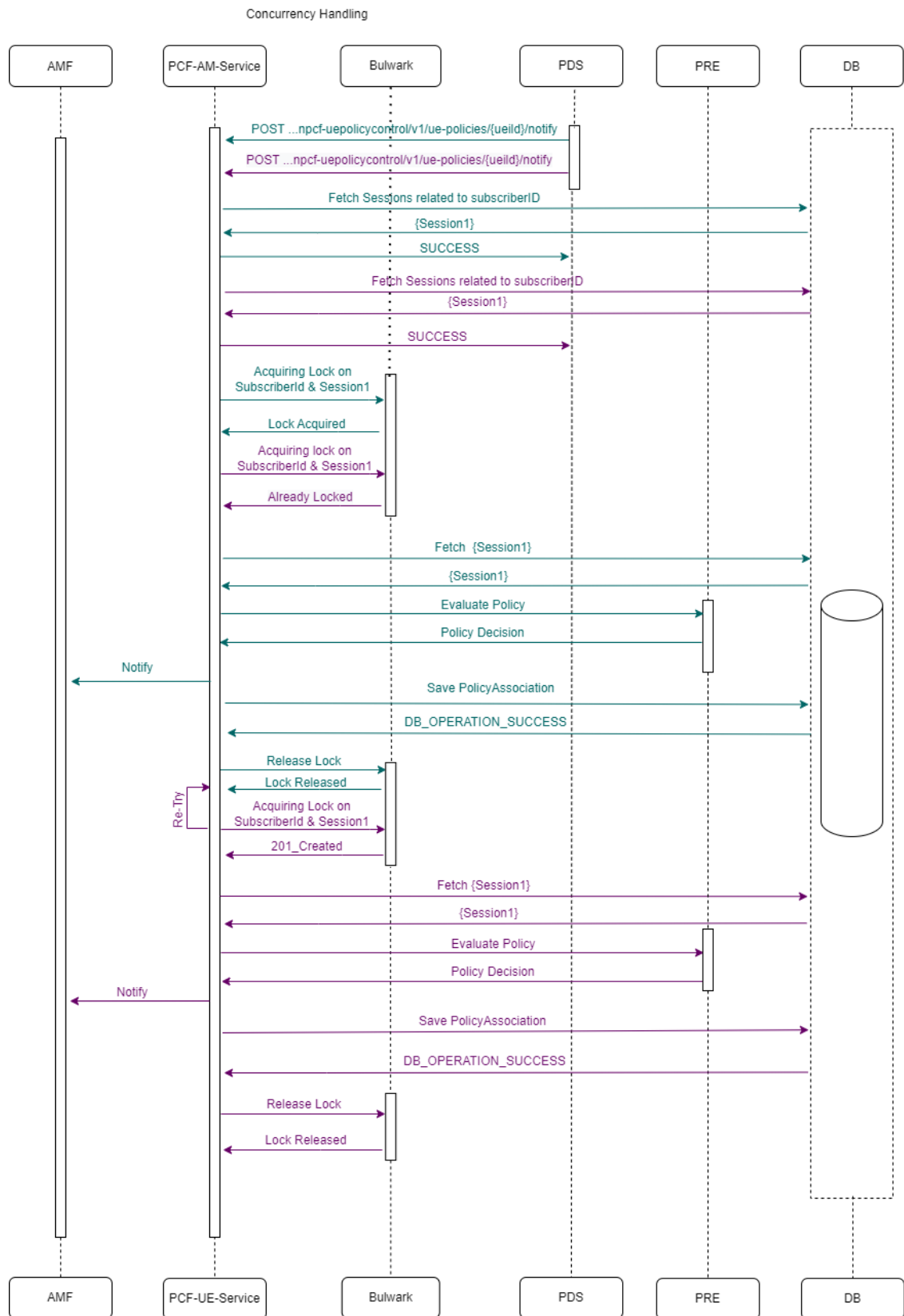
Figure 4-181 Two UENotify requests for same Subscriber each having 1 session
