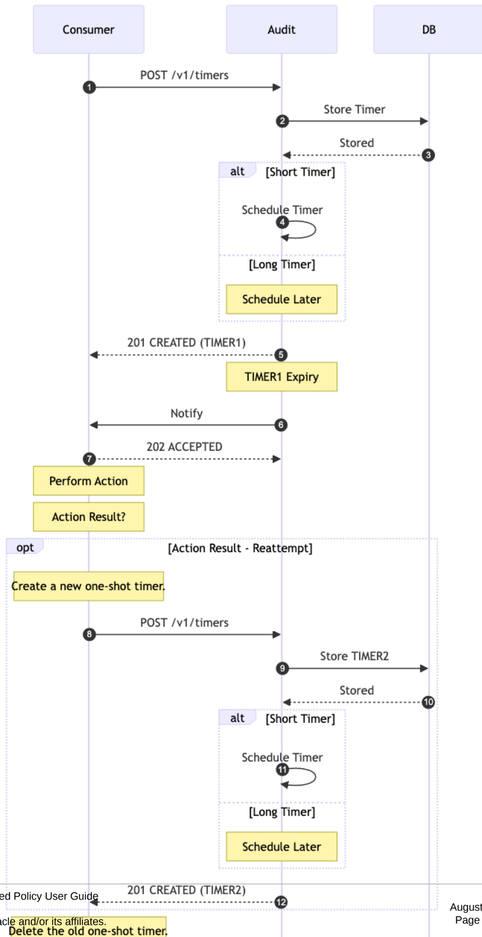
Figure 4-23 Timer Service Overview
