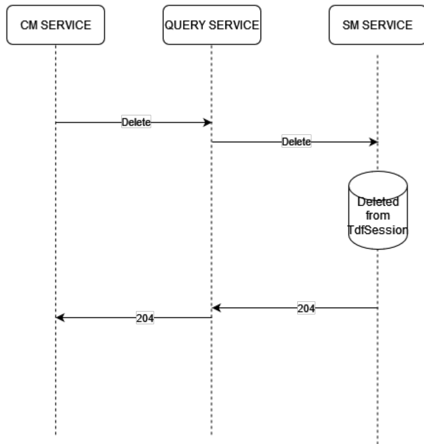
Figure 4-10 LOCAL DELETE TDF SESSION
