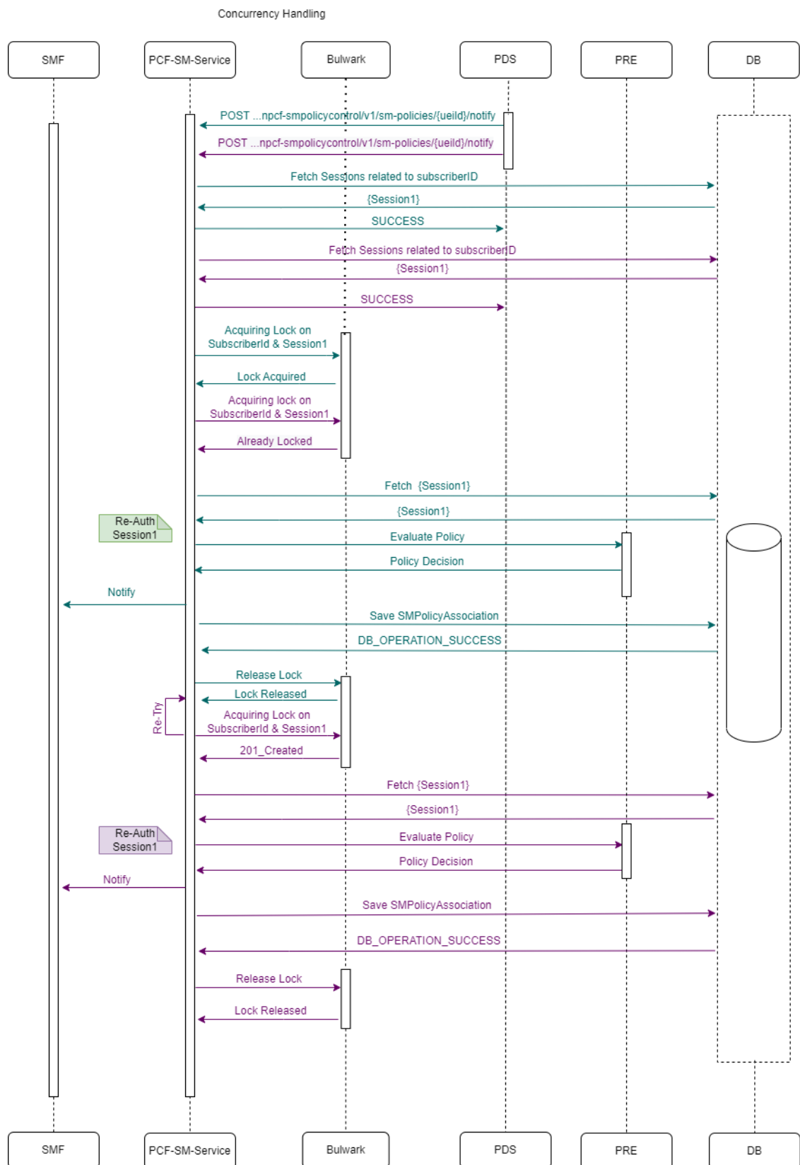
Figure 4-154 Call Flow for SM Update-Notify Request (Two Notifications and 1 Session)
