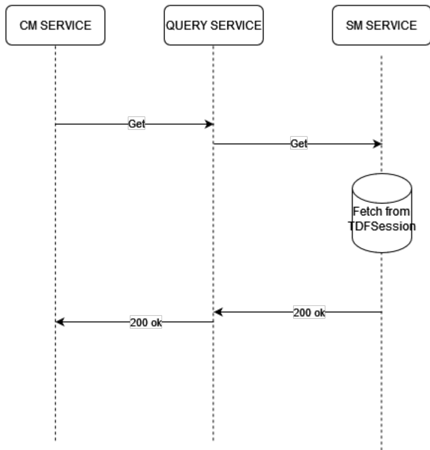
Figure 4-9 Fetch TDF Session
