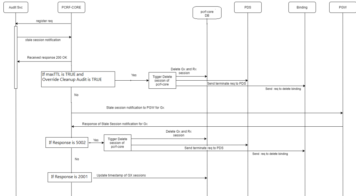
Figure 4-135 Example call flow for Stale Session Detection and Handling in PCRF Core Service
