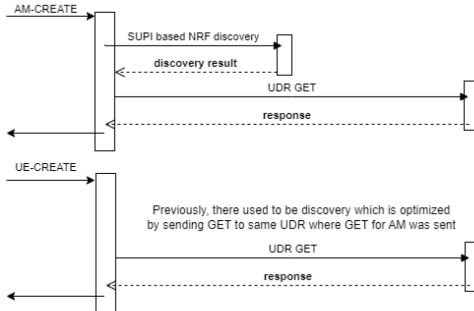
Figure 4-94 Reuse of UDR profile for amPolicyData GET in uePolicySet GET
