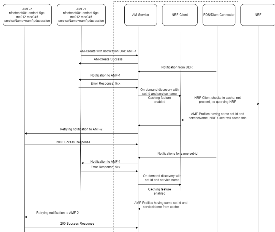
Figure 4-66 AMF Notification for AM Policy (NFSetid based discovery for retry on Notification Request failure)
