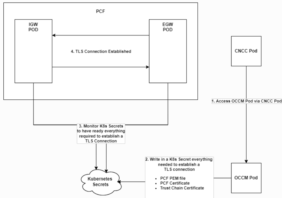
Figure 4-57 Policy Integration with OCCM
