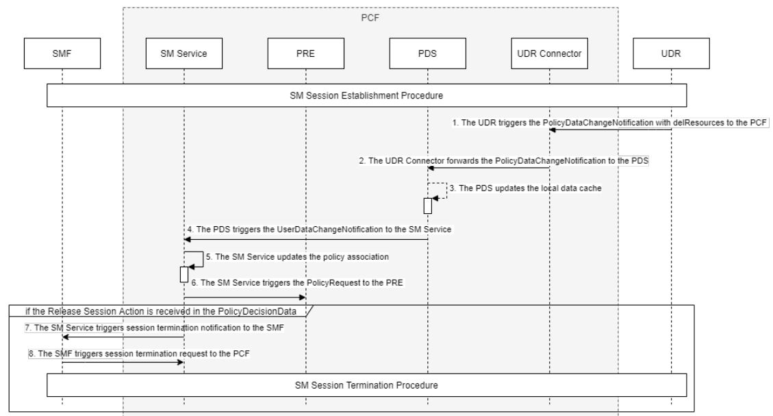
Figure 7-13 Call Flow for UDR Subscriber Resource Deletion
