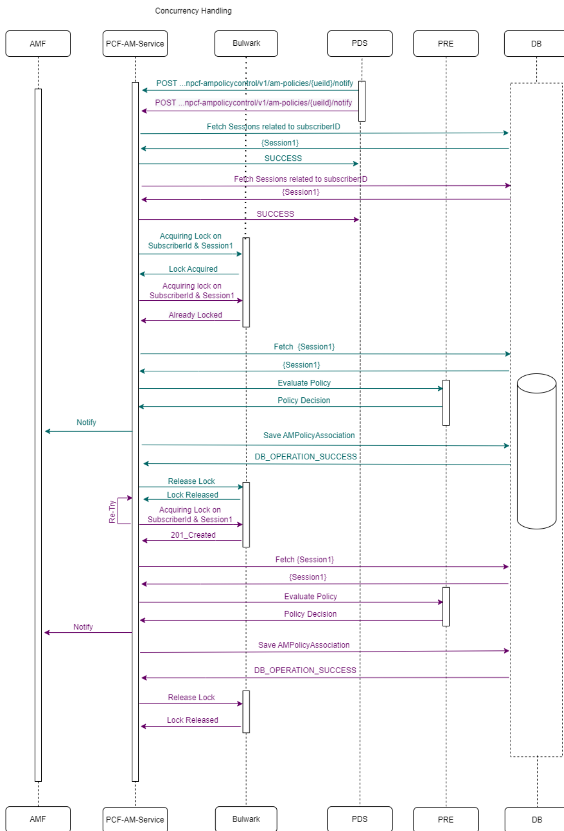
Figure 4-173 Two AM-Notify requests for same Subscriber each having 1 Session
