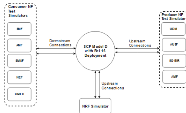
Figure 4-3 SCP Model D Topology 2
