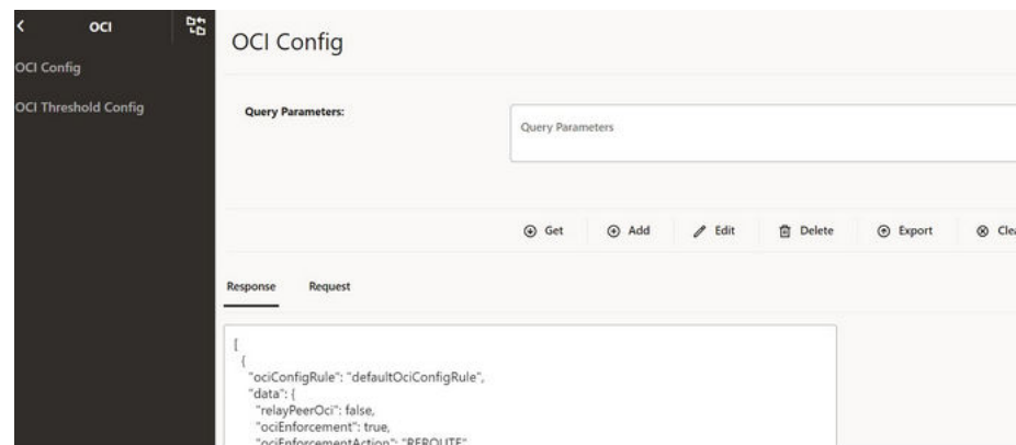
Figure 4-26 OCI Config
