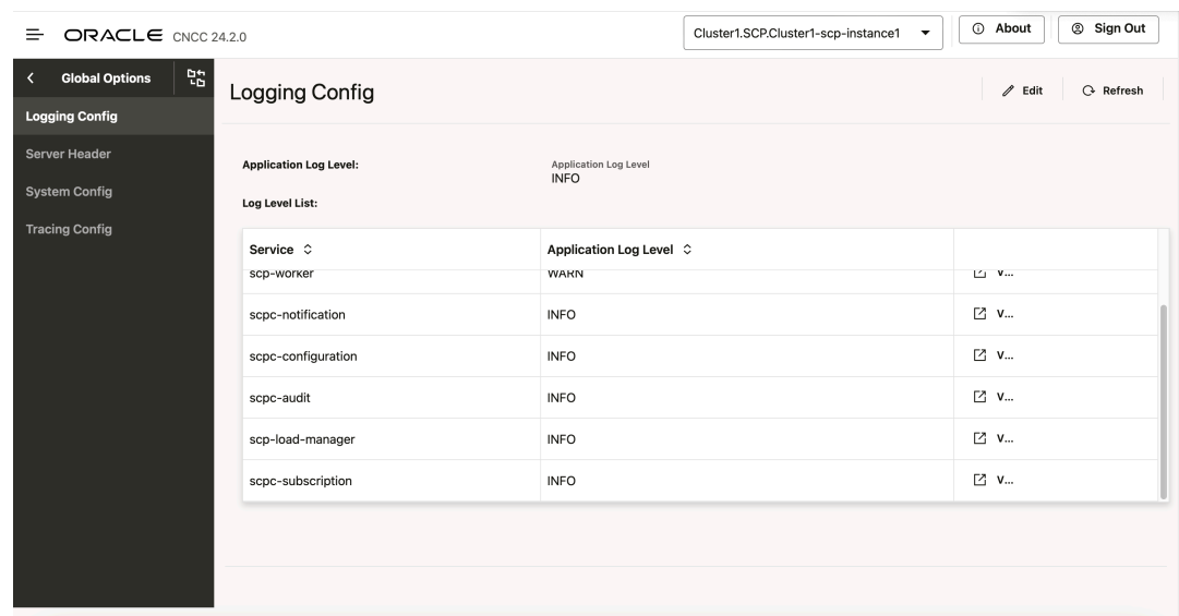
Figure 4-39 Logging Config
