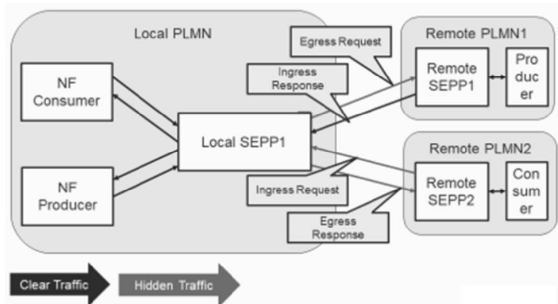
Figure 3-30 Topology Hiding Architecture
