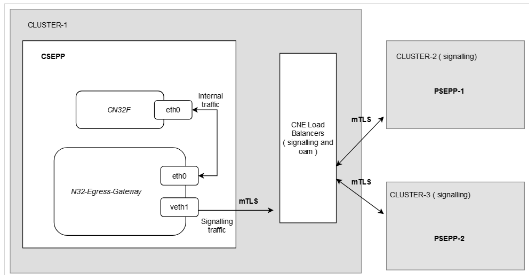
Figure 3-22 Egress Traffic Segregation
