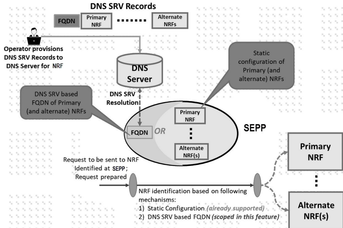
Figure 3-4 Call Flow of NRF Selection Mechanisms Using nrf client
