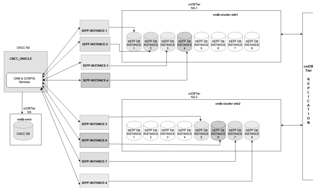
Figure 3-19 Multiple SEPP instances on shared cnDBTier cluster architecture
