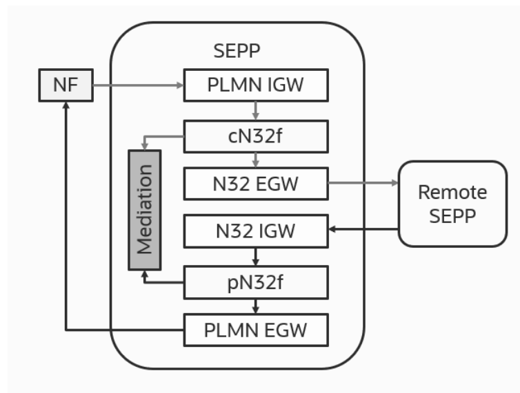
Figure 3-28 Mediation Representation with SEPP
