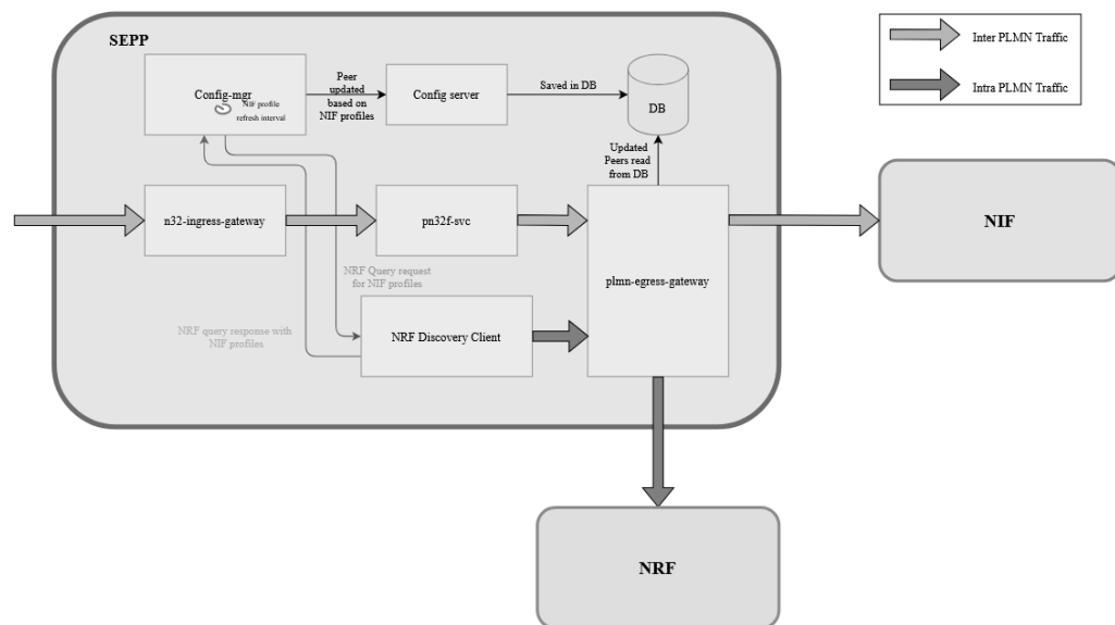
Figure 3-7 NIF Instance Selection and Traffic Routing
