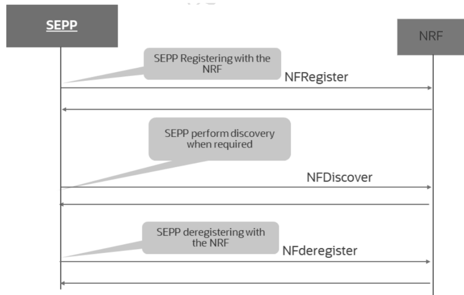
Figure 3-51 NRF Interface Registration and Reregistration
