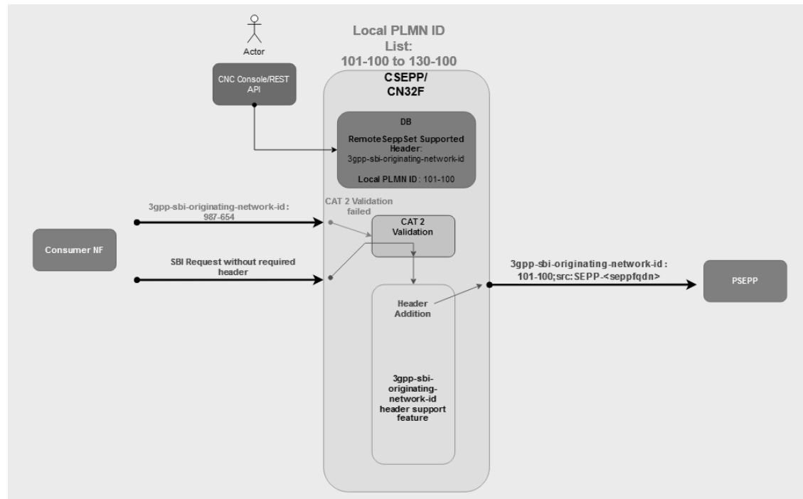
Figure 3-23 C SEPP side functionality
