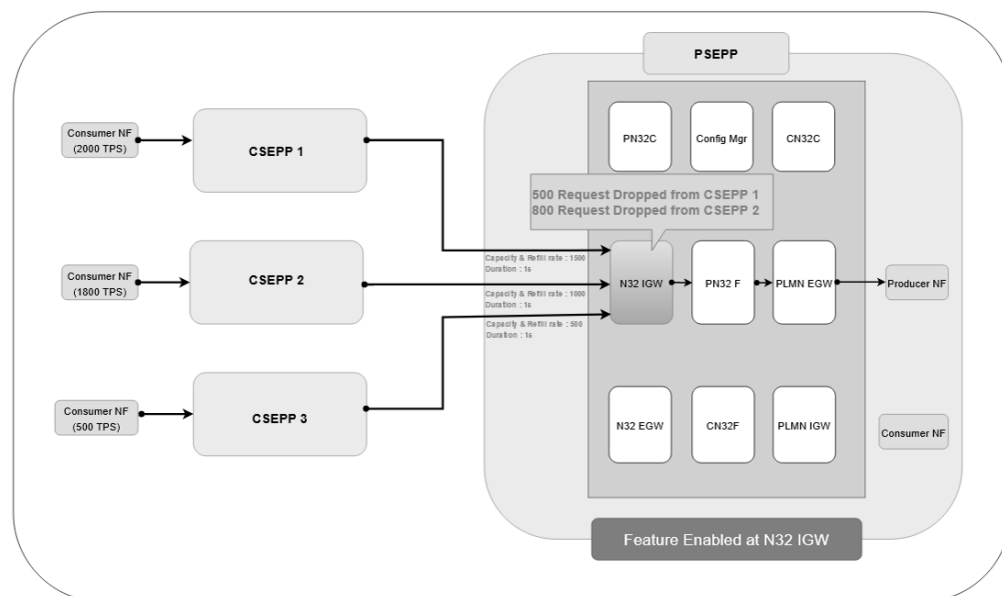
Figure 3-63 Rate limiting for Ingress Roaming Signaling per Remote SEPP Set Architecture
