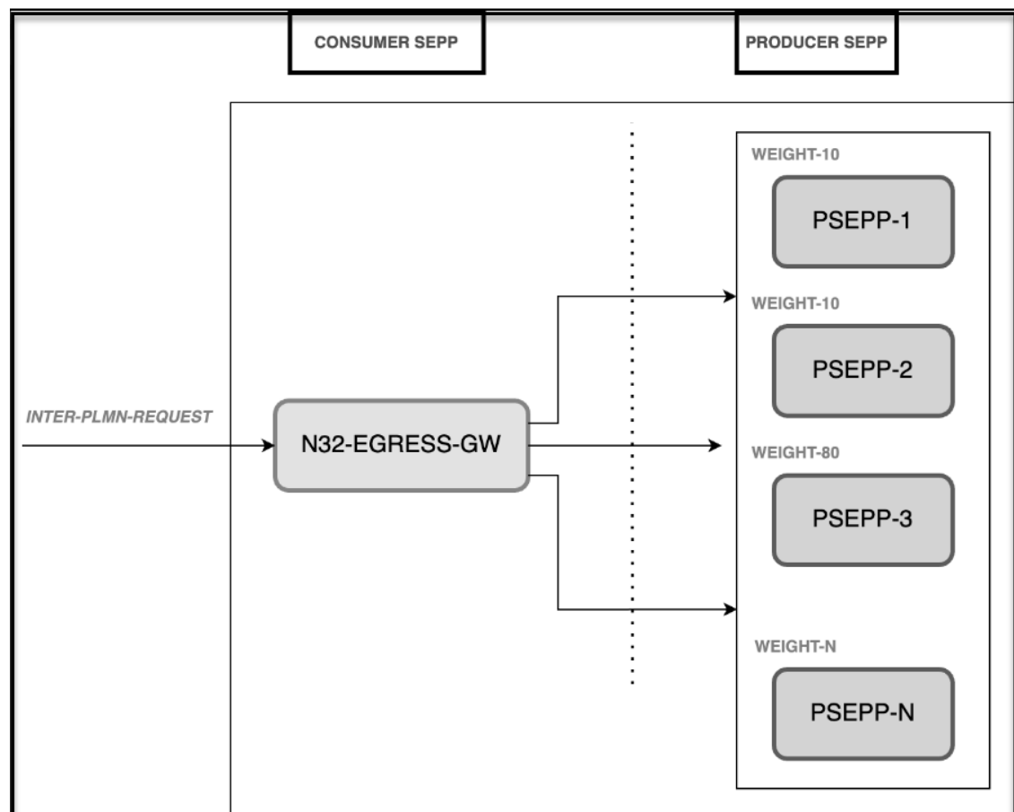
Figure 3-26 Architecture
