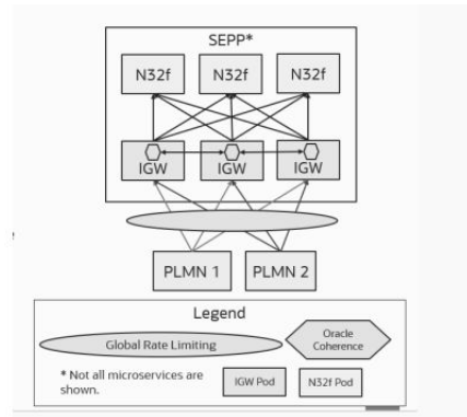
Figure 3-38 Architecture
