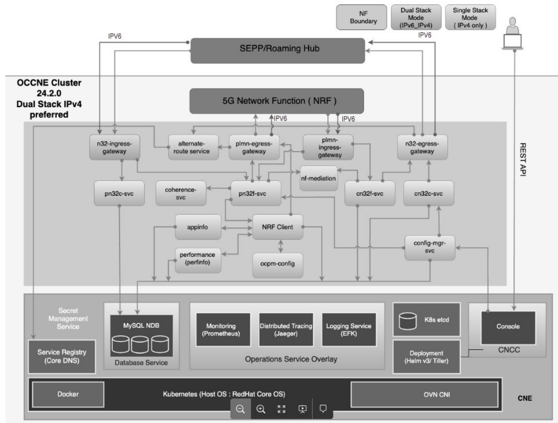
Figure 2-2 Security Edge Protection Proxy Architecture
