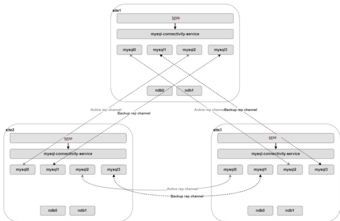
Figure 3-66 Three-Site Georedundancy
