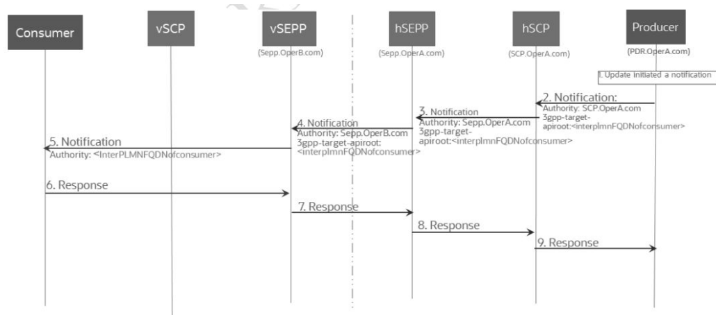
Figure 3-50 SEPP removes the 3GPP-SBI-Target-Apiroot header
