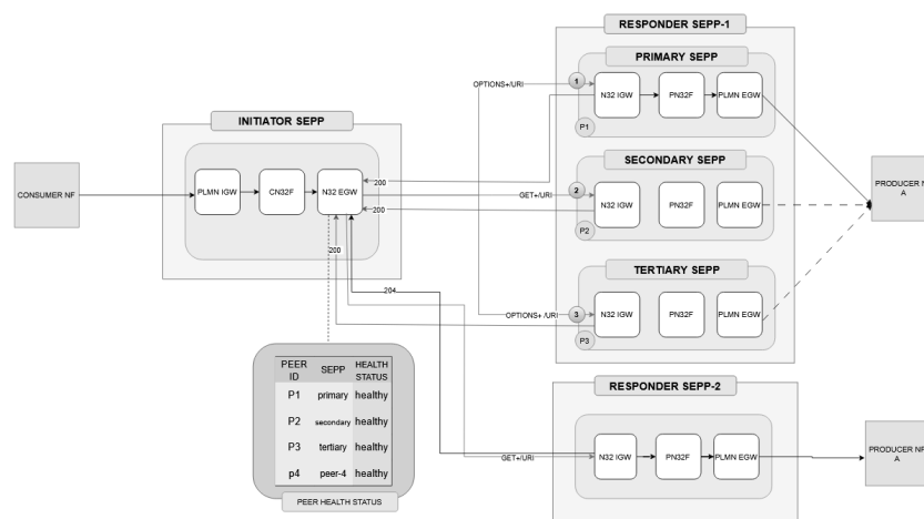
Figure 3-20 Proactive Status Updates on SEPP Architecture
