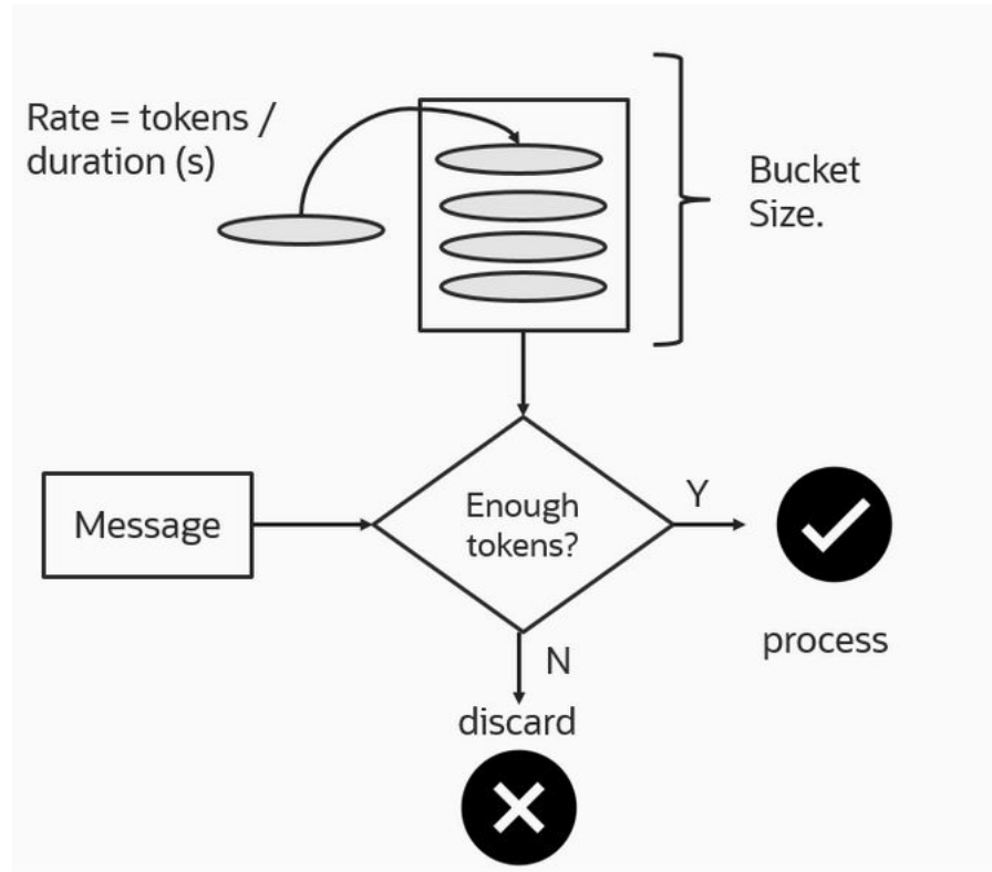
Figure 3-37 Algorithm Overview
