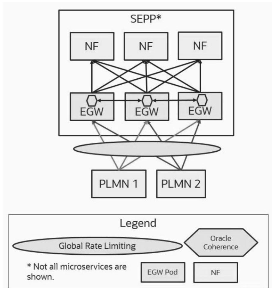
Figure 3-35 Architecture
