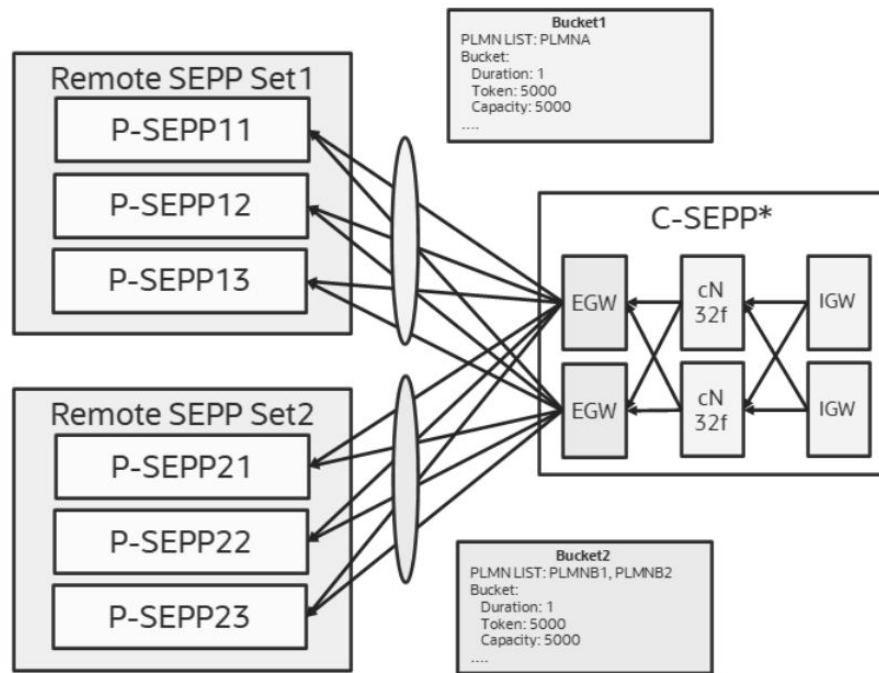
Figure 3-73 Implementation at C-SEPP
