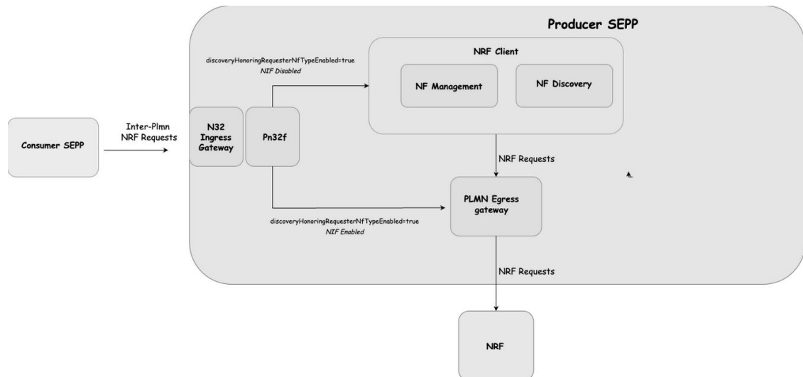
Figure 3-3 Architecture Diagram of NRF Selection Mechanisms Using nrf client
