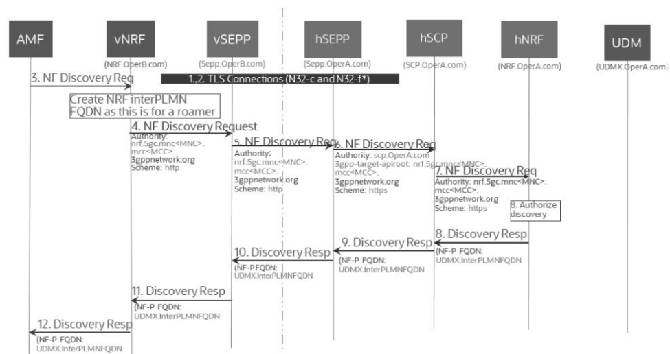
Figure 3-49 SEPP sets the 3GPP-SBI-Target-Apiroot header
