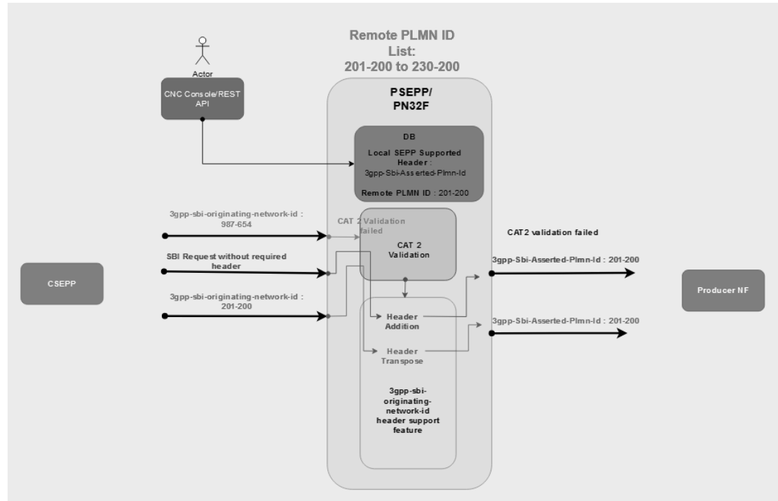
Figure 3-24 P SEPP side functionality
