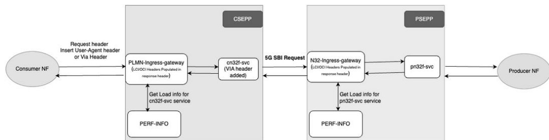
Figure 3-8 Architecture
