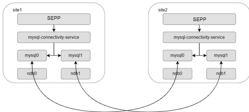
Figure 3-65 Two-Site Georedundancy
