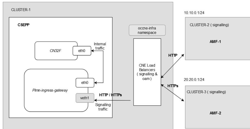
Figure 3-21 Ingress Traffic Segregation
