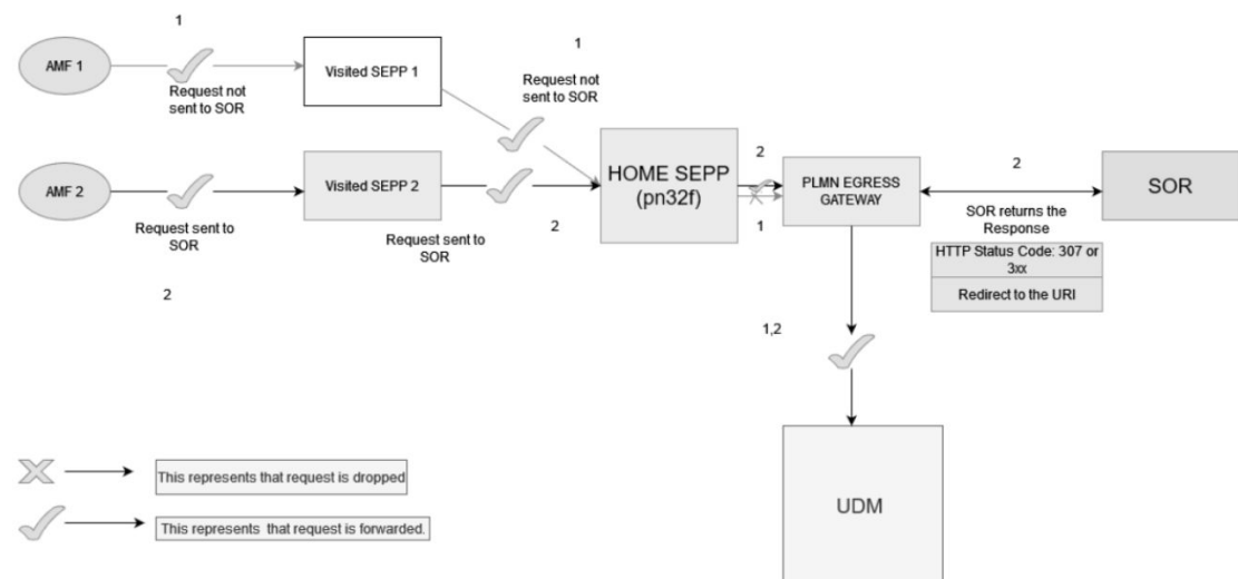
Figure 3-61 Redirection Enabled Mode
