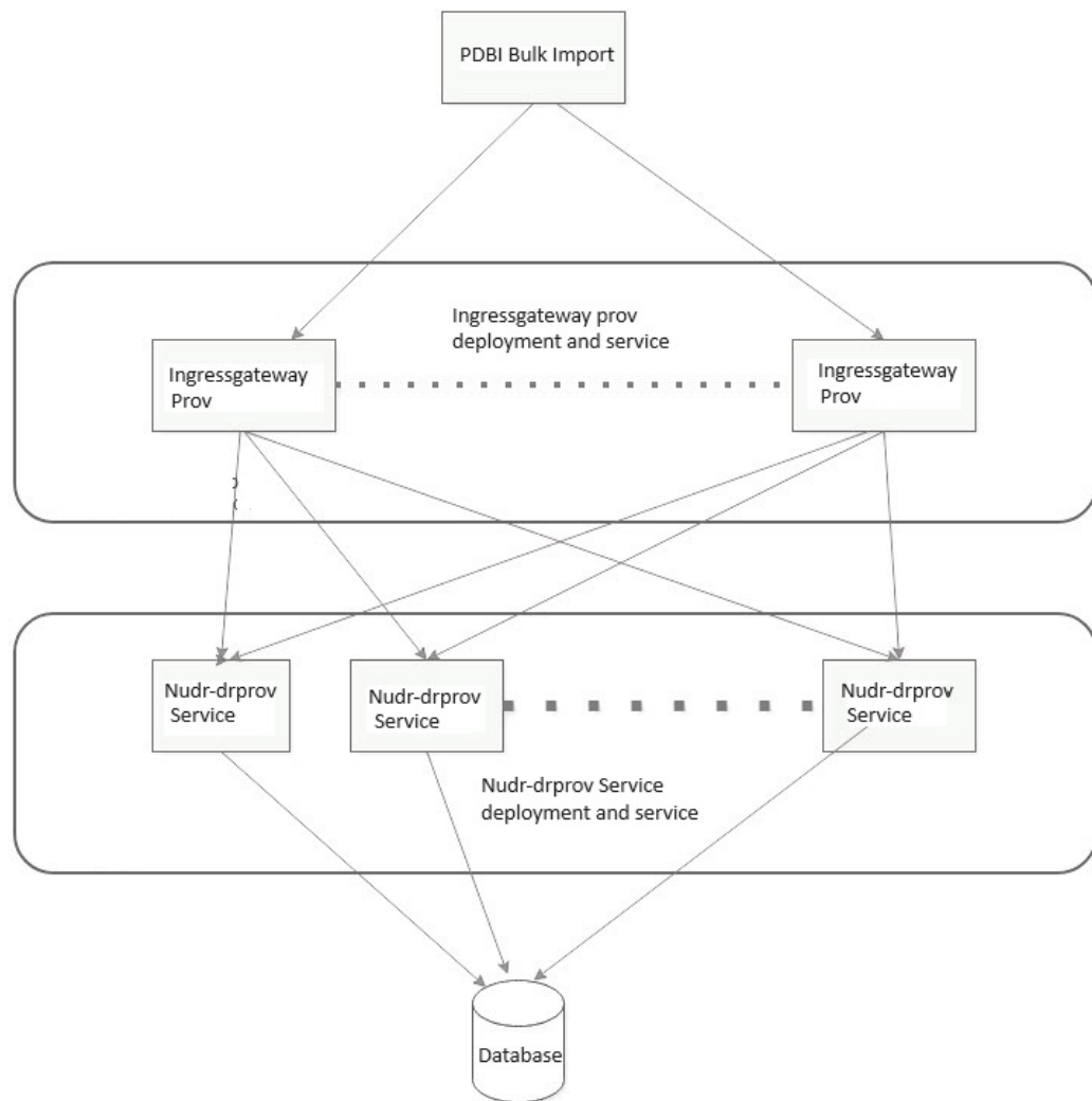
Figure 2-22 Equipment Data Provisioning
