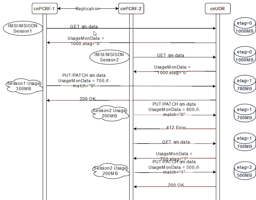
Figure 2-15 ETag in HTTP response
