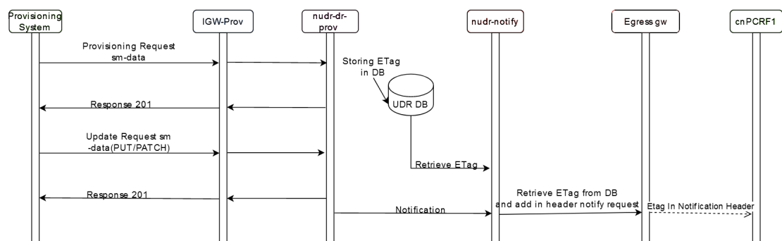
Figure 2-16 Etag Notifications for Provisioning Requests
