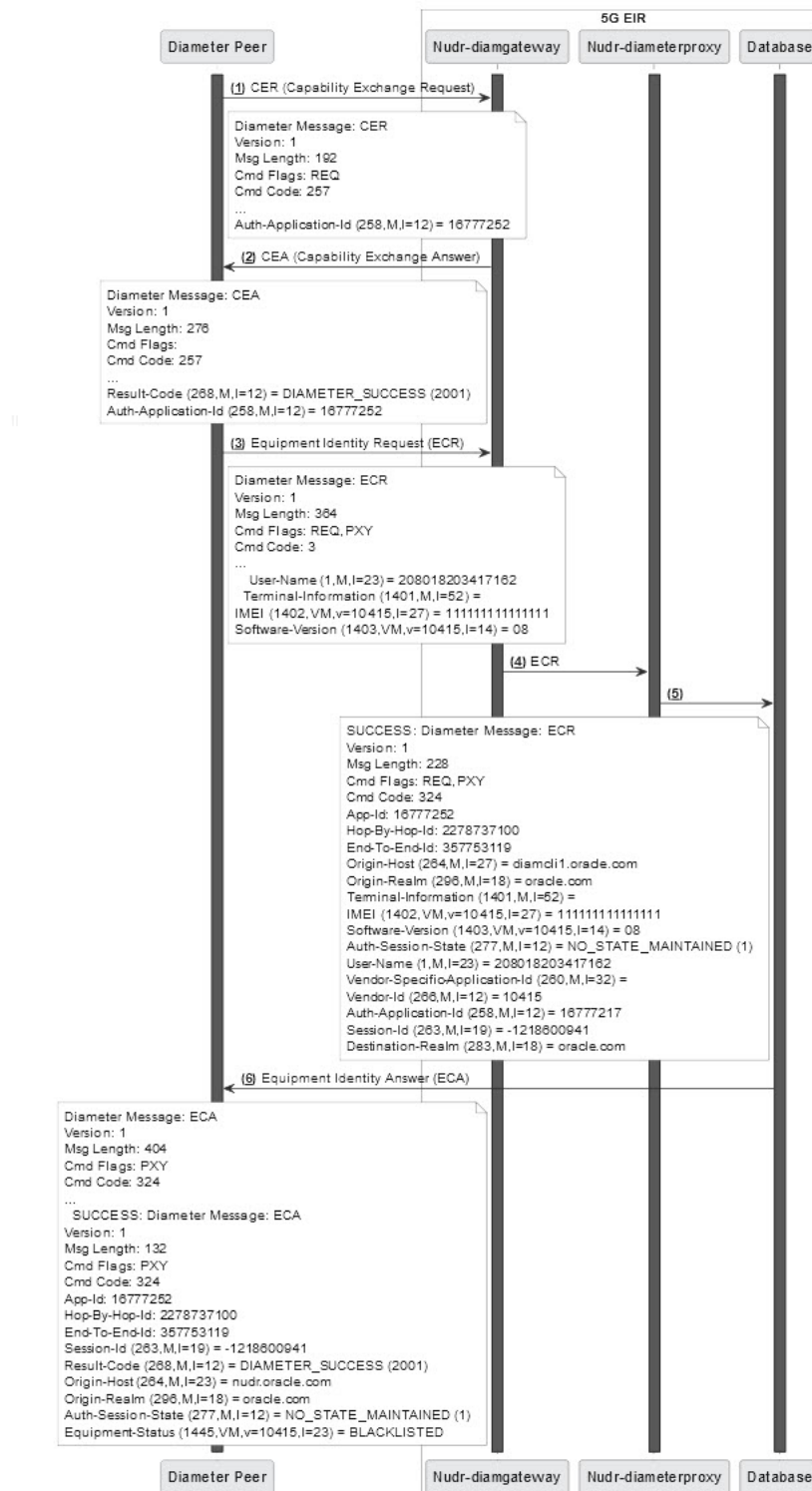
Figure 2-24 ECR Request
