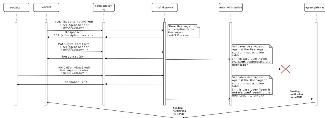
Figure 2-3 Signaling Requests
