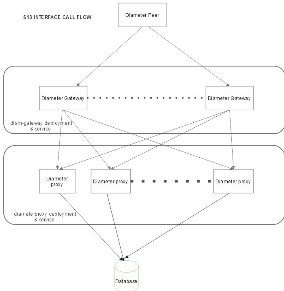
Figure 2-23 Diameter S13 Interface Call Flow
