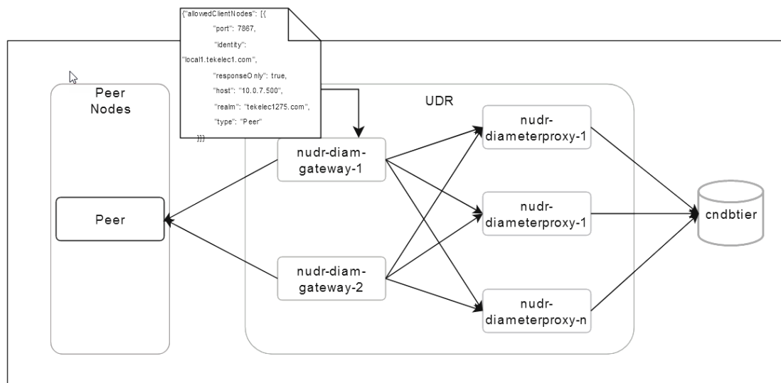
Figure 2-6 Diameter Connection Configuration
