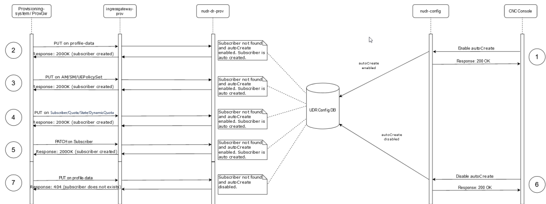
Figure 2-14 Auto Create
