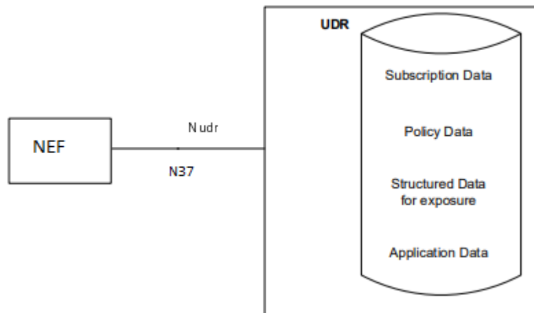
Figure 2-26 NEF Integration
