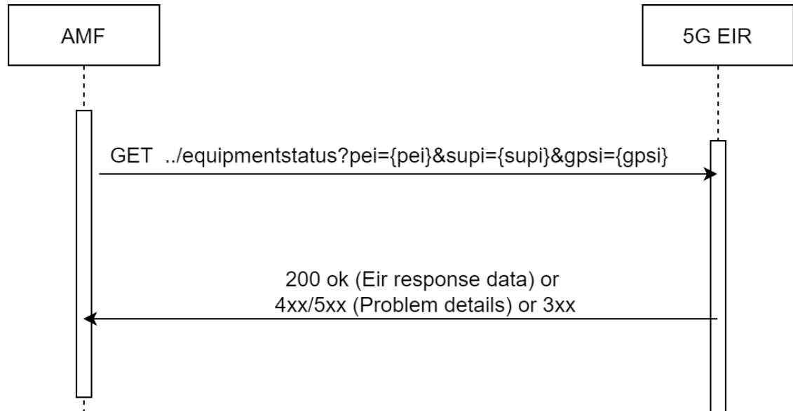
Figure 2-21 Reference Model – 5G-EIR
