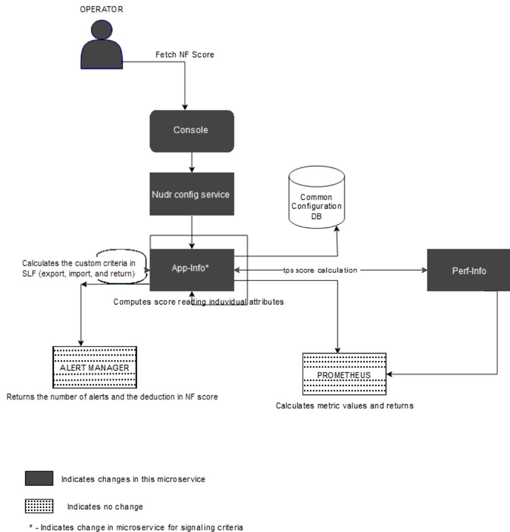
Figure 2-8 NF Scoring
