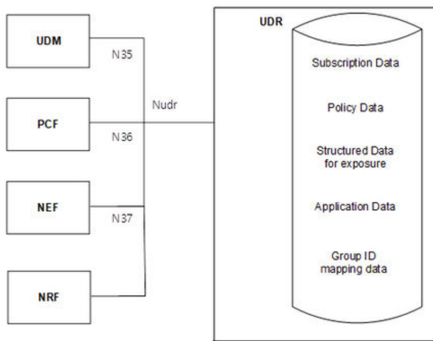
Figure 2-11 Data Storage Architecture
