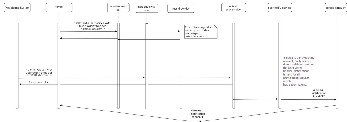
Figure 2-4 Provisioning Requests
