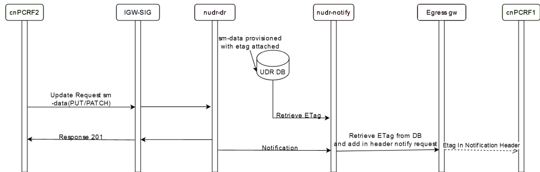
Figure 2-17 Notification for Signaling Requests
