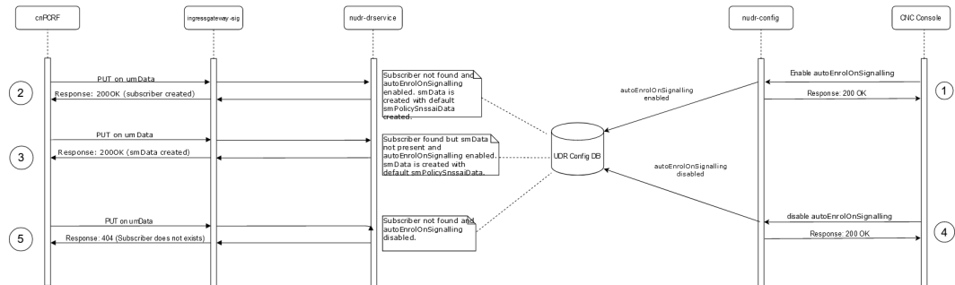
Figure 2-13 PUT operation for Auto Enrollment
