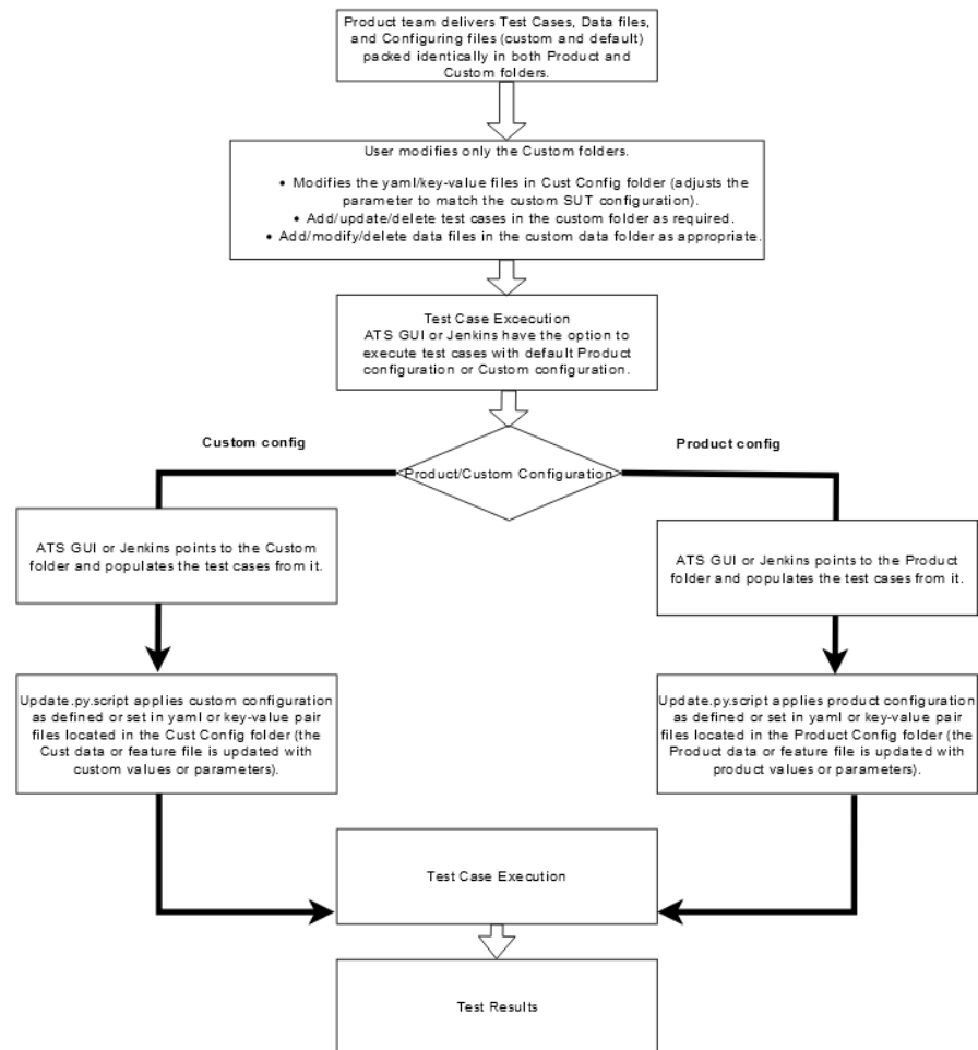
Figure 2-70 ATS Execution Flow
