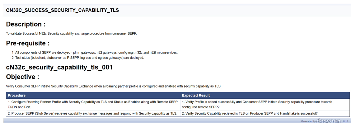
Figure 4-57 CN32C_SUCCESS_SECURITY_CAPABILITY_TLS
