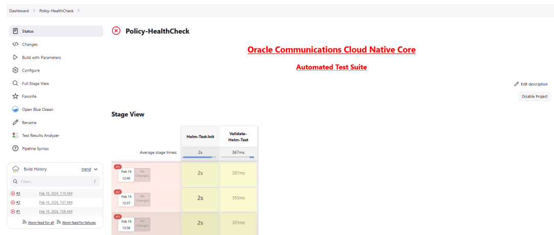
Figure 2-30 Configure Healthcheck
