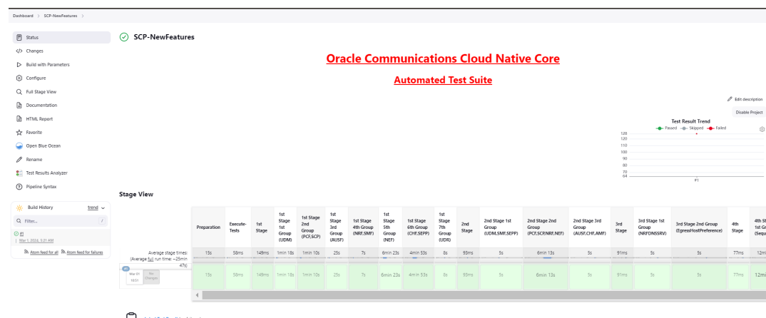
Figure 4-35 SCP-NewFeatures
