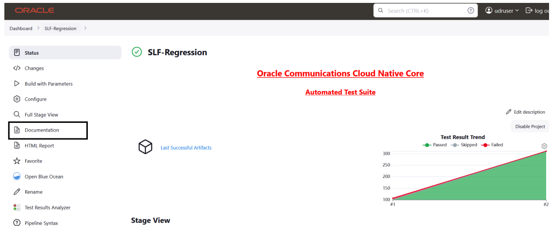
Figure 4-83 SLF-Regression Documentation
