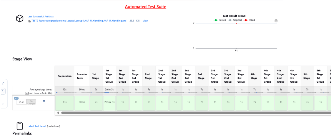
Figure 4-12 BSF_Regression Pipeline
