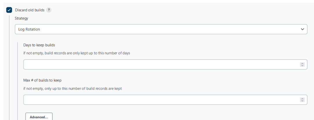
Figure 4-108 Discard Builds
