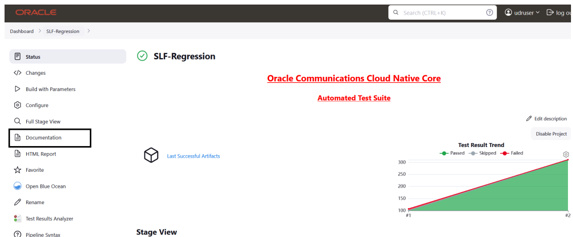
Figure 4-84 SLF-Regression Documentation
