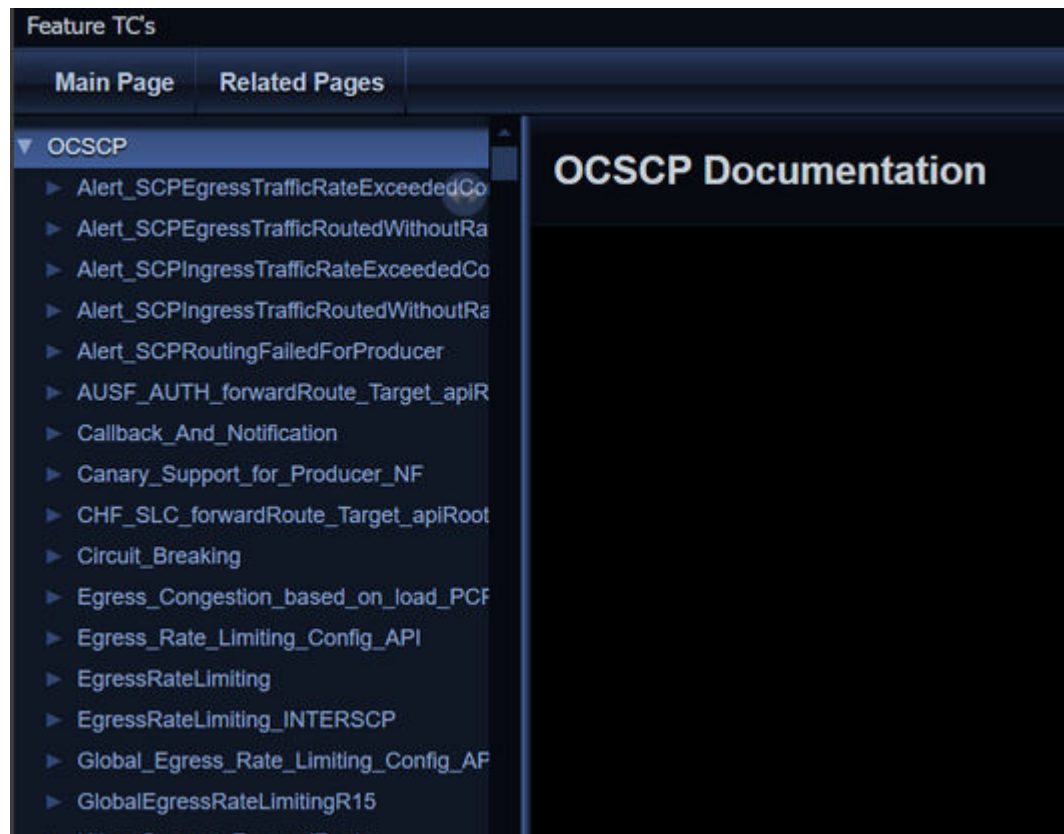
Figure 4-39 SCP-NewFeatures Documentation
