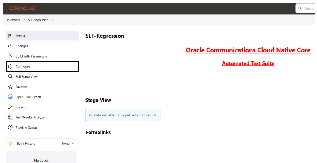
Figure 4-70 SLF-Regression Pipeline
