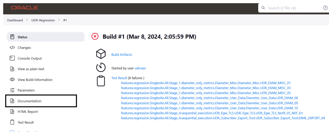
Figure 4-102 UDR-Regression Documentation
