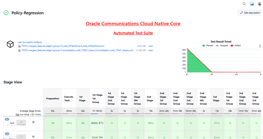
Figure 4-28 Regression Pipeline
