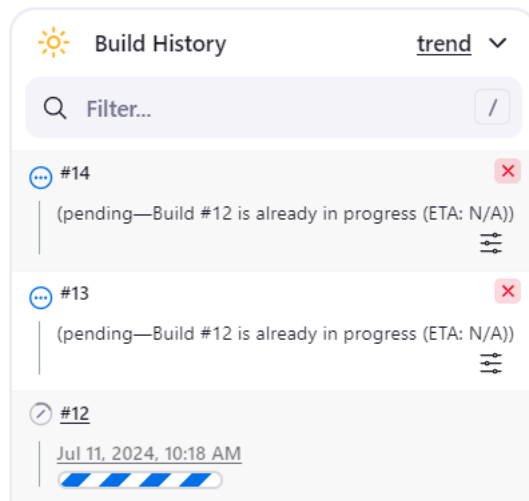
Figure 2-10 Stopping Builds
