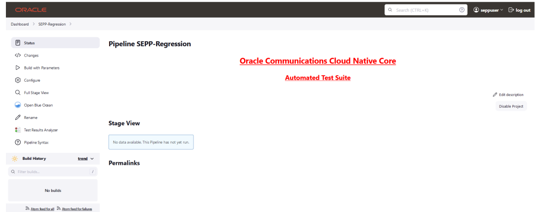
Figure 4-54 SEPP Regression
