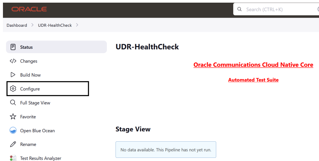
Figure 4-97 UDR-HealthCheck Pipeline
