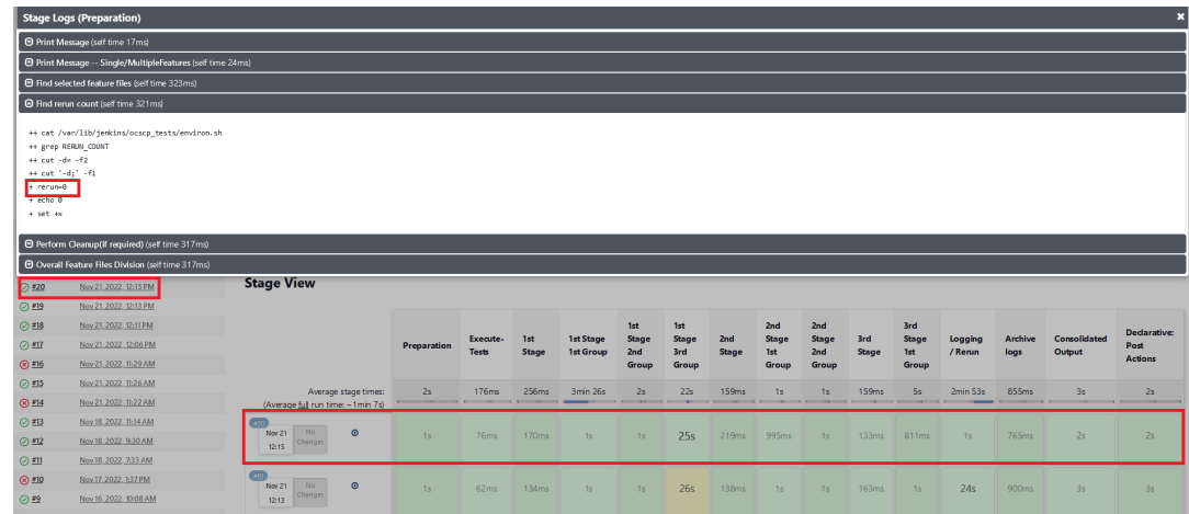
Figure 2-47 Test Cases Fail on the Initial Run but Pass in the Rerun
