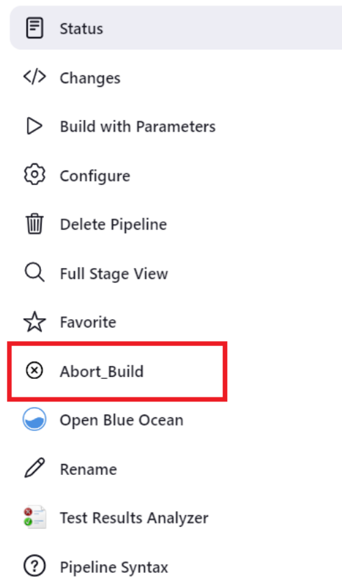
Figure 2-11 Abort Build
