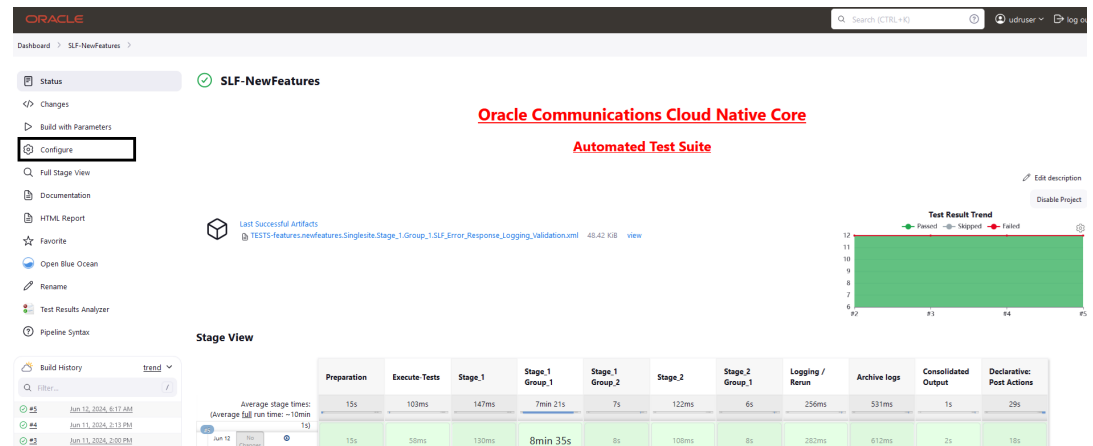
Figure 4-65 SLF-NewFeatures Configure
