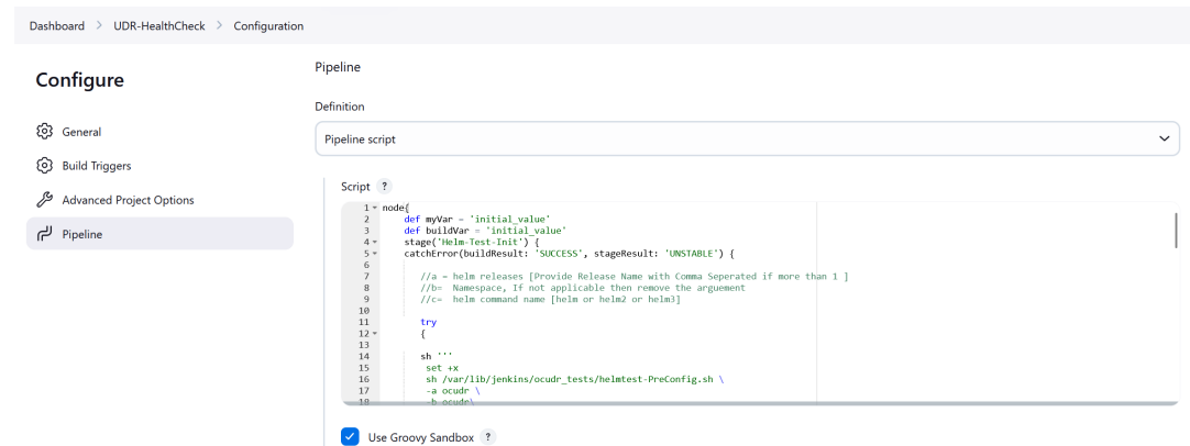
Figure 4-98 UDR-HealthCheck Configuration
