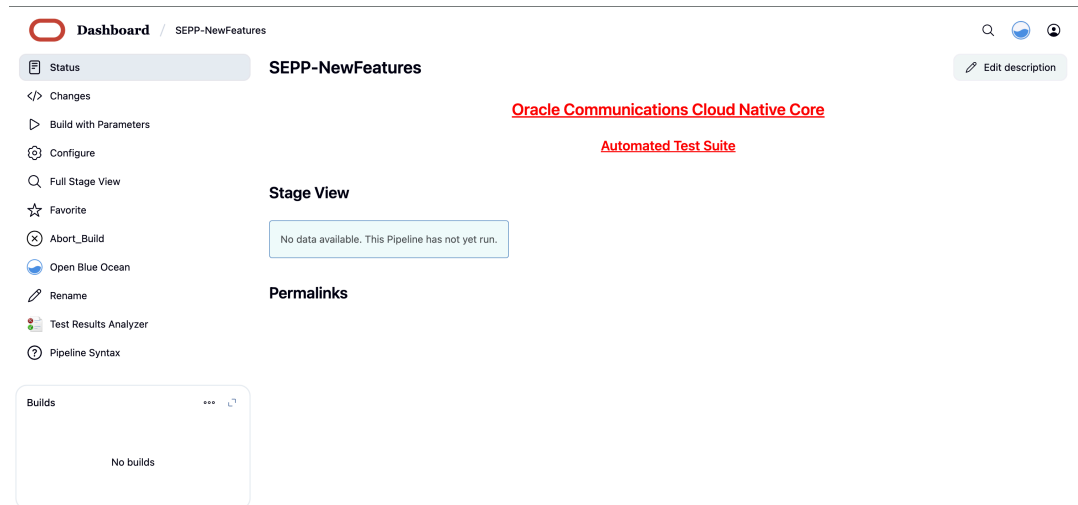
Figure 4-48 SEPP-NewFeatures Pipeline
