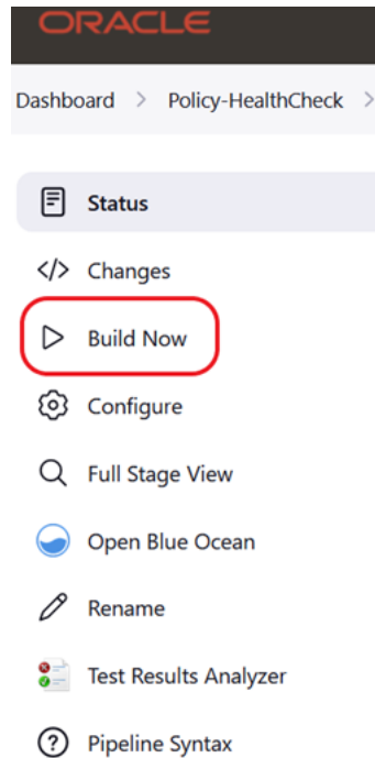
Figure 2-32 Build Now
