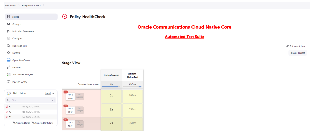
Figure 2-33 Configure Healthcheck
