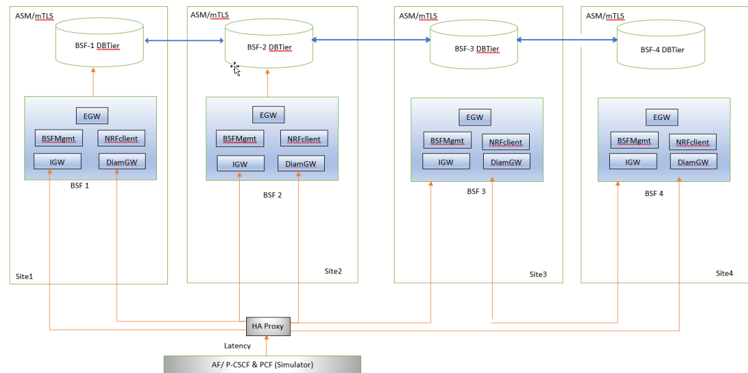
Figure 3-8 ASM Enabled Four-site Georedundant Setup
