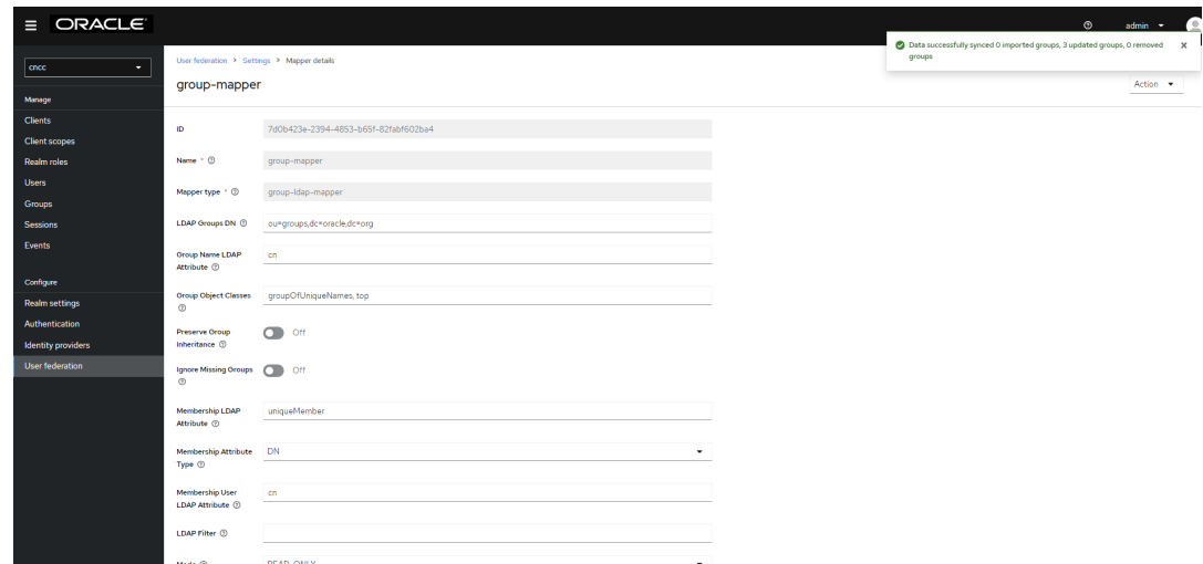
Figure 4-58 Group Mapper
