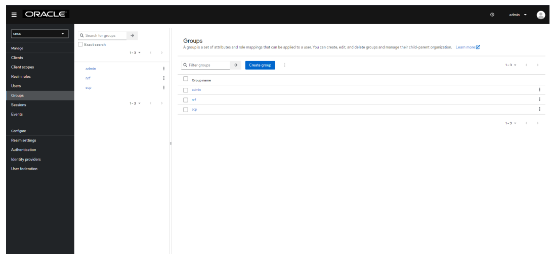
Figure 4-59 Groups
