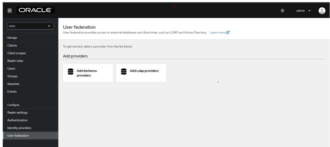
Figure 4-47 User Federation
