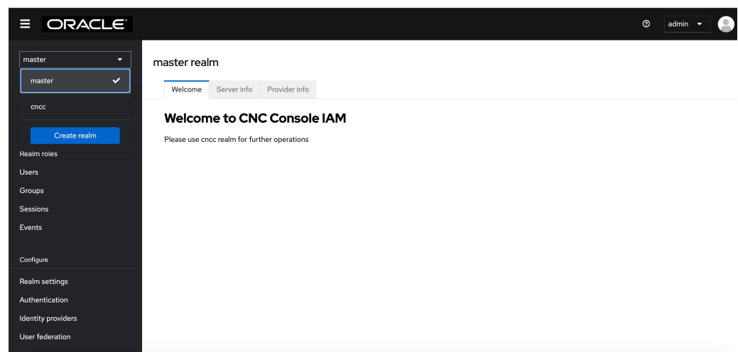
Figure 4-19 default realm
