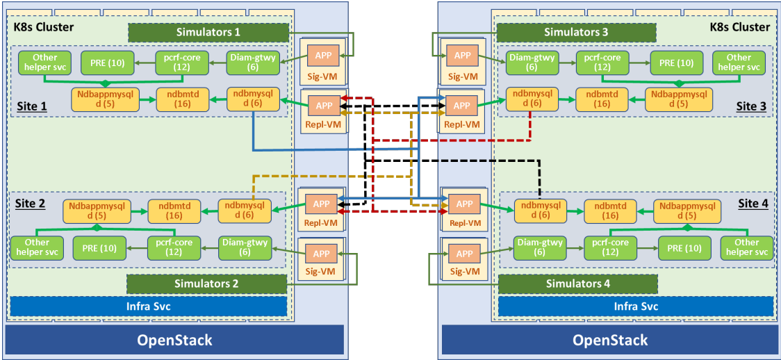
Figure 2-3 Policy Deployment in Four-Site GR Setup
