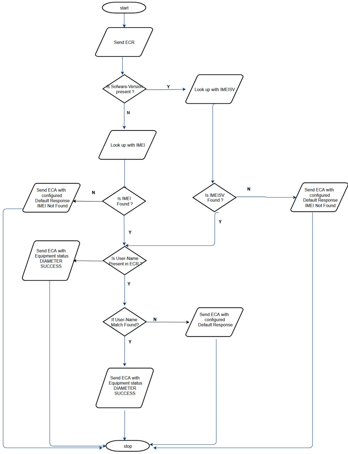
Figure 2-26 Equipment Status Retrieval Call Flow
