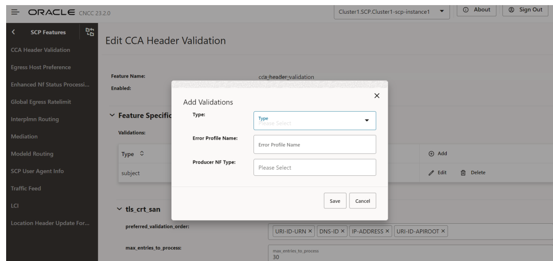
Figure 4-17 Add Validations
