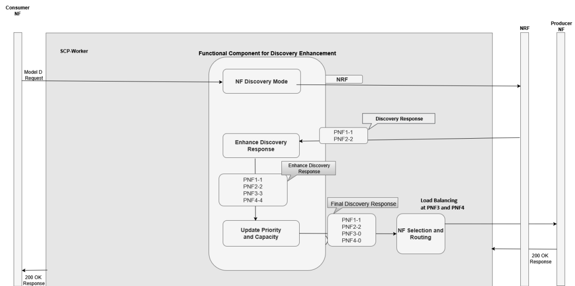
Figure 3-14 Processing a Model D Discovery Request When the Discovery Mode is NRF
