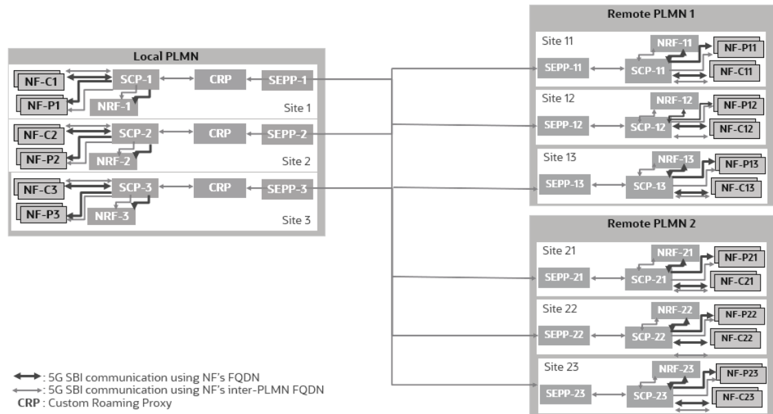
Figure 3-16 Custom Roaming Proxy
