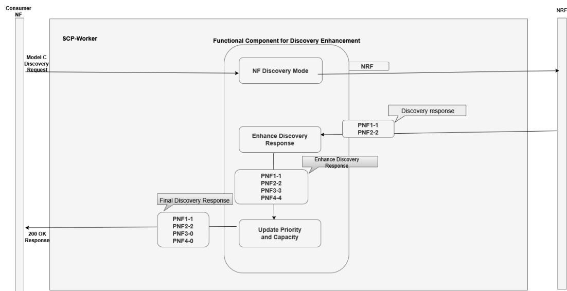
Figure 3-13 Processing a Model C Discovery Request When the Discovery Mode is NRF
