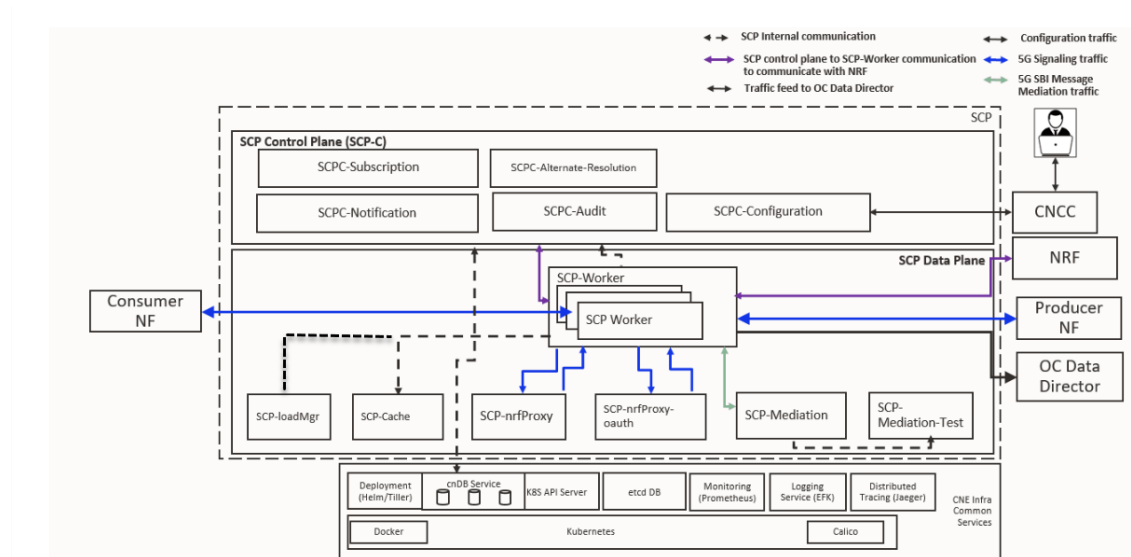
Figure 2-1 Service Communication Proxy Architecture
