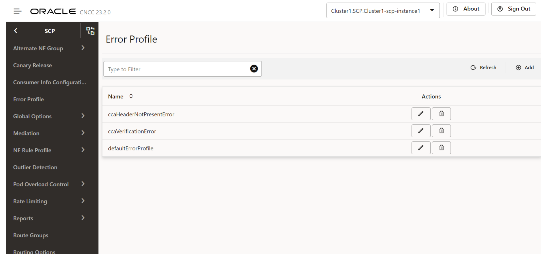
Figure 4-34 Error Profile
