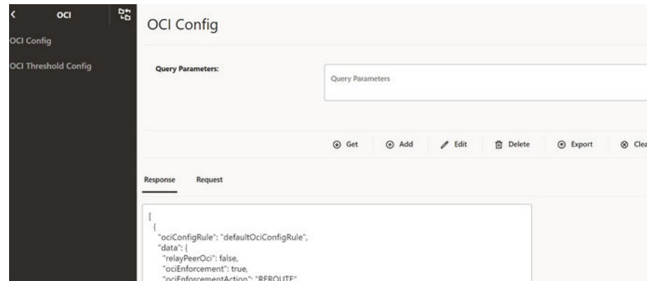
Figure 4-26 OCI Config
