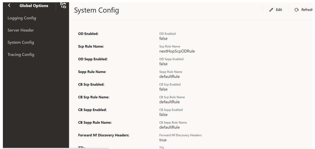
Figure 4-41 System Config
