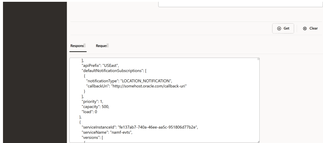
Figure 4-55 Response data
