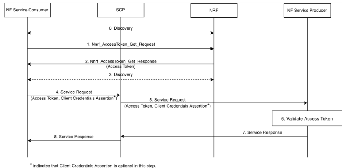
Figure 3-6 NF Consumer Obtains Access Tokens from NRF
