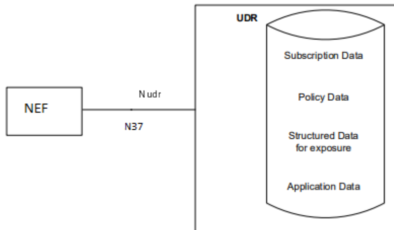
Figure 2-29 NEF Integration
