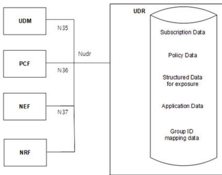
Figure 2-13 Data Storage Architecture
