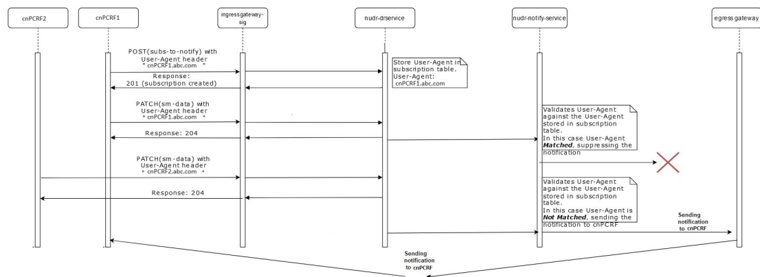
Figure 2-5 Signaling Requests
