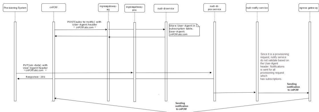
Figure 2-6 Provisioning Requests
