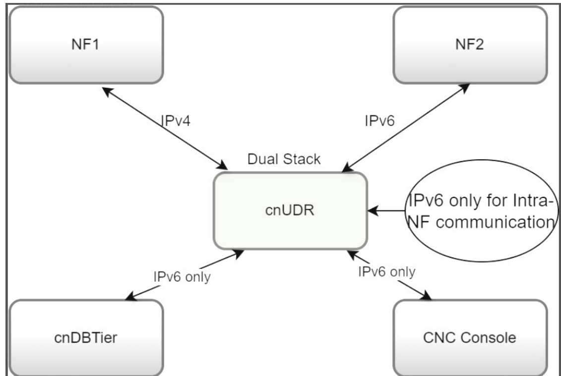
Figure 2-4 Dual Stack
