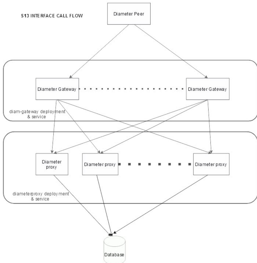
Figure 2-25 Diameter S13 Interface Call Flow
