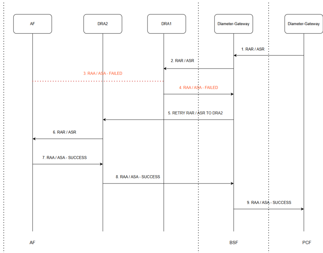
Figure 3-17 RX-RAR / RX-ASR Retry - Success Case
