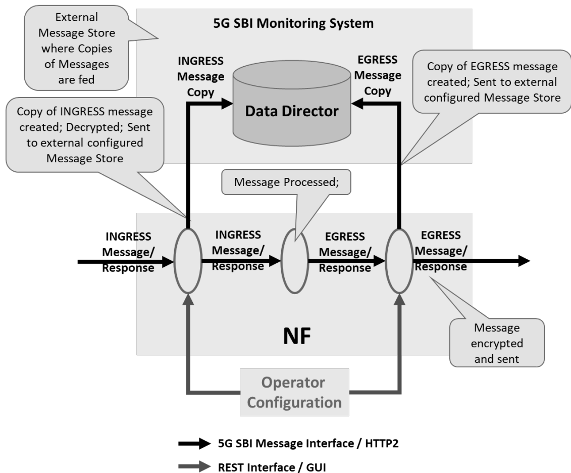
Figure 3-52 BSF Message Feed Architecture
