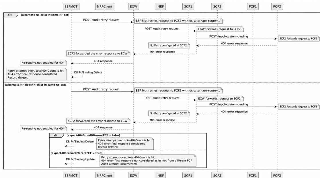
Figure 3-41 BSF Audit Retry Flow with Alternate NF Selection and 404 Error Handling
