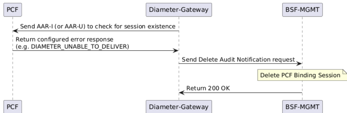
Figure 3-38 Stale Session Notification from Diameter Gateway
