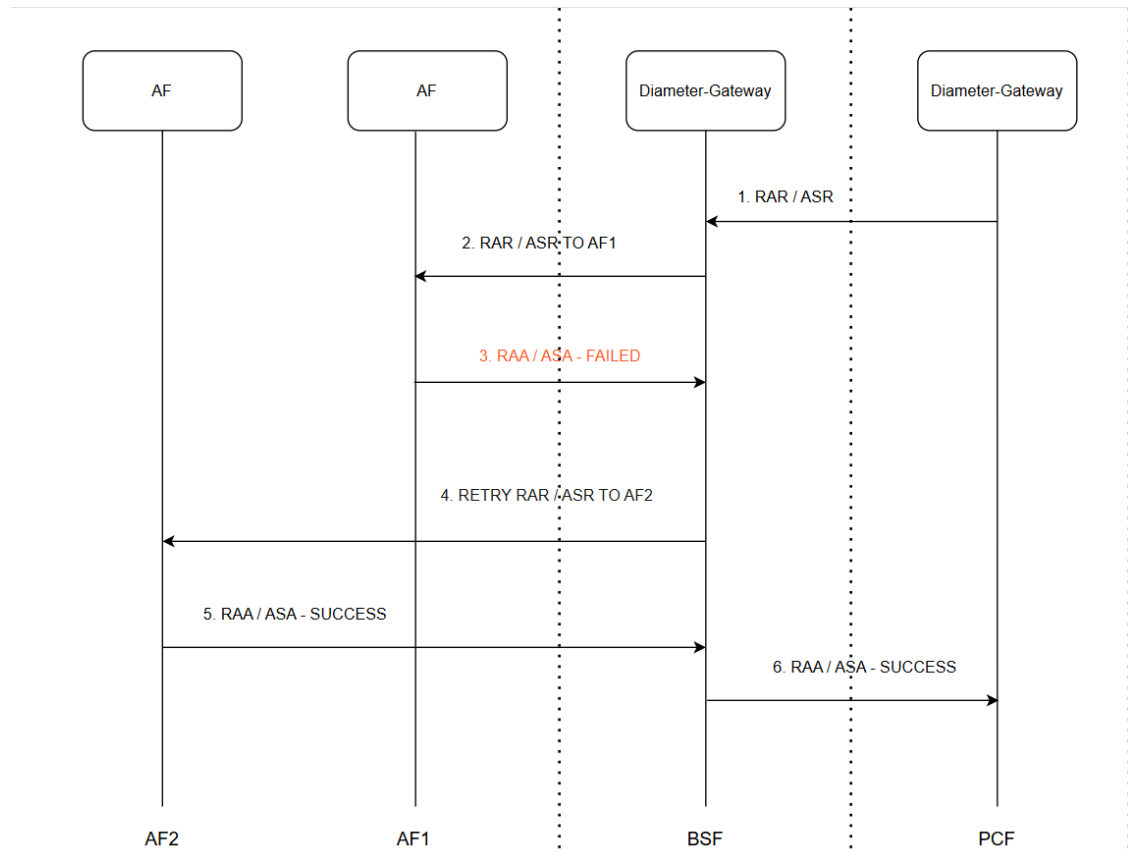
Figure 3-20 RX-RAR / RX-ASR Retry without FQDN Peers - BSF Directly Connected to AFs
