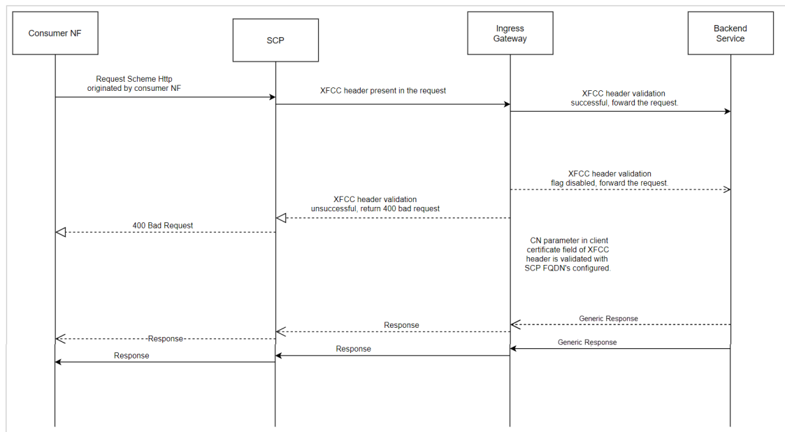
Figure 3-27 Call Flow Validation of Single XFCC Header
