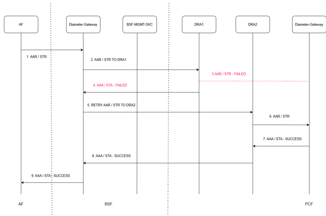
Figure 3-14 RX-AAR / RX-STR Retry - Success Case
