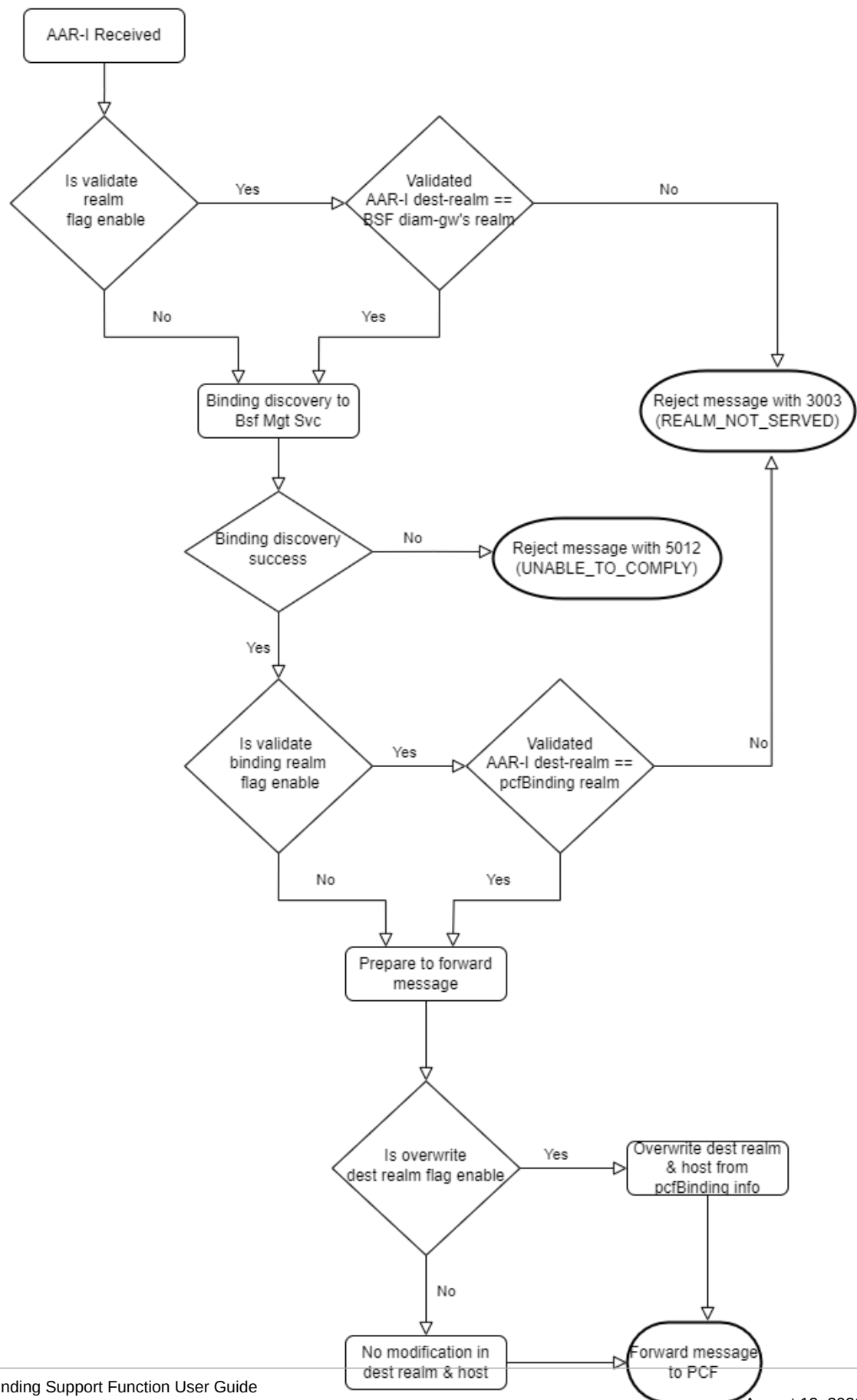
Figure 3-9 destination-realm Validation Process
