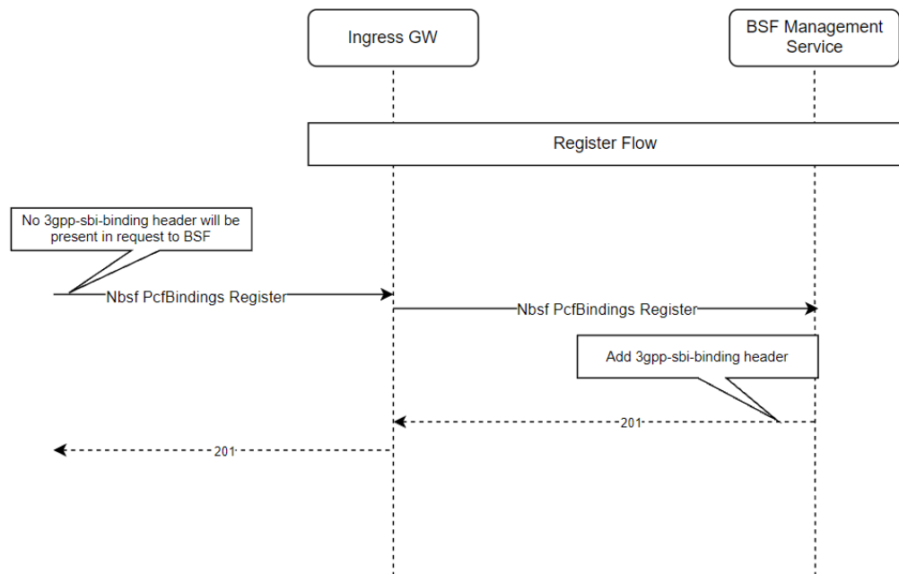
Figure 3-45 Example of NF Set and Binding Header in BSF
