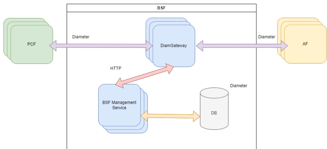
Figure 3-8 Diameter Gateway for BSF
