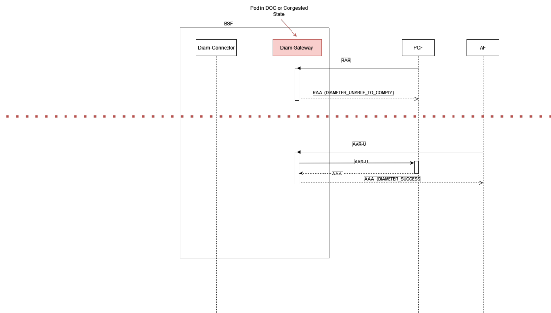
Figure 3-33 Call flow diagram for Diameter Congestion Control
