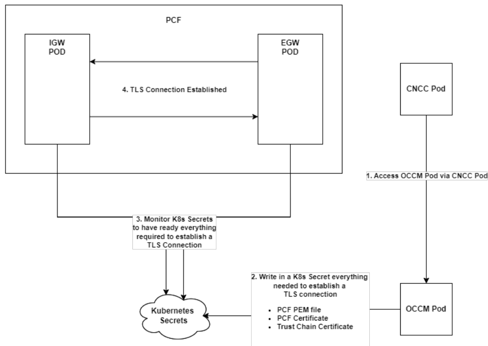
Figure 3-10 BSF Integration with OCCM
