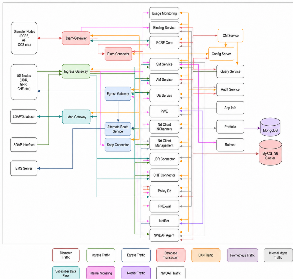
Figure 2-1 Architecture of Binding Support Function
