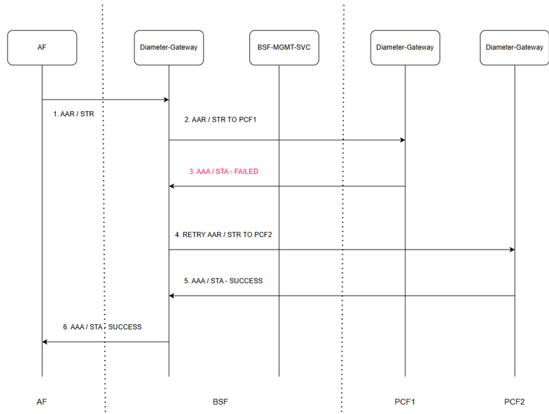
Figure 3-19 RX-AAR / RX-STR Retry without FQDN Peers - BSF Directly Connected to PCFs
