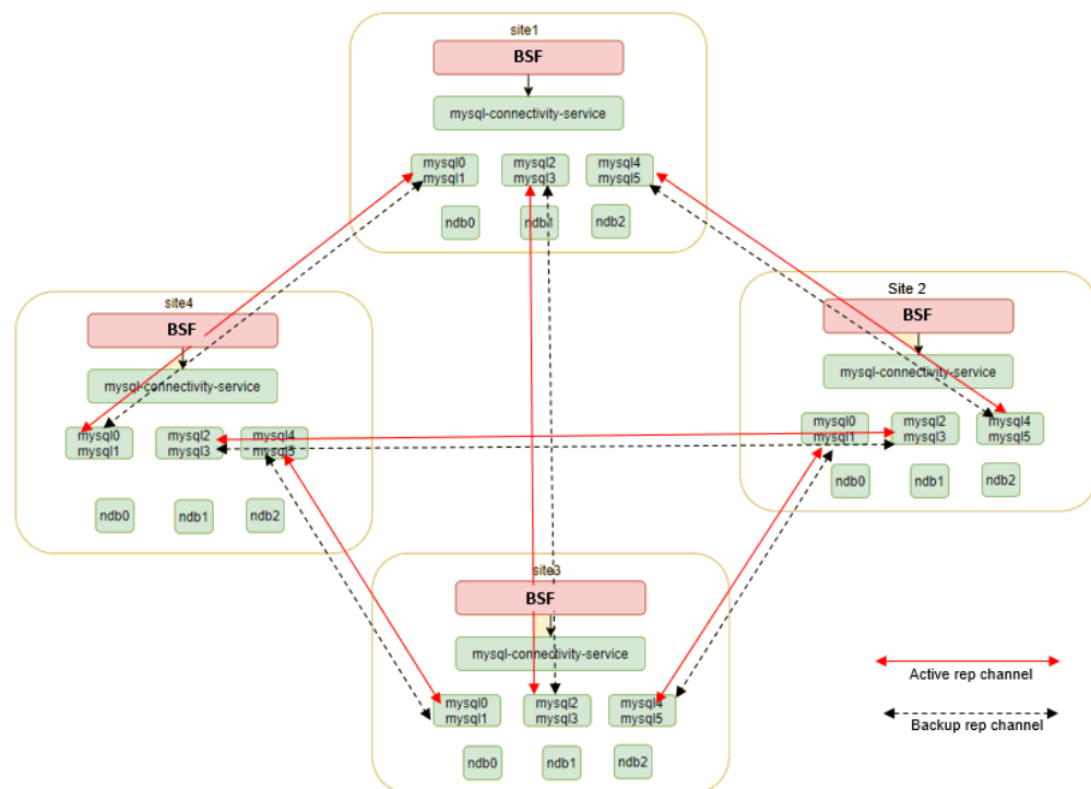
Figure 3-31 Four-Site Georedundancy Deployment
