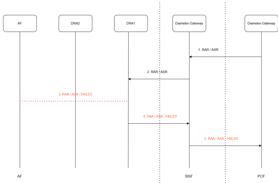
Figure 3-16 RX-RAR / RX-ASR Existing - Failed Case
