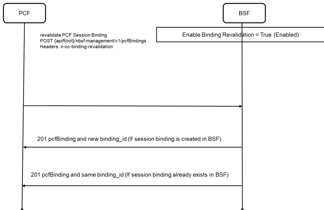
Figure 3-6 Binding revalidation in BSF
