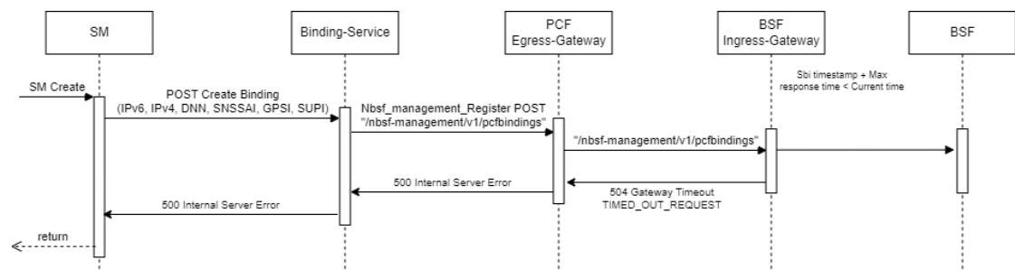
Figure 3-22 Request Timeout in BSF
