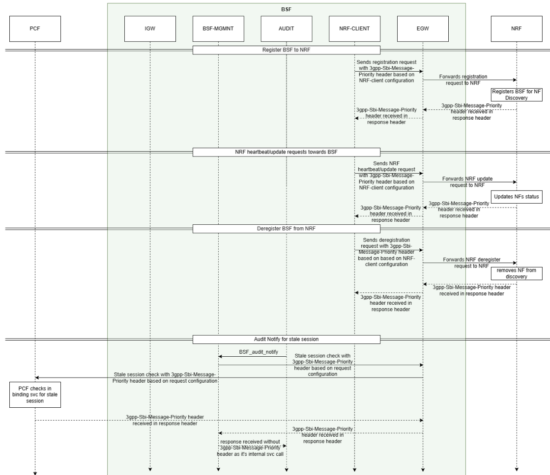
Figure 3-2 Sample call flow for session binding registration with BSF as a consumer
