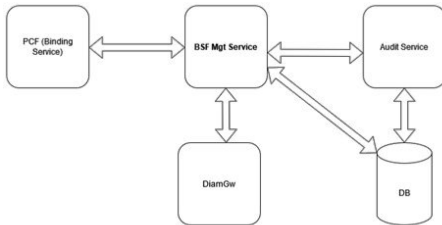
Figure 3-5 BSF Management Service interactions with other Services
