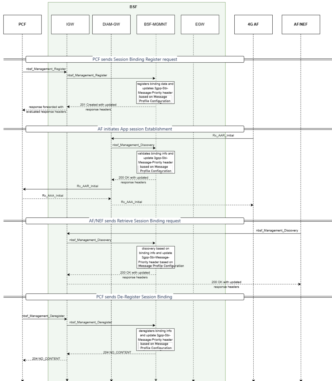
Figure 3-1 Sample call flow for session binding registration with BSF as a producer
