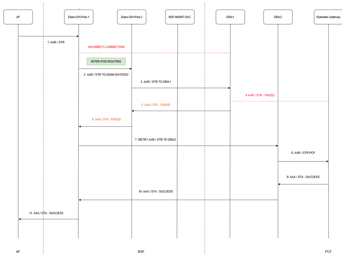
Figure 3-15 RX-AAR / RX-STR Retry - Inter-Pod Routing Case
