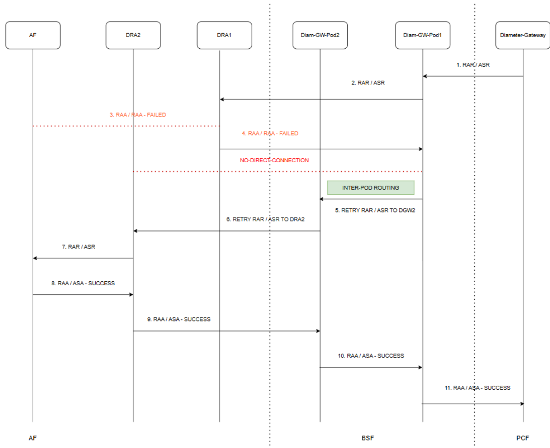
Figure 3-18 RX-RAR / RX-ASR Retry - Inter-Pod Routing Case
