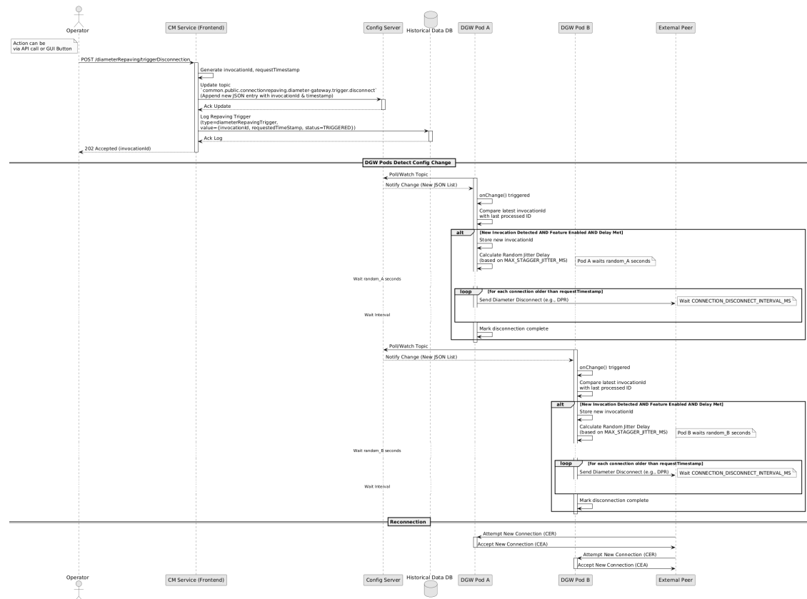
Figure 3-53 Diameter Gateway Connection Termination
