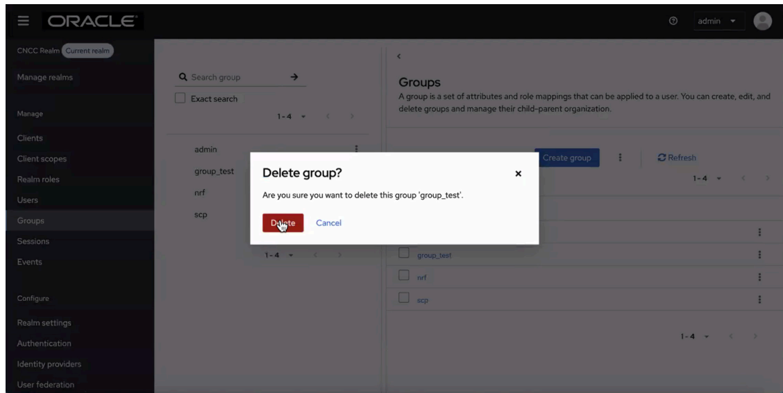
Figure 11 Delete group
