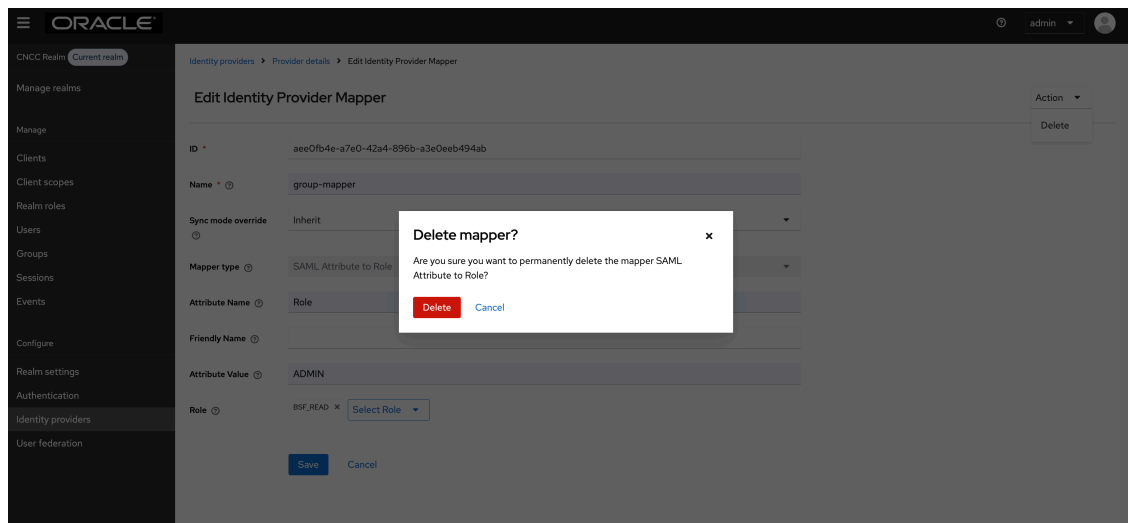
Figure 24 Delete Mapper
