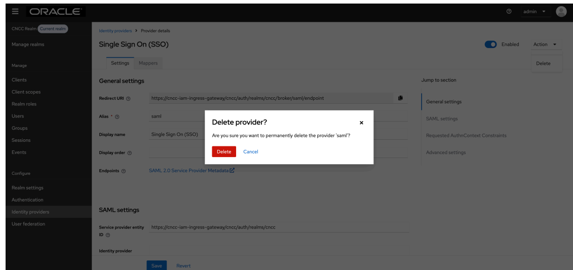
Figure 20 Delete provider
