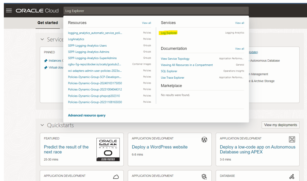
Figure 2-2 Log Explorer
