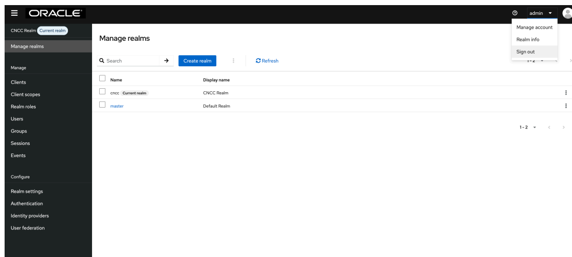
Figure 25 Sign out
