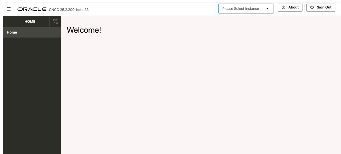
Figure 26 Sign Out
