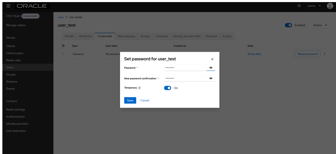
Figure 15 Set Password
