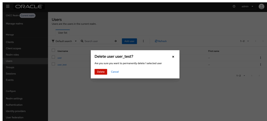
Figure 7 Delete user
