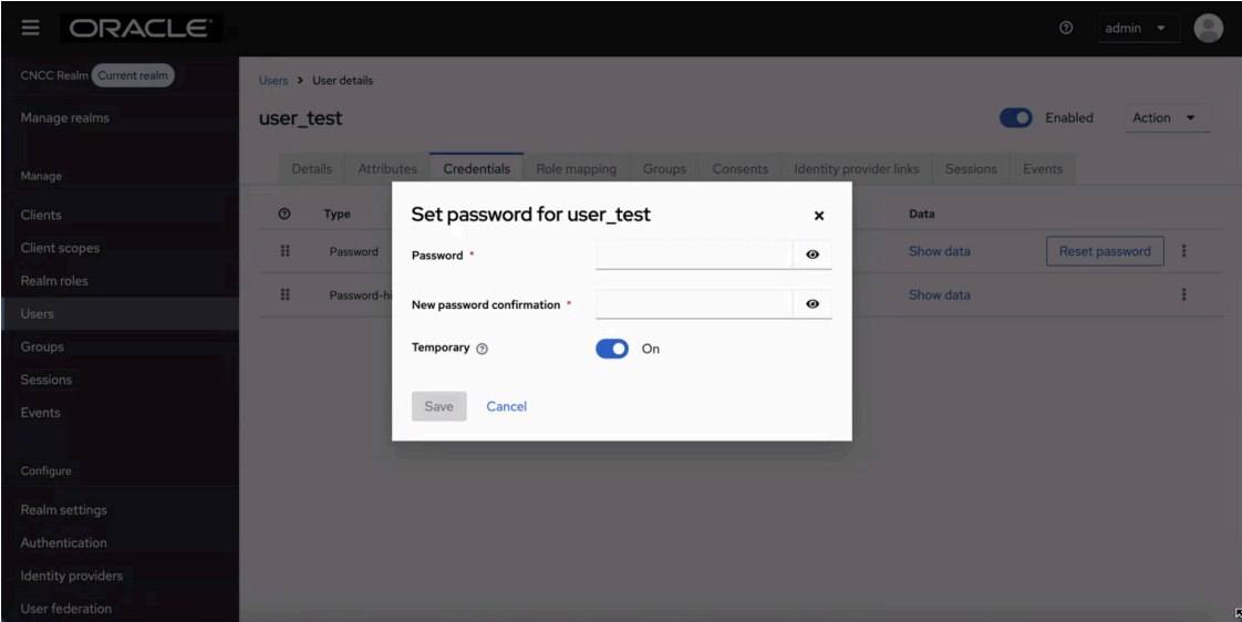
Figure 13 Set Password
