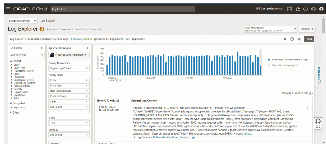
Figure 2-4 View Logs
