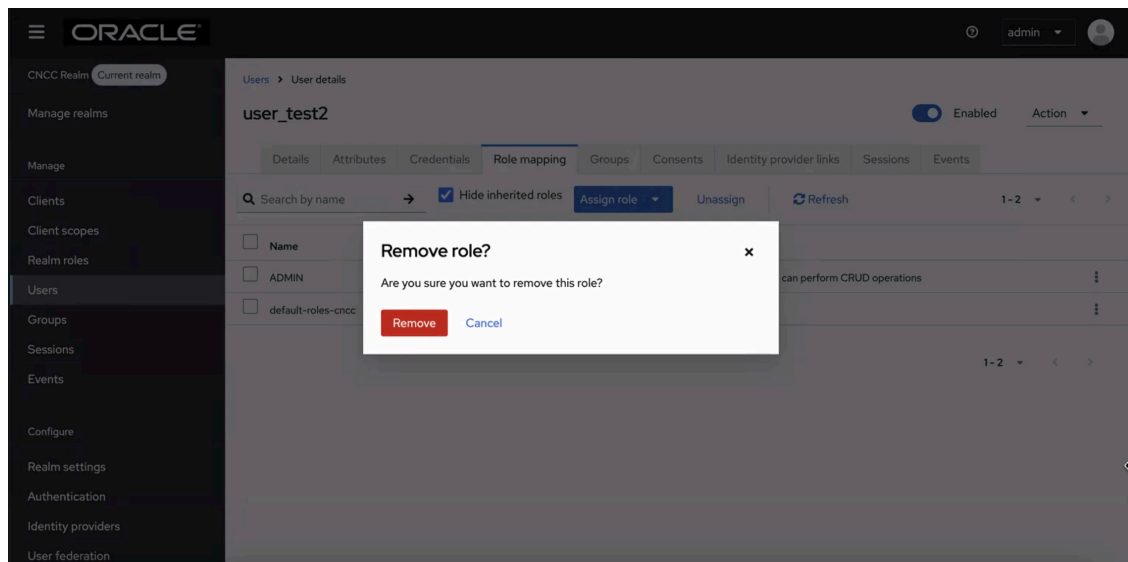
Figure 9 Remove role
