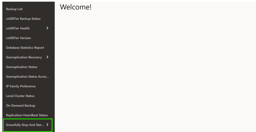
Figure 6-1 Start Georeplication
