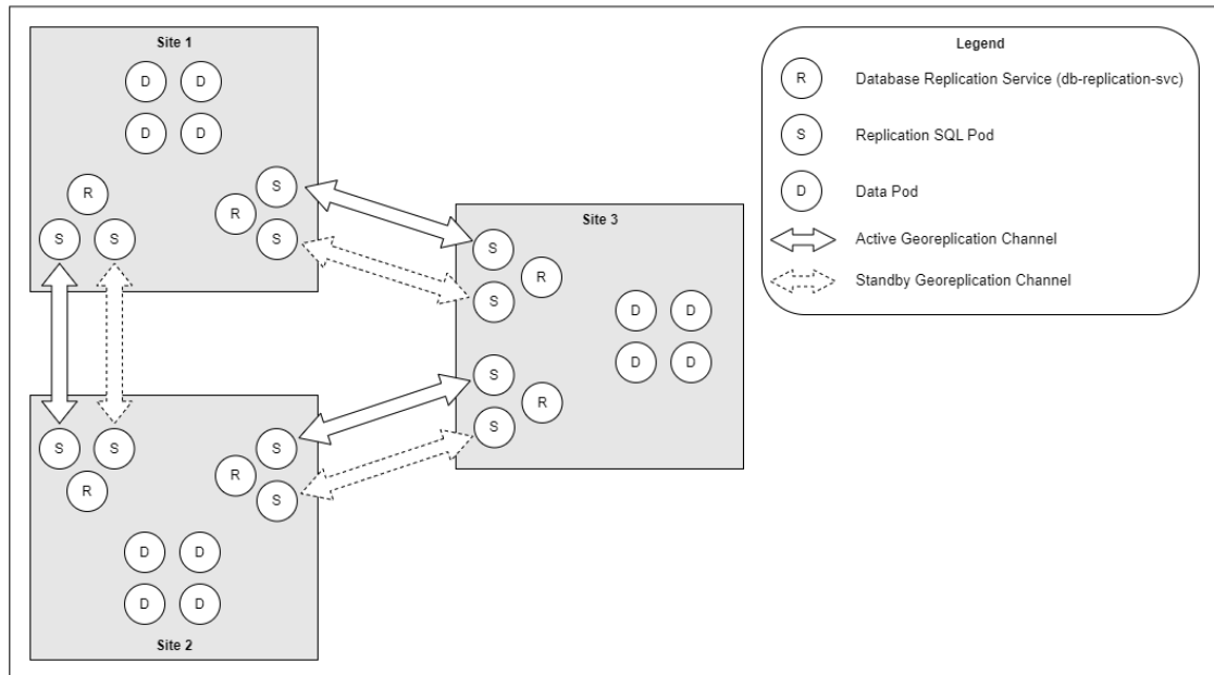
Figure 2-4 Three-Site Replication
