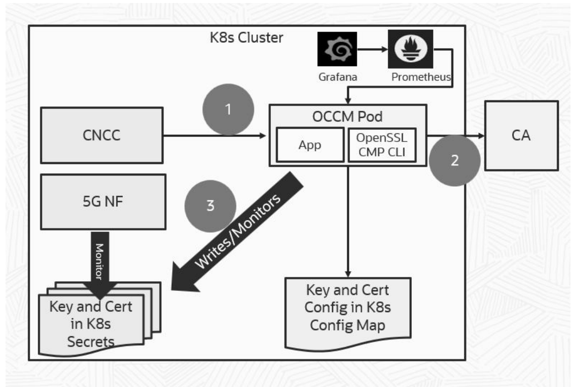
Figure 2-1 OCCM Architecture
