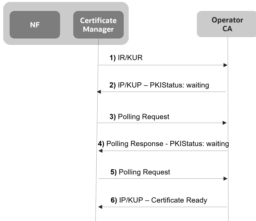
Figure 3-61 Polling for Certificates
