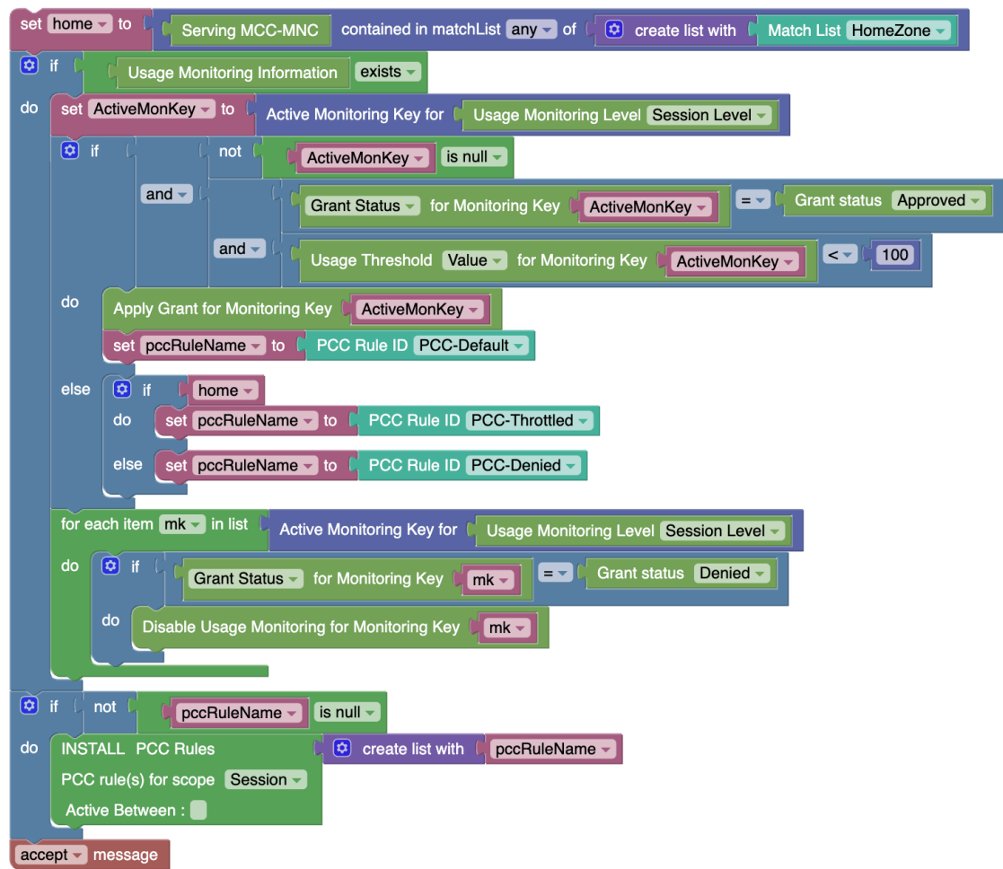
Figure 4-49 PCRF Core Project for Home Monthly Plan with Top-ups
