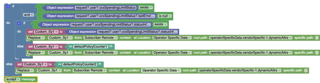
Figure 4-13 Blockly to Use Remote Subscriber State Variables to write OSD PATCH to UDR from OCS data
