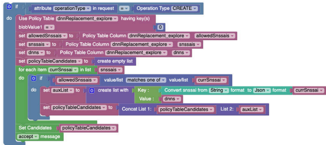
Figure 4-22 Example1: DNN Replacement using Policy Tables
