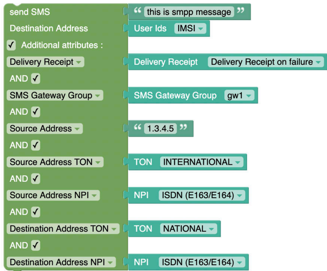
Figure 4-29 Sample Send SMS blockly configuration
