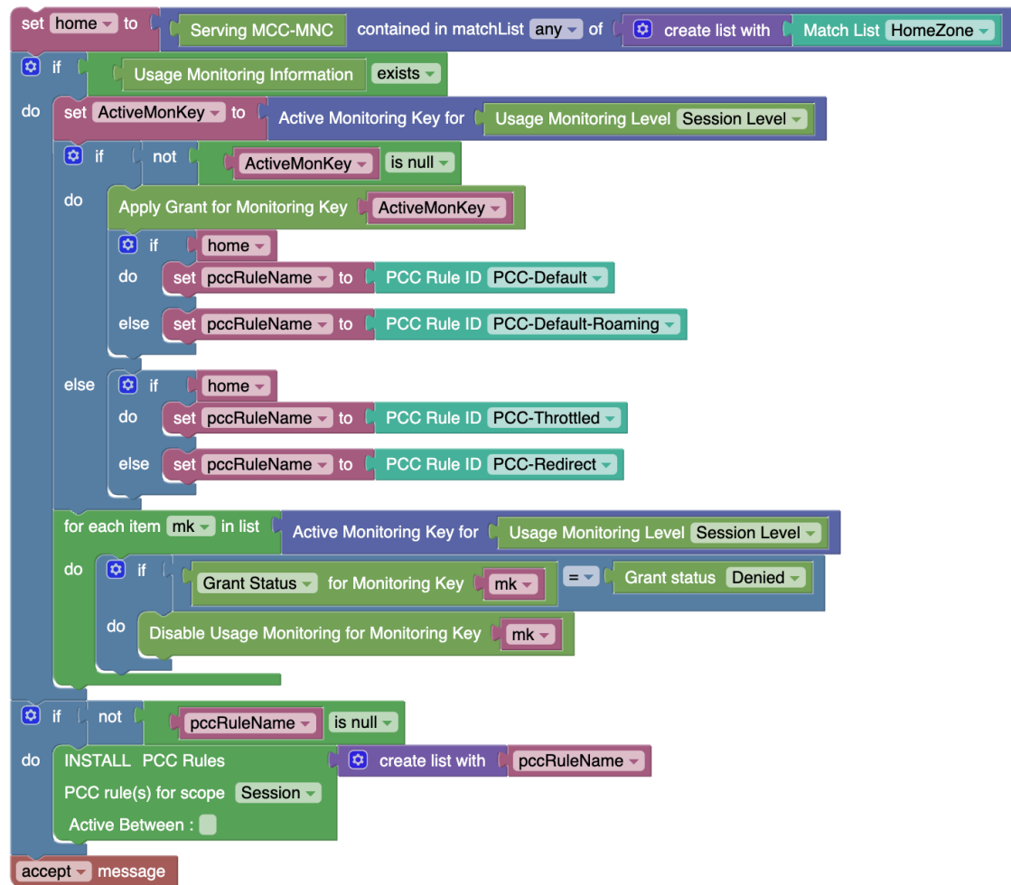
Figure 4-42 PCRF Core Project for Home Monthly Plan with Roaming Passes
