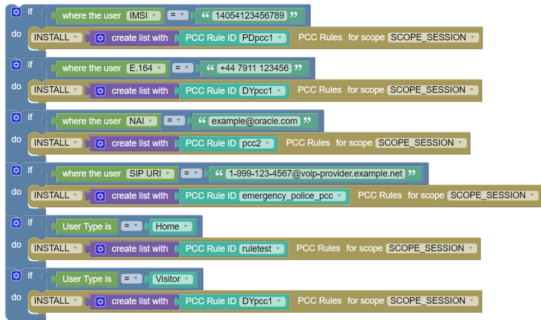
Figure 4-27 Use case for User specific conditions
