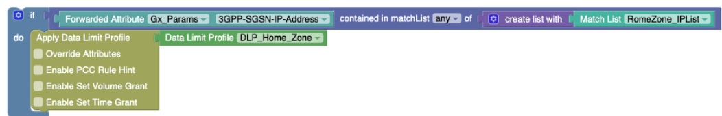
Figure 4-64 Example for IPV4 Data Type in Match List
