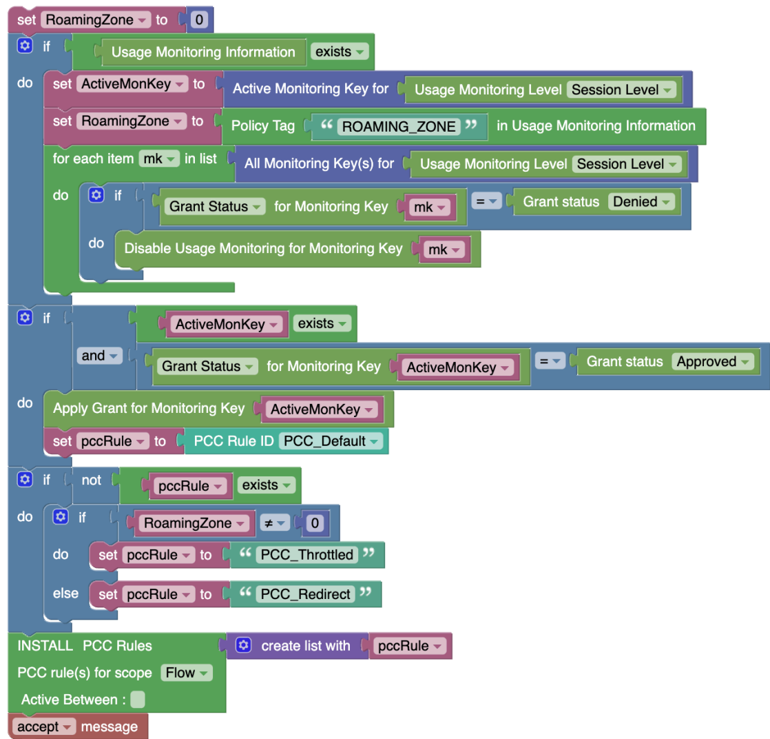
Figure 4-60 PCRF Core Project for Autoenrolled Roaming Subscriber with Multiple Roaming Passes
