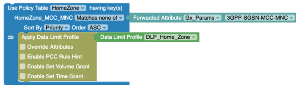
Figure 4-70 Example: Use Policy Table with Matches None Of option
