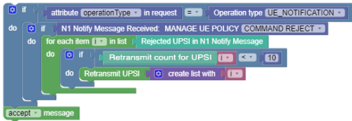
Figure 4-17 Use case scenario 4:
