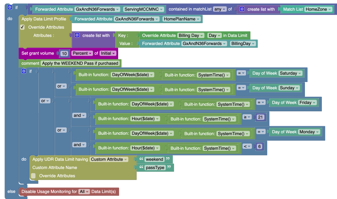
Figure 4-54 Policy Project for Home Monthly Plan with Weekend Passes
