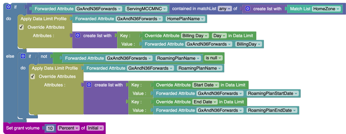
Figure 4-41 Policy Project for Home Monthly Plan with Roaming Passes
