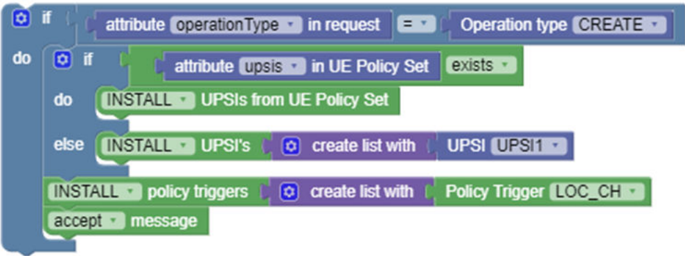
Figure 4-18 PCF UE use case
