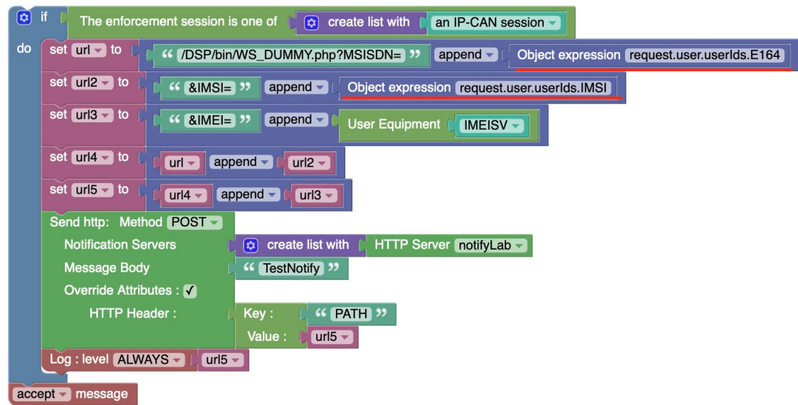
Figure 4-28 Configuring URI Based Parameters for Subscriber Notification
