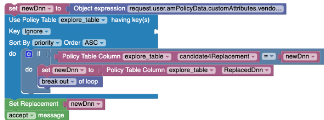
Figure 4-23 Example2: DNN Replacement
