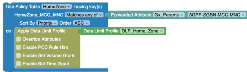
Figure 4-69 Example: Use Policy Table with Matches Any Of option
