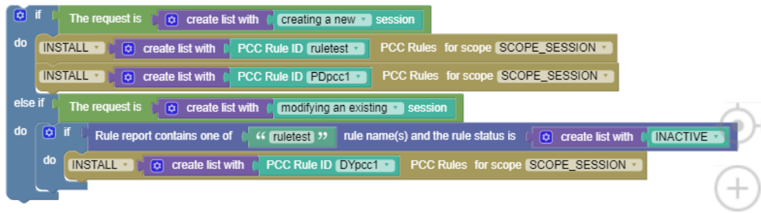
Figure 4-26 Use case for Rule Report Conditions
