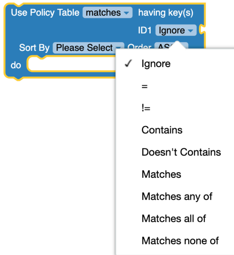
Figure 4-66 Exmple for Use Policy Table
