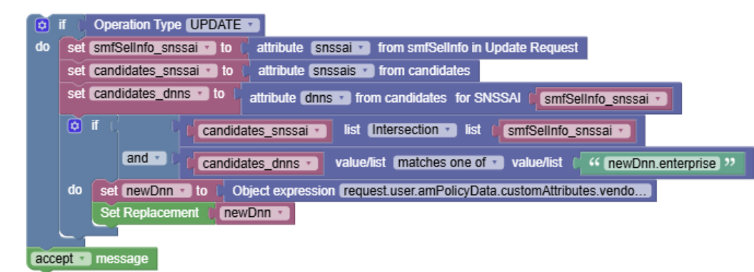
Figure 4-20 Using Intersection for Getting Allowed Candidates for Update Request
