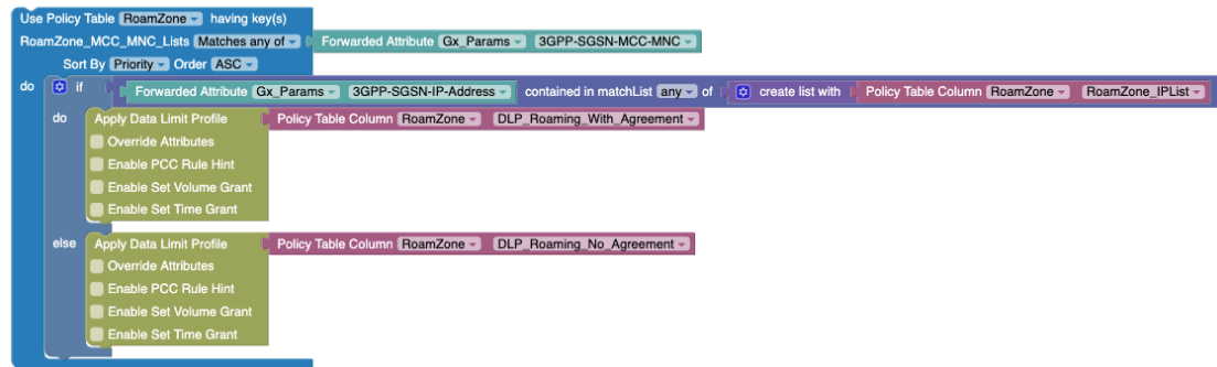
Figure 4-72 Example: Use of Policy Table Column block
