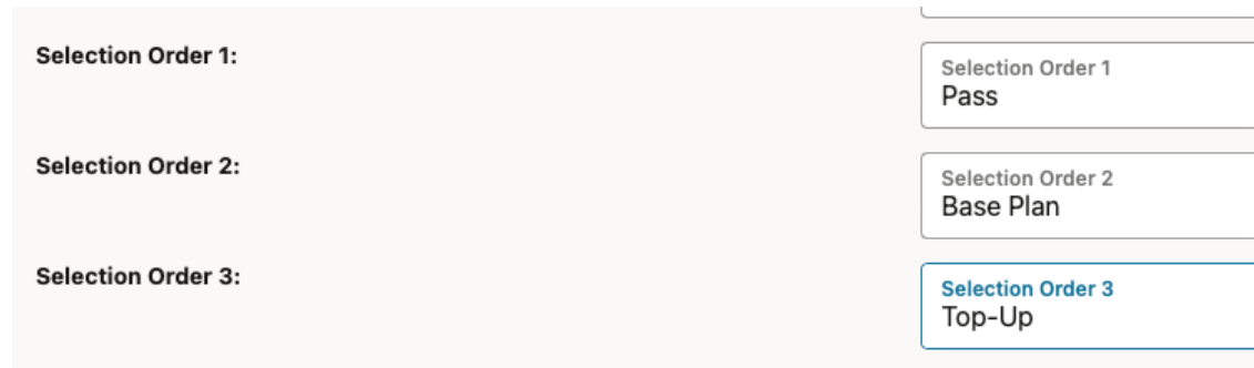
Figure 4-53 PCRF Core Configuration for Monthly Plan with Weekend Pass
