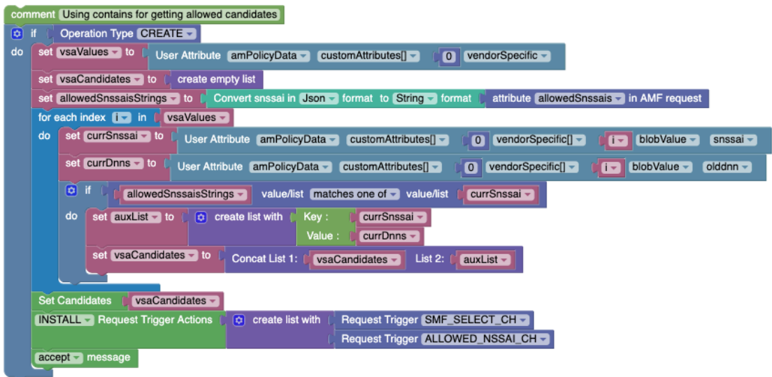
Figure 4-21 Using Contains for Getting Allowed Candidates
