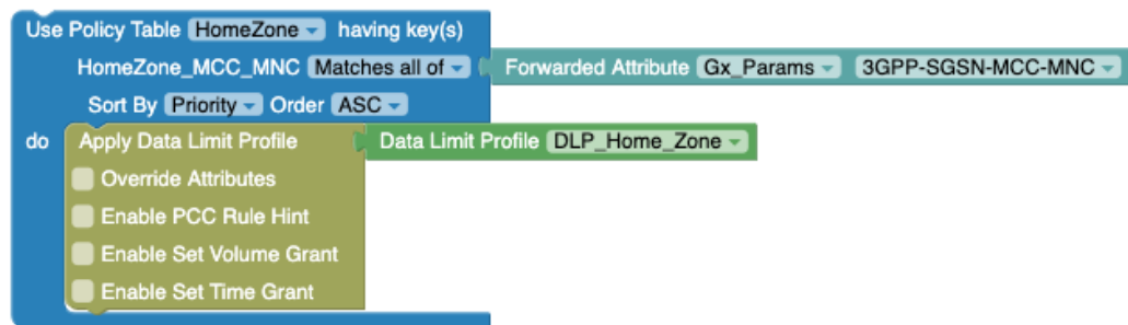
Figure 4-68 Example: Use Policy Table with Matches All Of option
