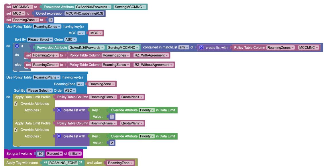
Figure 4-59 Policy Project for Autoenrolled Roaming Subscriber with Multiple Roaming Passes
