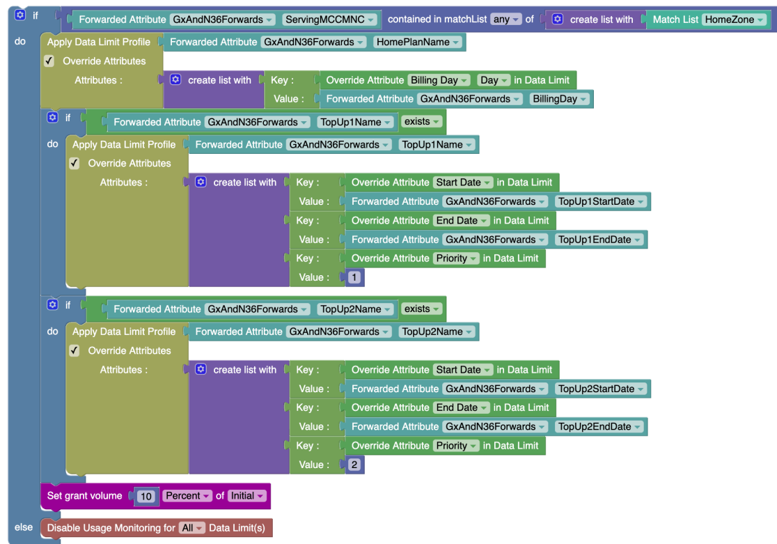
Figure 4-56 Policy Project for Monthly Plan with Multiple Top-ups
