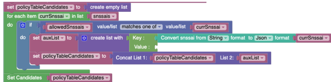
Figure 4-25 Example4: DNN Replacement - Candidates with no DNNs
