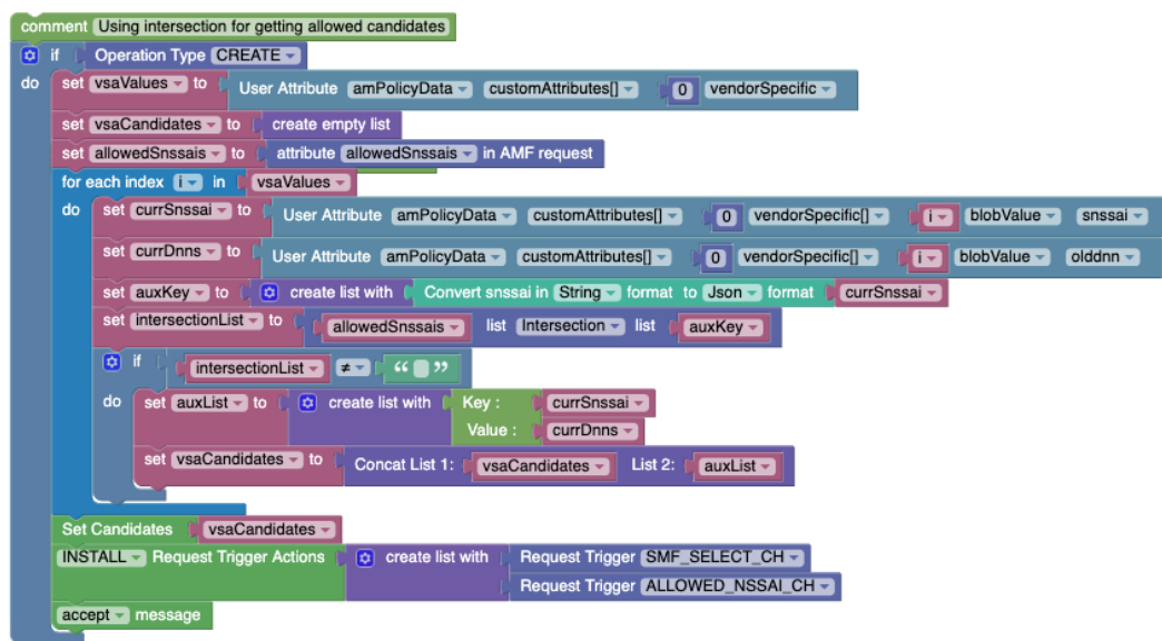
Figure 4-19 Using Intersection for Getting Allowed Candidates for Create Request
