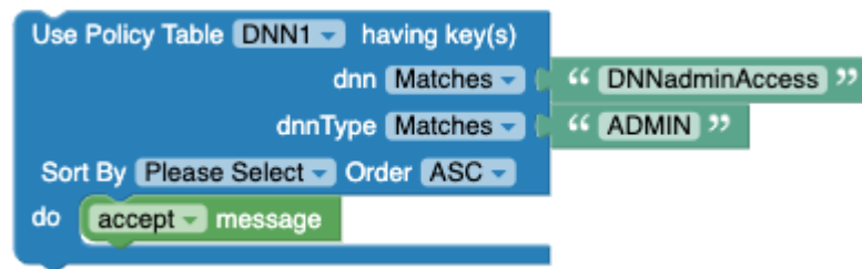
Figure 4-67 Example: Use Policy Table with Matches option
