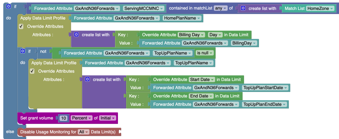
Figure 4-48 Policy Project for Home Monthly Plan with Top-ups
