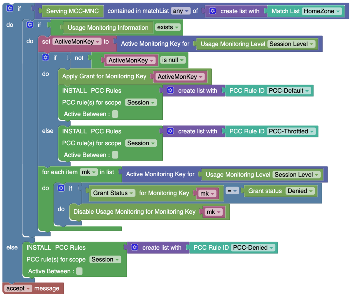
Figure 4-34 PCRF Core Policy Project
