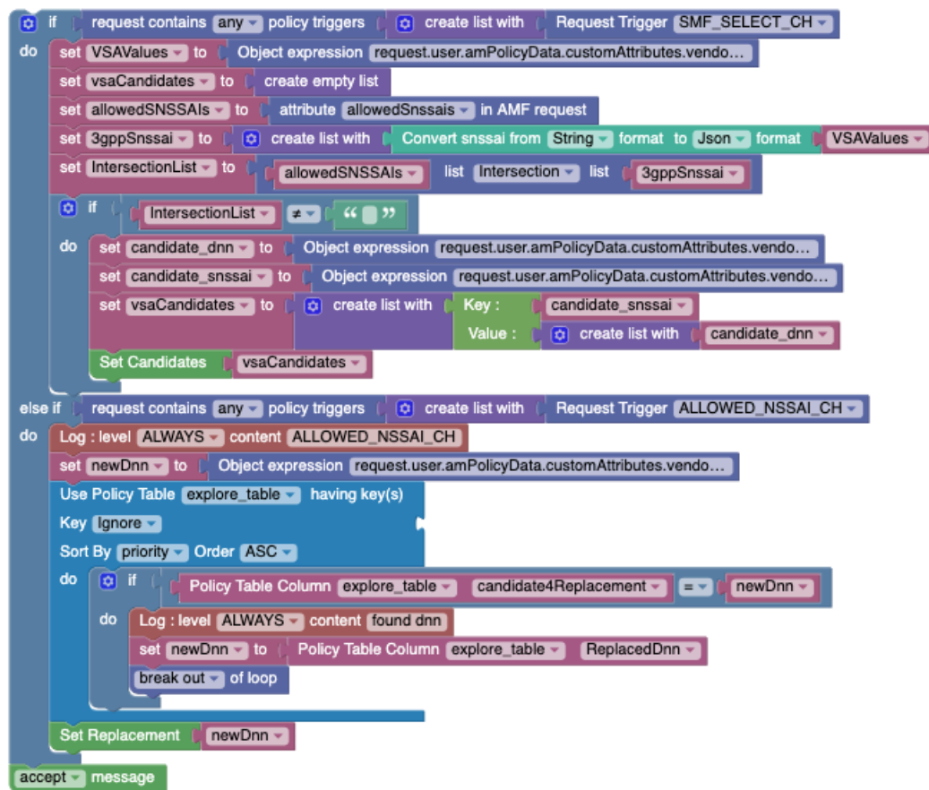
Figure 4-24 Example3: DNN Replacement
