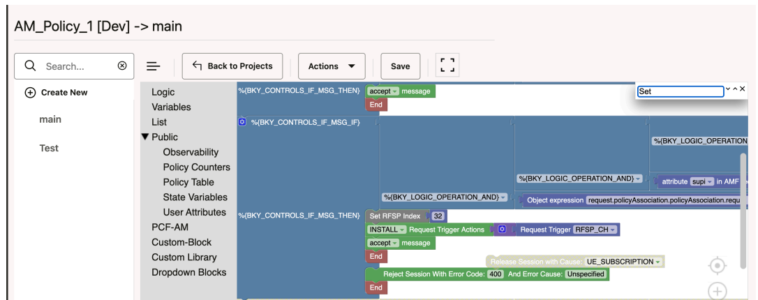
Figure 3-3 Wokspace Search Plugin
