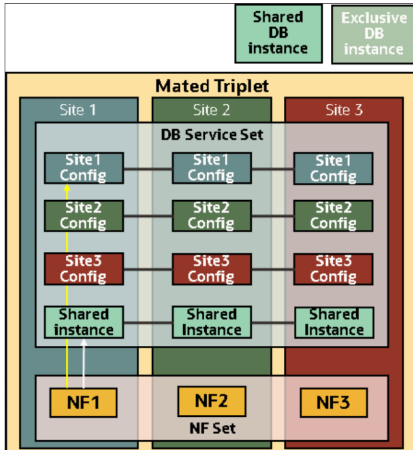
Figure 8-1 Database Model
