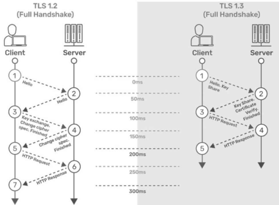
Figure 3-4 TLS 1.2 and TLS 1.3 Handshake
