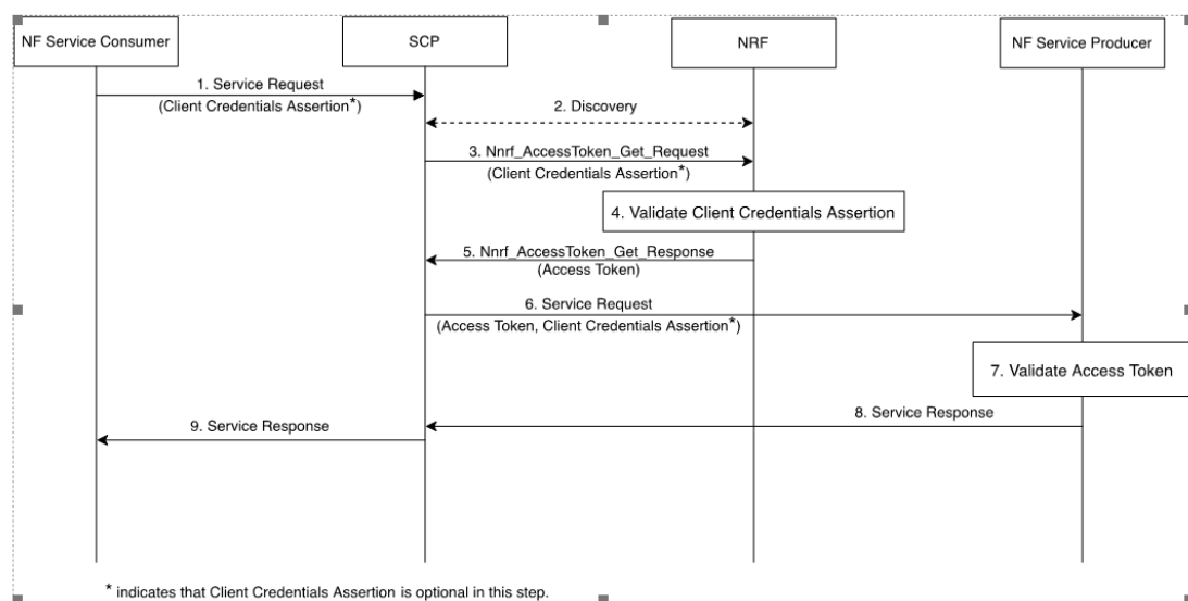
Figure 3-6 SCP Obtains Access Tokens from NRF
