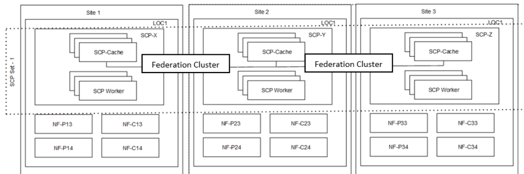
Figure 3-12 Role of SCP-Cache
