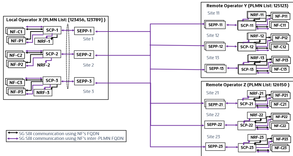
Figure 3-16 Local and Remote Routing
