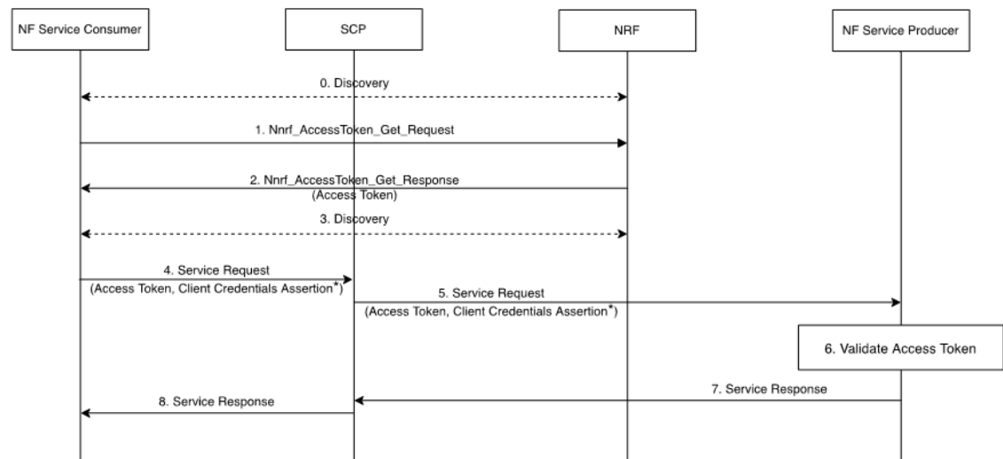
Figure 3-7 NF Consumer Obtains Access Tokens from NRF
