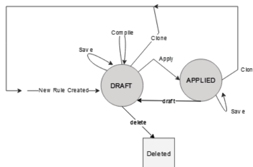
Figure 3-8 Rule Status Flow
