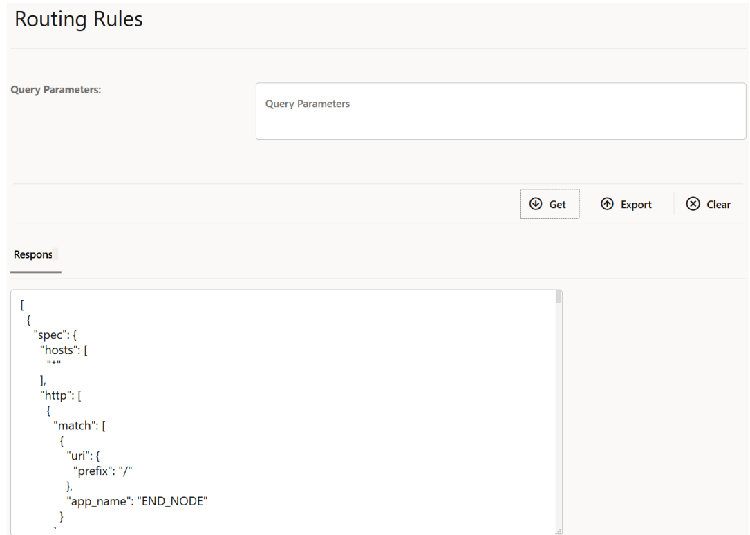
Figure 4-48 Response data
