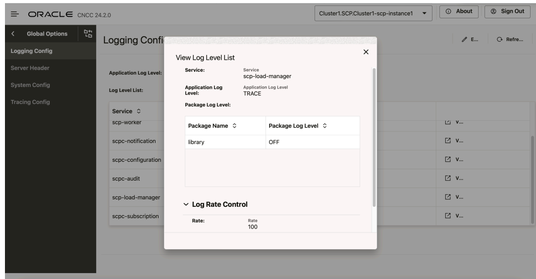
Figure 4-39 TRACE Log Level
