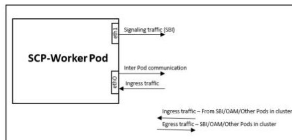
Figure 3-13 Networking-Multus Support
