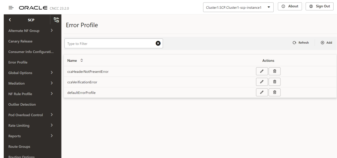
Figure 4-34 Error Profile
