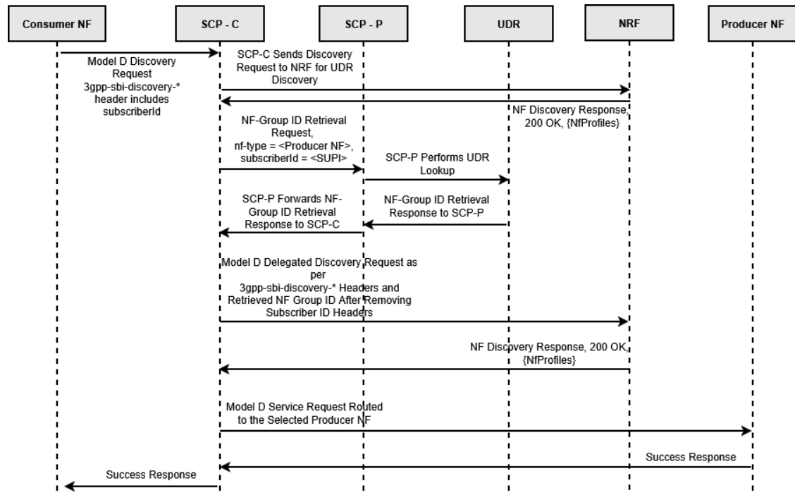
Figure 3-1 SUPI to Group ID Resolution
