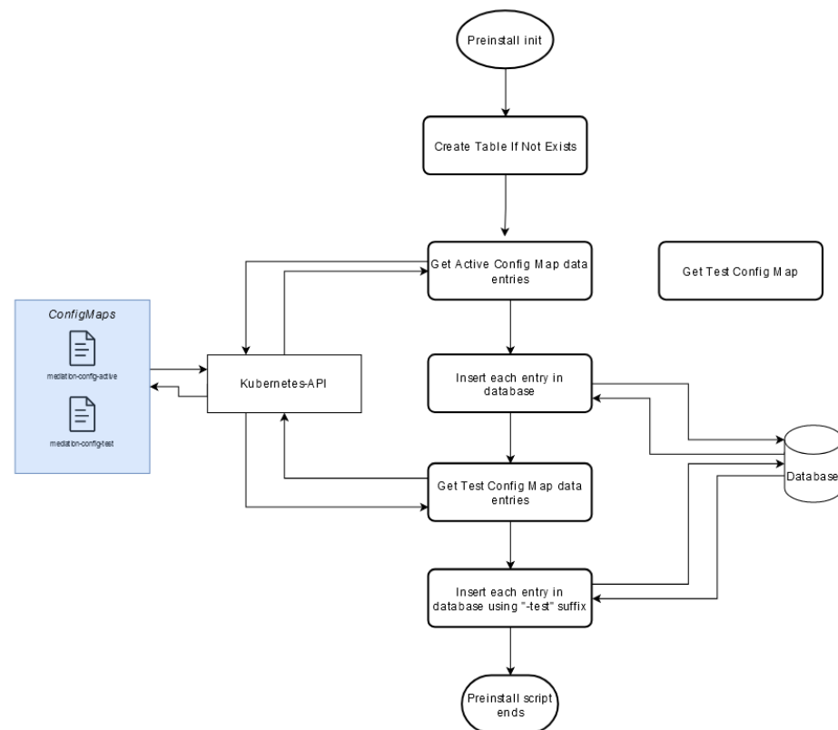
Figure 3-9 Migration to Database table
