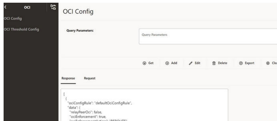
Figure 4-26 OCI Config
