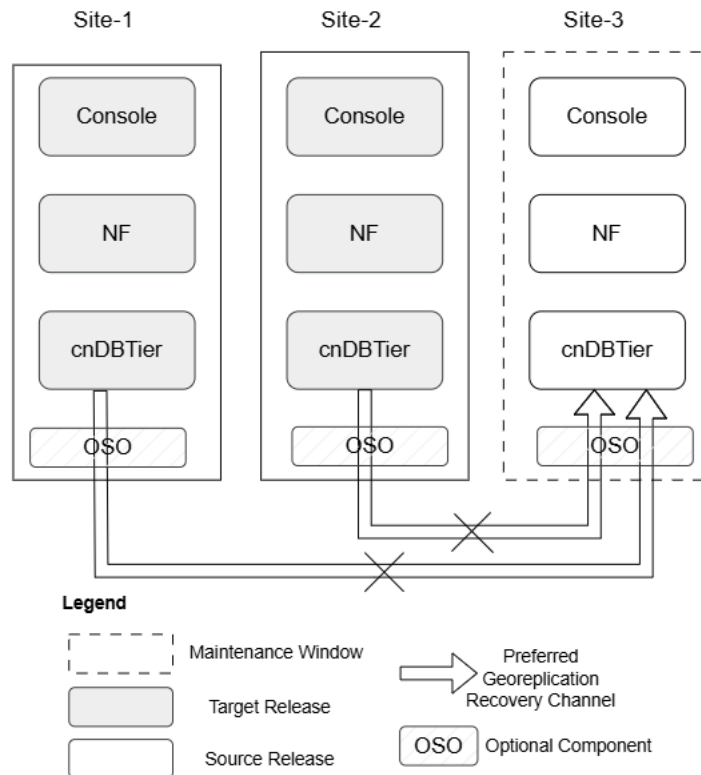
Figure 3-22 Scenario 7: Site 3 Rollback when replication break
