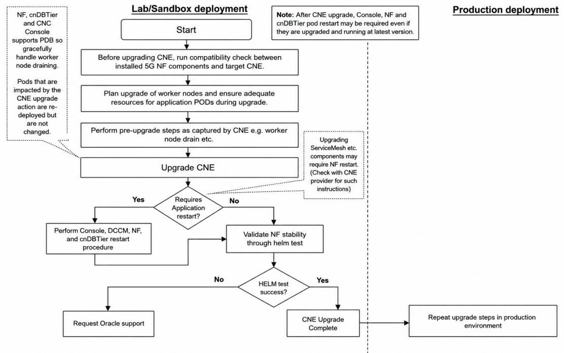
Figure 3-10 Non-Oracle CNE Upgrade
