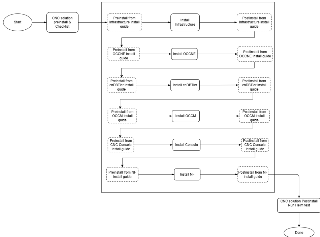
Figure 2-4 Planning Installation of CNC Solution
