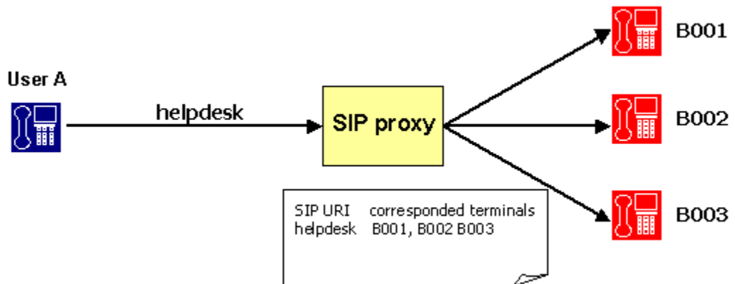
Figure 2-4 Proxy Forking
