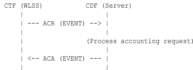
Example 3-1 Message Flow for Event-Based Charging
