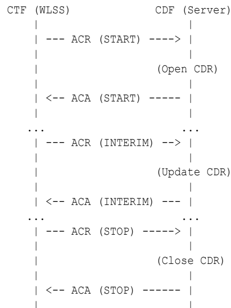
Example 3-2 Message Flow for Session-Based Charging
