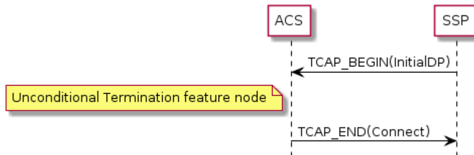
Figure 2-1 Unconditional Call Connection Message Sequence
