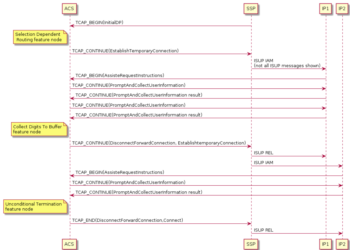
Figure 2-8 Prompt for Digits Using External Intelligent Peripheral SRF Message Sequence
