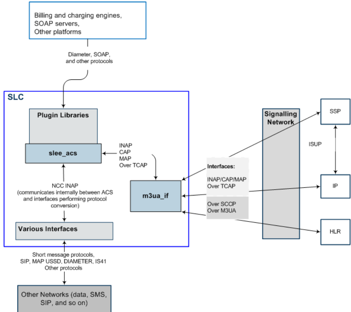
Figure 1-1 Relationship of ACS to INAP, CAP, and MAP Interfaces
