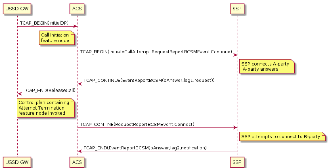
Figure 2-14 Call Initiation (CS1) Message Sequence
