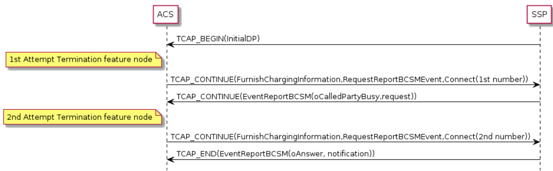
Figure 2-5 FurnishChargingInformation Message Sequence
