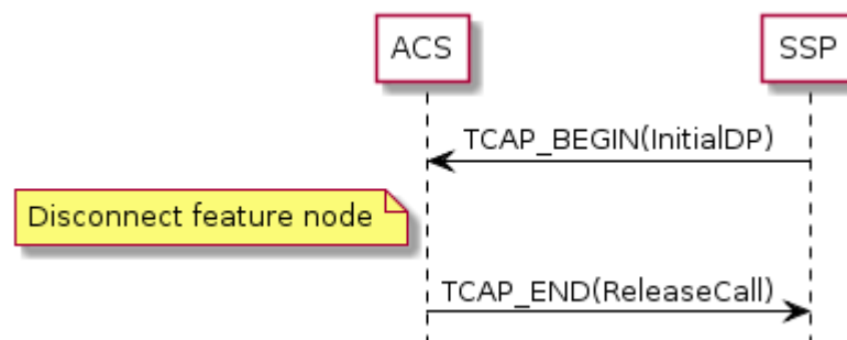
Figure 2-2 Release Call Message Sequence
