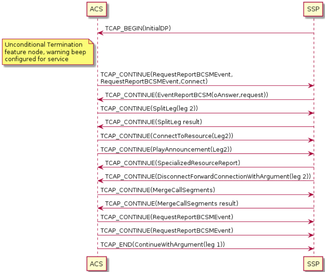
Figure 2-9 Post Answer Beep or Announcement Message Sequence
