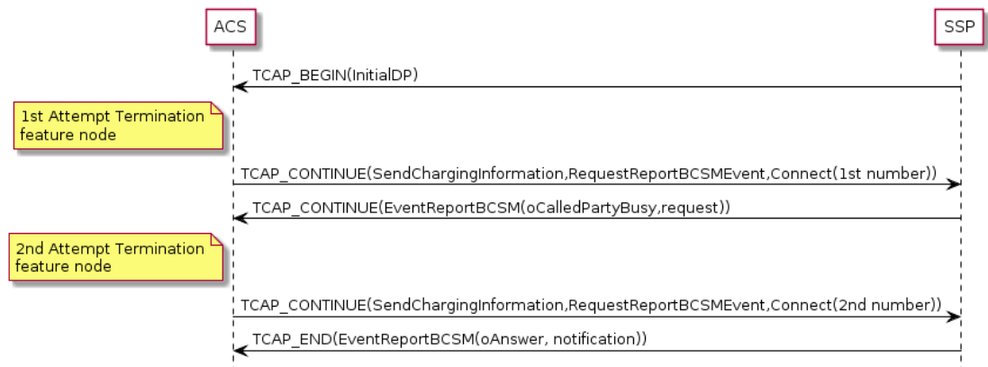
Figure 2-6 FurnishChargingInformation Message Sequence
