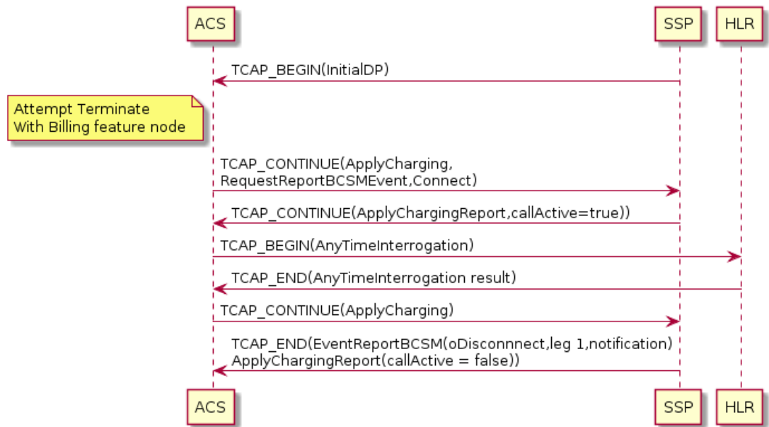
Figure 2-13 Real Time Charge, Location Information Retrieval Message Sequence
