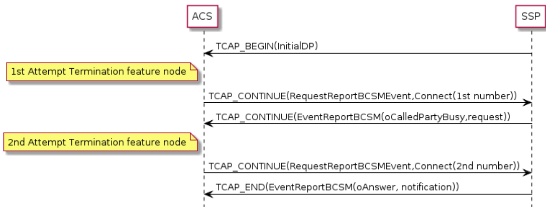
Figure 2-3 Divert on Busy Message Sequence
