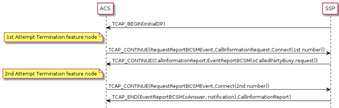
Figure 2-4 CallInformationReport Message Sequence
