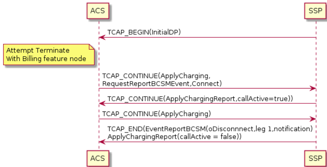
Figure 2-10 Real Time Charging, Caller Hangs Up Message Sequence
