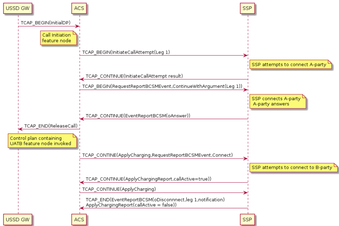
Figure 2-15 Call Initiation (CAP4) Message Sequence
