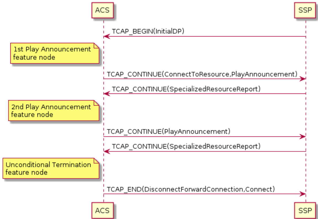
Figure 2-7 Play an Announcement (Internal SRF) Message Sequence
