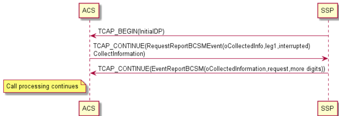
Figure 2-16 CollectInformation Message Sequence
