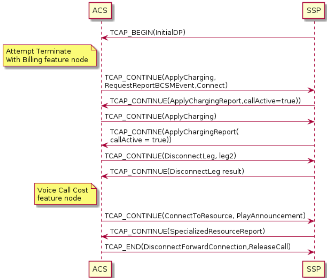
Figure 2-12 Real Time Charge, Disconnect B-party When Funds Exhausted Message Sequence
