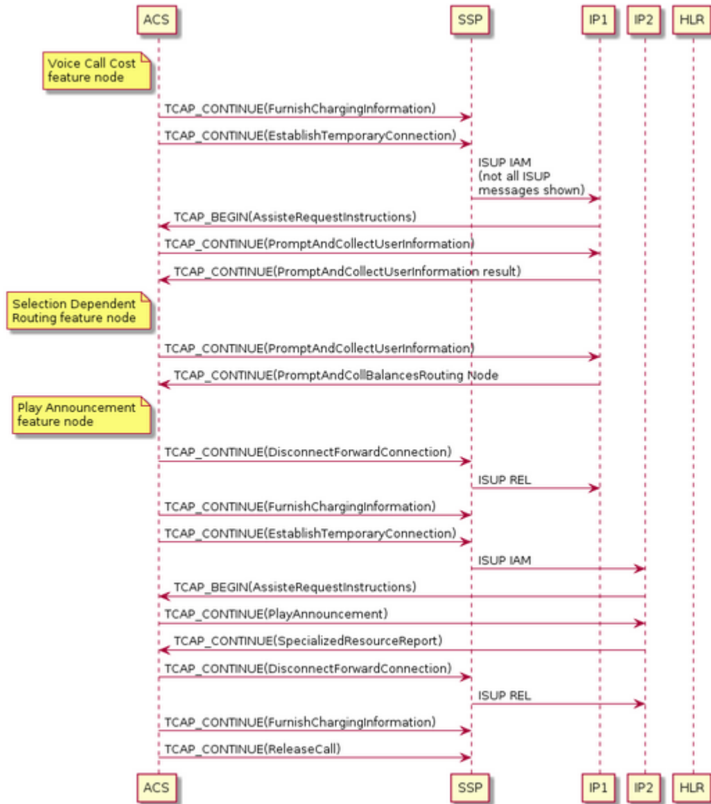
Figure 2-18 Combined Message Sequence Example 2
