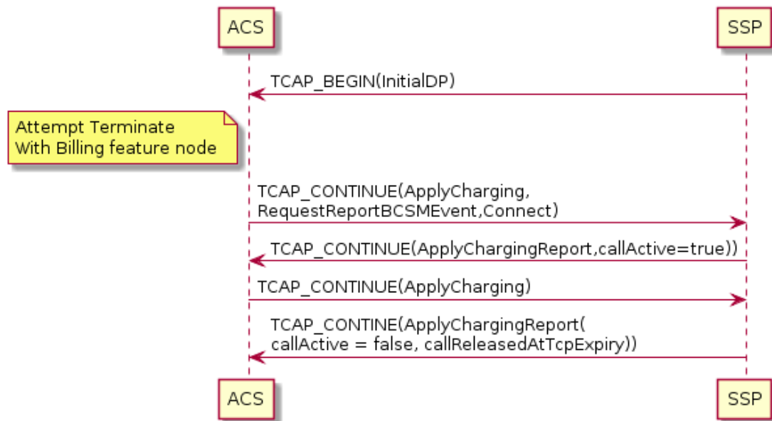
Figure 2-11 Real Time Charging, Funds Exhausted Message Sequence
