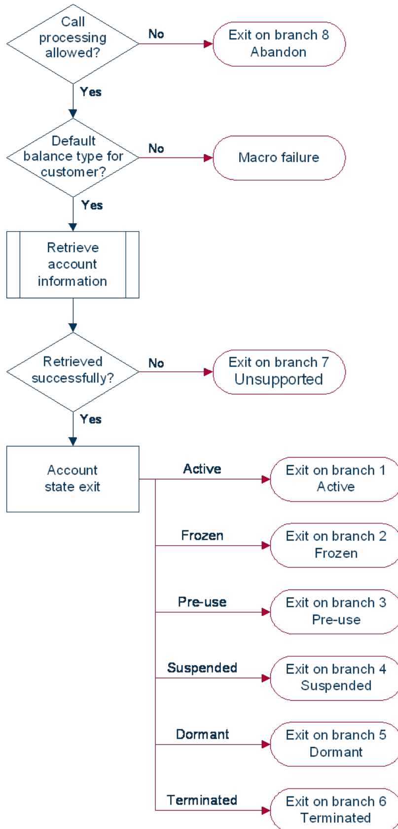
Figure 7-1 Node logic
