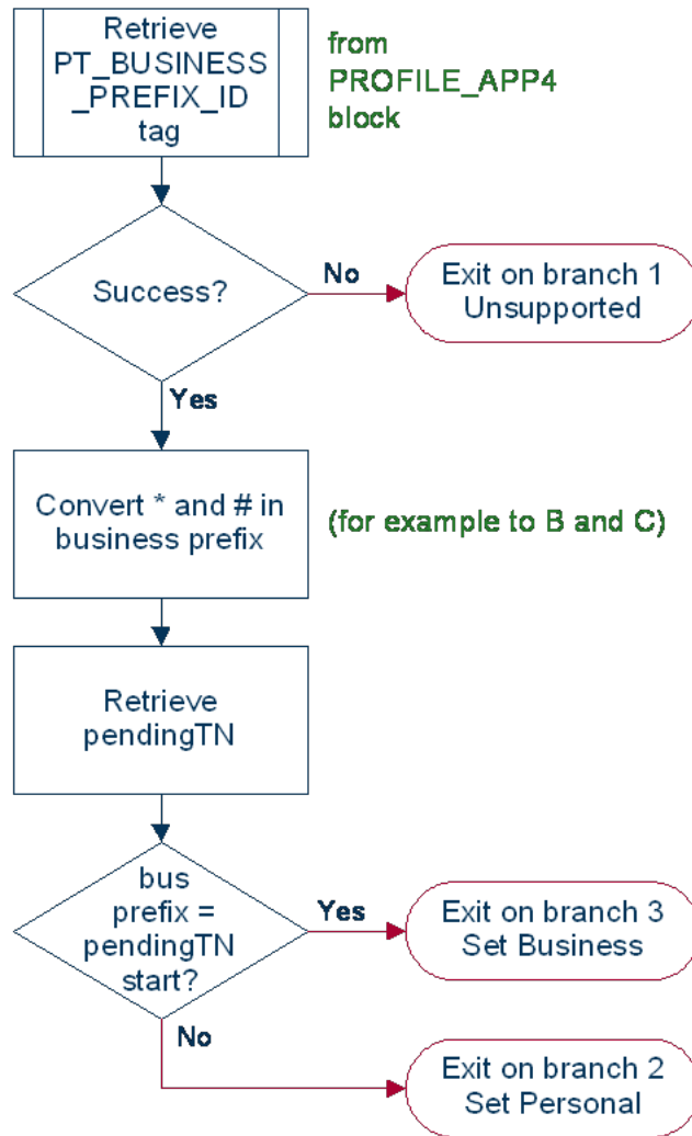
Figure 3-2 Node logic
