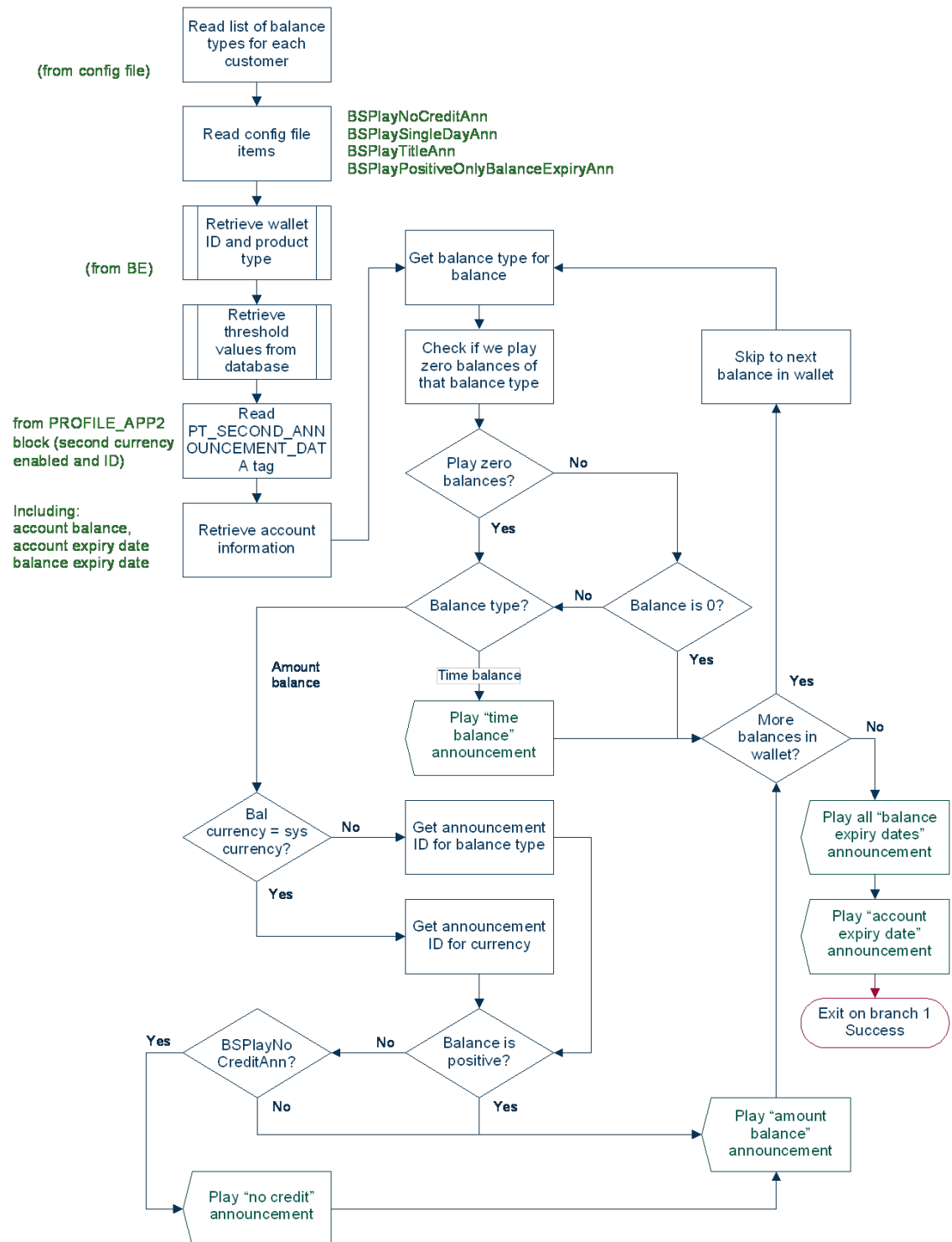
Figure 7-2 Node logic
