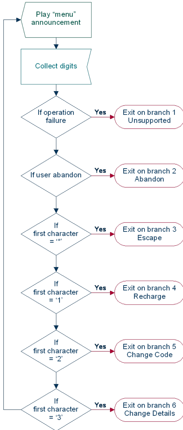
Figure 5-2 Node logic
