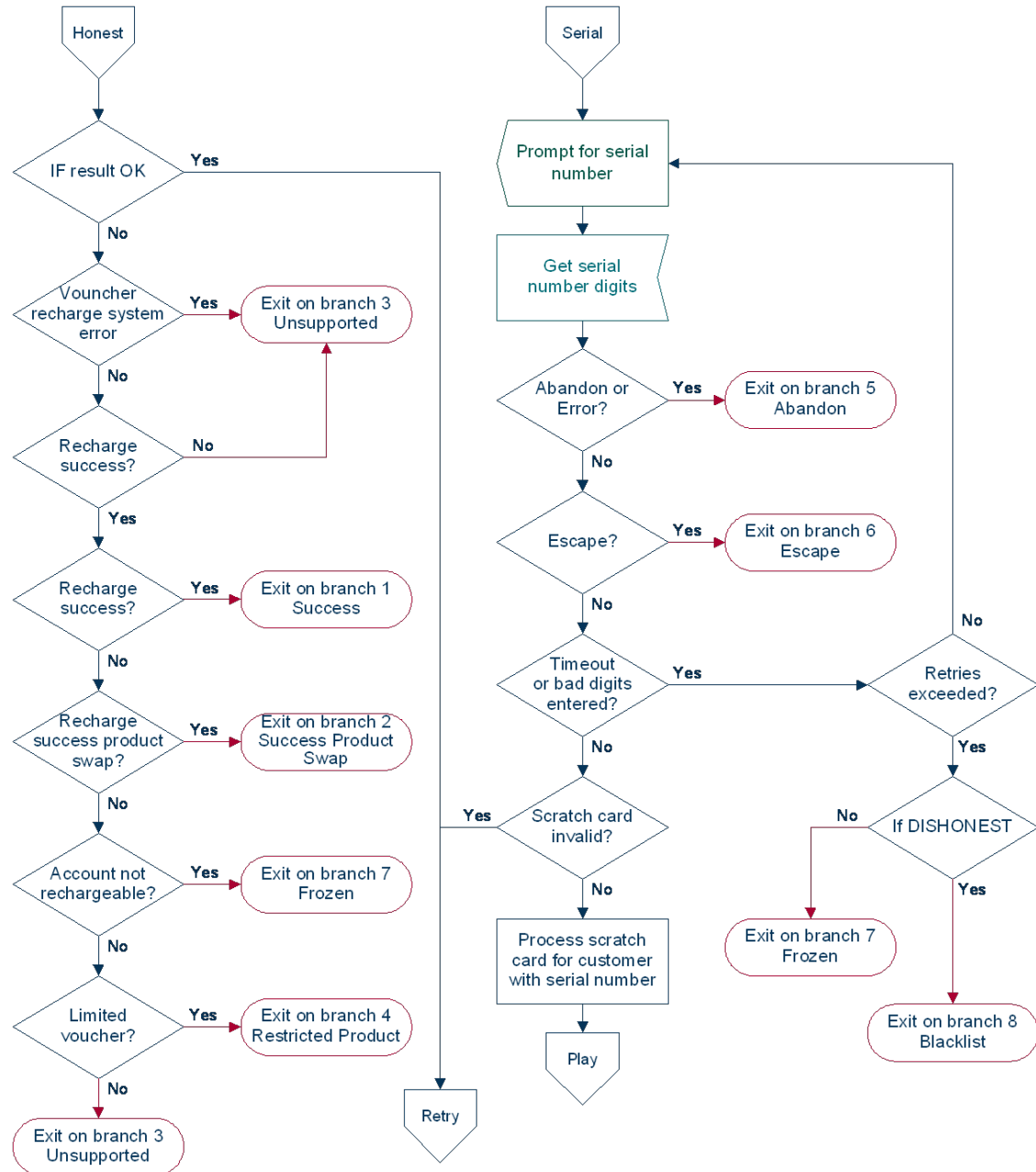
Figure 6-7 Node logic
