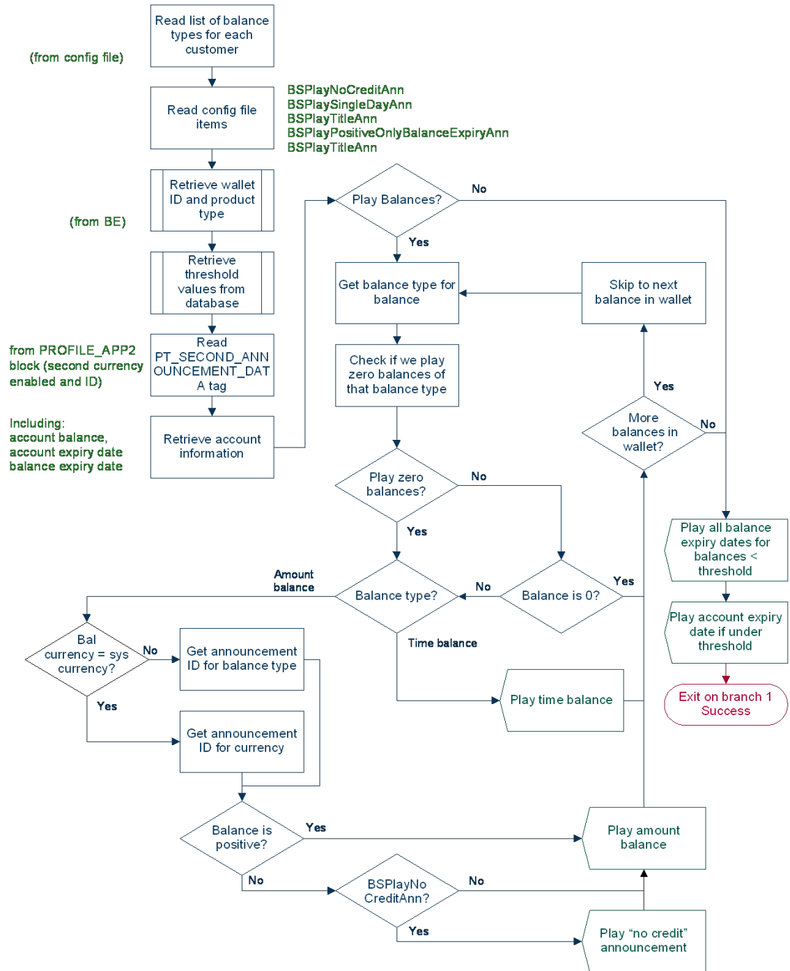
Figure 7-4 Node logic
