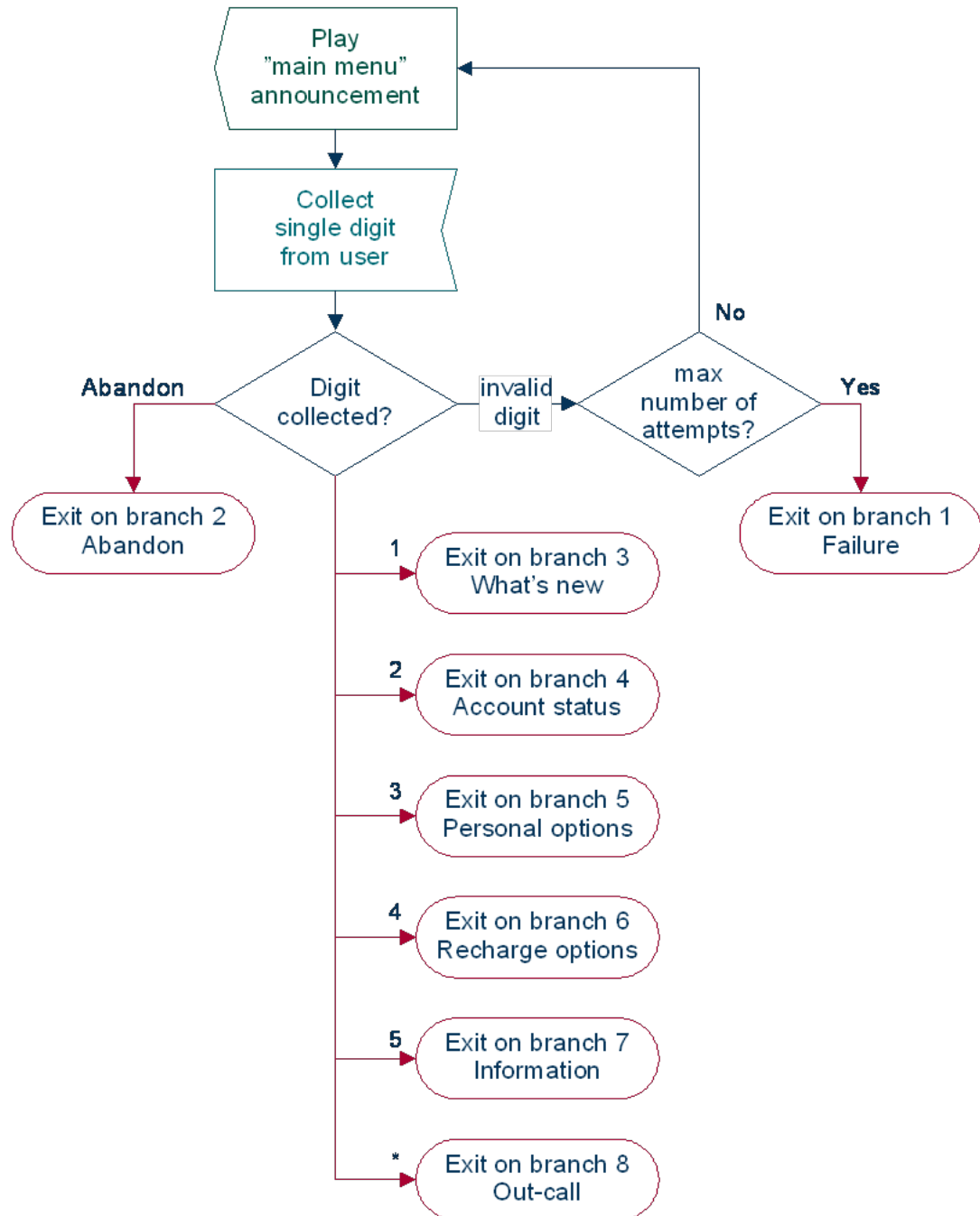
Figure 5-6 Node logic
