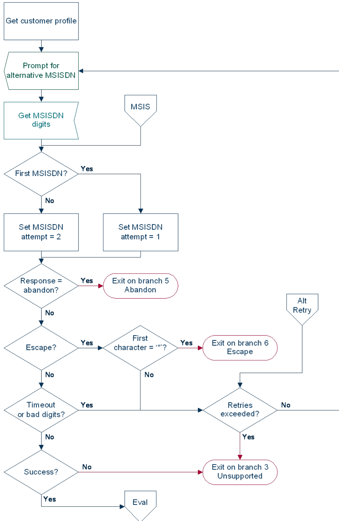
Figure 6-3 Node logic
