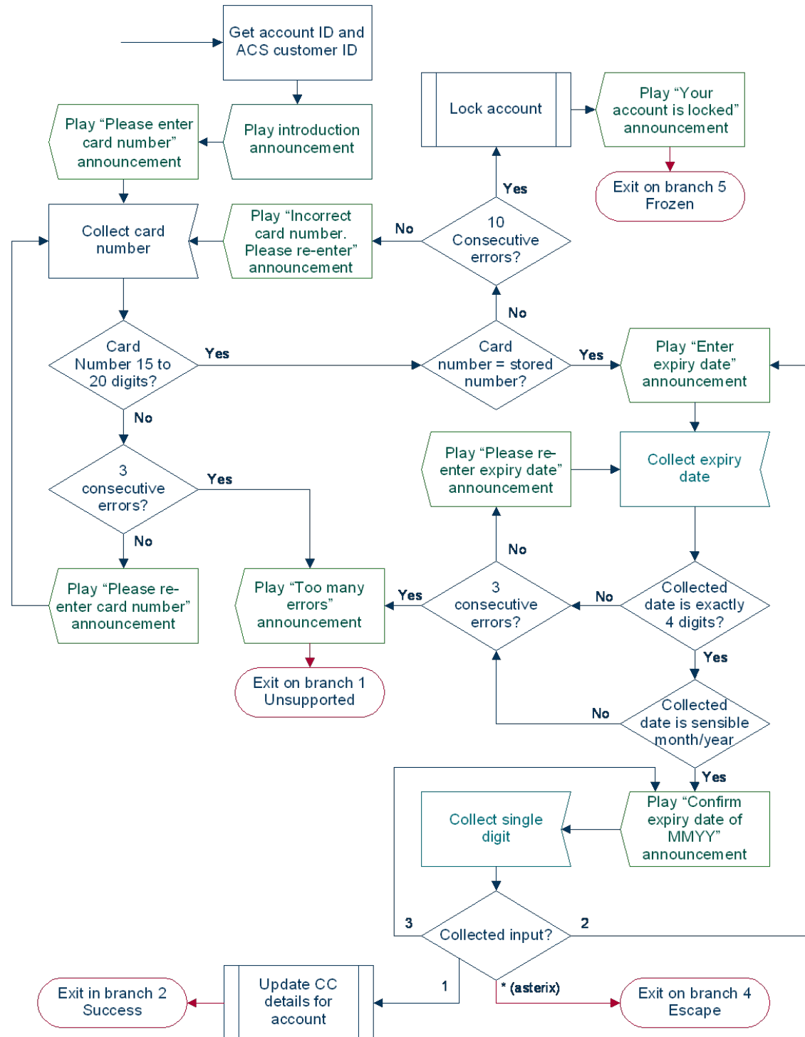
Figure 5-1 Node logic
