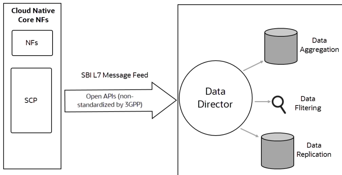
Figure 2-2 Solution Overview
