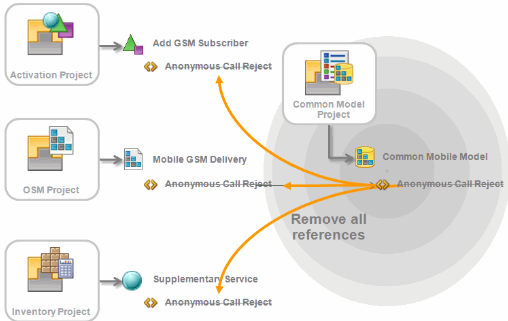
Figure 2-13 Refactoring Solutions Using Remove
