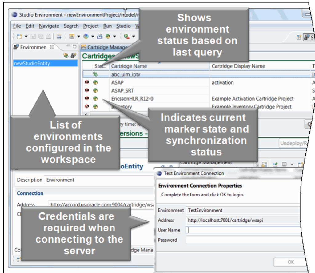
Figure 5-1 Environment Perspective
