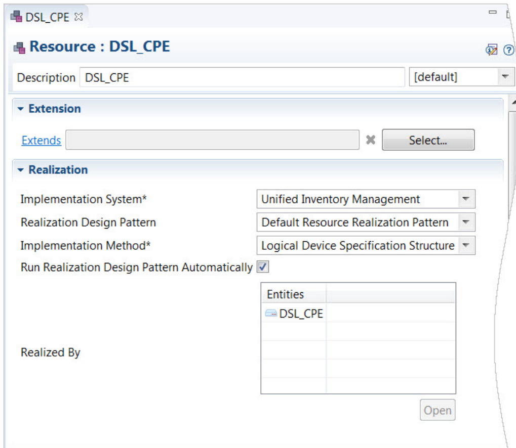
Figure 4-13 DSL_CPE Properties
