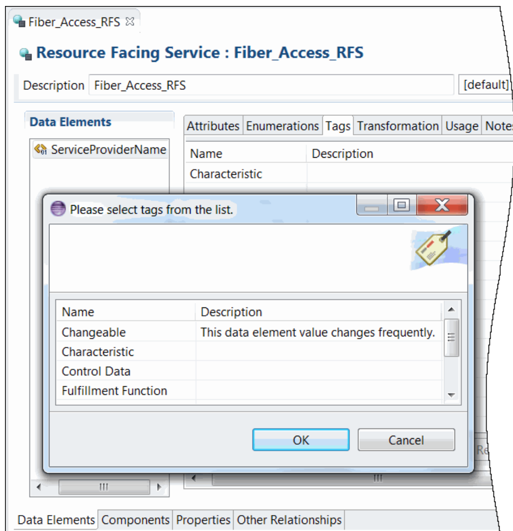
Figure 2-4 Tags Tab
