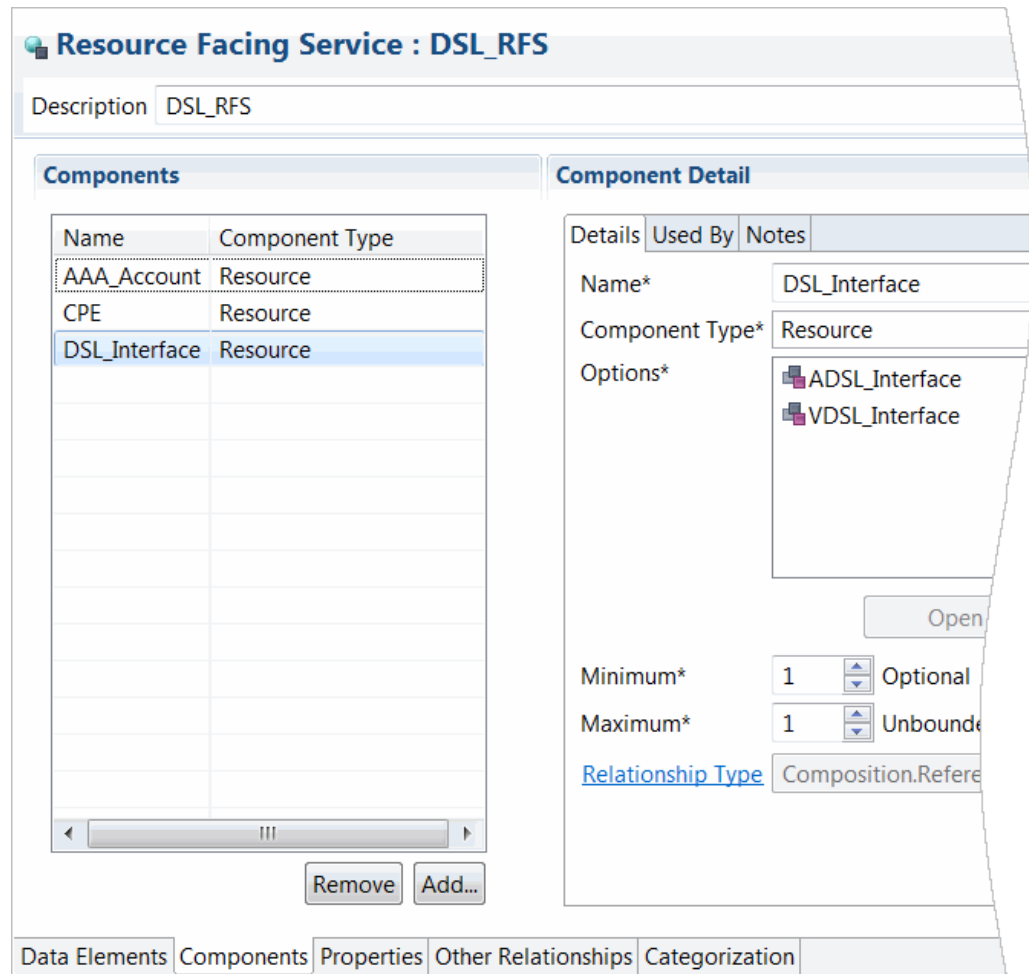
Figure 4-8 DSL_RFS Components
