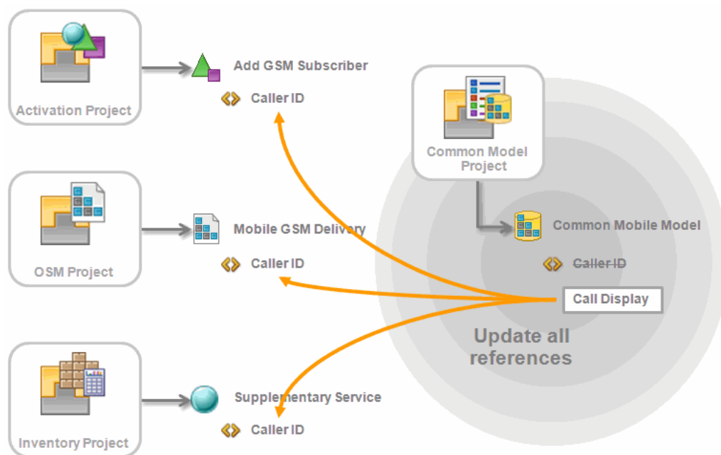
Figure 2-12 Refactoring Solutions Using Renaming
