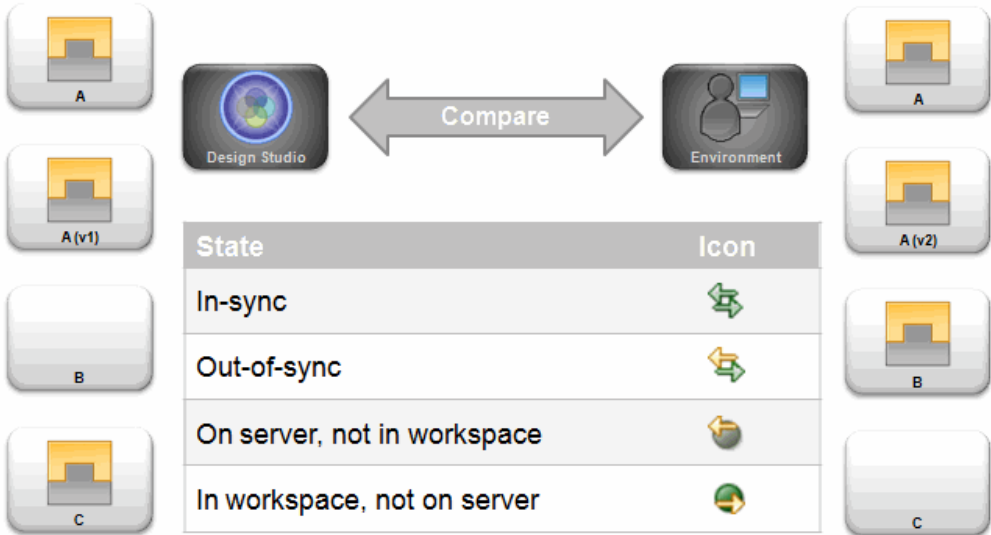
Figure 5-3 Cartridge Deployment Synchronization
