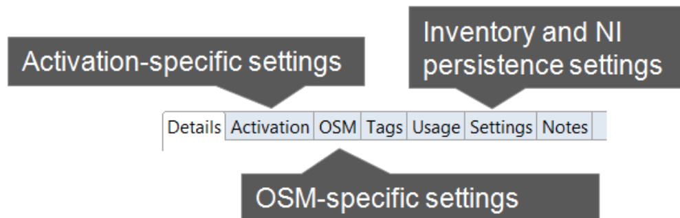
Figure 2-5 Application-Specific Tabs
