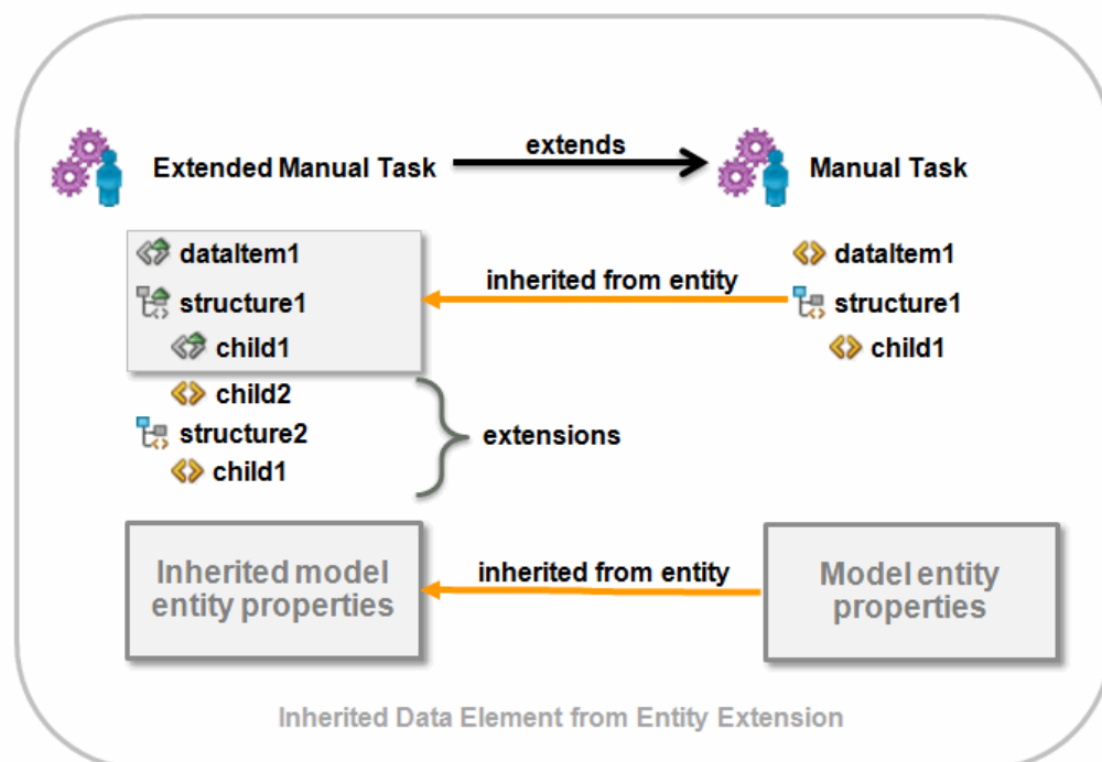
Figure 2-10 Extending Entities
