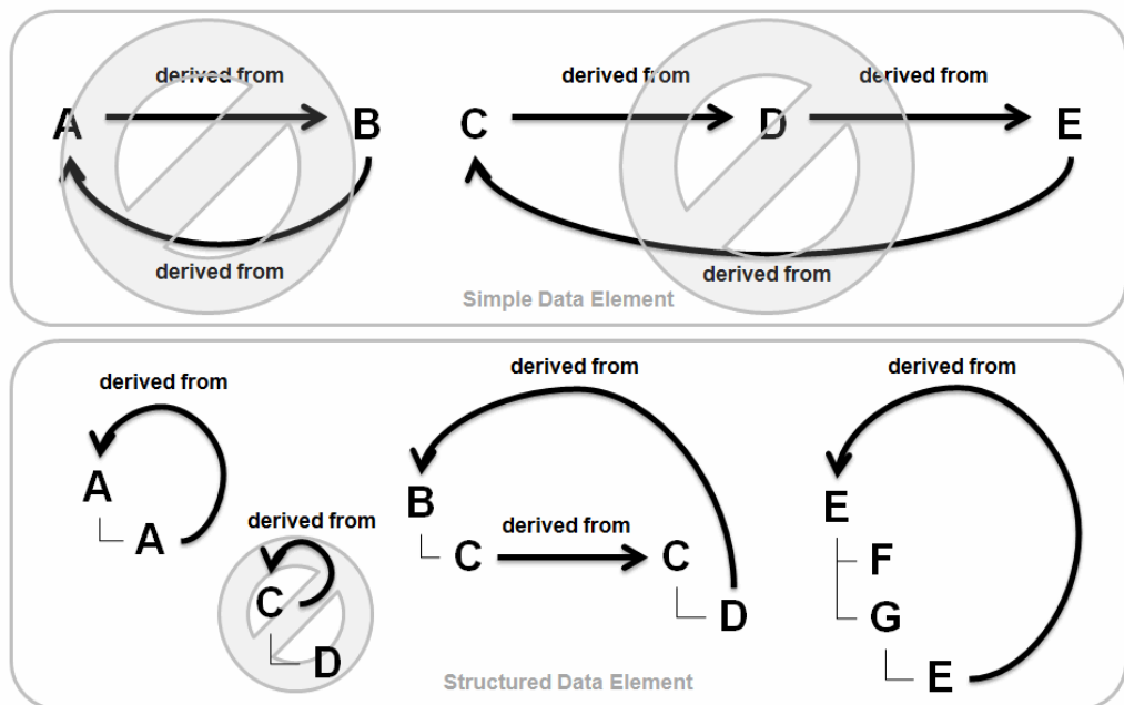
Figure 2-8 Recursion Patterns
