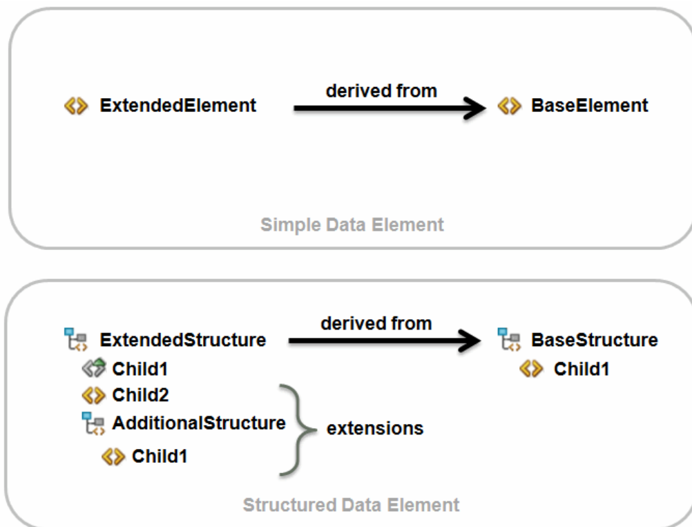
Figure 2-6 Derived Data Elements
