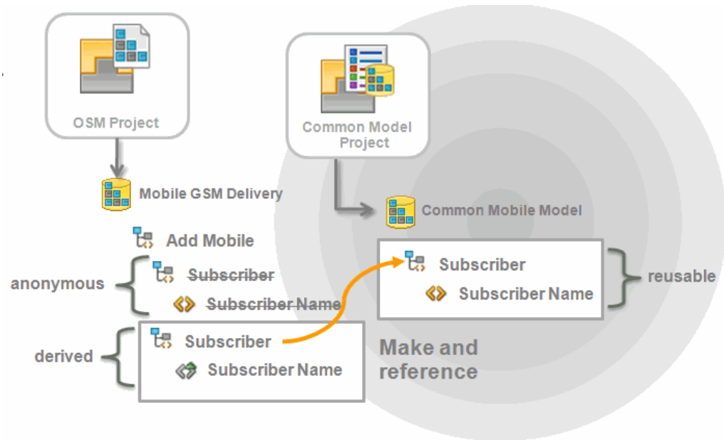
Figure 2-14 Refactoring using Make Reusable
