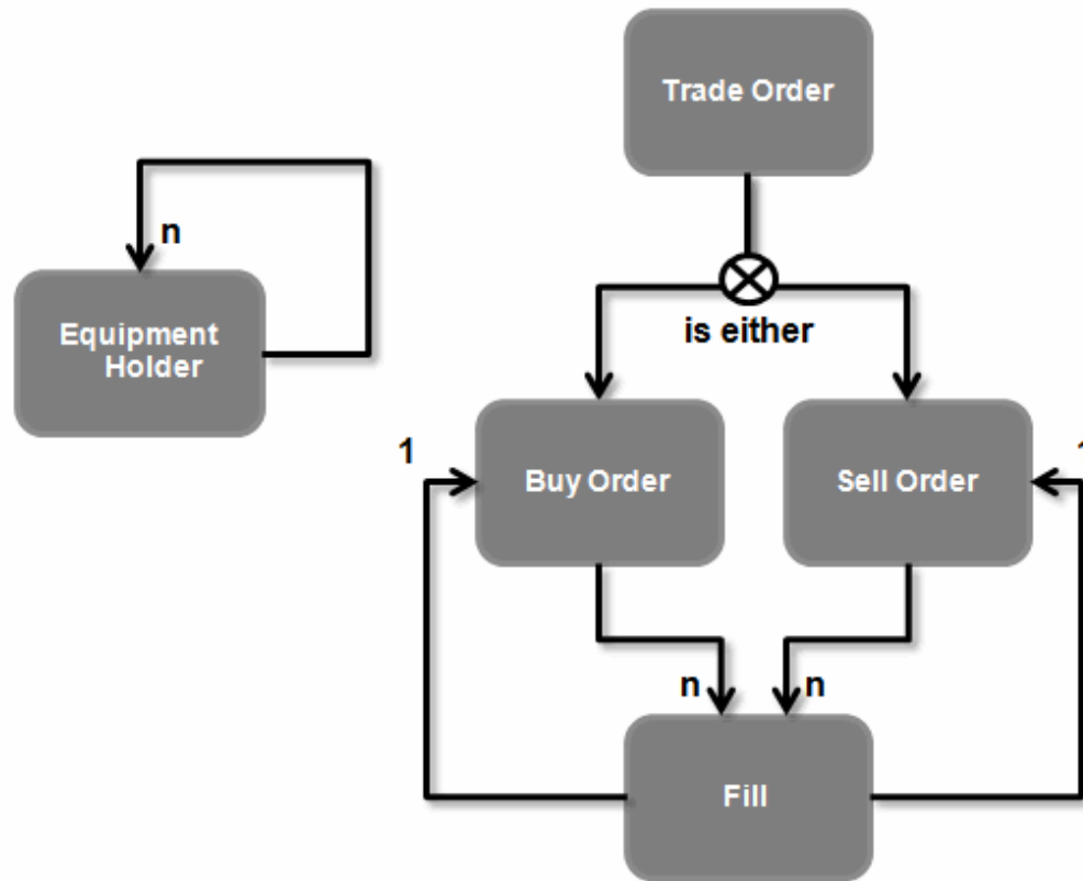
Figure 2-9 Data Models Illustrating Recursion
