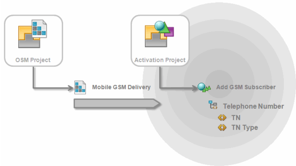
Figure 2-17 Example: OSM Leveraging Activation Data
