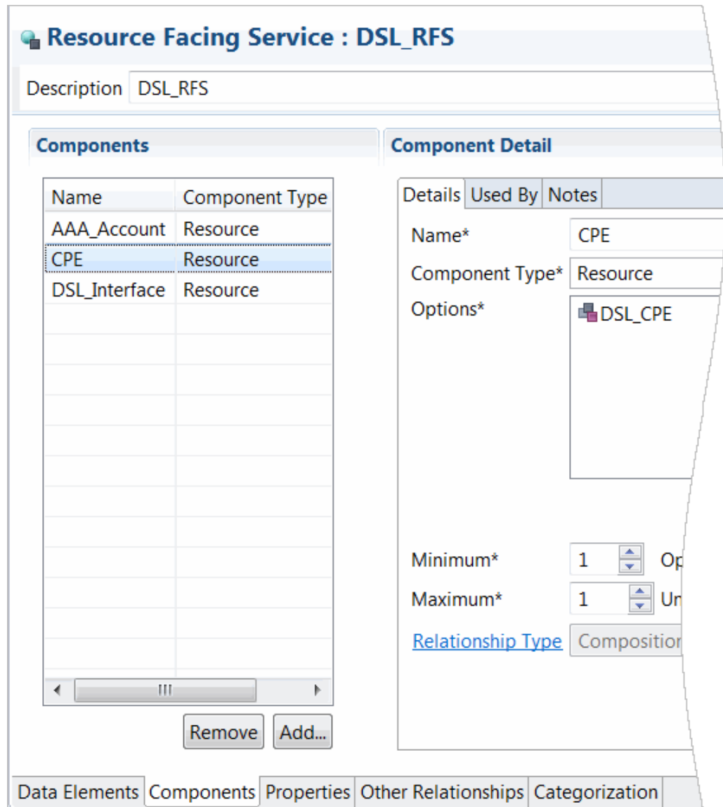
Figure 4-10 The CPE Component and the DSL_CPE Option
