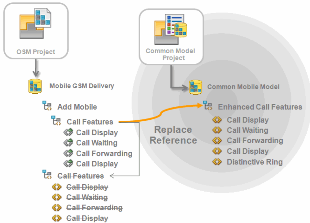
Figure 2-15 Refactoring Solutions Using Replace
