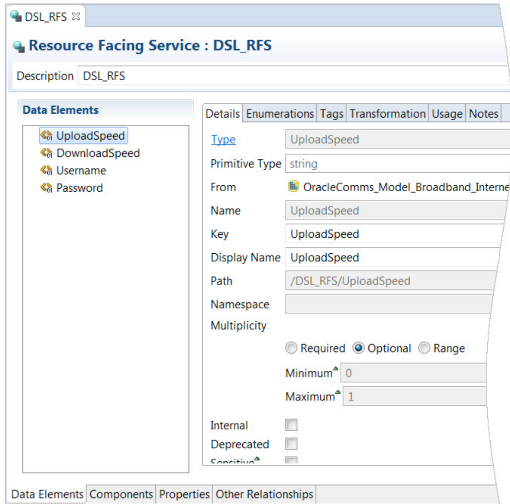
Figure 4-7 DSL_RFS Simple Data Elements
