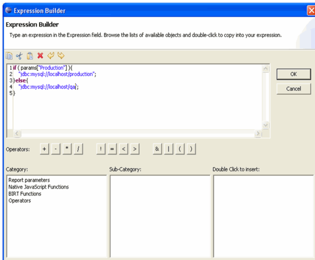
Figure 6-2 Expression Builder
