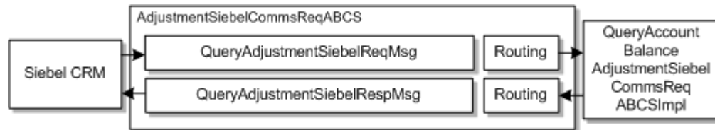
Figure 3-6 AdjustmentSiebelCommsReqABCS
