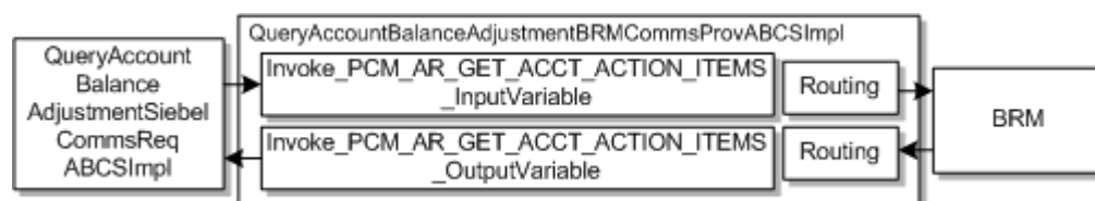
Figure 3-8 QueryAccountBalanceAdjustmentBRMCommsProvABCImpl
