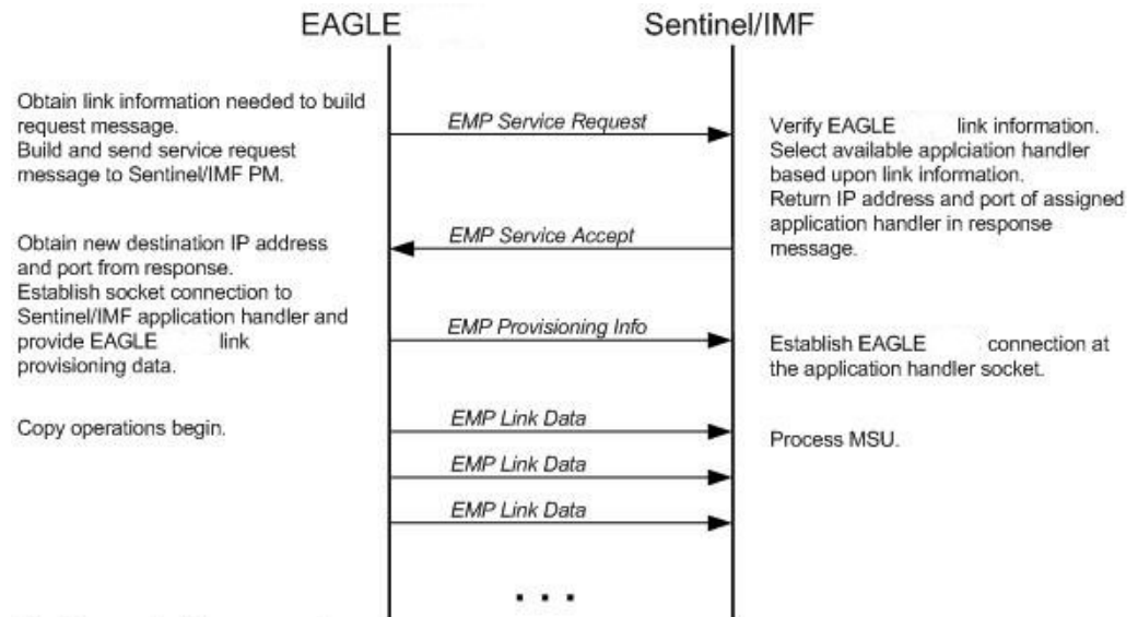
Figure 6-4 Ethernet Link Establishment - EMP Link Data
