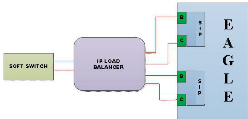
Figure 2-6 SLIC Card Signaling Network Redundancy
