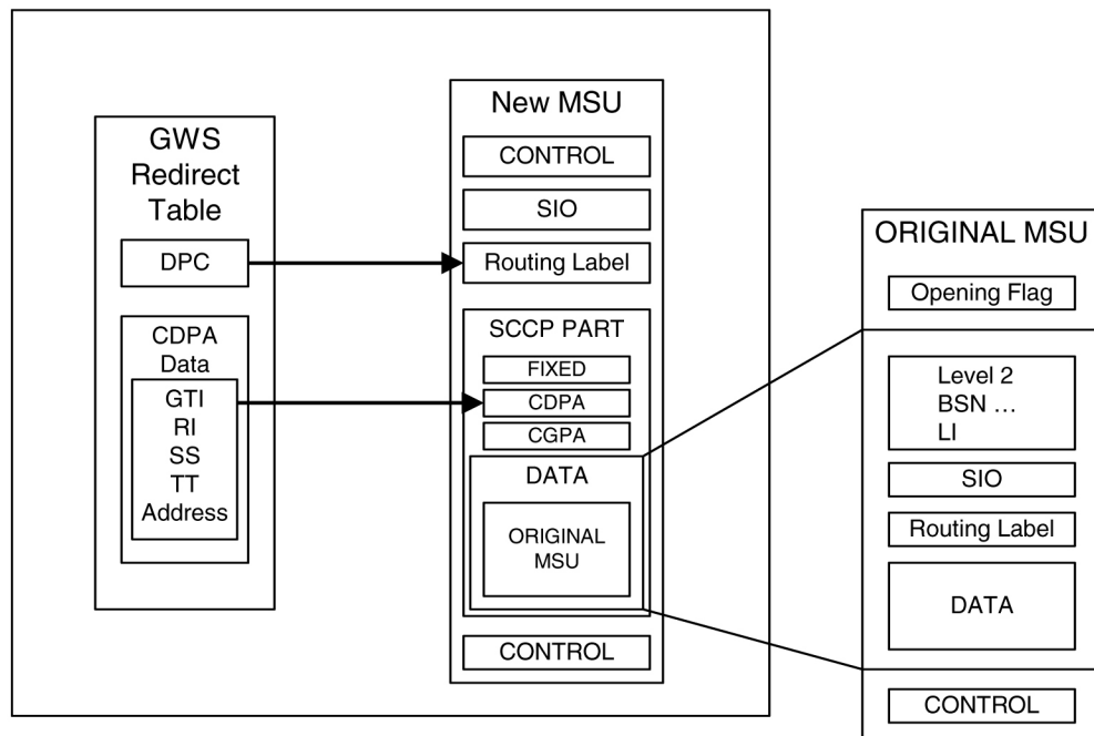
Figure 4-2 DTA Encapsulation
