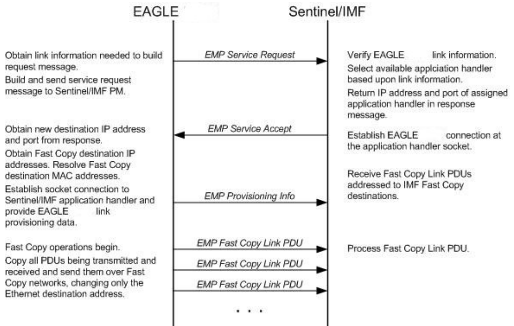
Figure 6-5 Ethernet Link Establishment - EMP Fast Copy Link PDU
