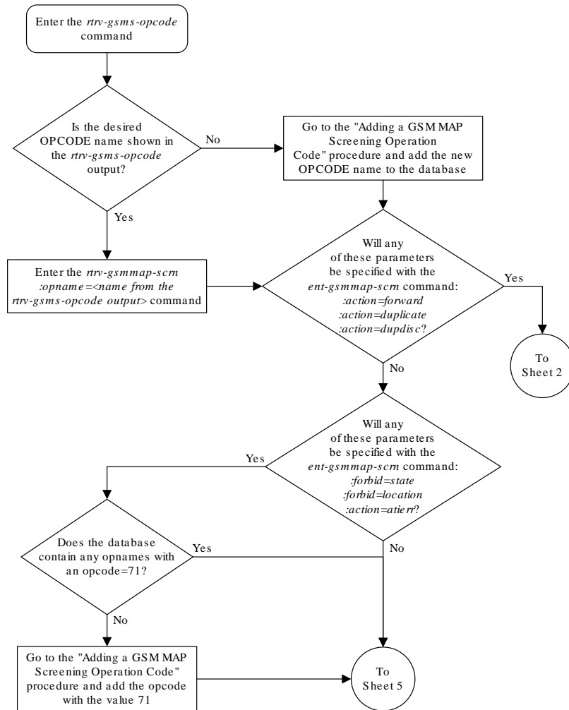
Figure 5-13 Adding a GSM MAP Screening Entry
