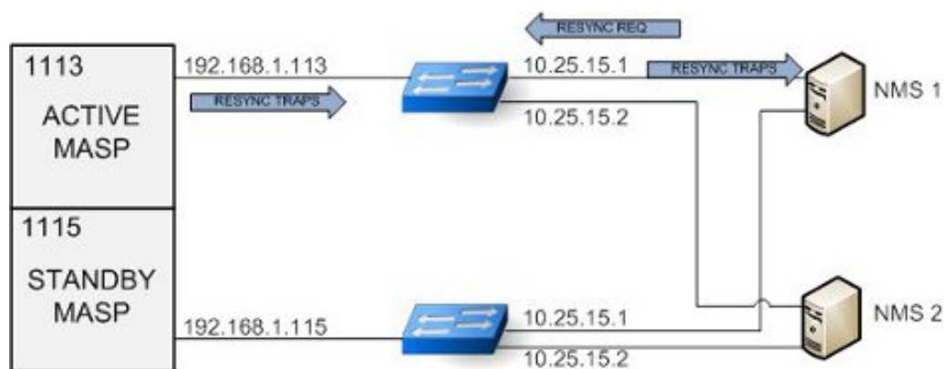
Figure 3-3 Resynchronization Request/Trap Flow
