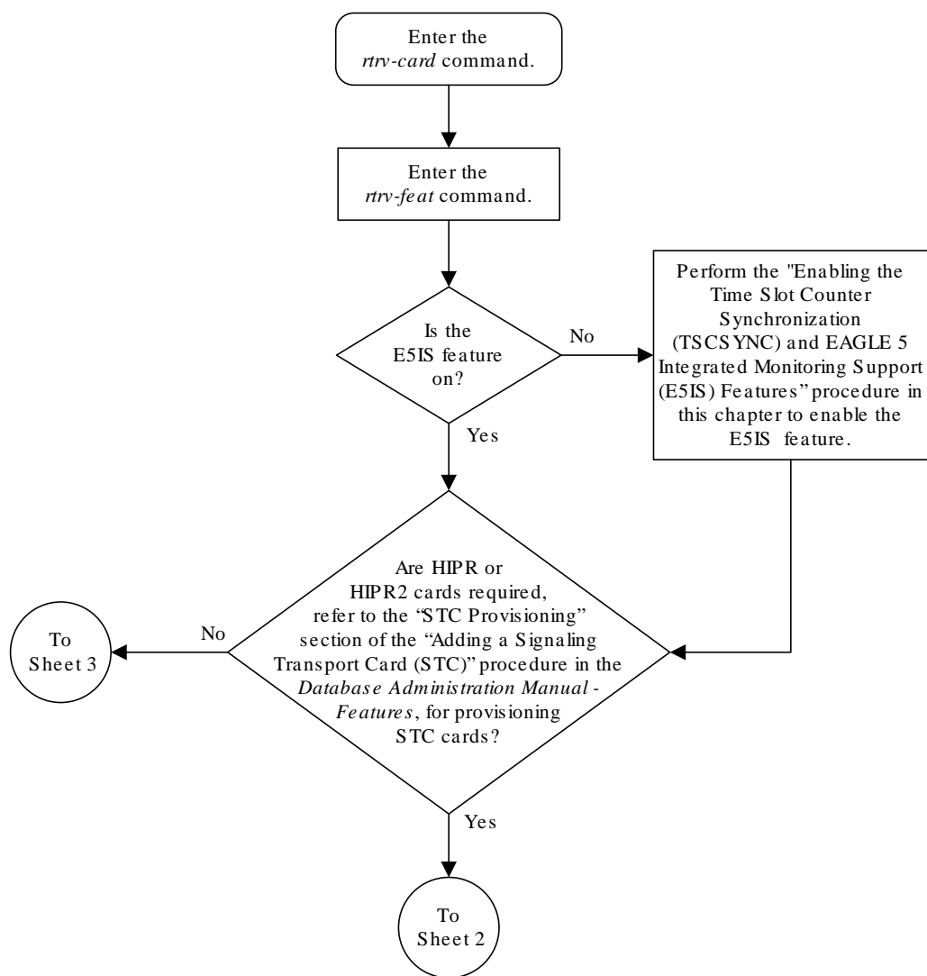
Figure 6-11 Adding a Signaling Transport Card (STC)
