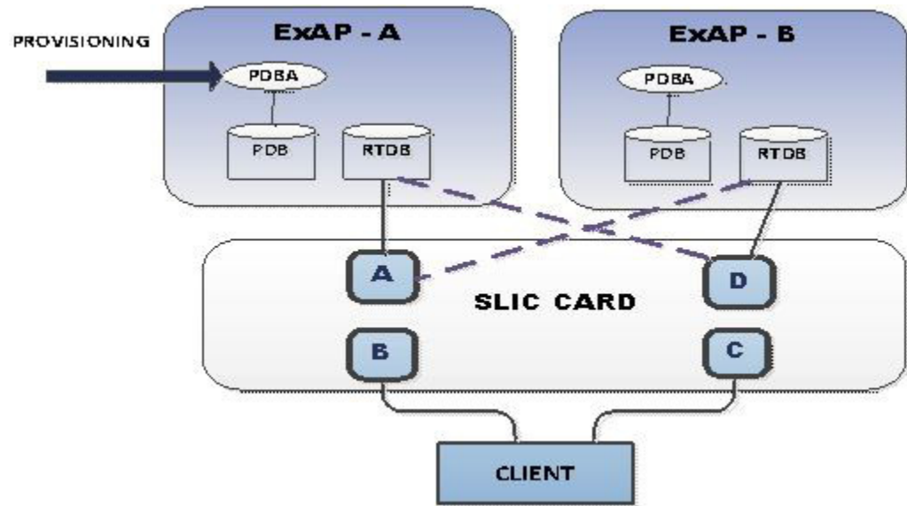
Figure 2-5 SLIC Network Redundancy Model
