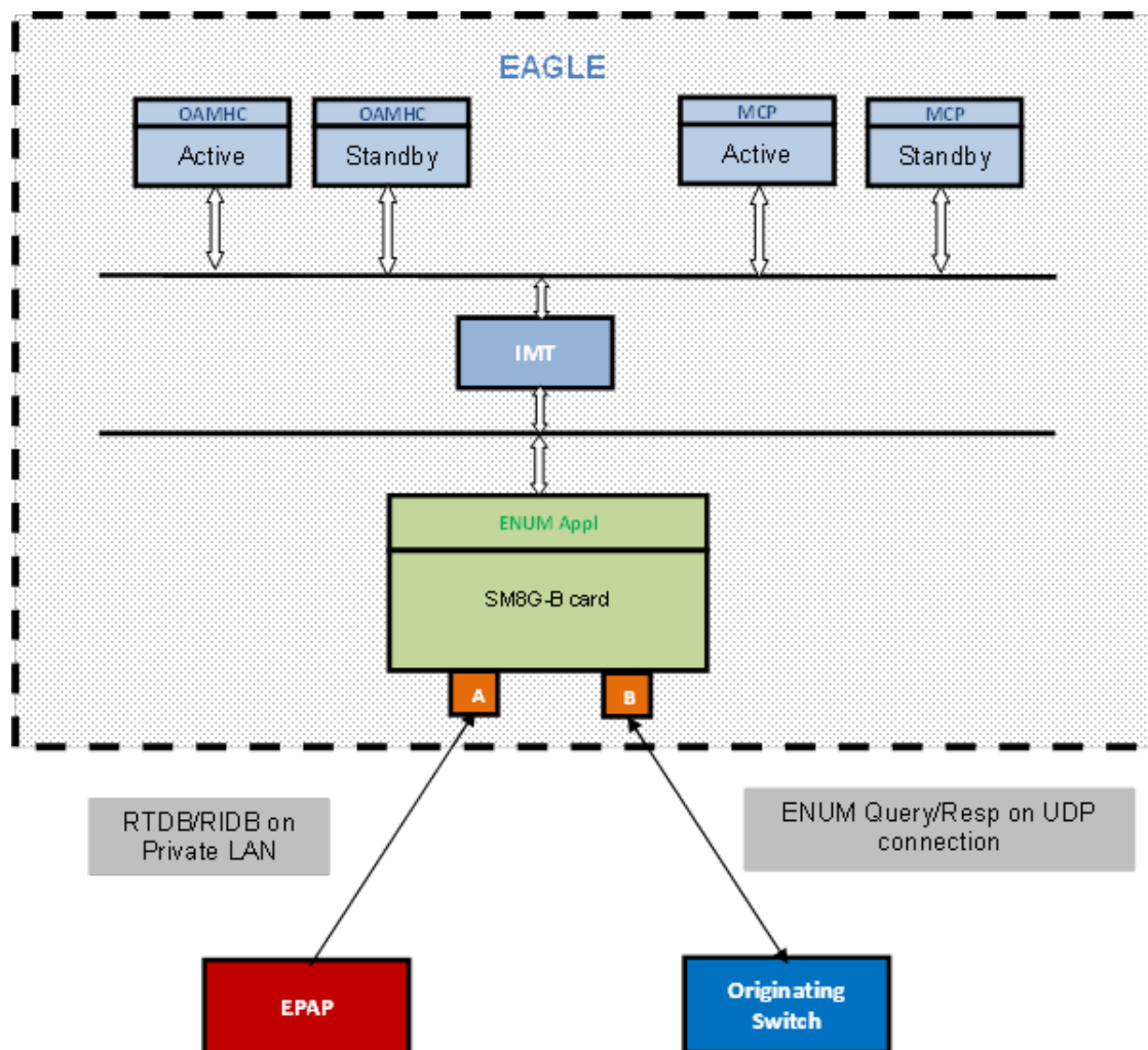
Figure 2-1 ENUM Architecture on EAGLE
