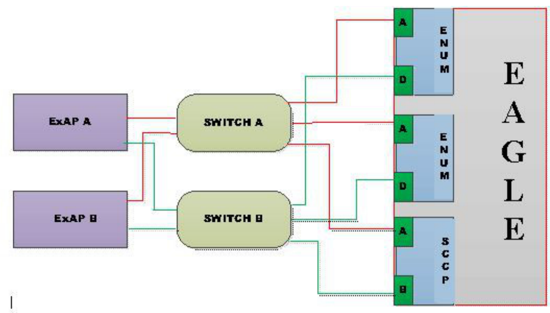
Figure 2-6 SLIC Card Private Network Redundancy
