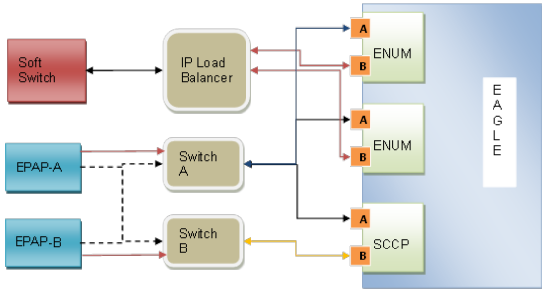
Figure 2-3 Network Redundancy with E5-SM8G-B Cards
