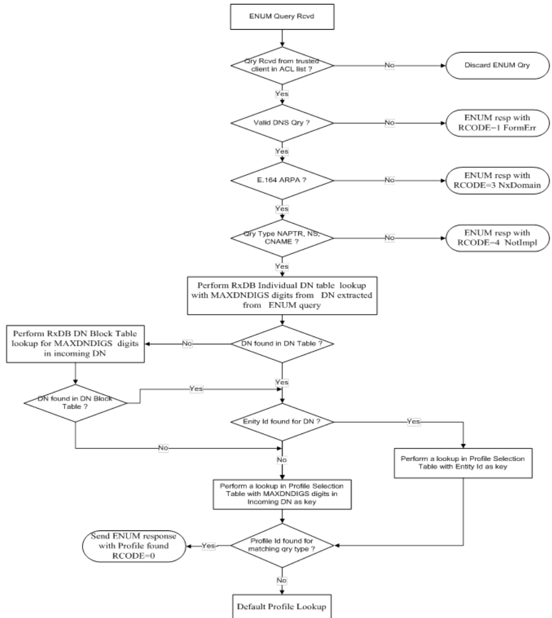
Figure 2-7 ENUM Message Flow for MNP
