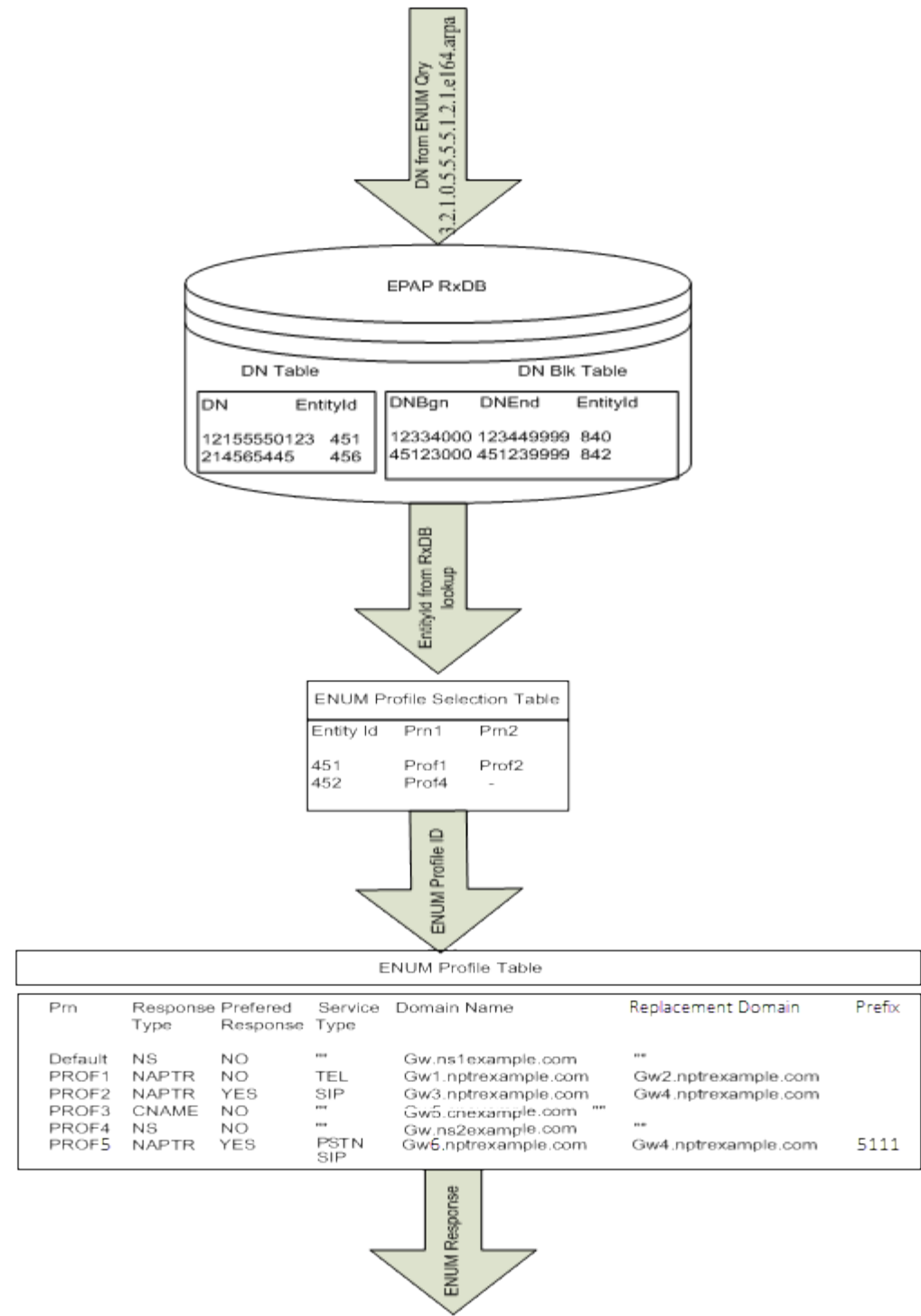
Figure 2-8 ENUM Message Flow within EAGLE
