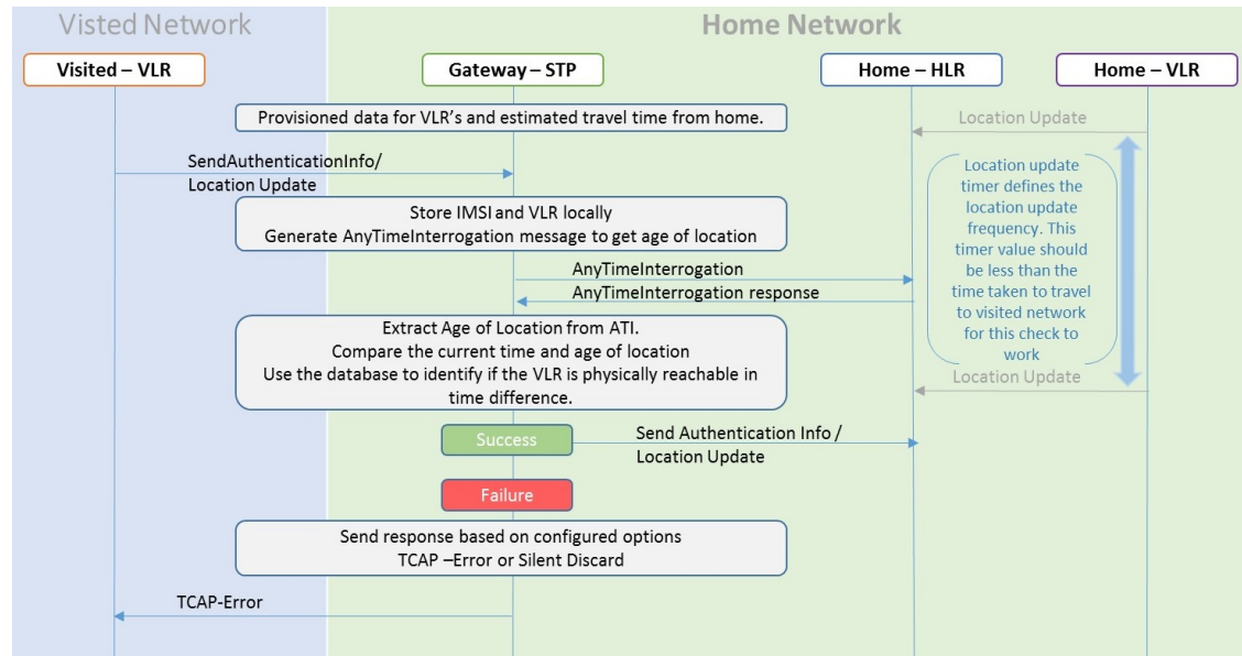
Figure 2-2 Call Flow for Velocity Check Using ATI
