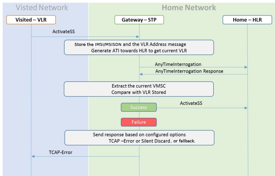
Figure 2-1 Call Flow for VLR Validation
