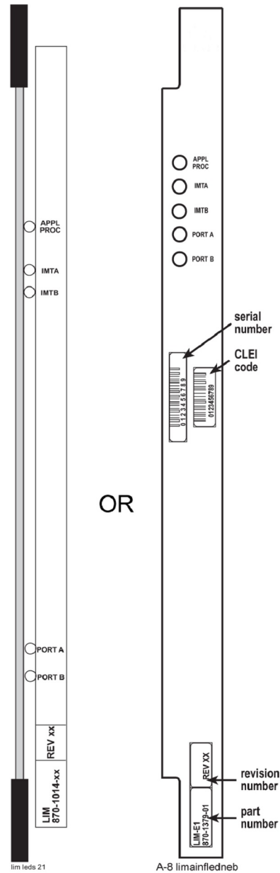
Figure 3-2 Card LEDs
