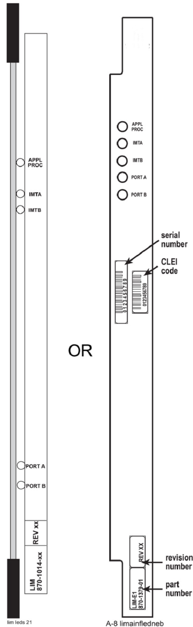
Figure 3-4 Card LEDs
