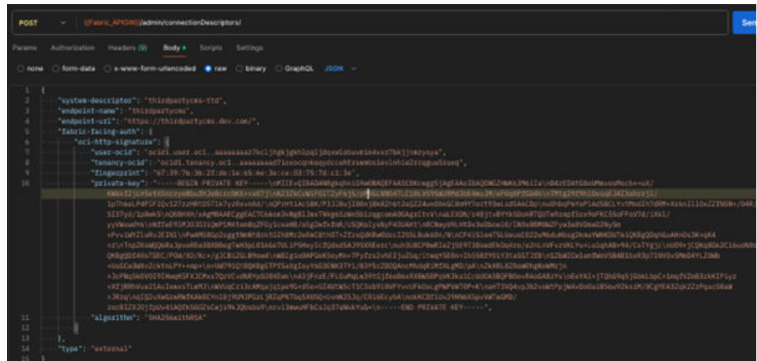
Figure 5-6 Private Key (in Single Line ) in the Payload
