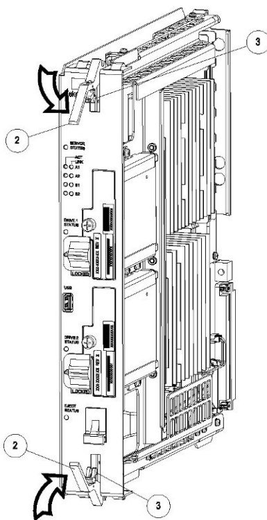
Figure 9-4 E5-APP-B Card Inject Levers
