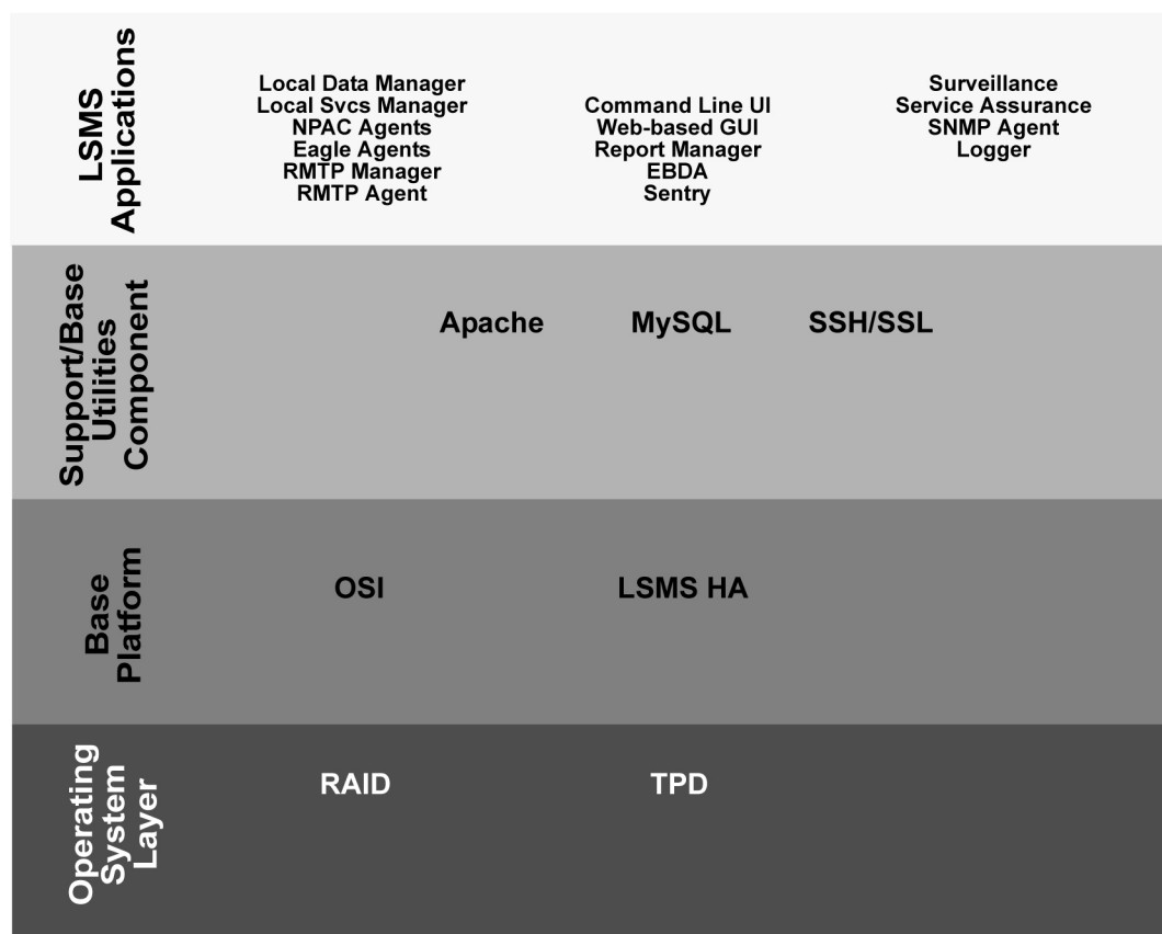
Figure 2-2 Software Allocation on the LSMS Platform
