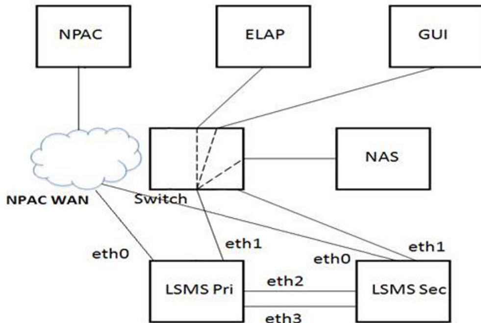
Figure 2-3 Physical Port Assignments - E5-APP-B Segmented Configuration
