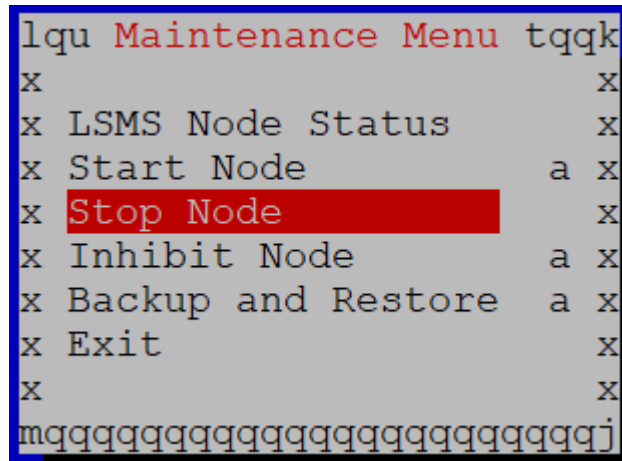
Figure 5-56 Stop Node
