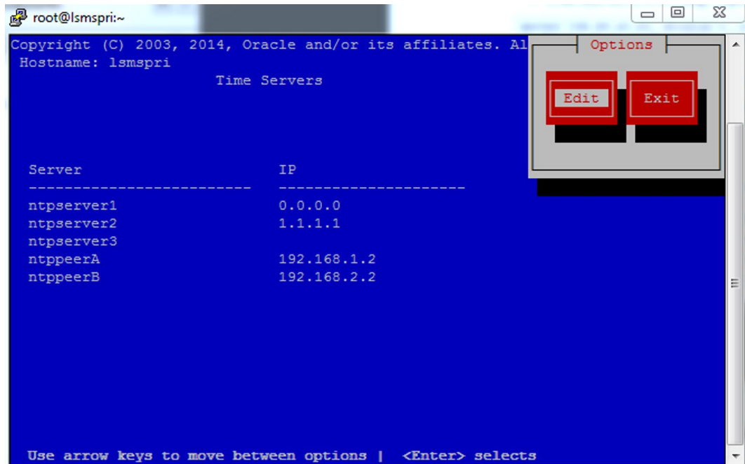
Figure 5-3 Displaying NTP Time Servers Screen
