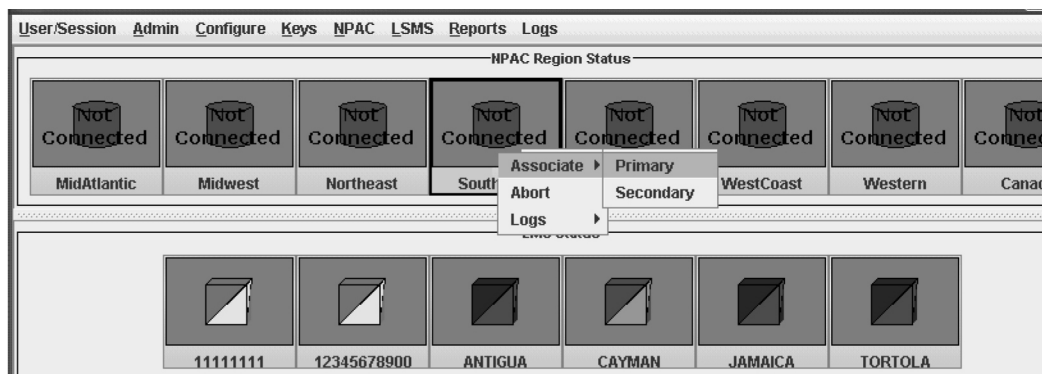
Figure 3-55 Associate with NPAC
