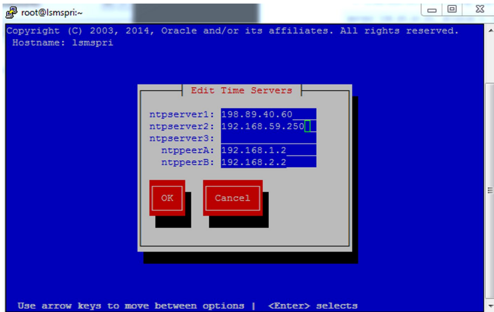
Figure 5-4 Assigning an NTP Server to the LSMS
