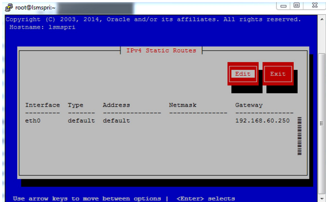
Figure 2-8 Displaying Current System Routes
