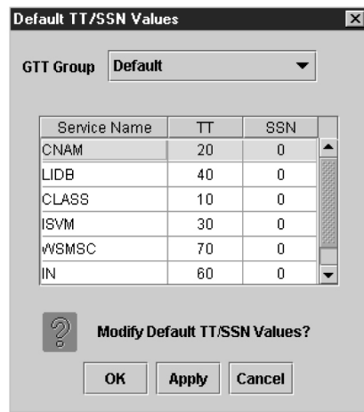
Figure 3-52 Changing Default TT/SSN Values
