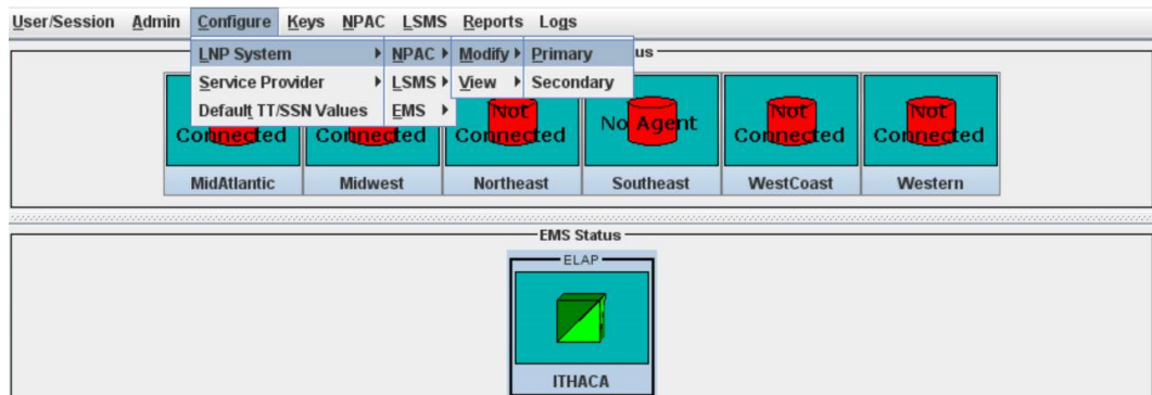
Figure 3-47 LSMS Console
