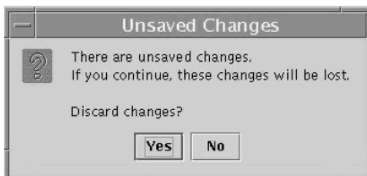
Figure 5-15 Confirmation Dialog
