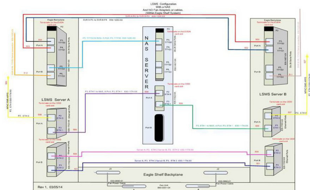
Figure 2-1 LSMS Configuration: Single Subnet Backplane Connections
