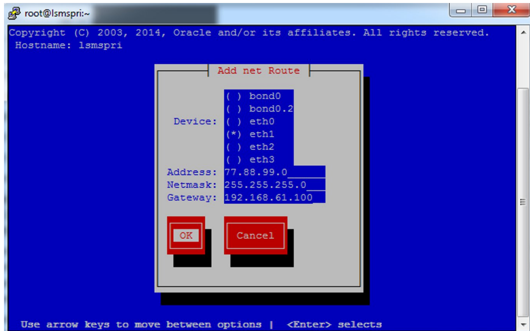
Figure 2-12 Entering a New Add net Route Screen
