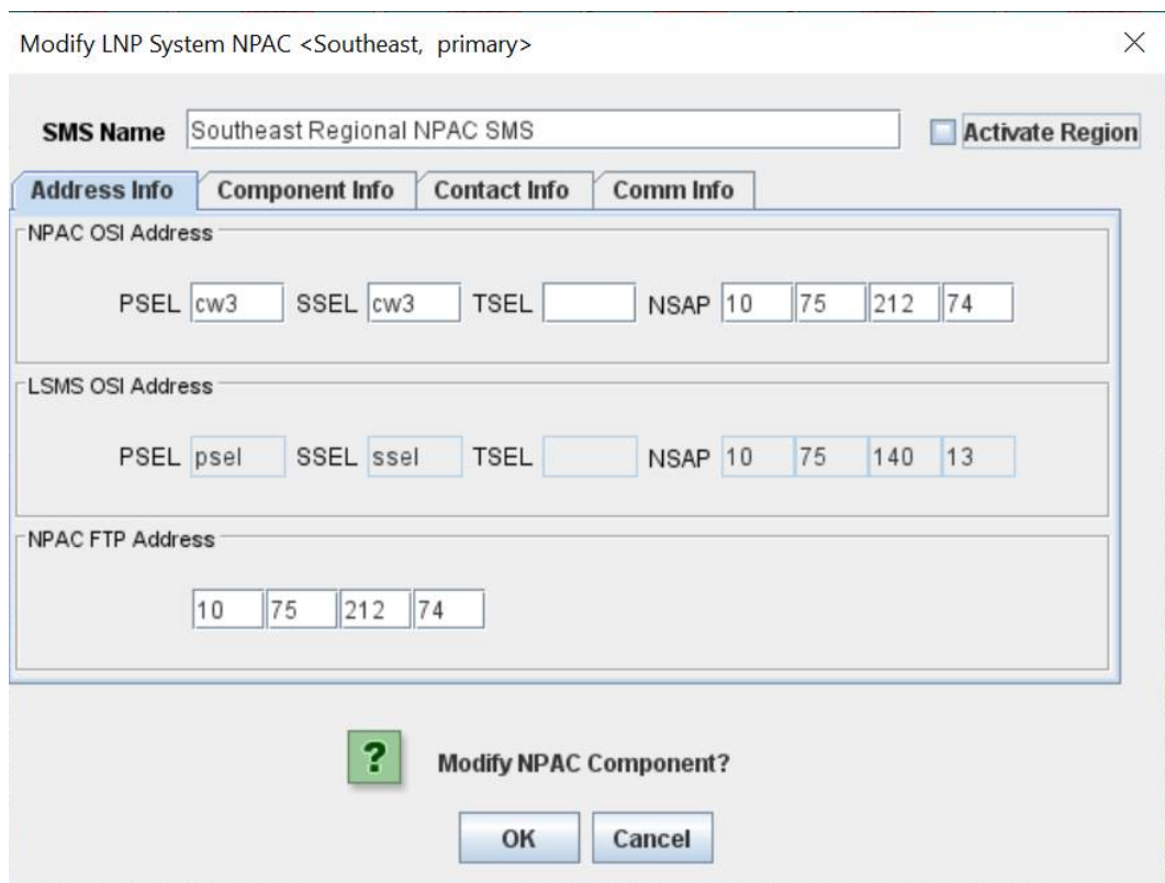
Figure 3-48 Modify LNP System NPAC
