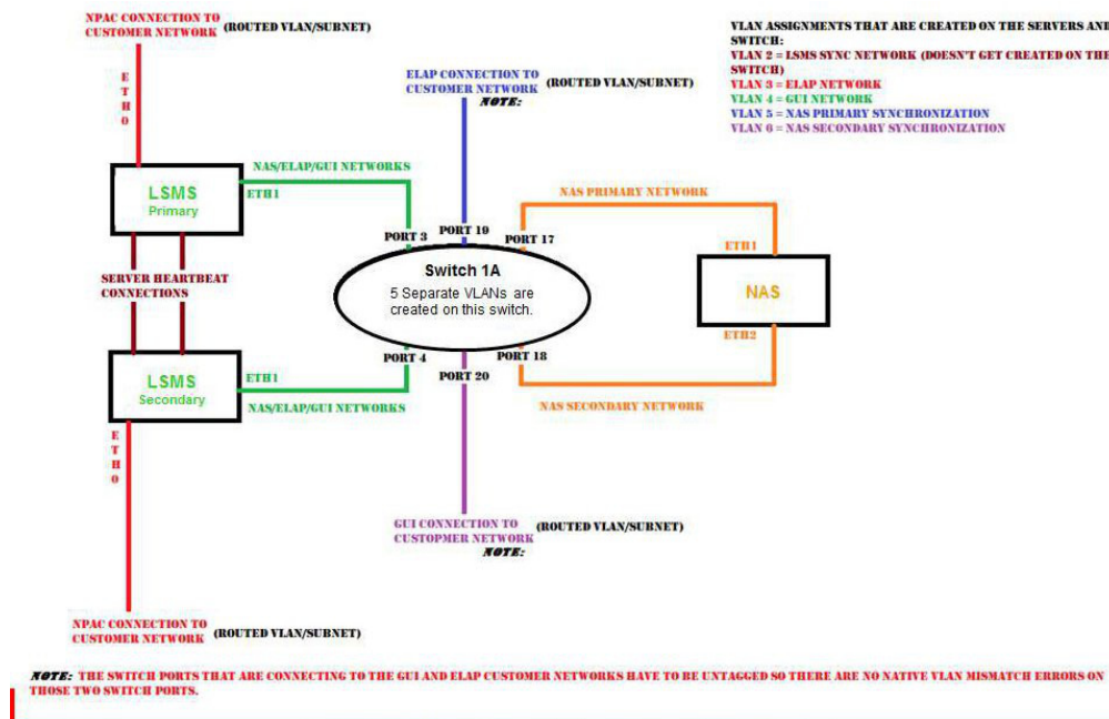
Figure 2-4 LSMS Configuration: Segmented Configuration
