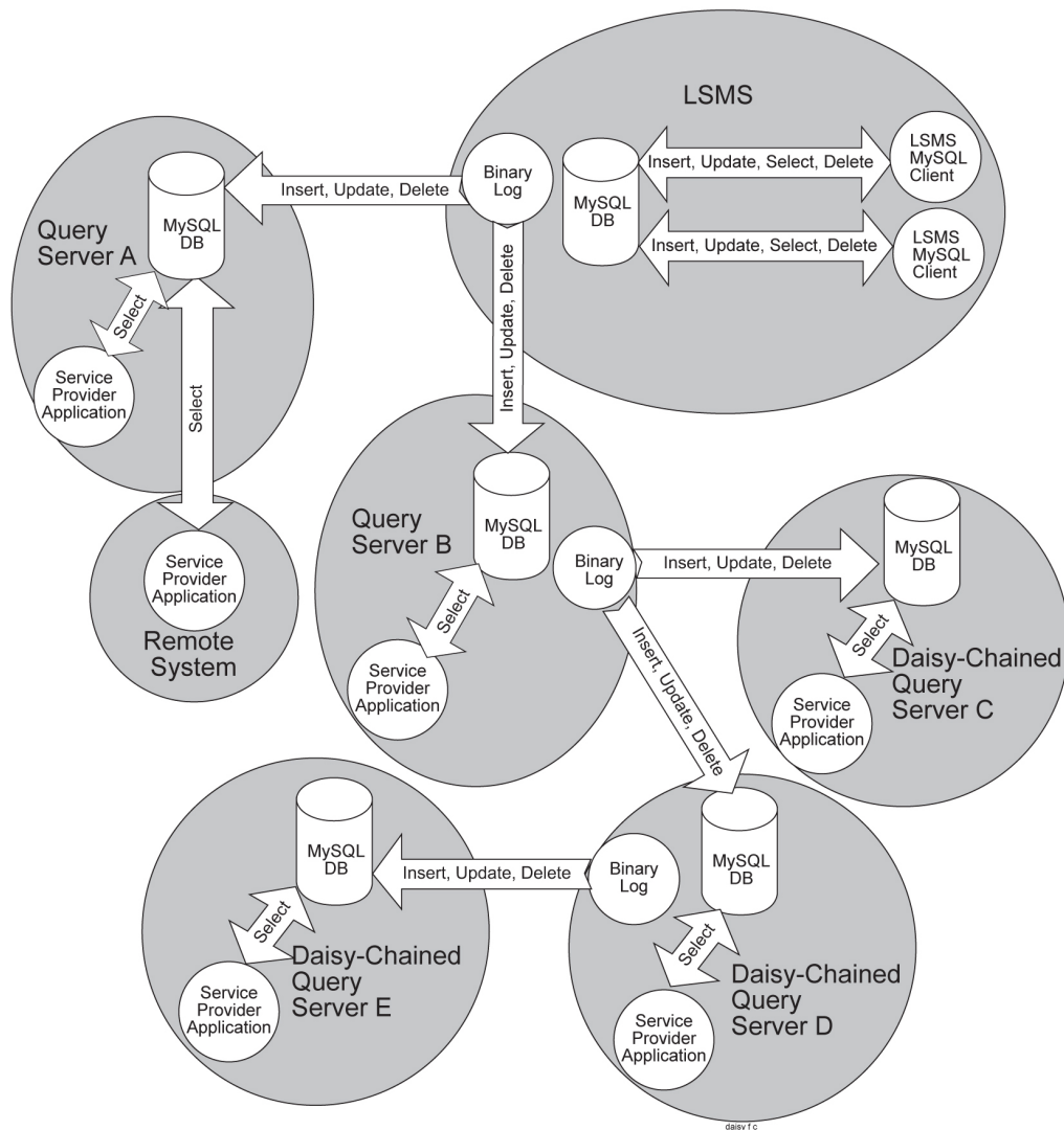
Figure A-2 LSMS Query Server Configuration Scenario
