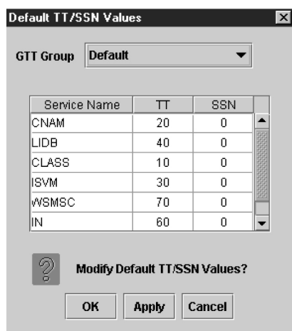
Figure 3-51 Default TT/SSN Values Window
