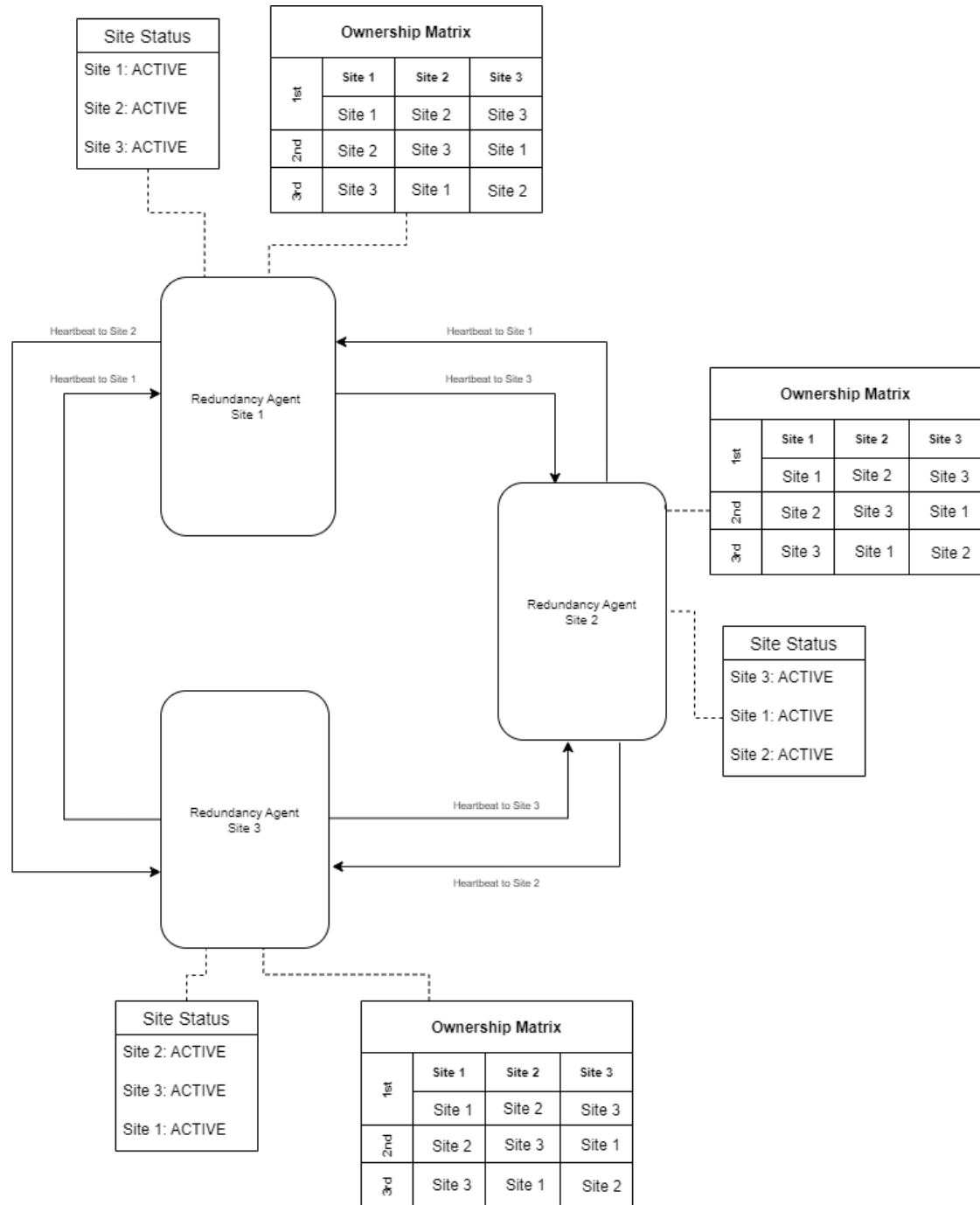
Figure 3-6 Three-Site Georedundancy
