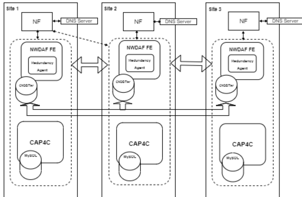
Figure 3-2 Georedundant Architecture
