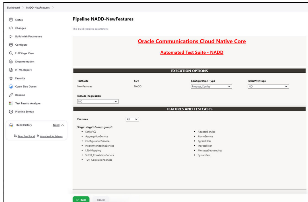
Figure 4-5 Pipeline NADD_NewFeatures
