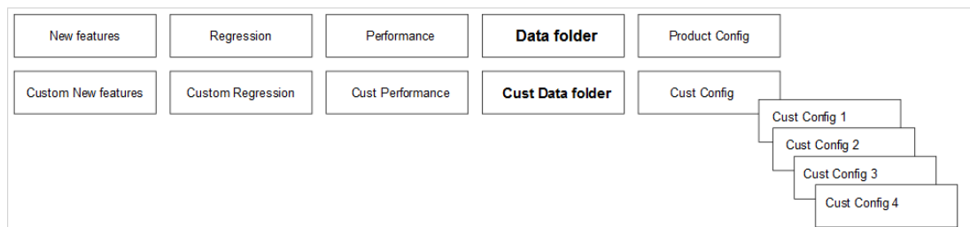
Figure 2-59 Folder Structure
