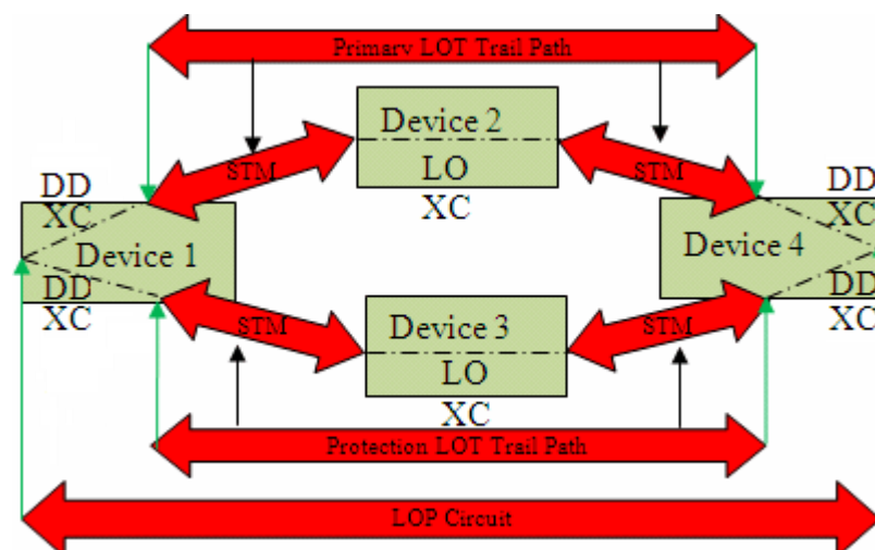
Figure 5-3 Fully-Protected LOP
