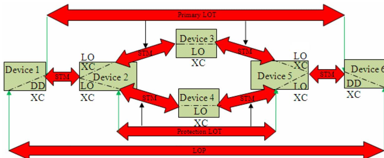
Figure 5-4 Partially-Protected LOP
