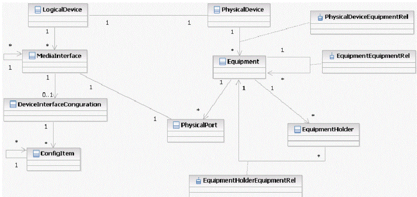
Figure 4-1 UIM Integration Cartridge UML Representation
