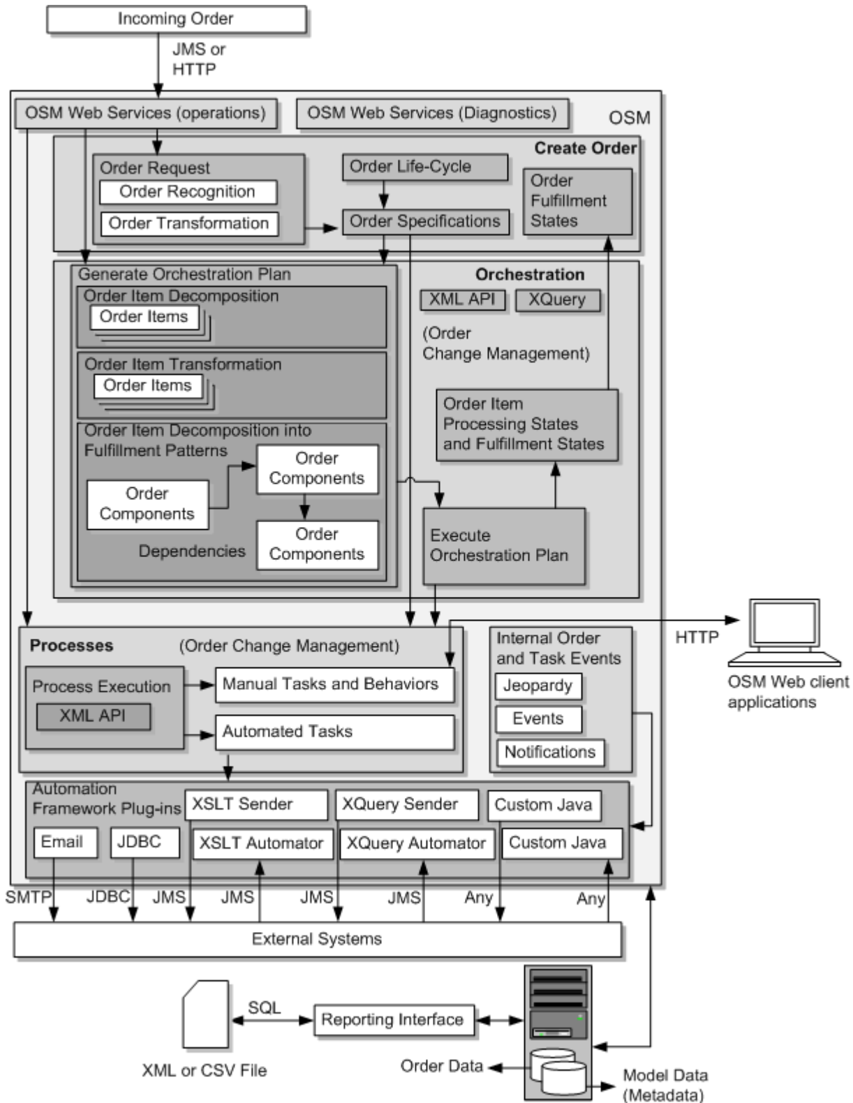
Figure 8-1 OSM Functional Diagram
