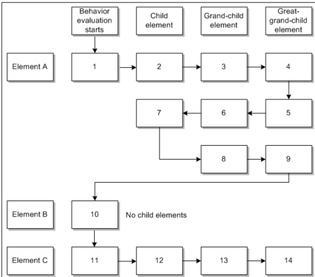
Figure 9-3 Element Selection
