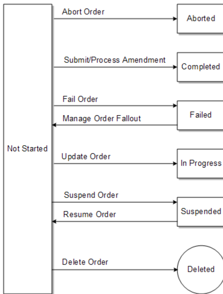
Figure 3-14 Order States that Can Transition to or from the Not Started Order State
