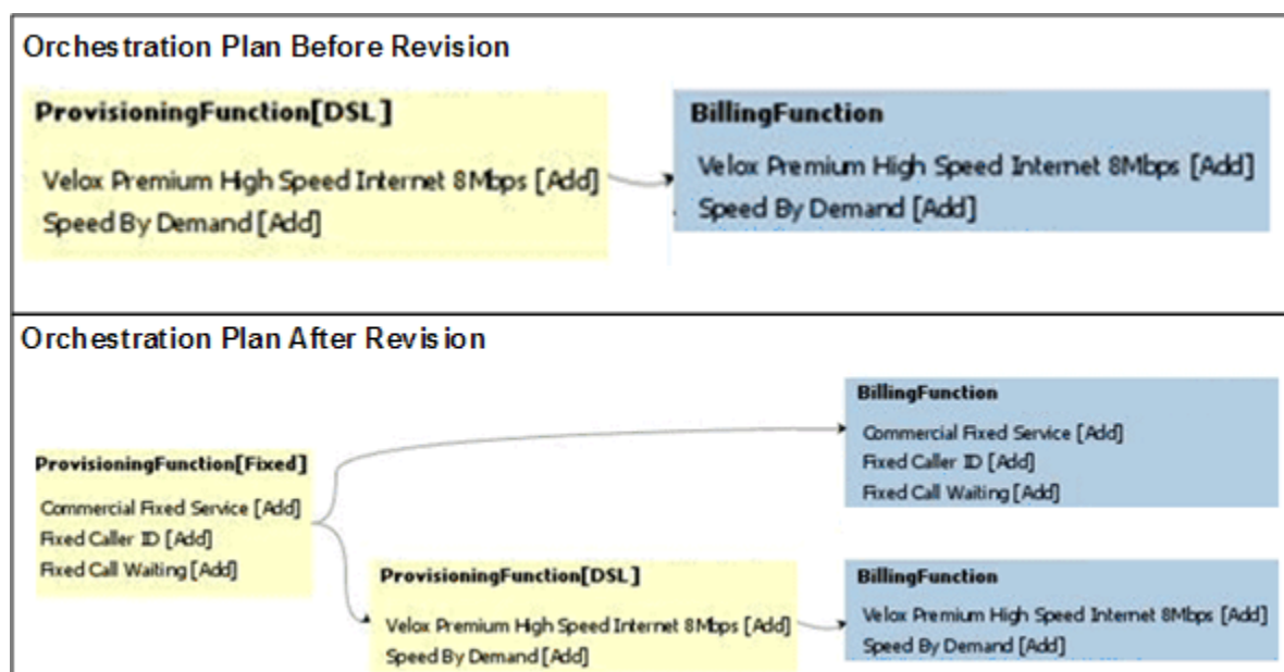
Figure 10-22 Orchestration Change Due to Revision: Add Service to Order
