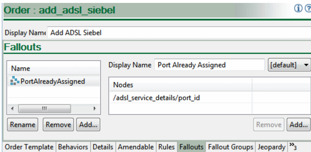
Figure 11-3 Fallout Defined in an Order
