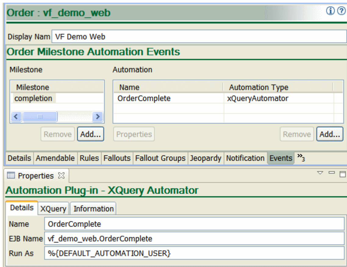
Figure 13-4 Event Notification Based on an Order Milestone
