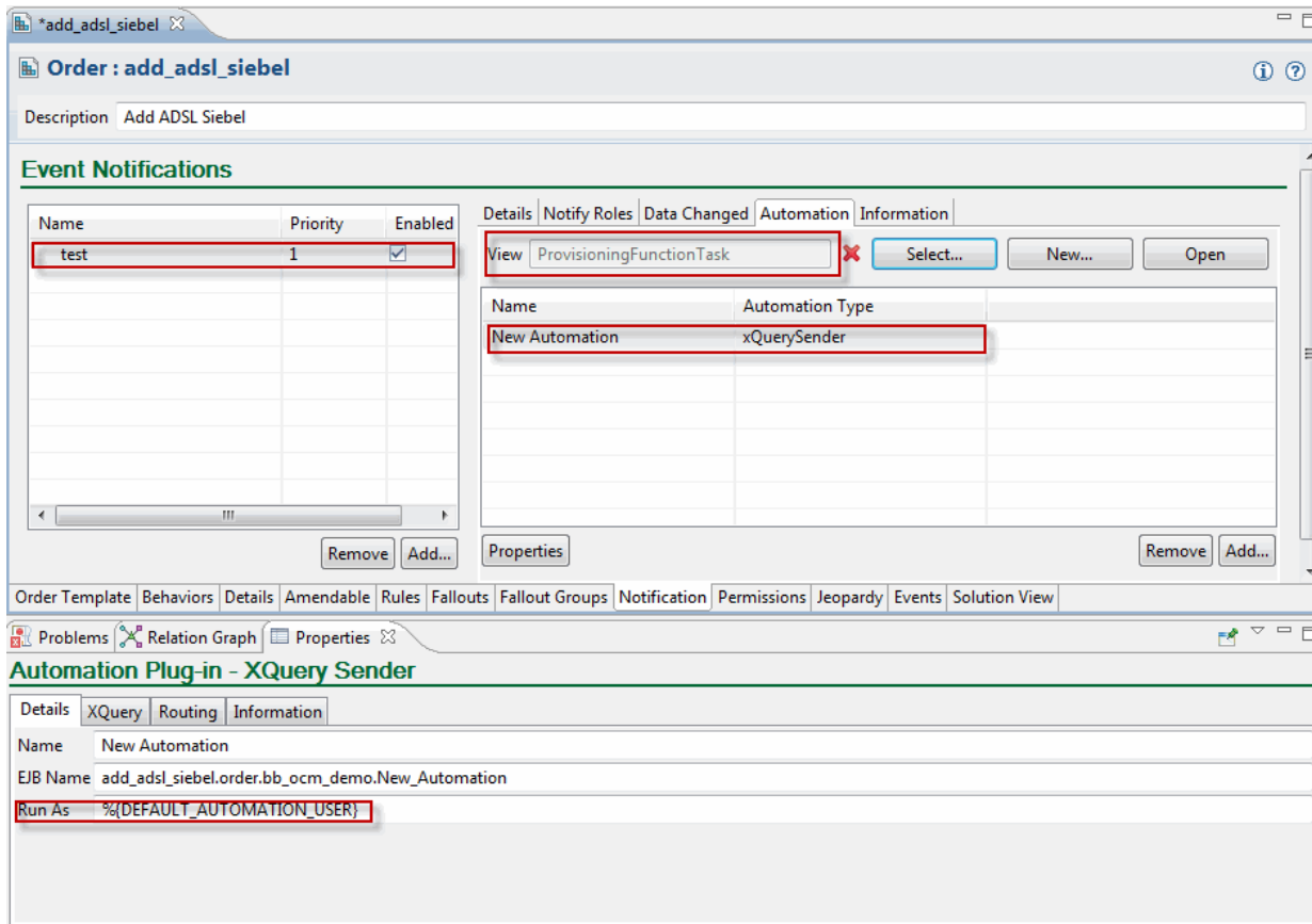
Figure 7-14 Order Event Notification Automation Query Task
