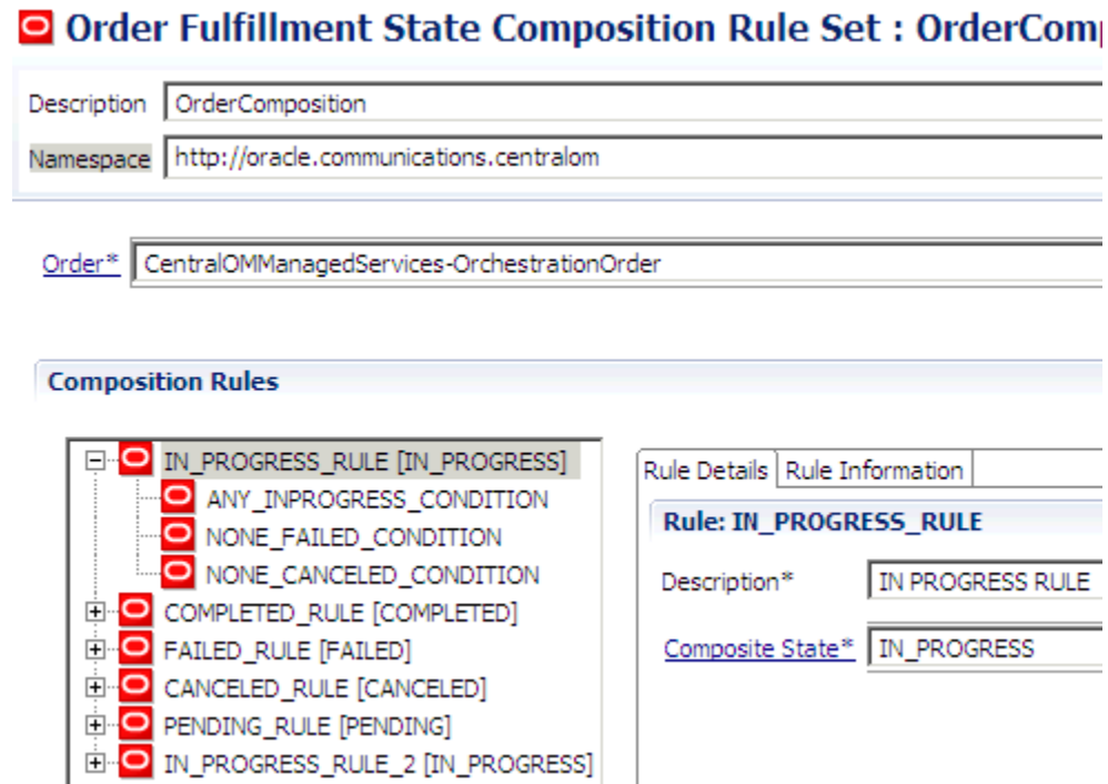
Figure 12-3 Detail from Order Fulfillment State Composition Rule Set Editor
