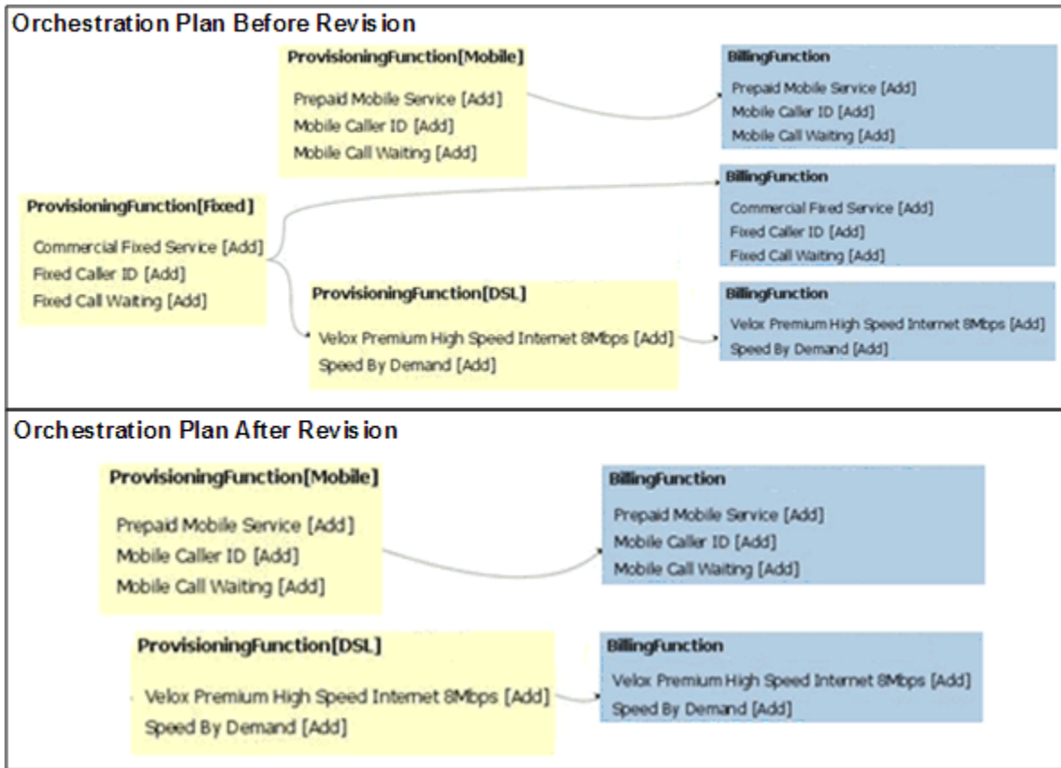
Figure 10-21 Orchestration Change Due to Revision: Remove Service From Order
