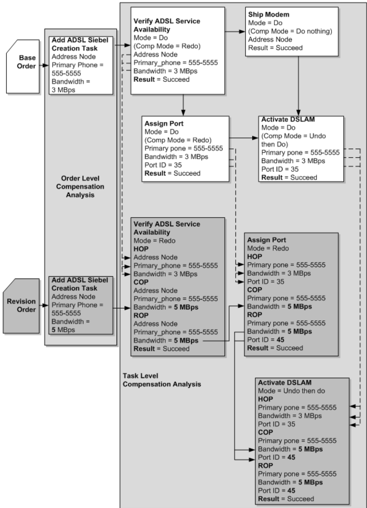
Figure 10-8 Changing a Service Request
