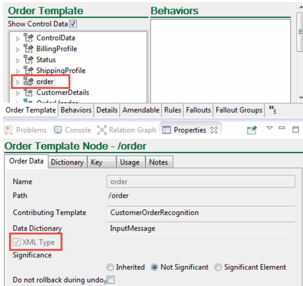
Figure 8-3 Input Order Data as XML Type
