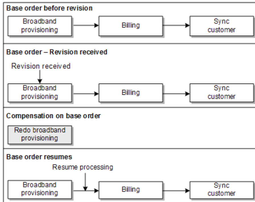
Figure 10-17 Example of Compensation that Occurs During Provisioning
