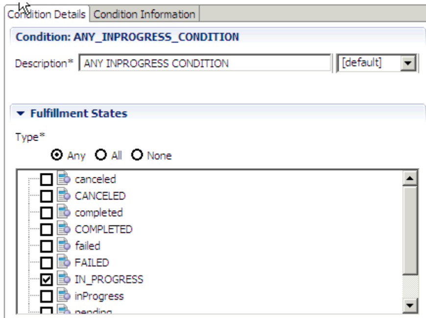
Figure 12-4 Fulfillment States Section of Condition Details Subtab
