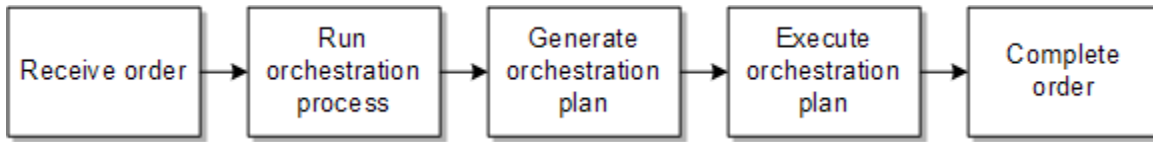
Figure 2-3 Orchestration-Based Order
