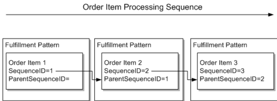
Figure 5-24 Order Item Processing Sequence
