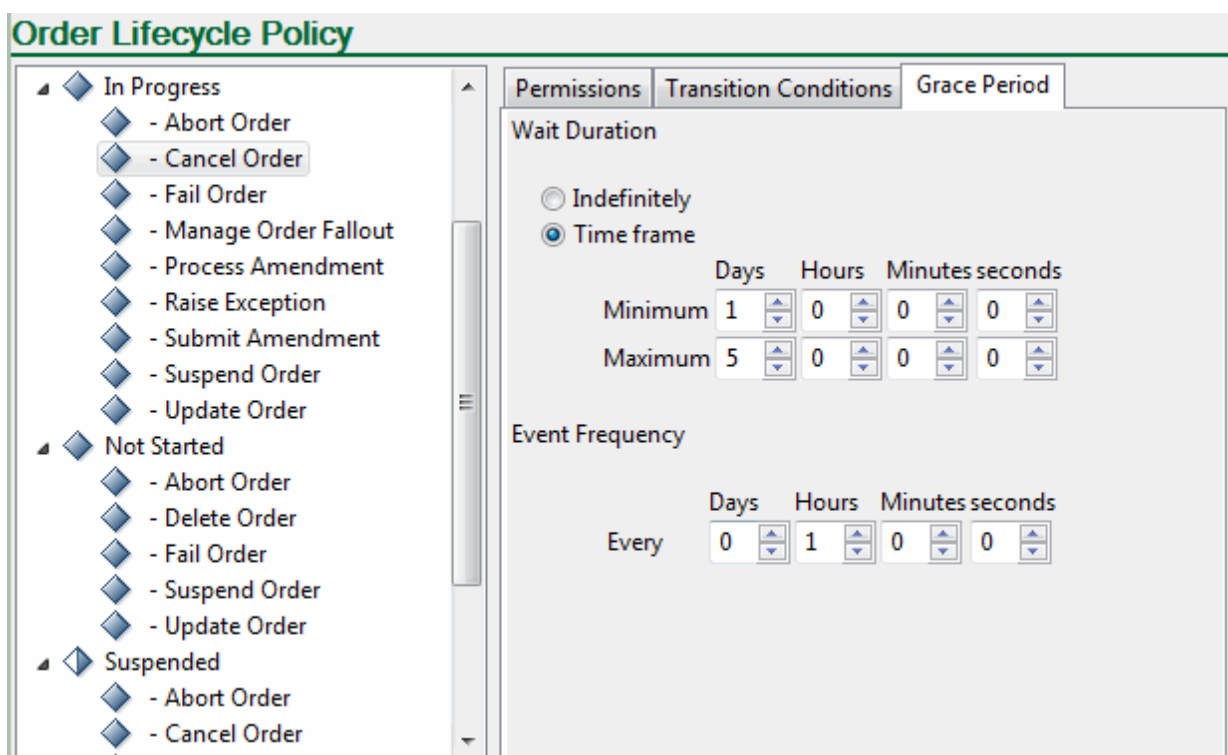
Figure 3-2 Order Life Cycle in Design Studio
