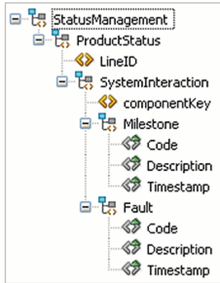
Figure 8-9 Status Data in Order Item
