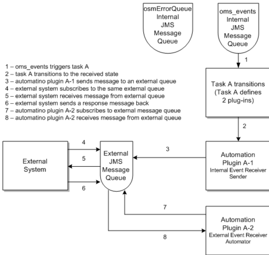
Figure 11-2 Automation Flow: Simple Synchronous
