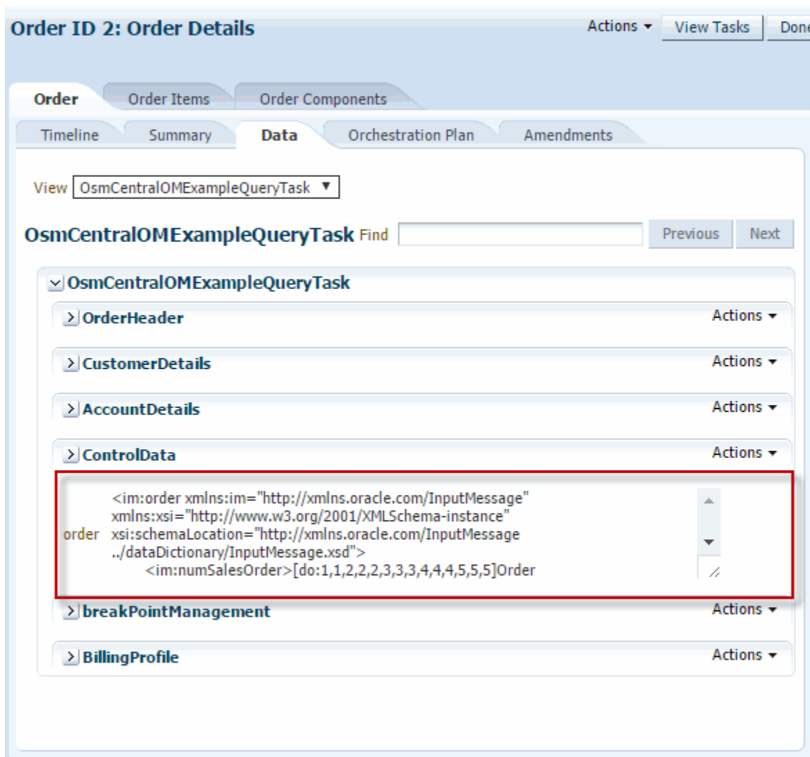
Figure 8-4 Order Management Web Client Input Order Data XML Structure
