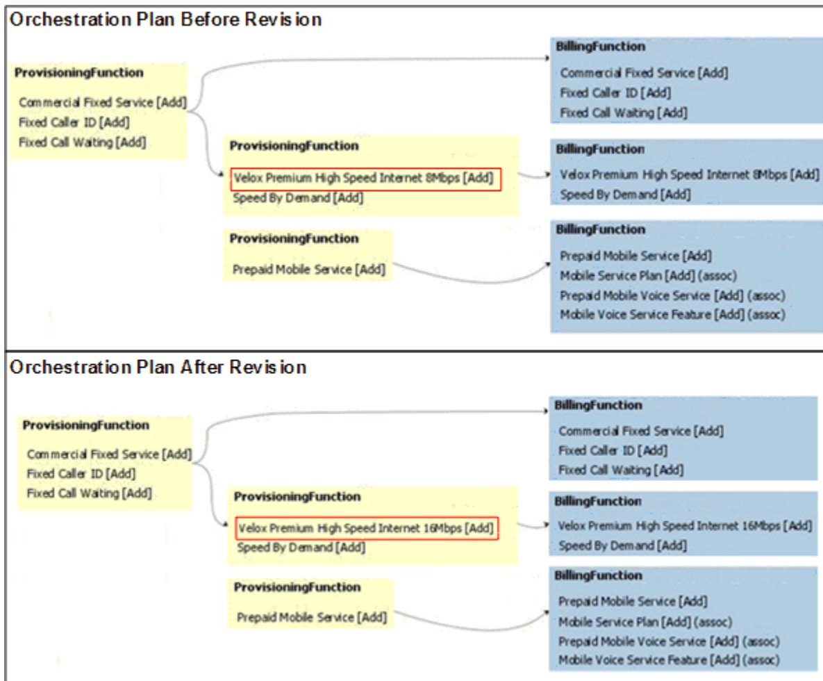
Figure 10-20 Orchestration Change Due to Revision: Change Service Attribute
