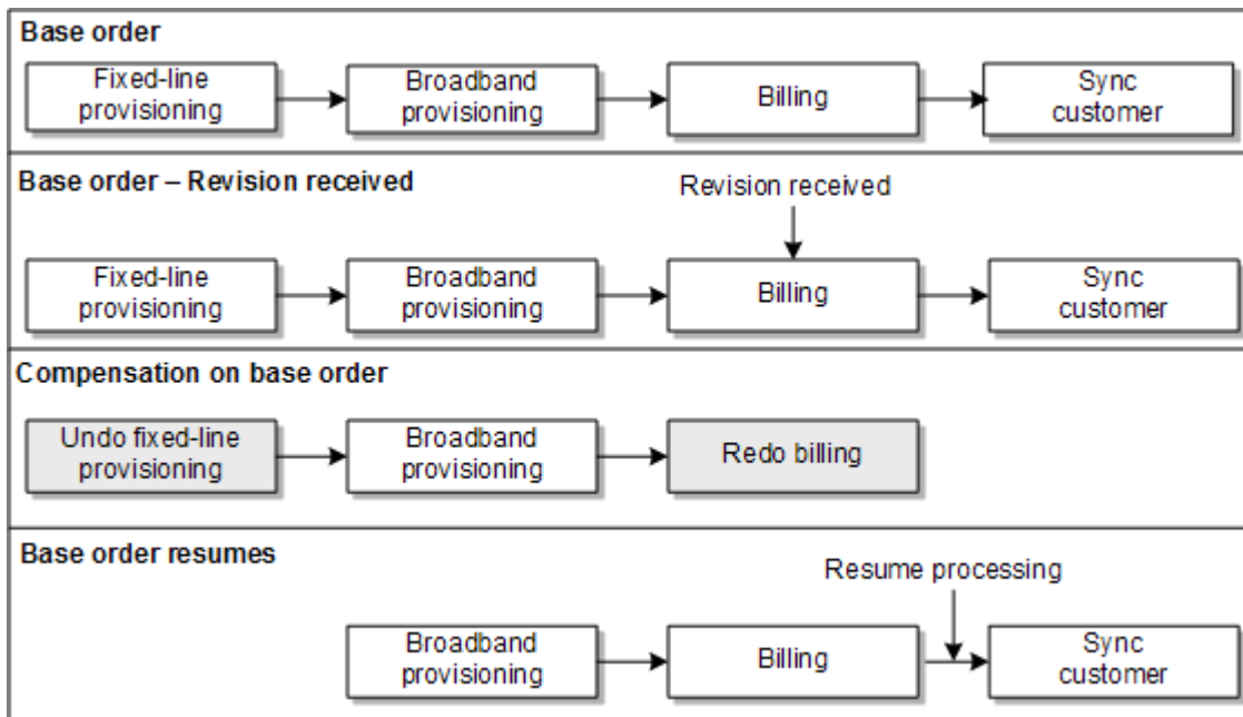
Figure 10-18 Compensation for Removing a Service
