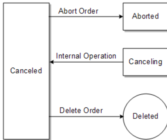
Figure 3-8 Order States that Can Transition to or from the Canceled Order State if the Order Has an Orchestration Plan
