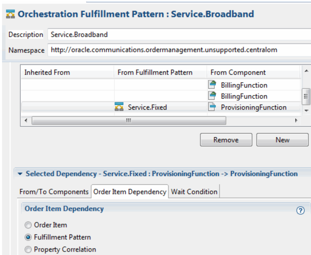
Figure 5-20 Dependency Based on Fulfillment Pattern
