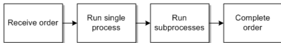
Figure 2-2 Process-Based Order
