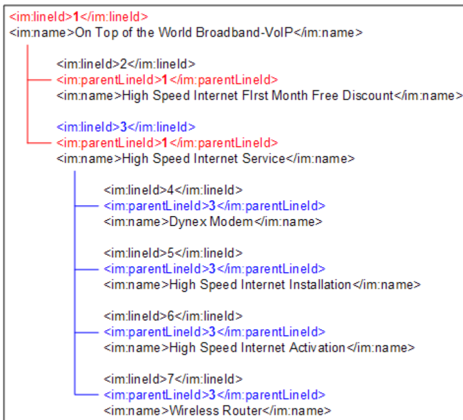
Figure 5-10 Item Hierarchies in an Incoming Customer Order
