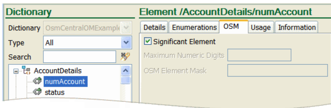
Figure 10-11 Data Significance Specified in the Data Dictionary
