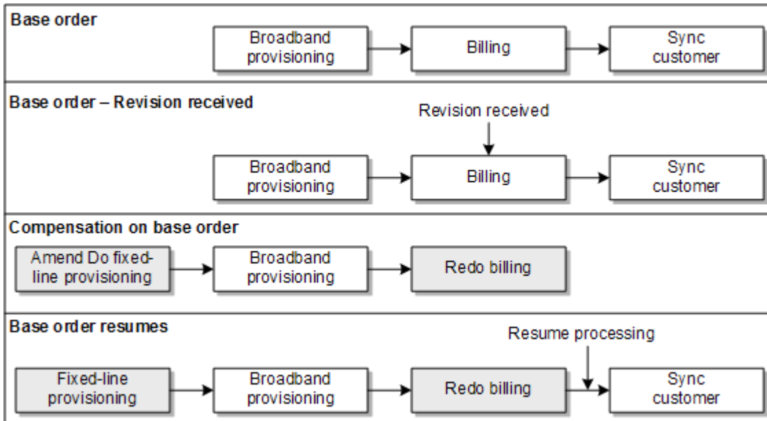
Figure 10-19 Compensation for Adding a Service
