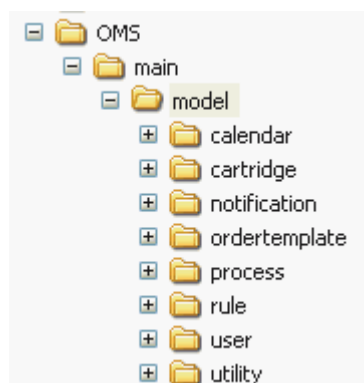
Figure 9-1 Uncompressed Files
