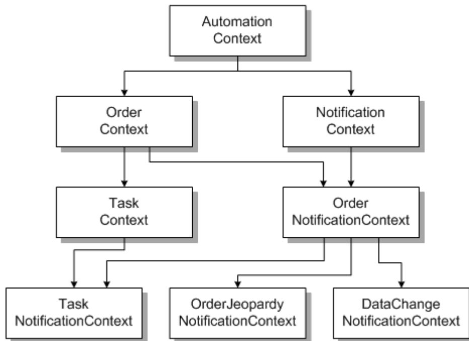
Figure 7-2 Context Object Class Hierarchy
