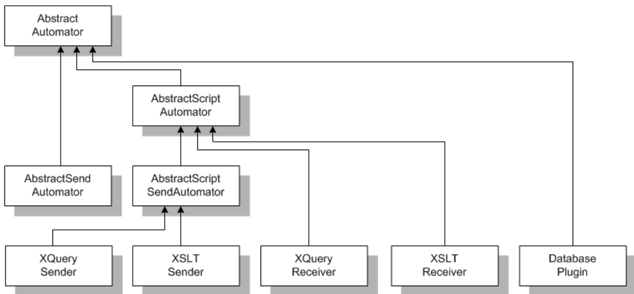
Figure 7-9 Predefined Automation Plug-in Class Hierarchy
