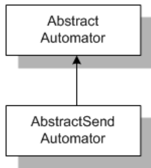
Figure 7-8 Class Hierarchy
