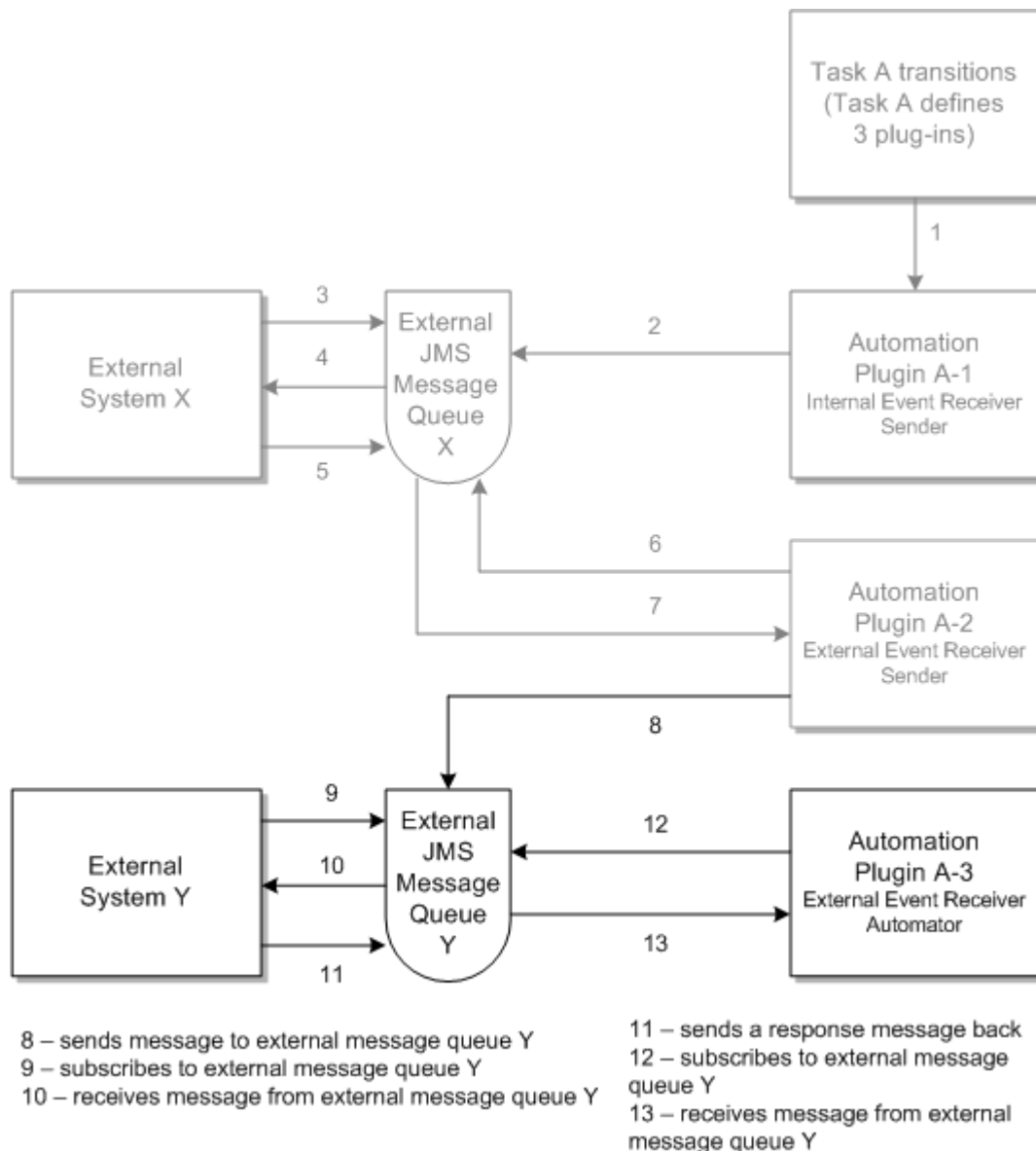
Figure 8-6 Automation Flow: Complex Synchronous
