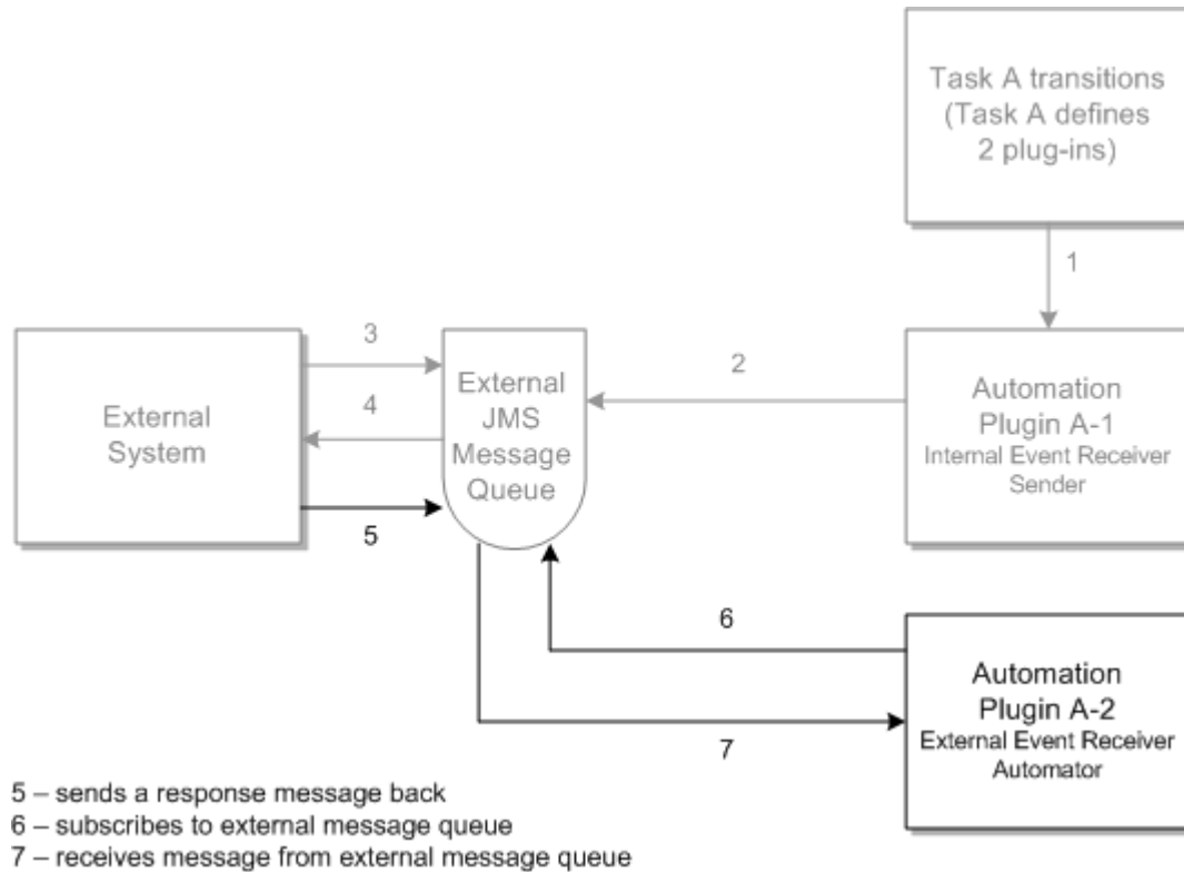
Figure 8-5 Automation Flow: Simple Synchronous
