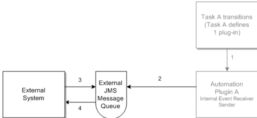
Figure 8-4 Automation Flow: Fire-and-Forget
