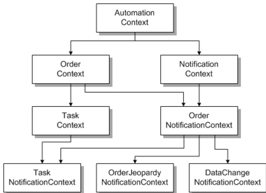
Figure 8-2 Context Object Class Hierarchy
