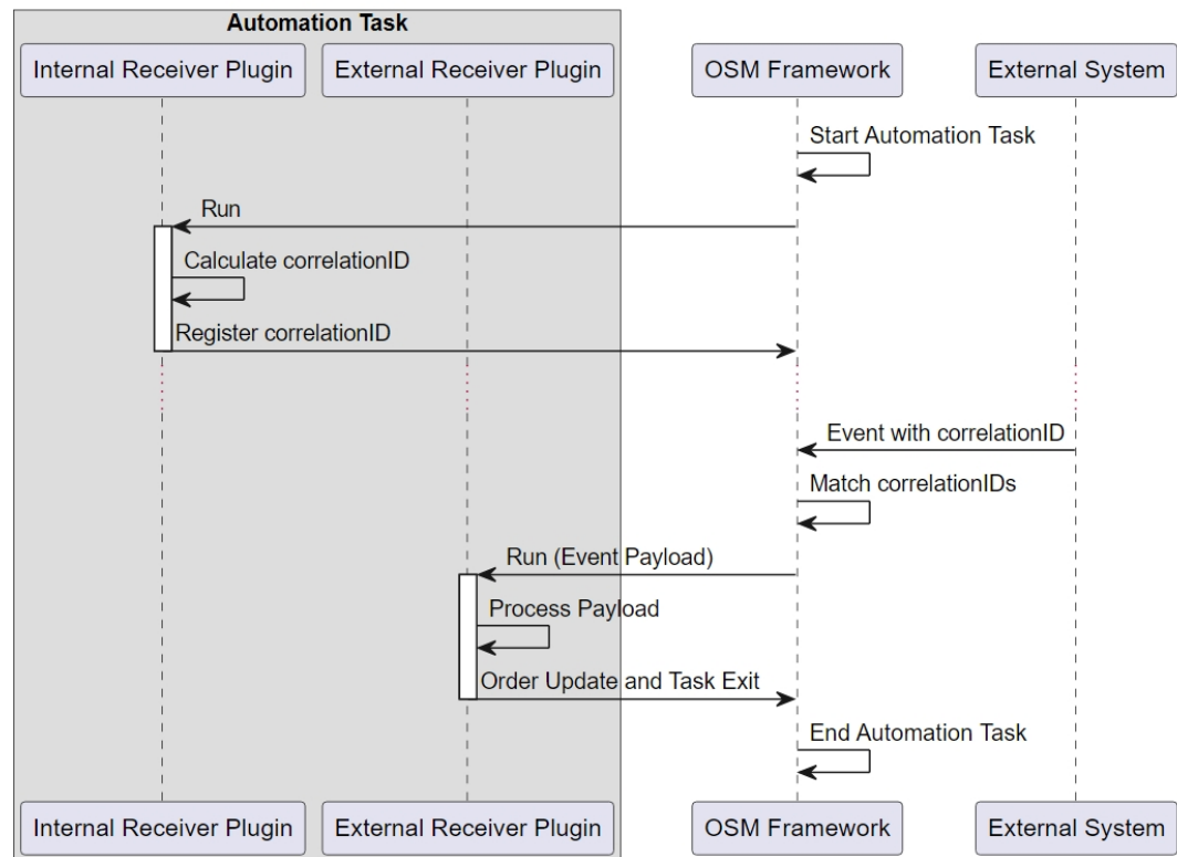
Figure 8-13 System Interaction Receiver Only
