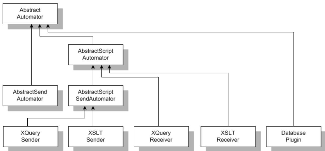
Figure 8-9 Predefined Automation Plug-in Class Hierarchy
