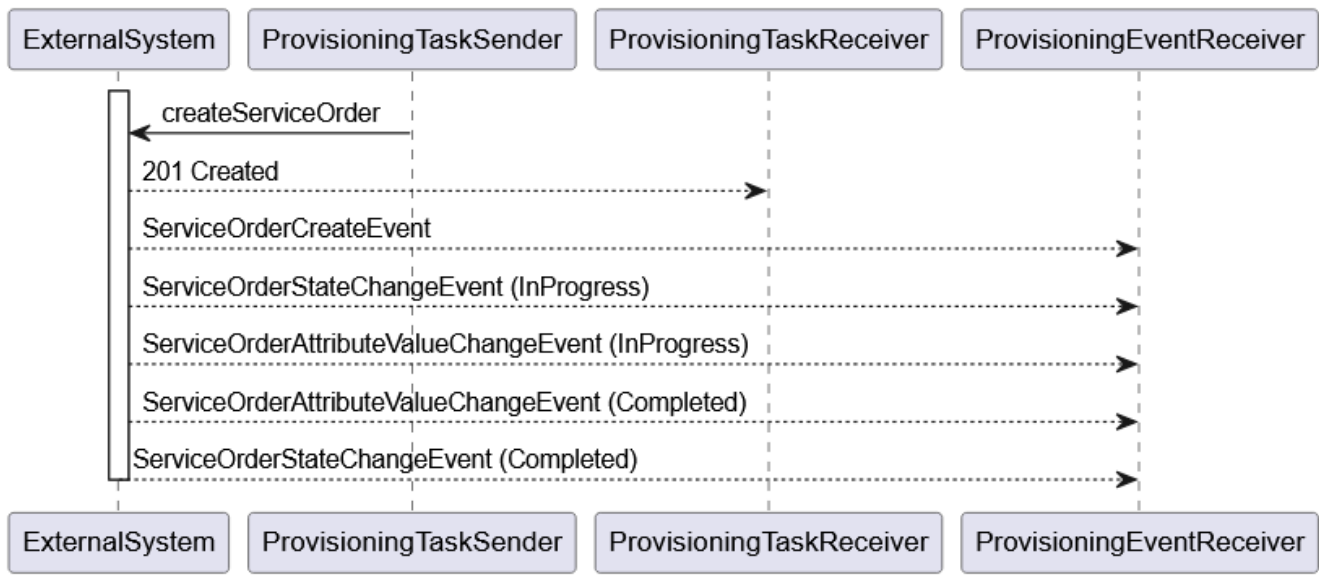
Figure 8-12 Typical REST Interaction
