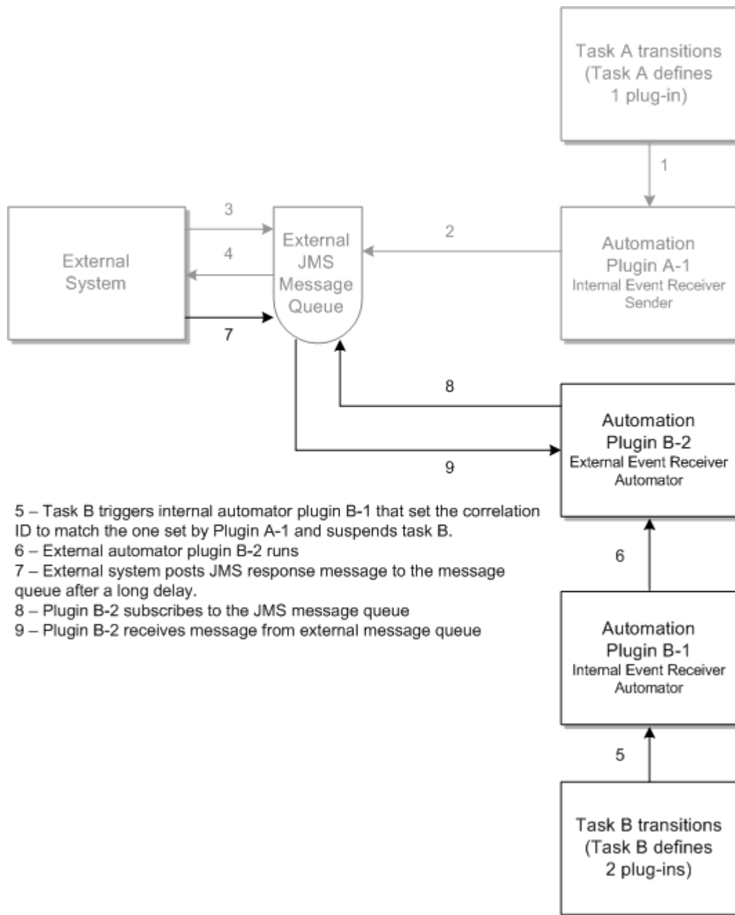
Figure 8-7 Automation Flow: Simple Asynchronous
