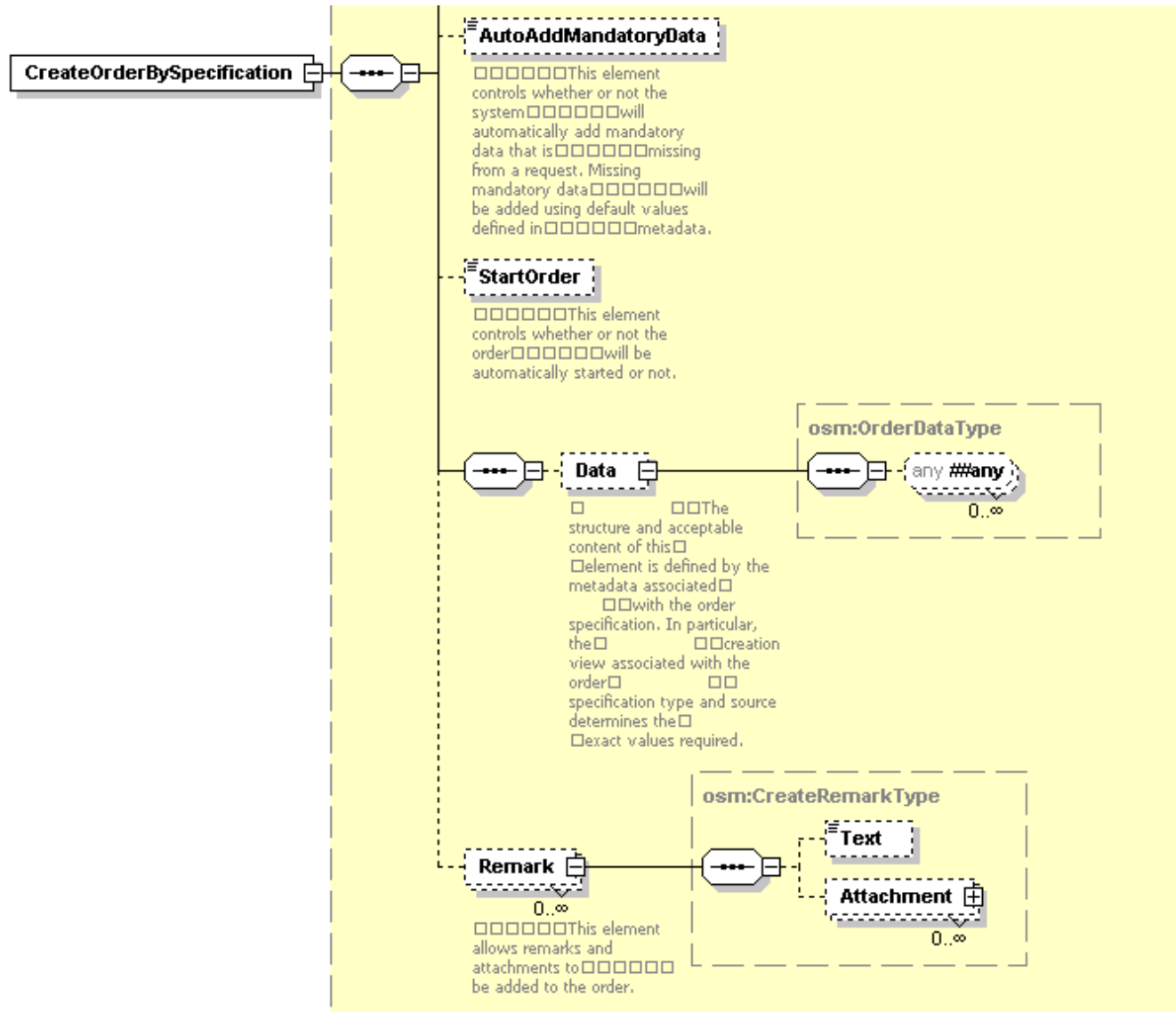
Figure 2-5 Further Expansion of Data and Remark Elements
