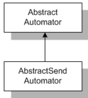
Figure 8-8 Class Hierarchy
