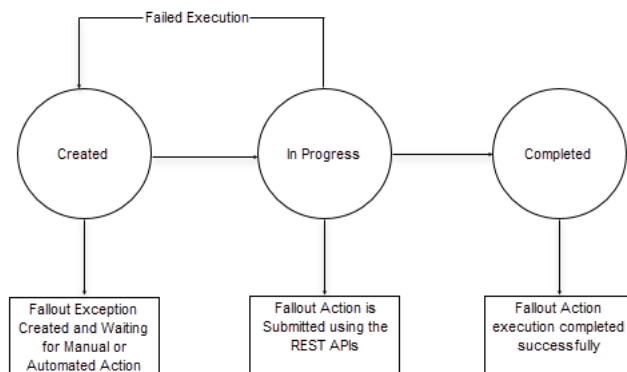
Figure 5-1 Fallout Exception Lifecycle
