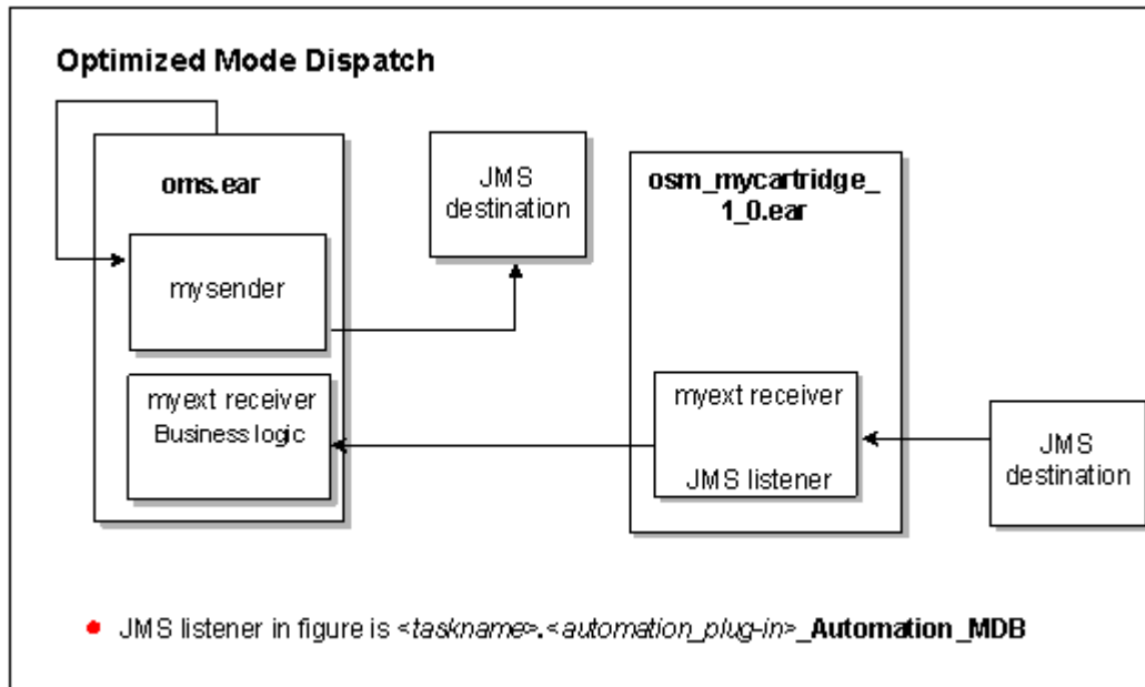
Figure 8-11 Dispatch of Automation Plug-ins
