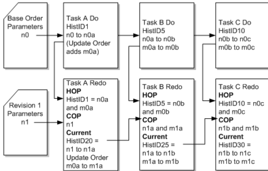
Figure 8-10 Update Orders in Task Compensation Analysis
