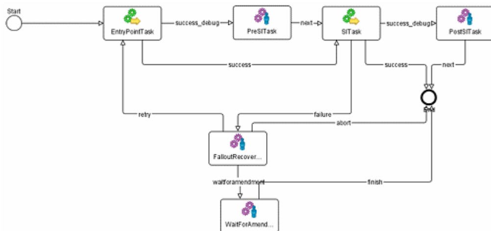
Figure 5-1 Creating Subprocesses
