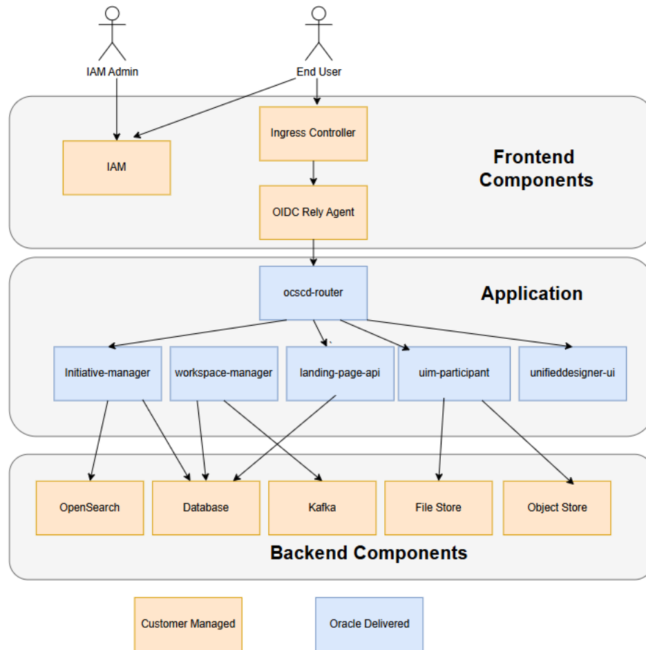
Figure 1-1 Solution Designer Architecture
